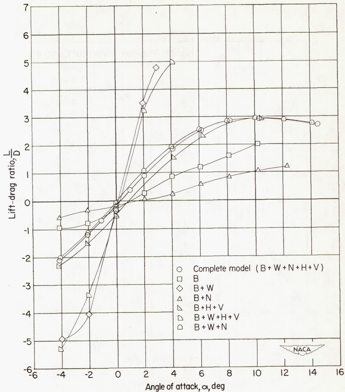
Figure 12.- Lift-drag ratio L/D as a function of angle of attack for the complete basic model and various combinations of its components. M = 1.61 .
