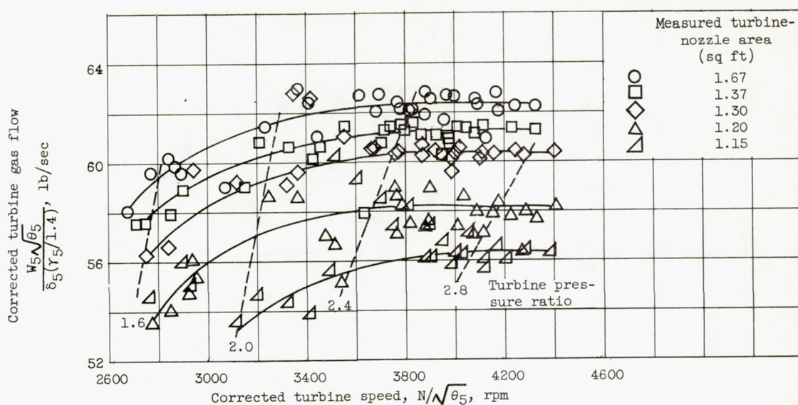
Figure 8. - Effect of turbine-nozzle area and corrected turbine speed on corrected turbine gas flow. Altitude, 30,000 feet; flight Mach number, 0.62.
