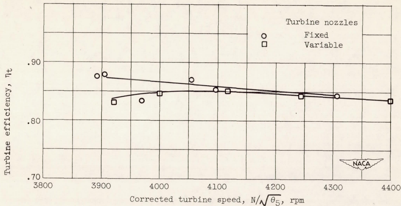
Figure 17. - Comparison of efficiencies obtained with fixed turbine nozzles and with variable-area turbine nozzles for an actual turbine-nozzle area of 1.30 square feet. Altitude, 30,000 feet; flight Mach number, 0.62; engine speed, 7260 rpm.
