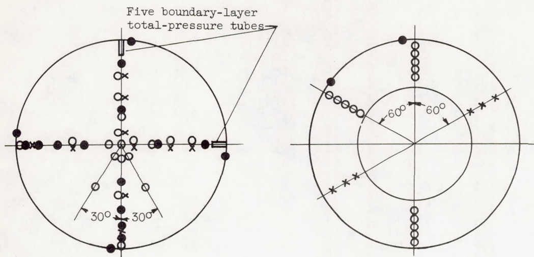
(b) Station 4, compressor outlet. Passage height, 3\frac{1}{8} inches; location, \frac{1}{2} inch downstream of trailing edge of fixed vanes.
