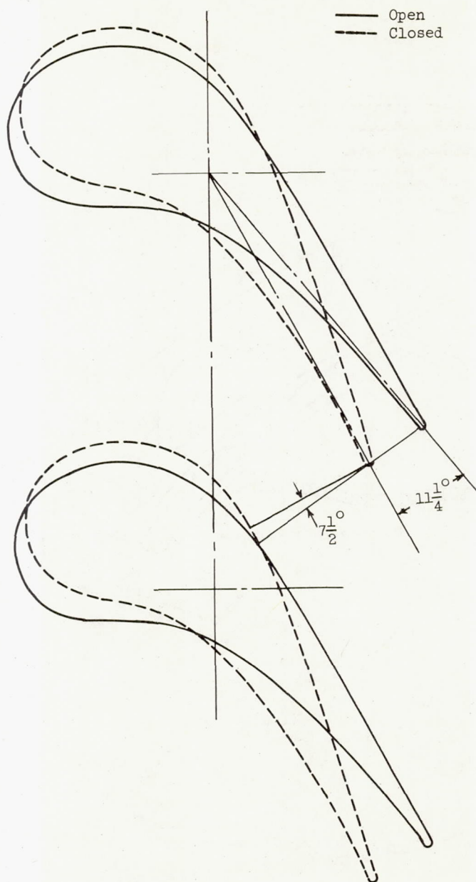
(a) Mid-vane cross-sections of two adjacent vanes ( 2\frac{1}{2} times actual size).
