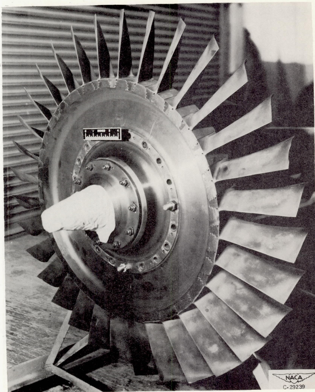
(b) Second-stage turbine rotor.
