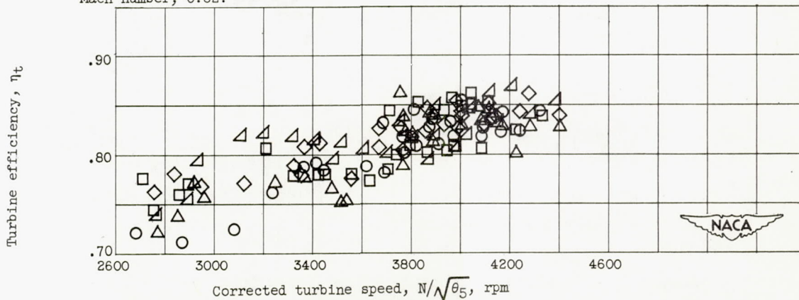
Figure 10. - Effect of turbine-nozzle area and corrected turbine speed on turbine efficiency. Altitude, 30,000 feet; flight Mach number, 0.62.
