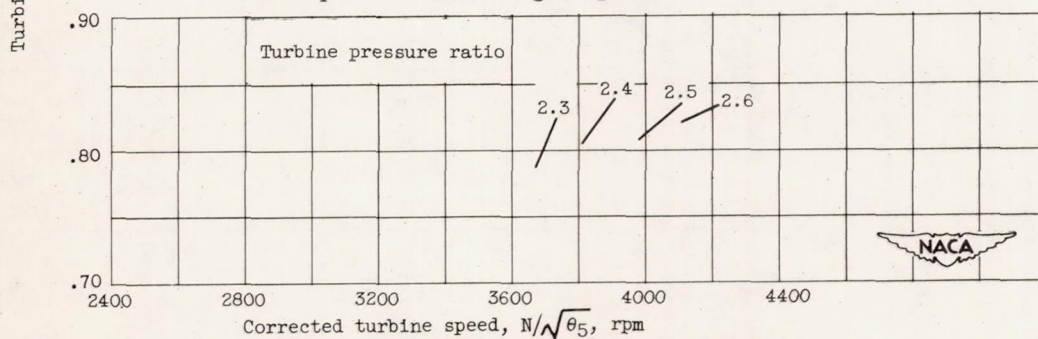
(c) Cross plots showing variation of turbine efficiency with corrected turbine speed at constant values of turbine pressure ratio.
