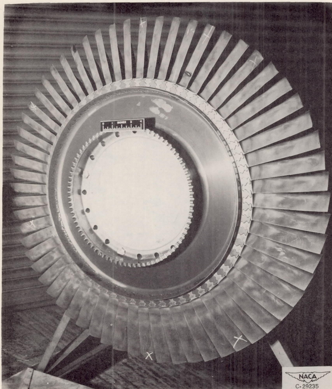
(a) First-stage turbine rotor.
