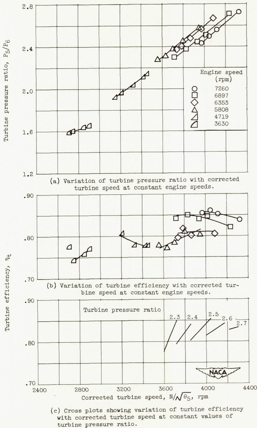
Figure 14. - Effect of various parameters on turbine pressure ratio and turbine efficiency. Altitude, 30,000 feet; flight Mach number, 0.62; turbine nozzle area, 1.37 square feet.
