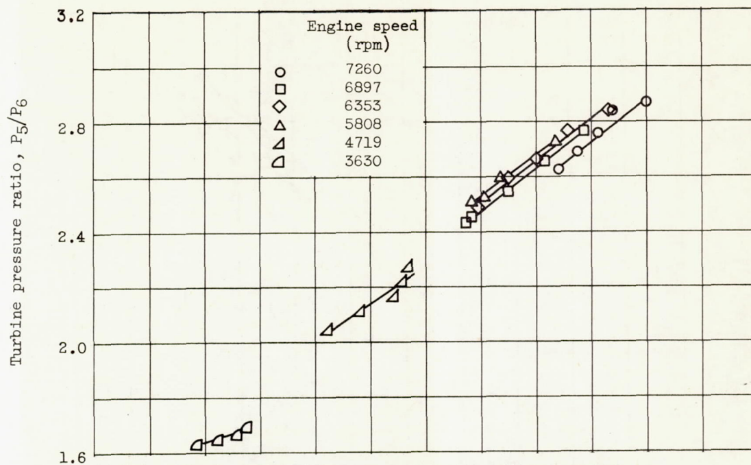
(a) Variation of turbine pressure ratio with corrected turbine speed at constant engine speeds.
