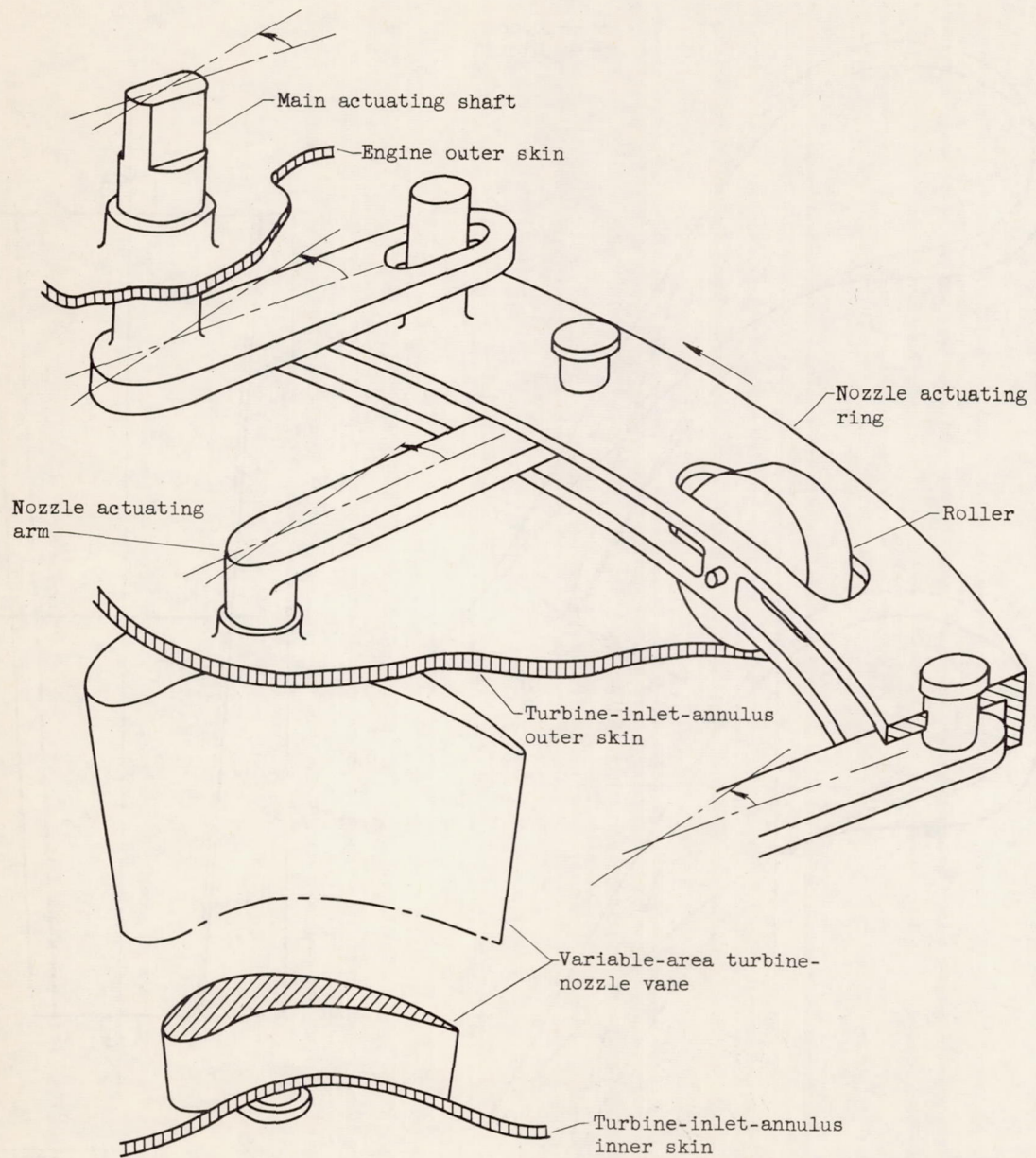
Figure 5. - Schematic sketch of variable-area turbine-nozzle actuating mechanism.
