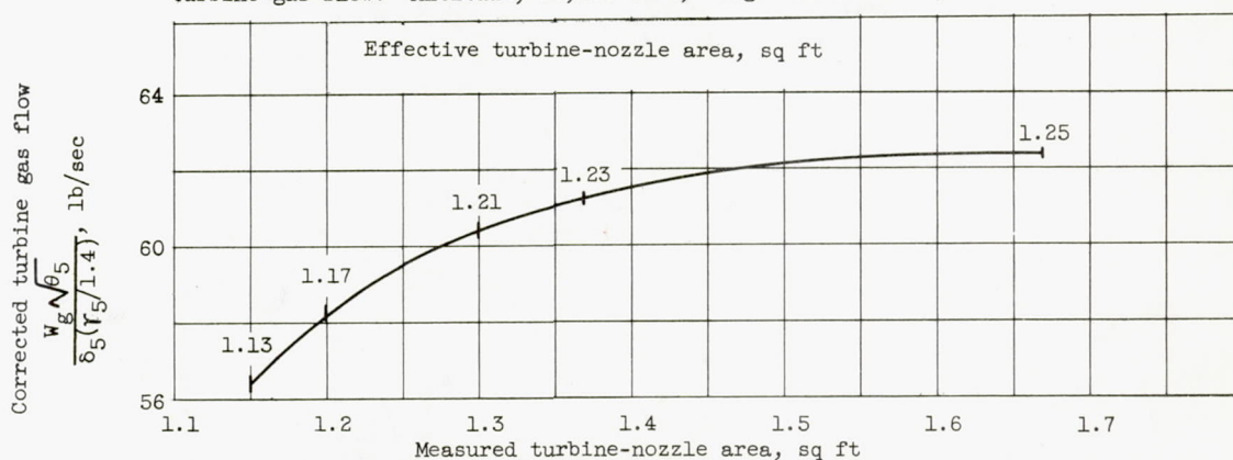
Figure 9. - Variation of maximum corrected turbine gas flow or effective turbine-nozzle area with measured turbine-nozzle area. Altitude 30,000 feet; flight Mach number, 0.62.
