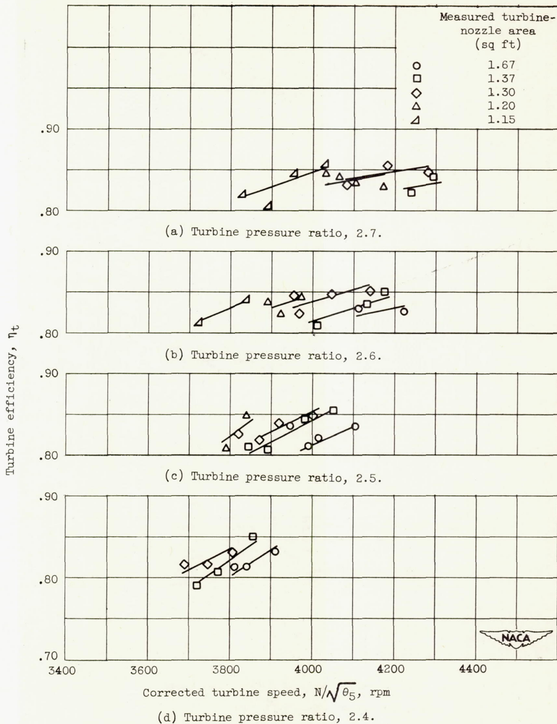
Figure 16. - Effect of turbine-nozzle area and corrected turbine speed on turbine efficiency at constant values of turbine pressure ratio. Altitude, 30,000 feet; flight Mach number, 0.62.
