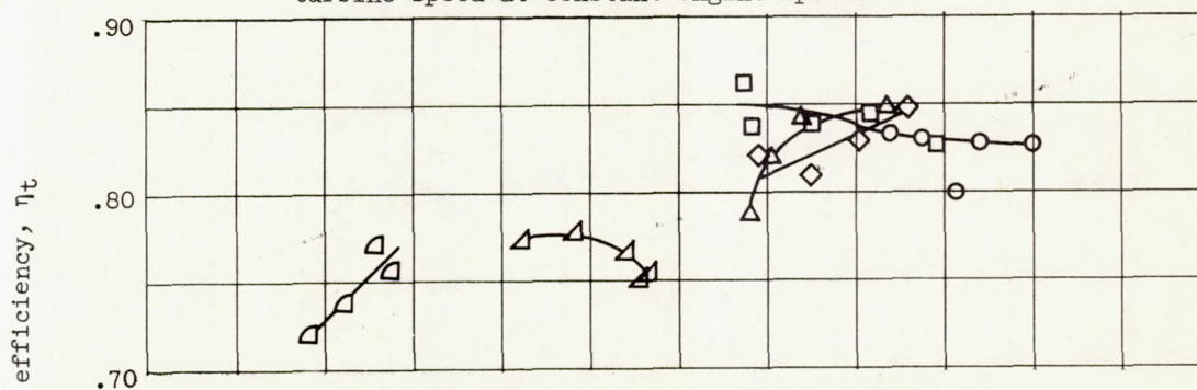
(b) Variation of turbine efficiency with corrected turbine speed at constant engine speeds.
