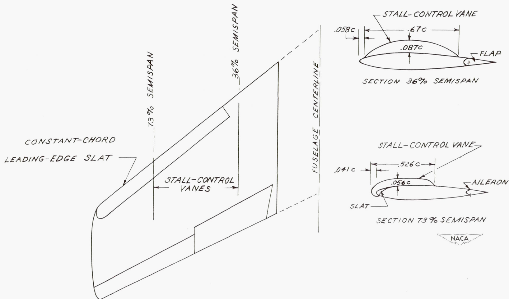
Figure 3.- Plan form and sections of the wing of the Douglas D-558-II airplane showing the location and shape of wing fences (stall-control vanes) used in the investigation.
