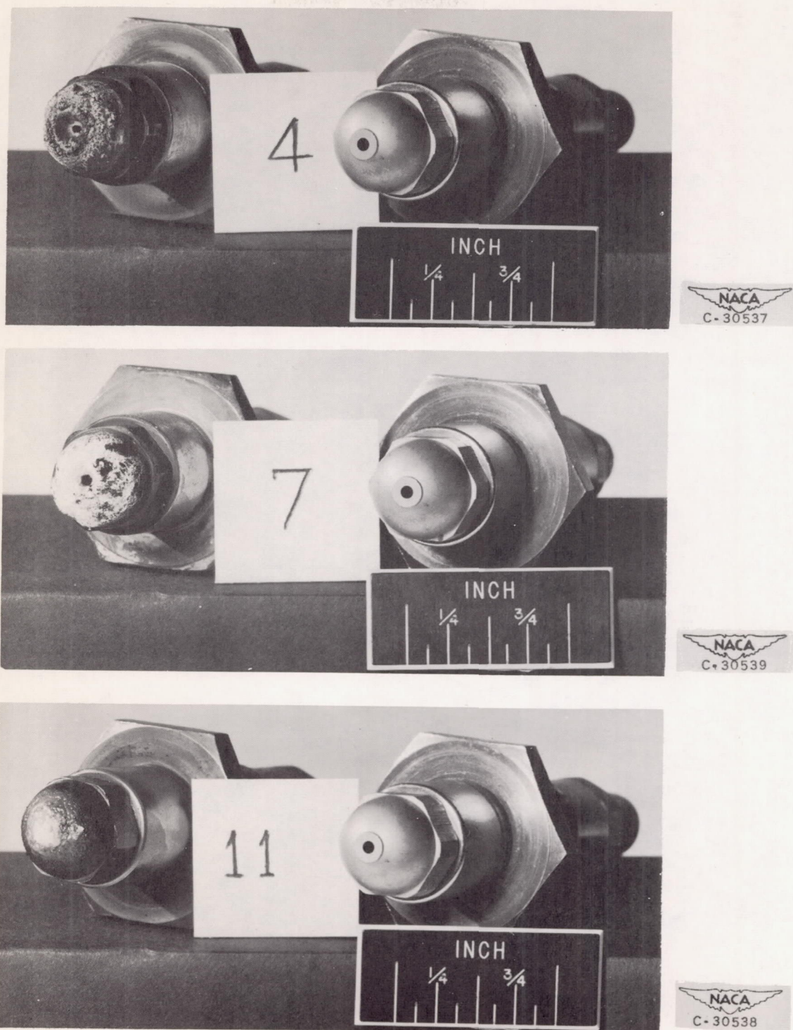
Figure 11. - Fuel nozzles after approximately 1 hour of operation with tributyl borate added to the fuel compared with clean nozzles.
