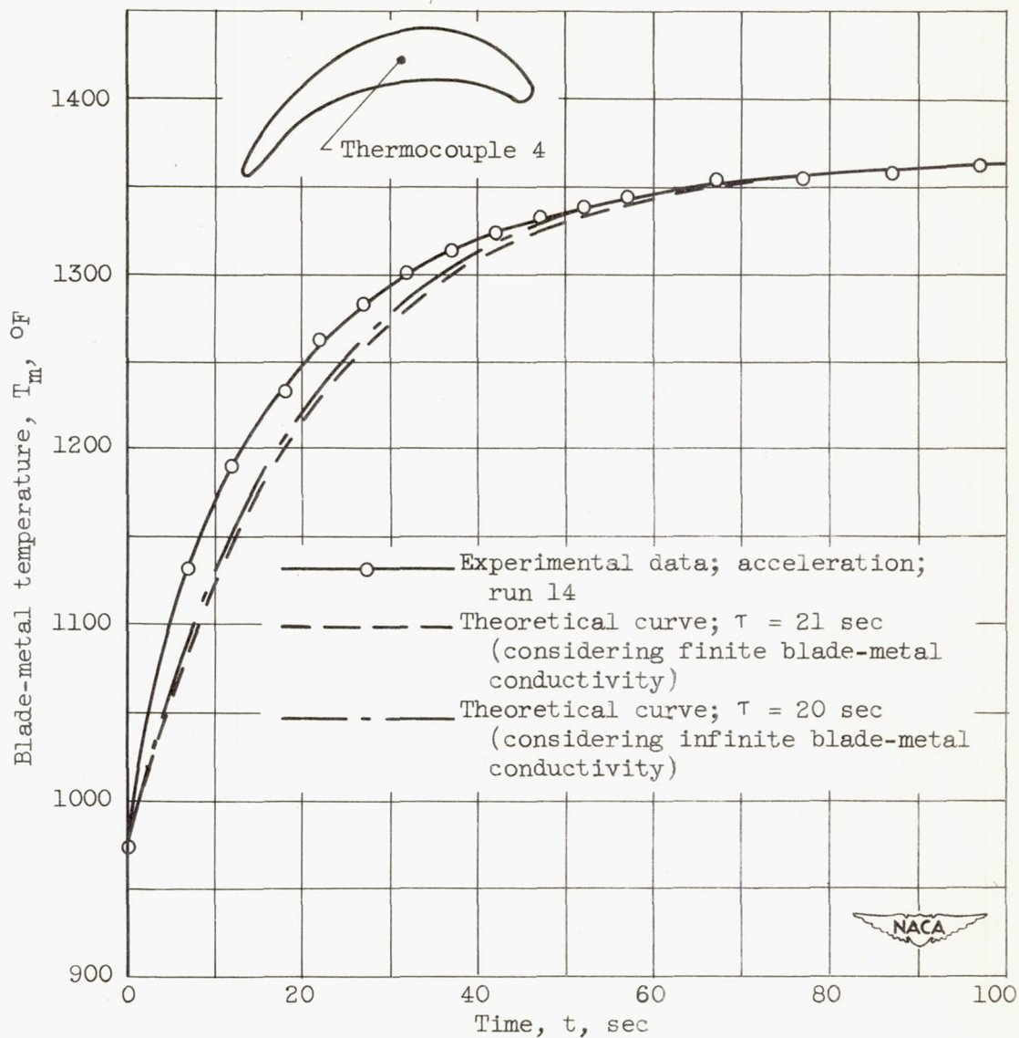
Figure 6. - Comparison of experimental and theoretical time-temperature relations at midchord, midthickness of uncoated rotor blade. Blade-metal initial temperature, 972° F; blade-metal final temperature, 1365° F.
