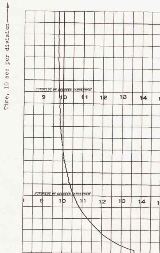
(b) Deceleration; run 9. Thermocouple located at midchord, midthickness of blade.
