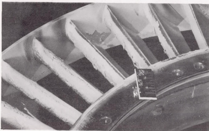
(b) Blades after 2\frac{1}{2} hours of operation.
