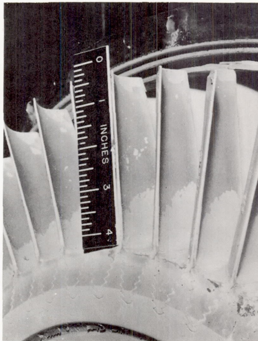
(c) Blades after 2\frac{1}{2} hours of operation.
