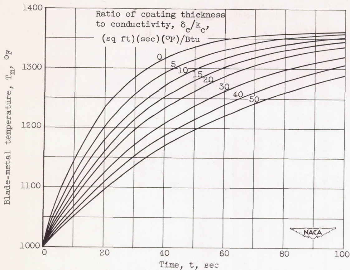
Figure 7. - Theoretical variation of time-temperature relation at blade midchord with ratios of coating thickness to coating conductivity. Blade-metal thermal conductivity considered infinite; blade-metal initial temperature, 1000° F; blade-metal final temperature, 1365° F.
