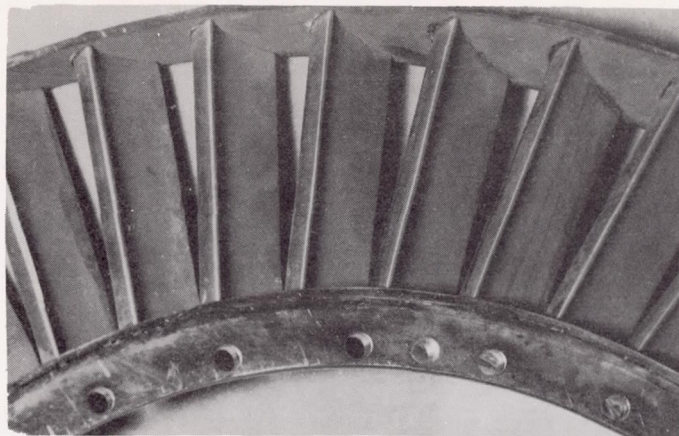
(a) Blades before operation.
