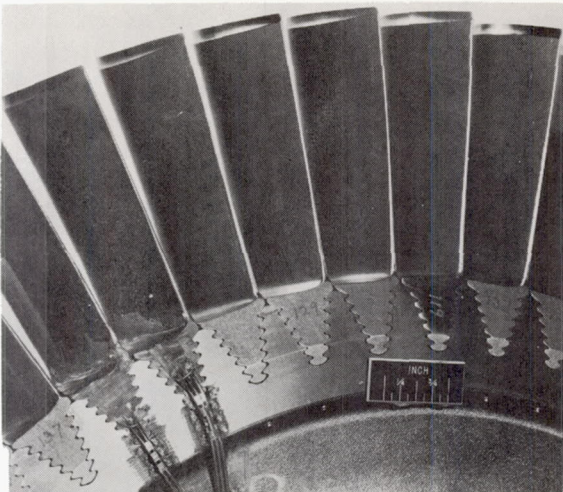
(a) Blades before operation.
