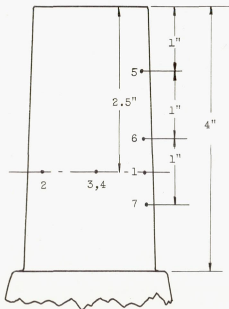
(a) Rotor blade.
