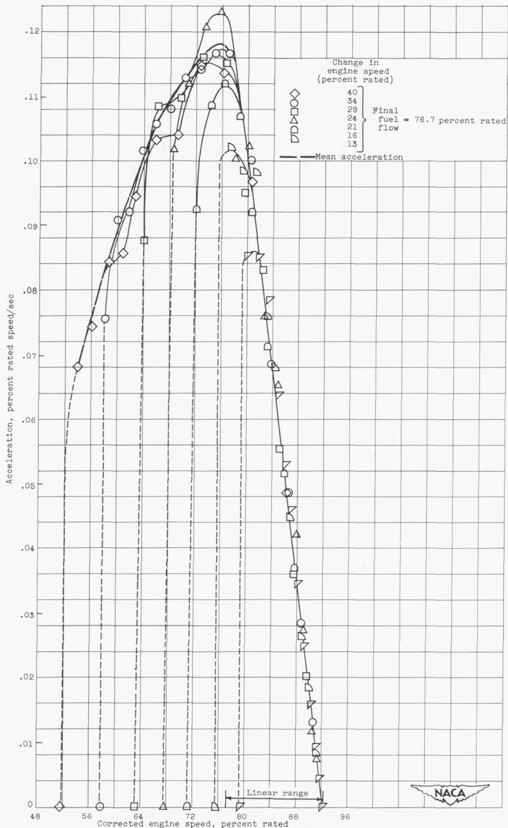
Figure 5. - Variation of acceleration from several initial engine speeds to set final engine speeds from fuel-flow steps. Accelerations to 92 percent rated speed.
