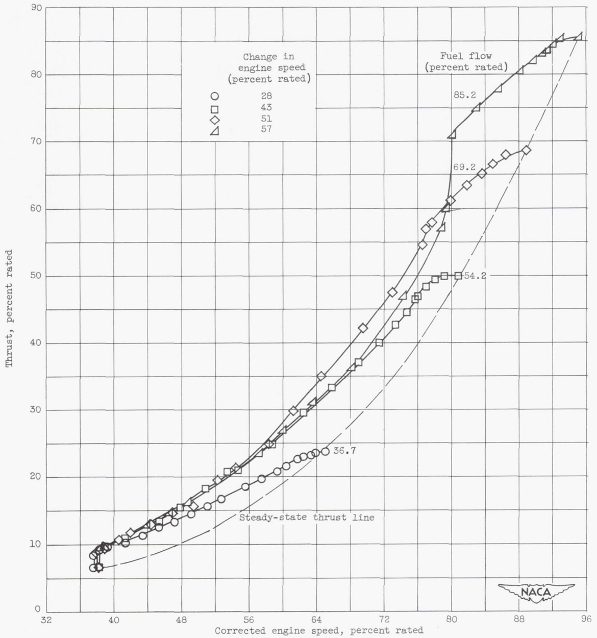
Figure 7. - Variation of thrust with speed for steps in fuel flow initiated at idle speed.
