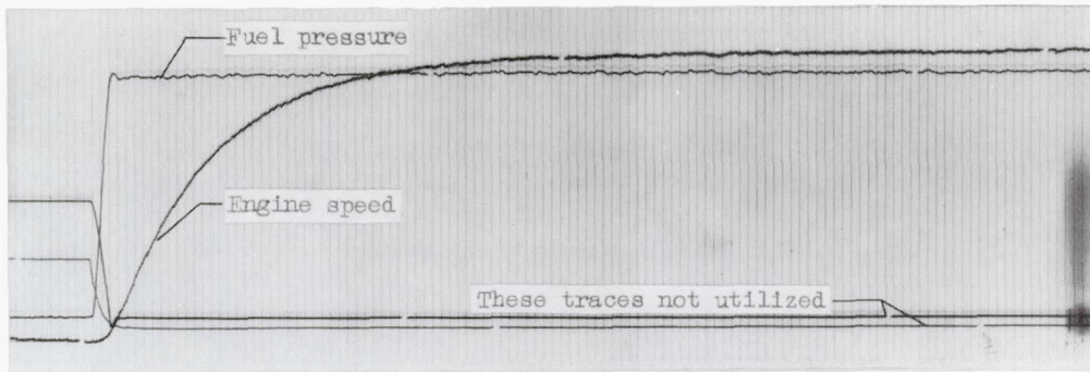
(a) Initial engine speed, 79 percent rated; change in engine speed, 13 percent rated.
