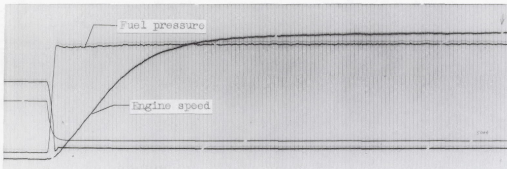
(e) Initial engine speed, 63 percent rated; change in engine speed, 29 percent rated.
