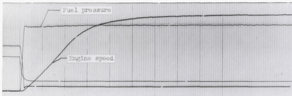
(f) Initial engine speed, 58 percent rated; change in engine speed, 34 percent rated.
