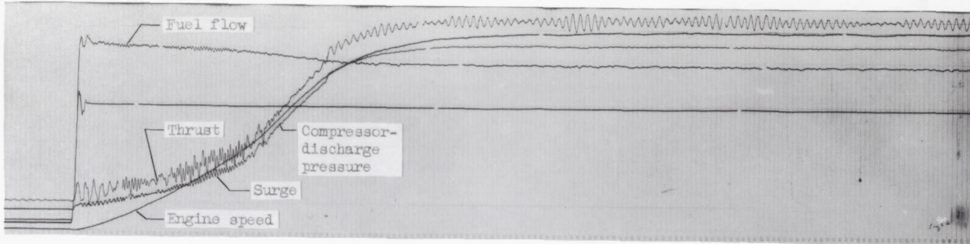
(d) Final engine speed, 89 percent rated; change in engine speed, 51 percent rated.
