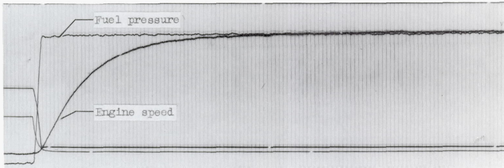
(b) Initial engine speed, 76 percent rated; change in engine speed, 16 percent rated.
