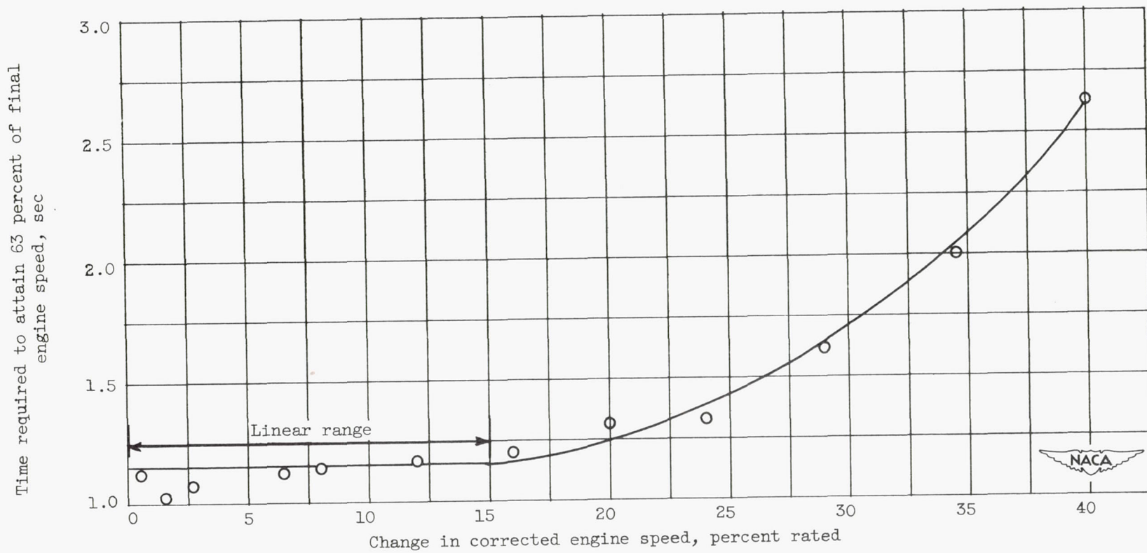
Figure 4. - Variation of response time with size of speed change for transients ending at 92 percent rated speed.
