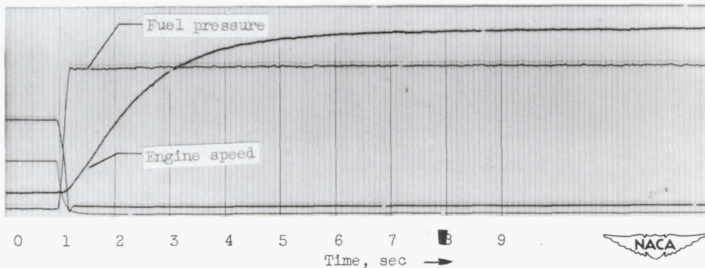
(d) Initial engine speed, 68 percent rated; change in engine speed, 24 percent rated.
