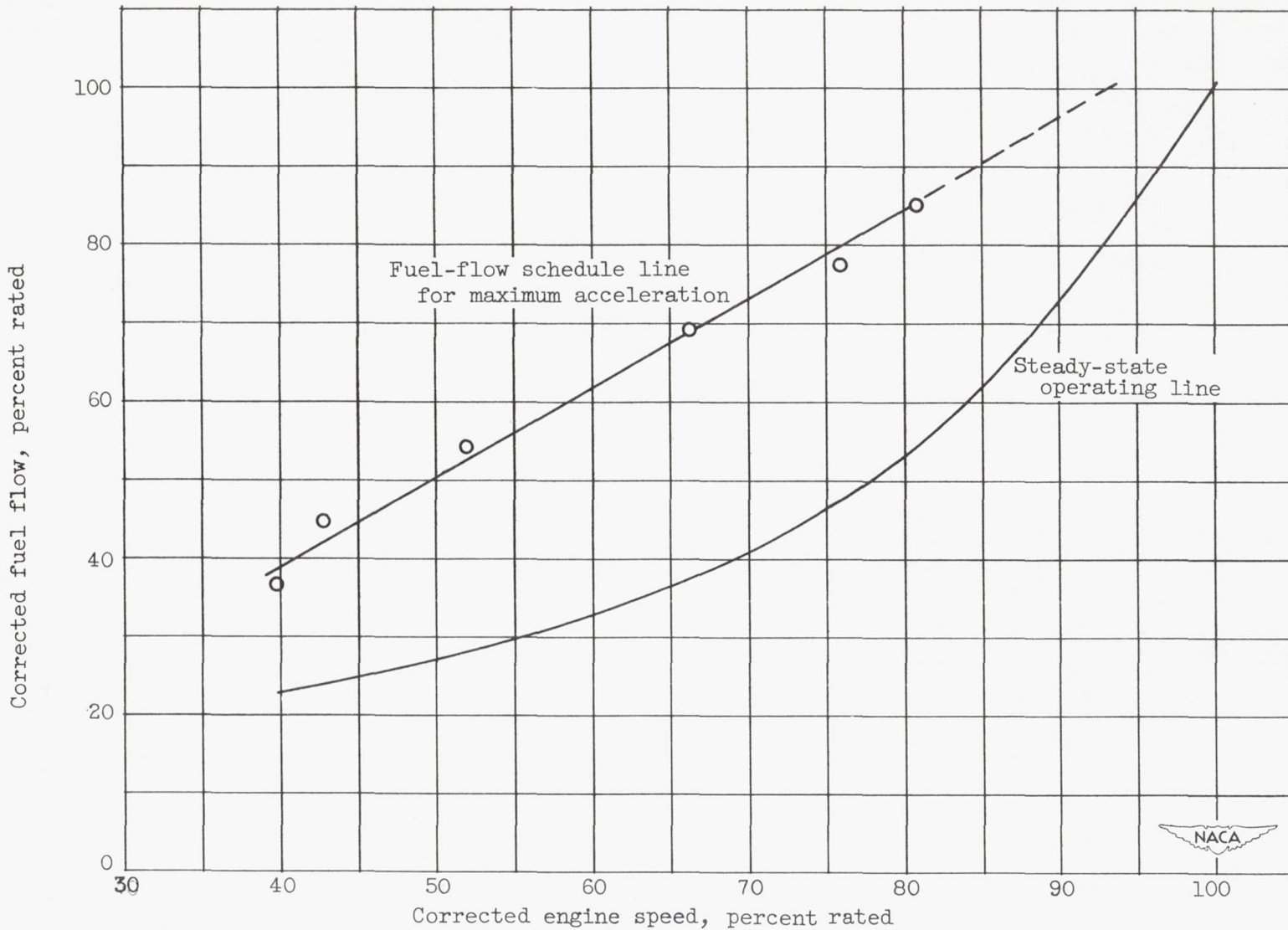
Figure 9. - Fuel-flow schedule for maximum acceleration.
