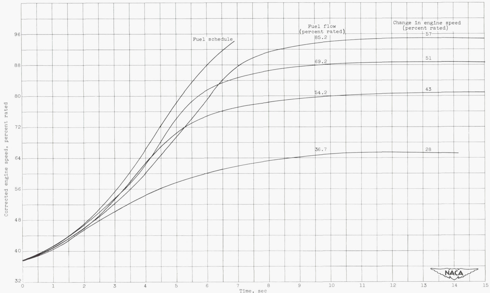
Figure 10. - Variation of engine speed with time for fuel-flow steps and scheduled fuel flow.
