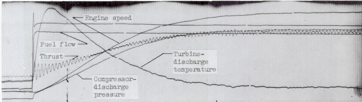
(a) Final engine speed, 66 percent rated; change in engine speed, 28 percent rated.
