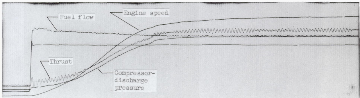
(b) Final engine speed, 74 percent rated; change in engine speed, 36 percent rated.
