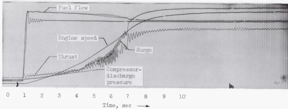
(e) Final engine speed, 95 percent rated; change in engine speed, 57 percent rated.
