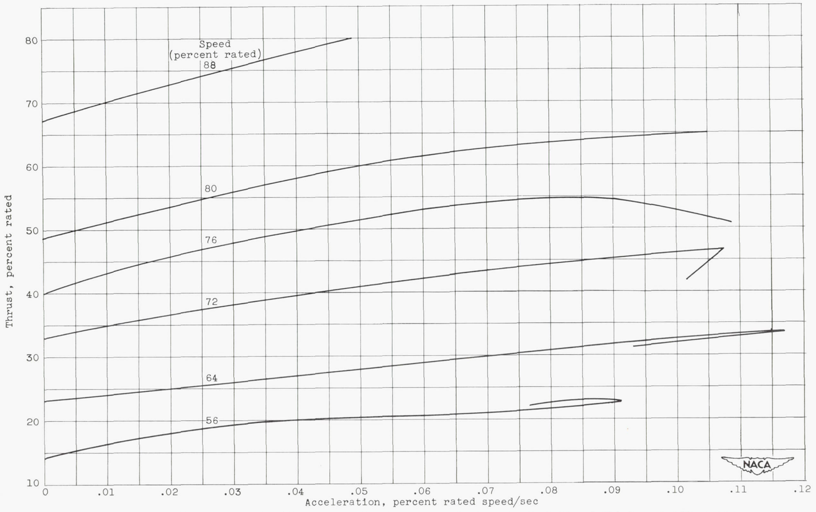
Figure 8. - Variation of thrust with acceleration from several steps in fuel flow initiated at idle speed (cross plot of figs. 7 and 8).
