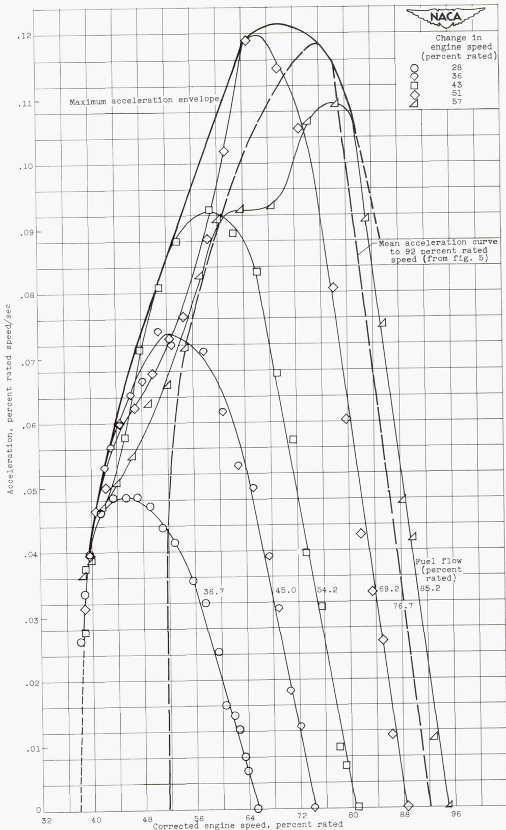
Figure 6. - Variation of acceleration from idle speed to several final speeds from fuel-flow steps.
