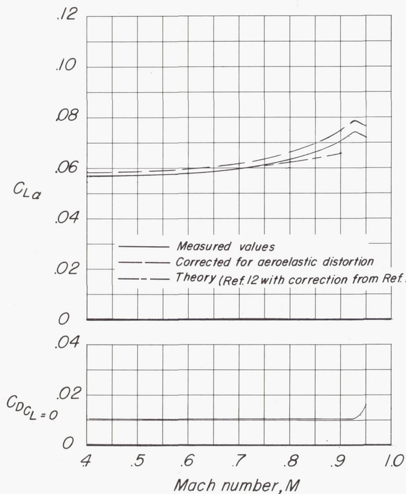
Figure 10.- Summary of the effect of Mach number on the aerodynamic characteristics of the 45-4-0.6-006 wing-fuselage combination.
