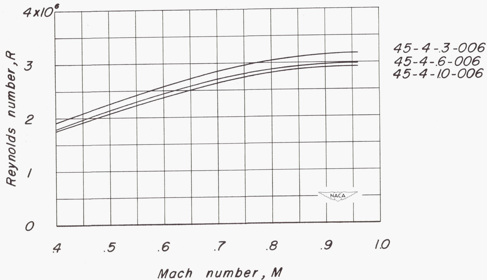
Figure 6.- Variation with Mach number of mean Reynolds number based on the mean aerodynamic chords.
