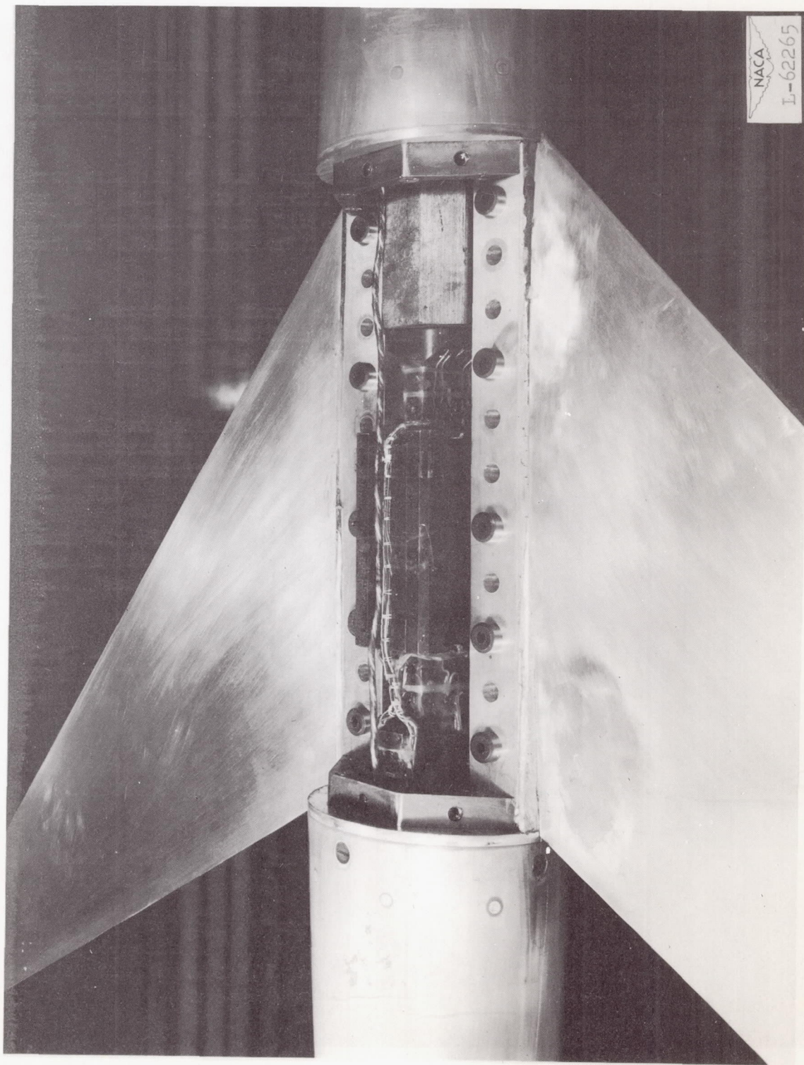
Figure 3.- Model showing installation of the strain-gage balance.
