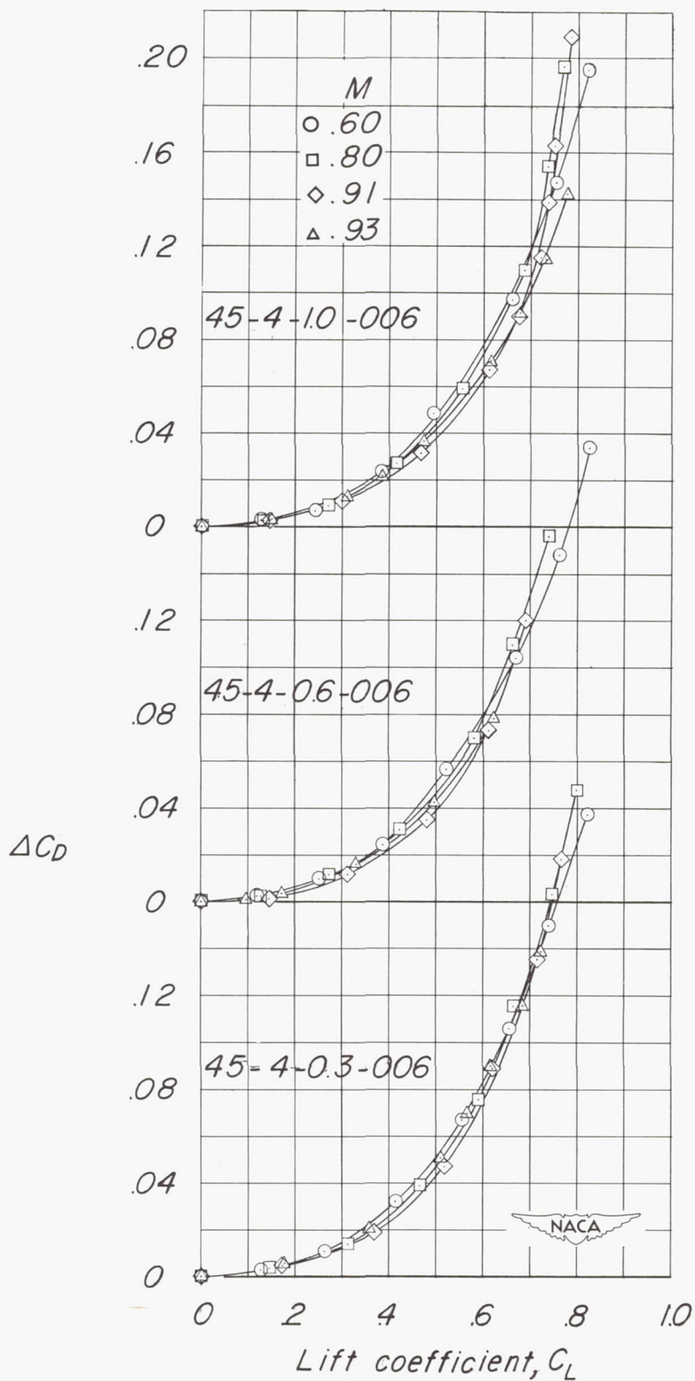
Figure 19.- Comparison of the effects of Mach number on the drag due to lift for the three wing-fuselage combinations.
