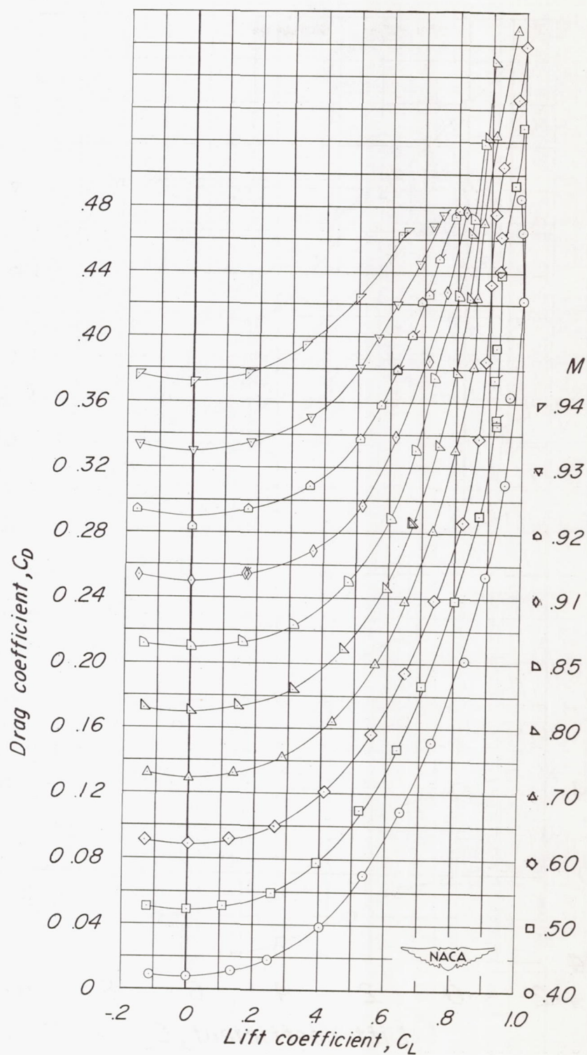
(c) Drag (45-4-0.3-006).
