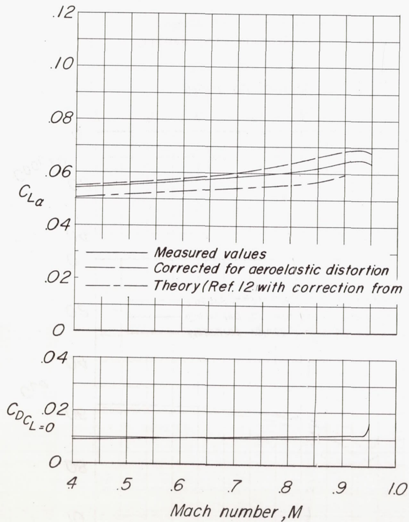
Figure 11.- Summary of the effect of Mach number on the aerodynamic characteristics of the 45-4-1.0-006 wing-fuselage combination.
