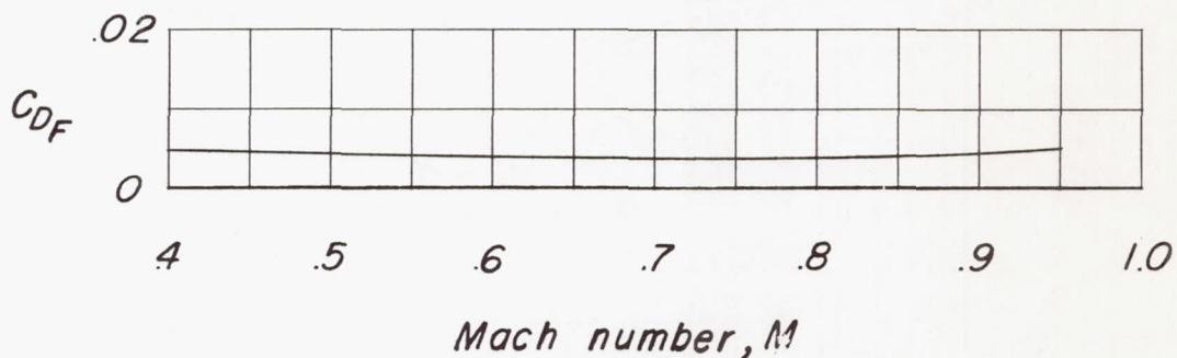
Figure 15.- Drag of the fuselage alone at zero angle of attack, based on the wing area. (Ref. 5.)
