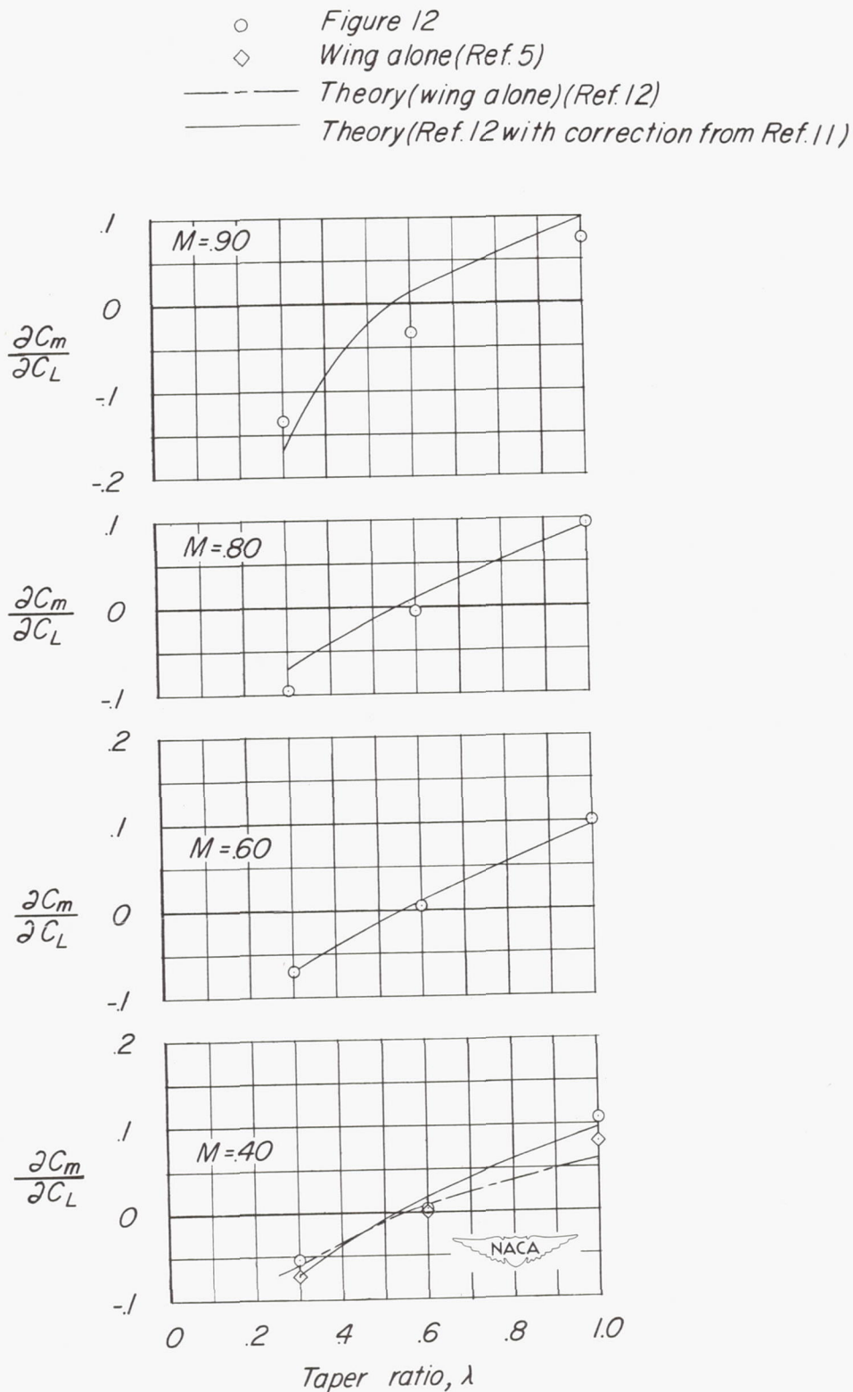
Figure 14.- Effect of taper ratio on the aerodynamic-center location at four Mach numbers. (Corrected for aeroelastic distortion.)
