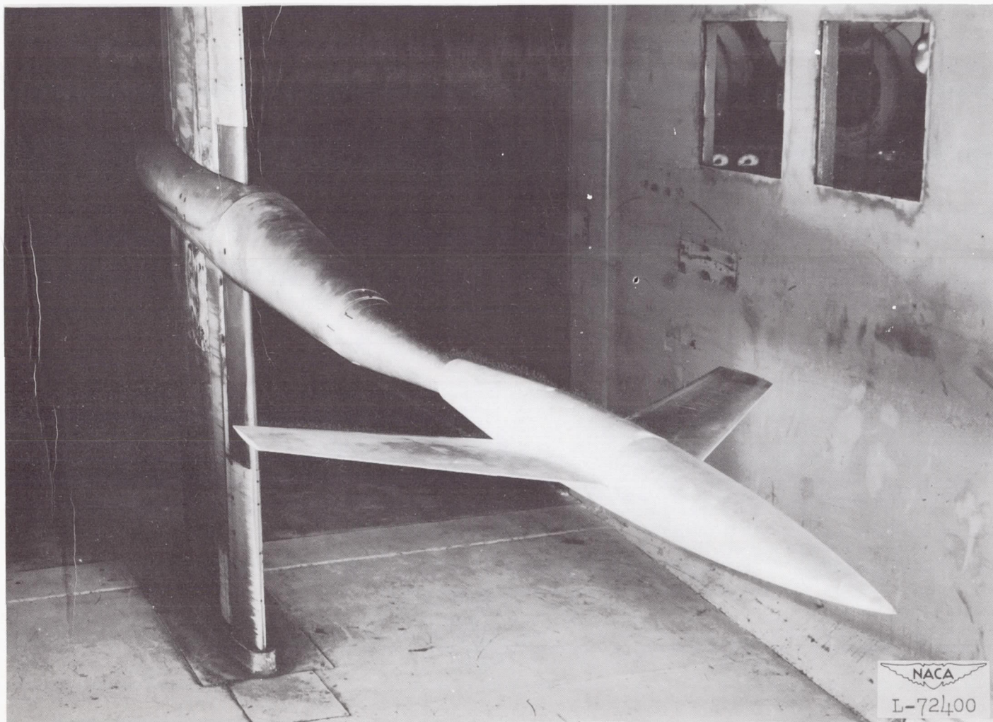
Figure 2.- Model installed on the variable-angle sting support used in the Langley high-speed 7- by 10-foot tunnel.
