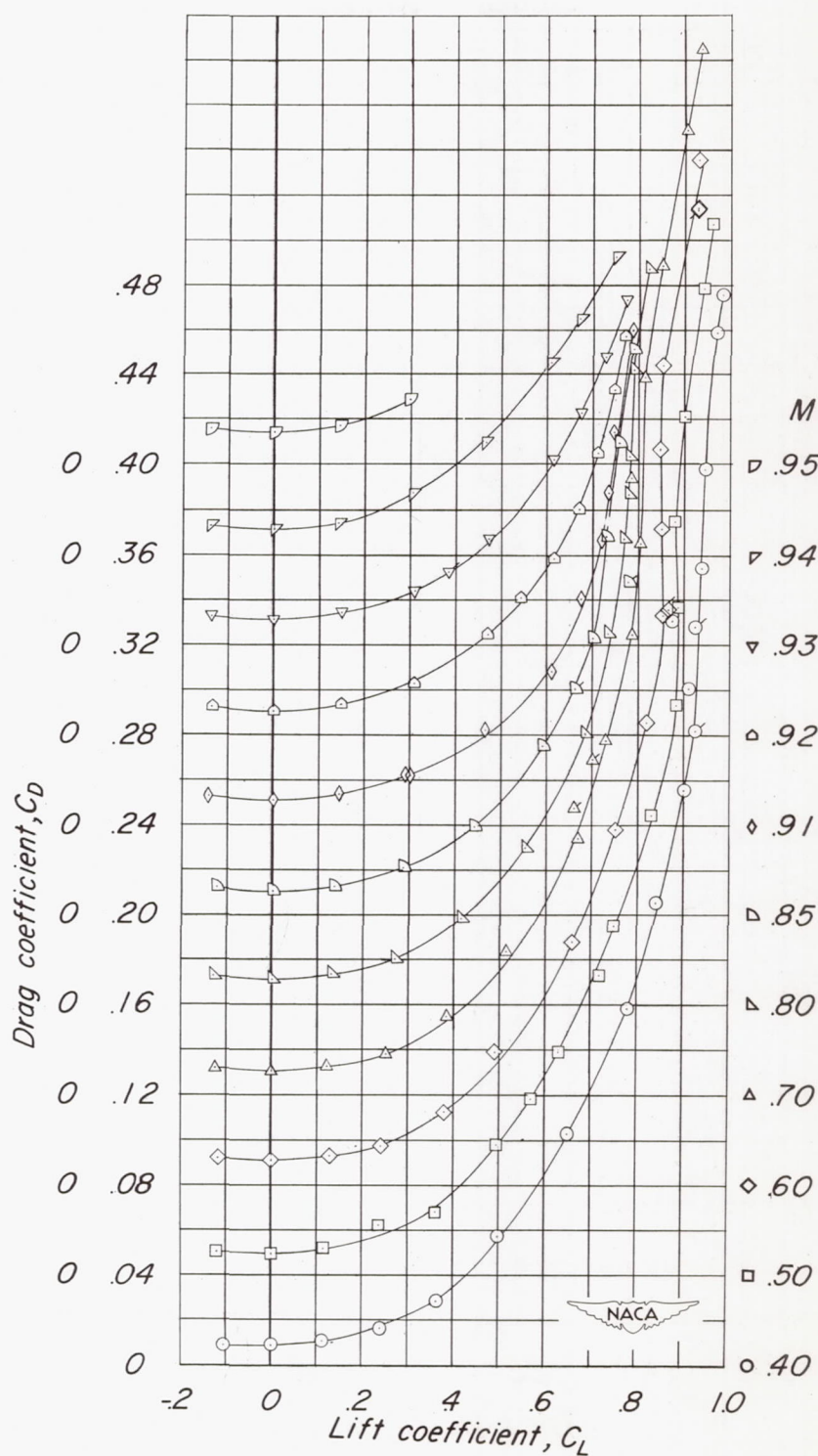
(c) Drag (45-4-1.0-006).
