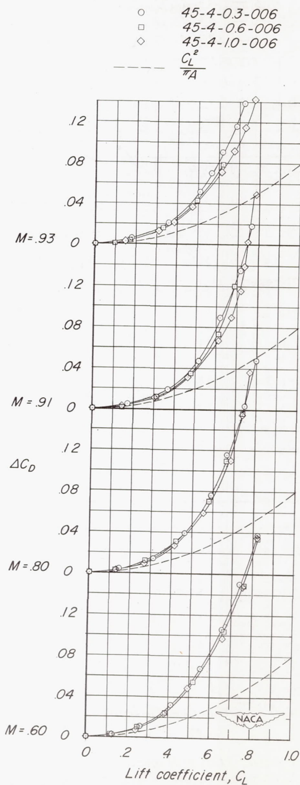
Figure 18.- Comparison of the effects of taper ratio on the drag due to lift at four Mach numbers.
