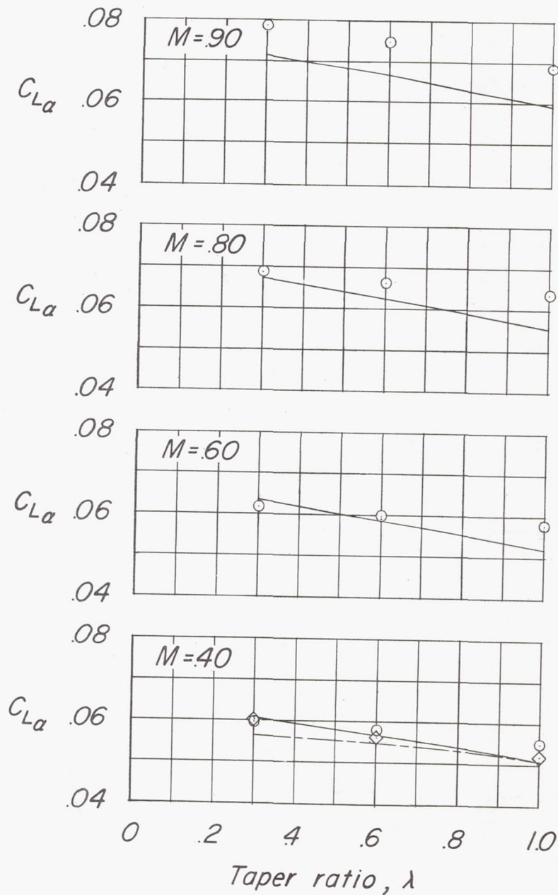
Figure 13.- Effect of taper ratio on the lift-curve slope at four Mach numbers. (Corrected for aeroelastic distortion.)
