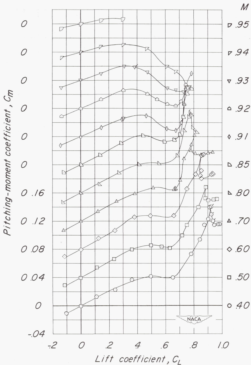
(b) Pitching moment (45-4-1.0-006).
