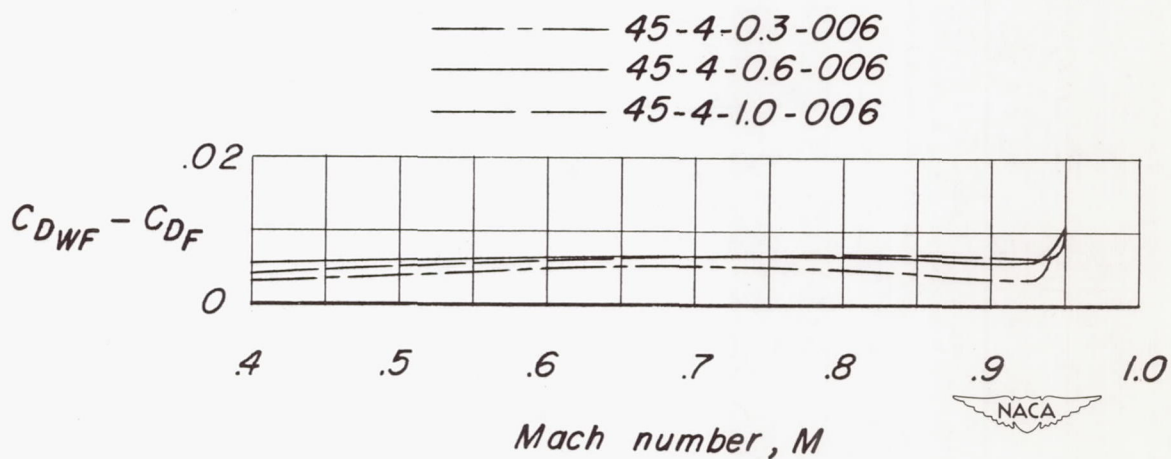
Figure 16.- Variation with Mach number of the wing plus wing-fuselage interference drag at zero lift for the three wings tested.
