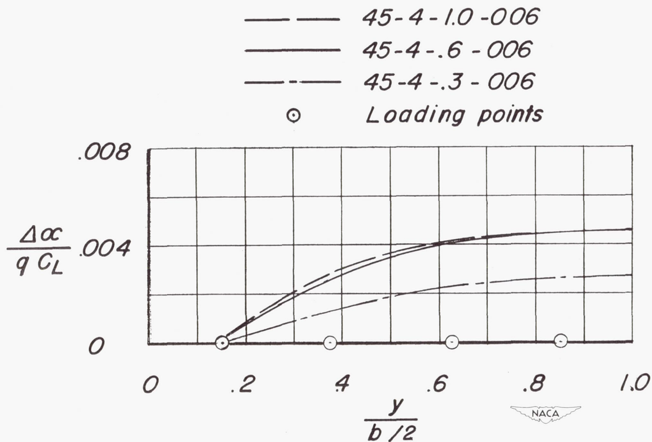
Figure 4.- Spanwise variation of angle of attack due to aeroelastic distortion.
