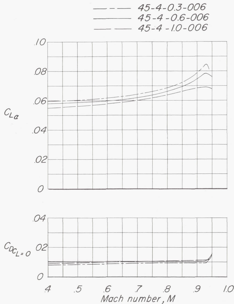
Figure 12.- Comparison of the effects of Mach number on the aerodynamic characteristics of the three wing-fuselage combinations. ( C_{L\alpha} and \partial C_m / \partial C_L corrected for aeroelastic distortion.)
