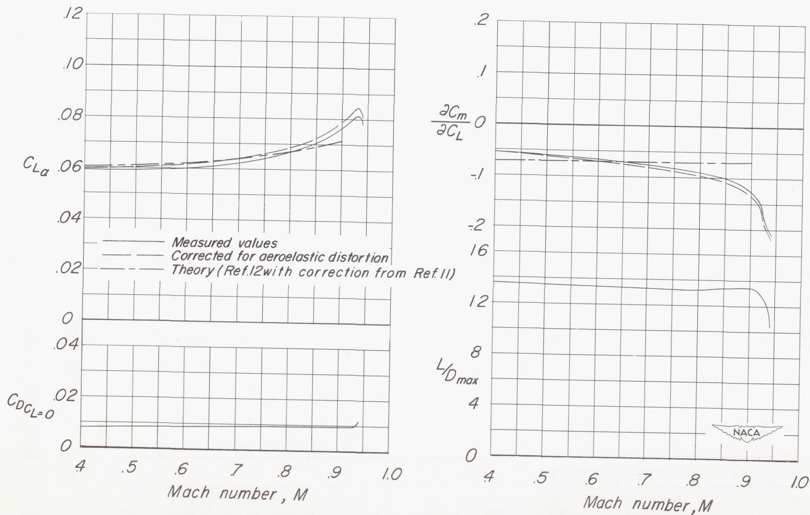
Figure 9.- Summary of the effect of Mach number on the aerodynamic characteristics of the 45-4-0.3-006 wing-fuselage combination.
