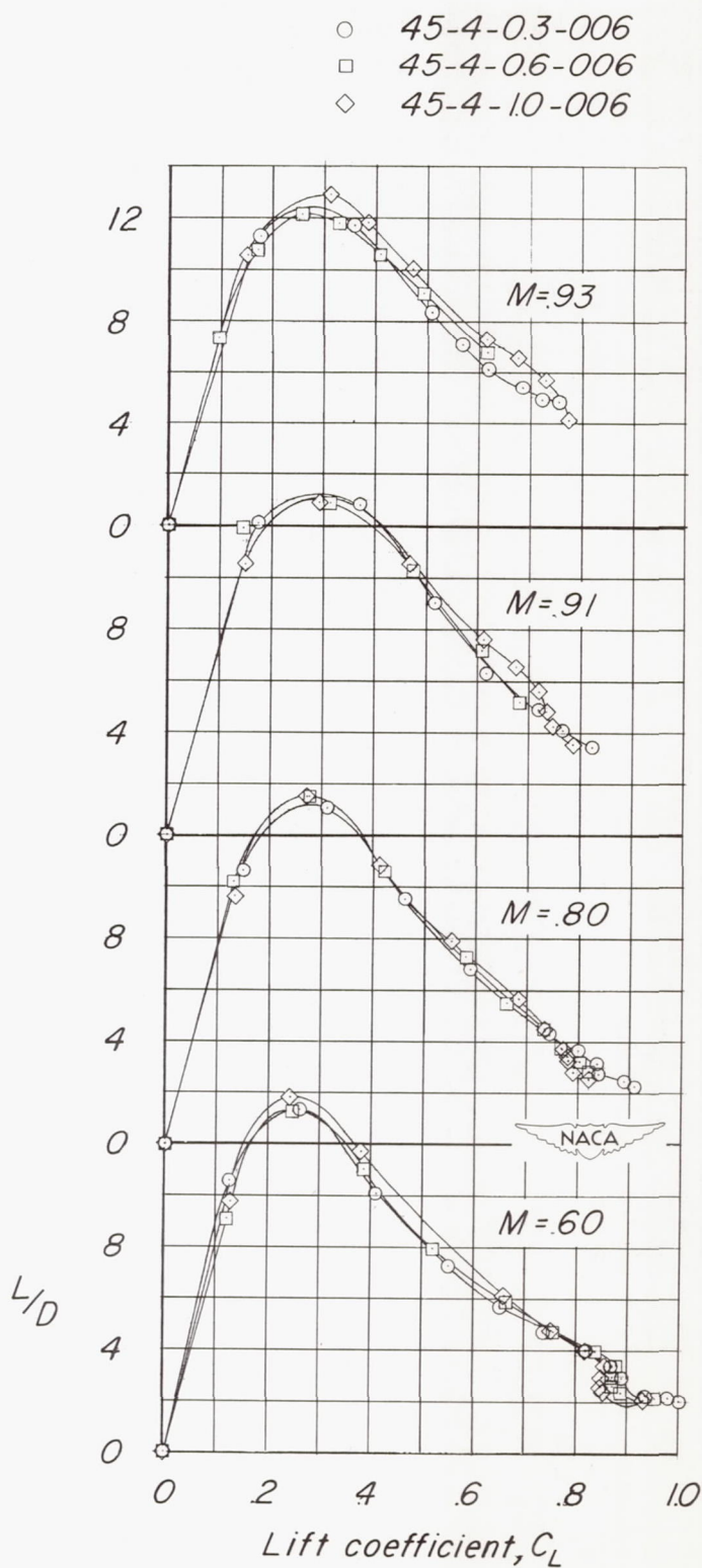
Figure 20.- Comparison of the lift-drag ratios of the three wing-fuselage combinations at four Mach numbers.
