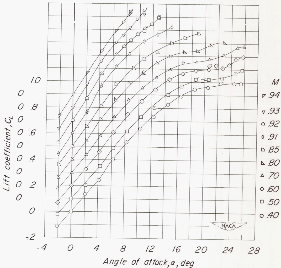
(a) Lift (45-4-0.3-006).
