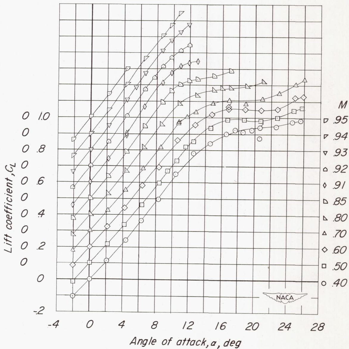
(a) Lift (45-4-1.0-006).
