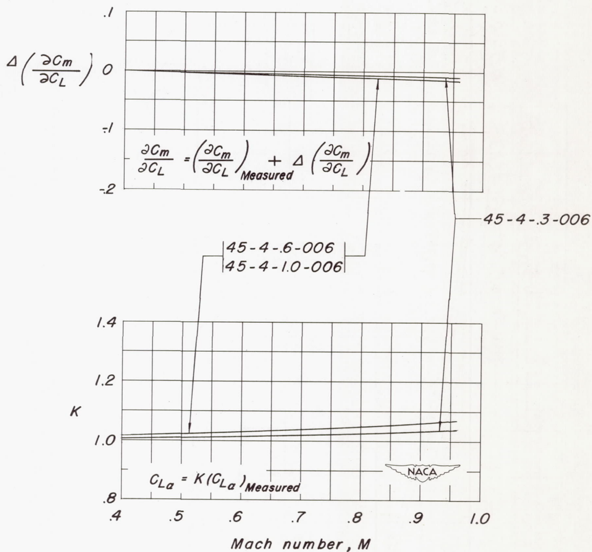
Figure 5.- Correction factors used to correct the summary data for the effects of aeroelastic distortion.
