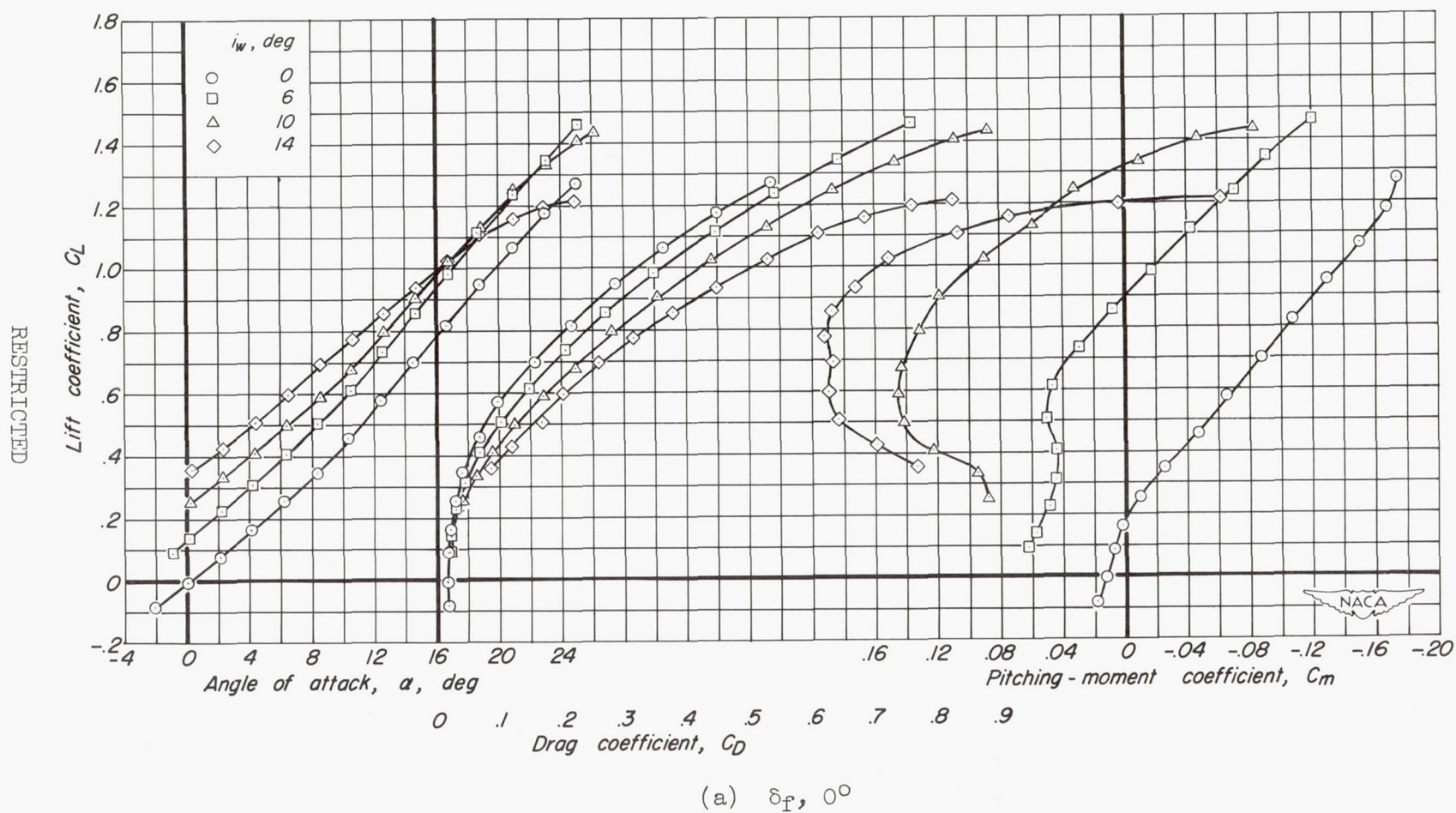
Figure 7.- Longitudinal characteristics of the model with the wing at four incidences and the tail in the low position; i_t, 0^\circ ; z/(b/2), 0 ; moment center, 0.4185.
