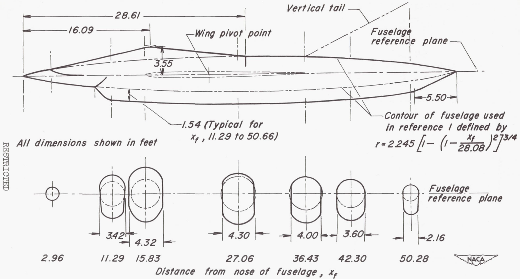
Figure 5.- Geometric details of the fuselage.
