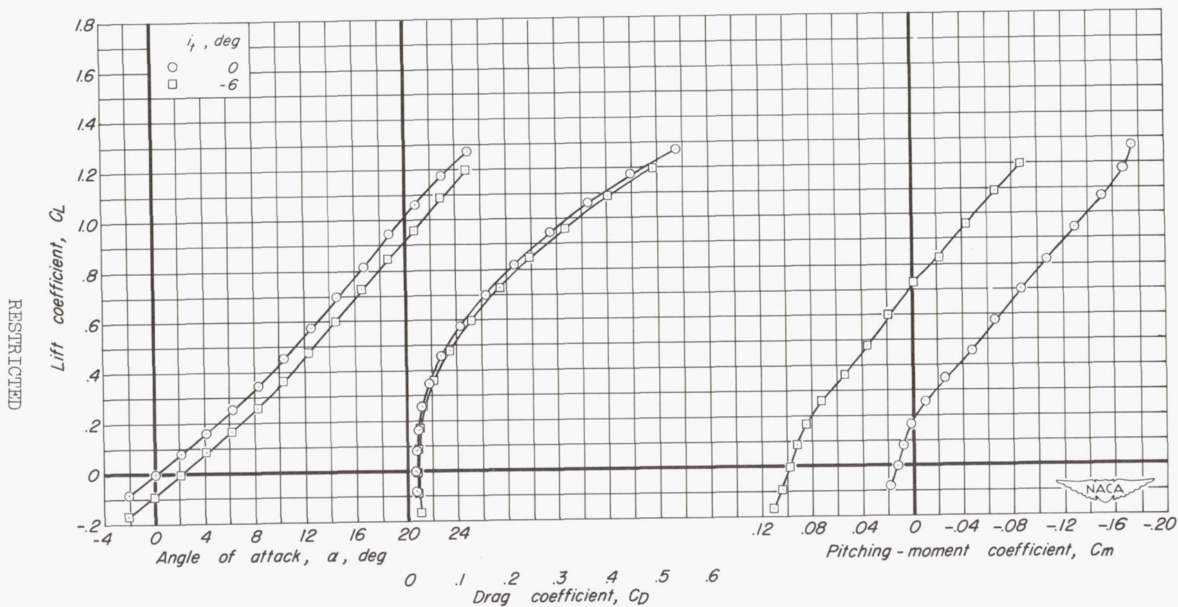
Figure 10.- The effect of tail incidence on the longitudinal characteristics of the model with the tail in the low position; z/(b/2), 0 ; moment center, 0.418\bar{c} .
