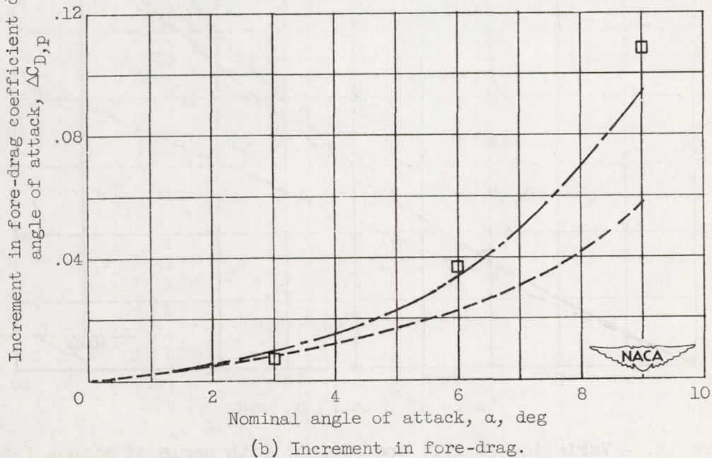
Figure 10. - Increment in drag coefficient due to angle of attack for Reynolds number of 14 \times 10^6 .
