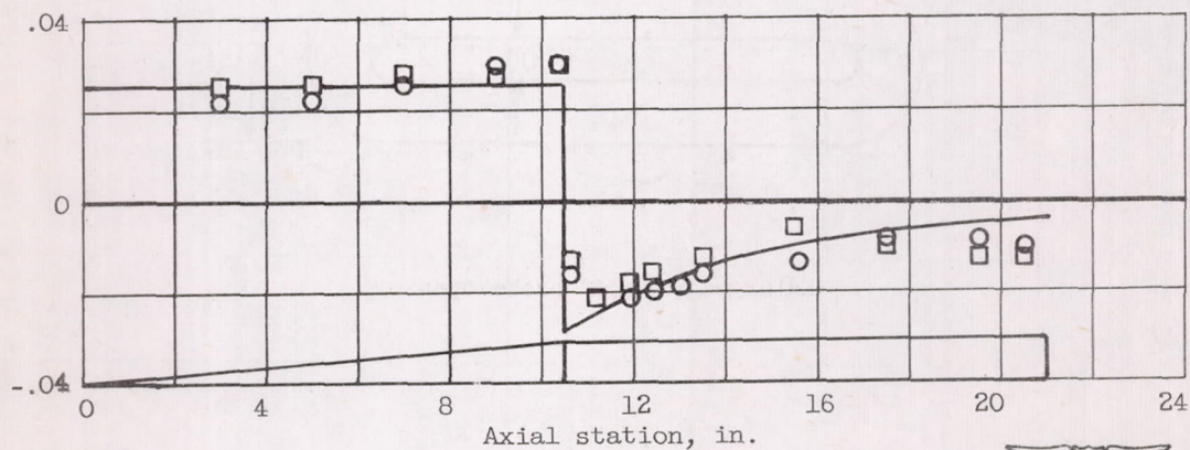
Figure 3. - Experimental and theoretical axial variation of pressure coefficient for model at zero angle of attack.
