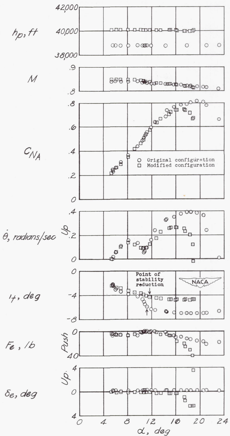
Figure 7.- Stabilizer pull-ups to the stall for the two fillet configurations at a Mach number of approximately 0.84.
