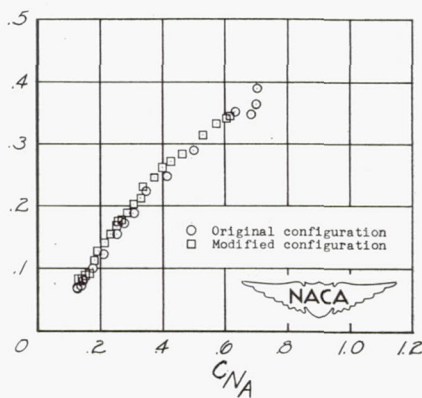
(c) M = 0.97 .
