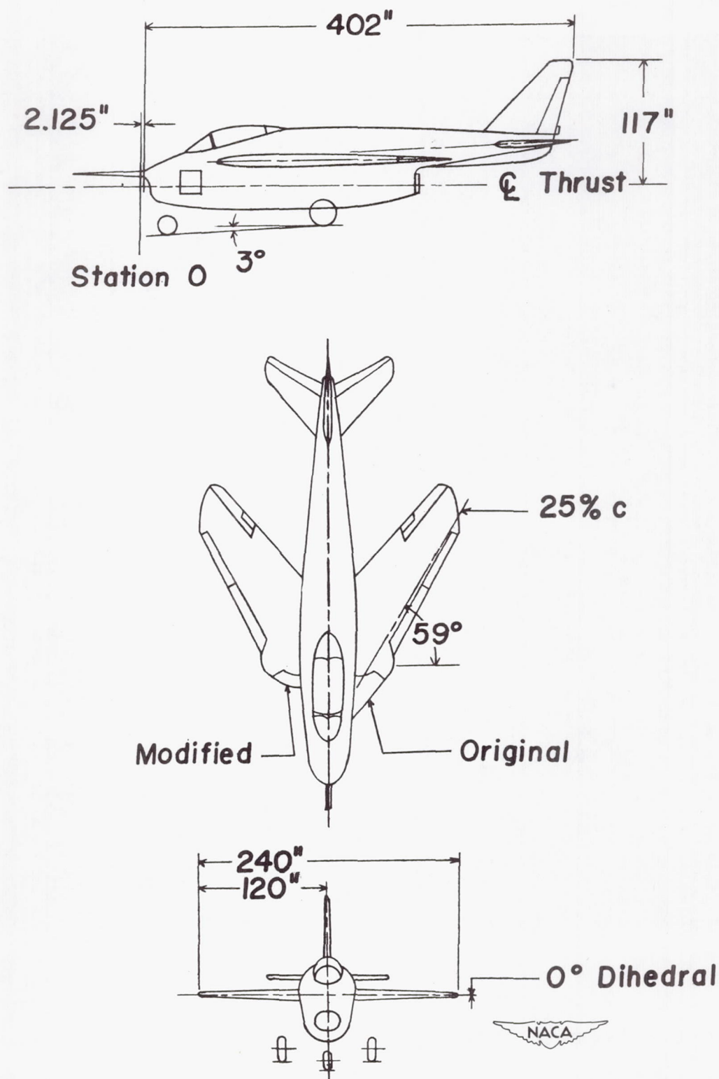
Figure 1.- Three-view drawing of original and modified configurations at 59° sweepback. (Right wing modified, left wing original.)
