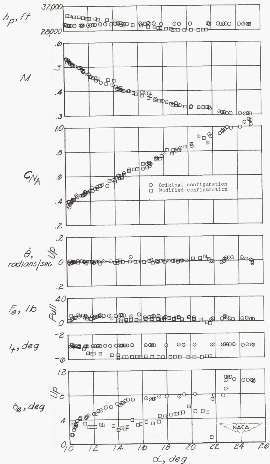
Figure 6.- Approach to an unaccelerated clean stall for the two fillet configurations.
