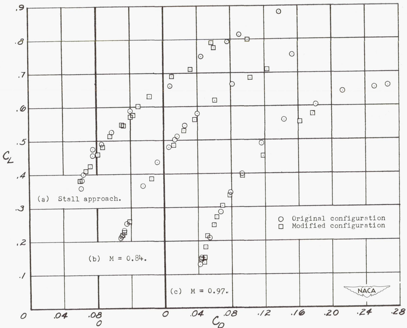
Figure 12.- Airplane polars for the two fillet configurations at the test Mach numbers.
