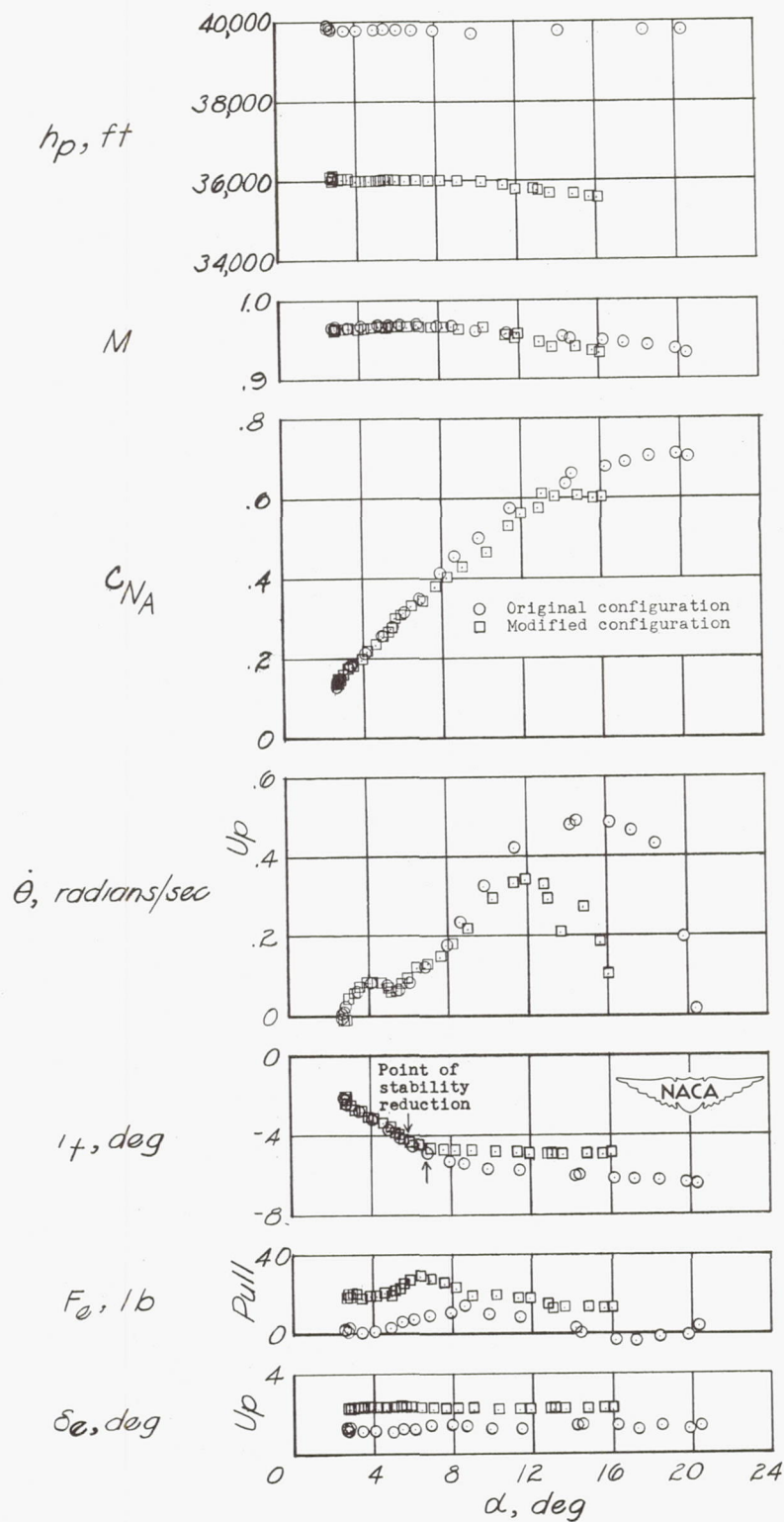
Figure 8.- Stabilizer pull-ups to the stall for the two fillet configurations at a Mach number of approximately 0.97.
