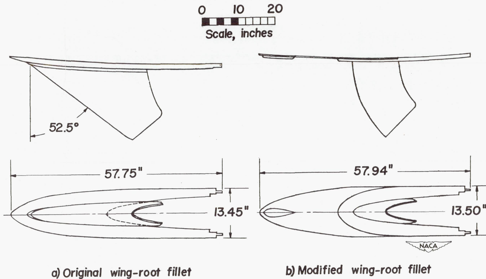
Figure 4.- Two-view drawing of original and modified wing-root fillets.
