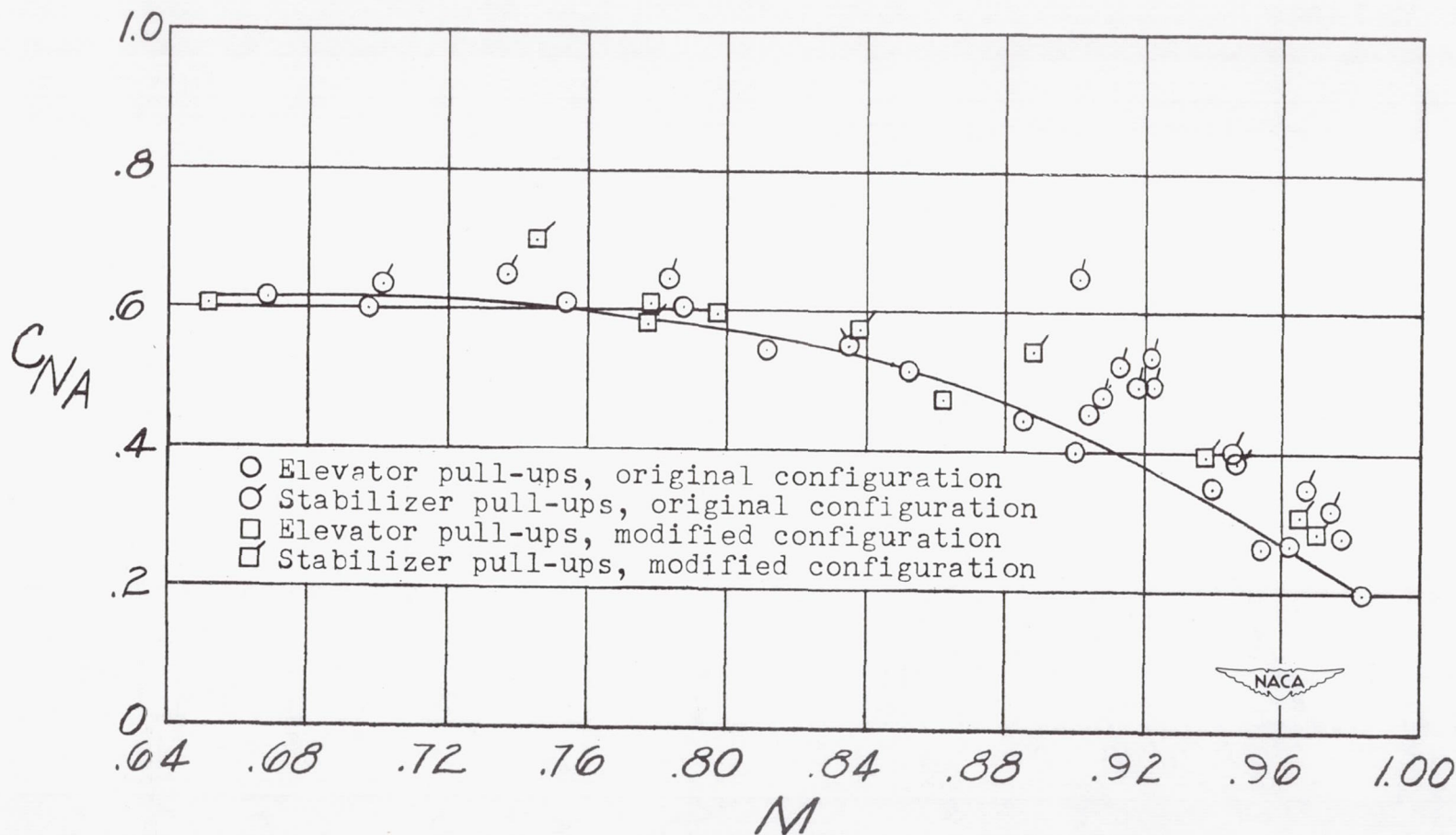
Figure 5.- Boundary for the reduction of longitudinal stability of the Bell X-5 research airplane at 59° sweepback, showing points for original and modified fillet configurations.
