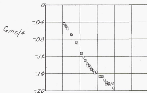
(b) M = 0.84 .
