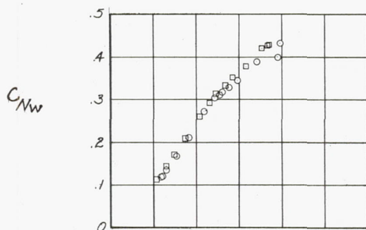
(b) M = 0.84 .
