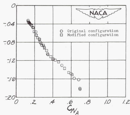
(c) M = 0.97 .
