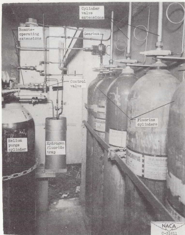
(a) Gaseous-fluorine supply cylinder manifold.
