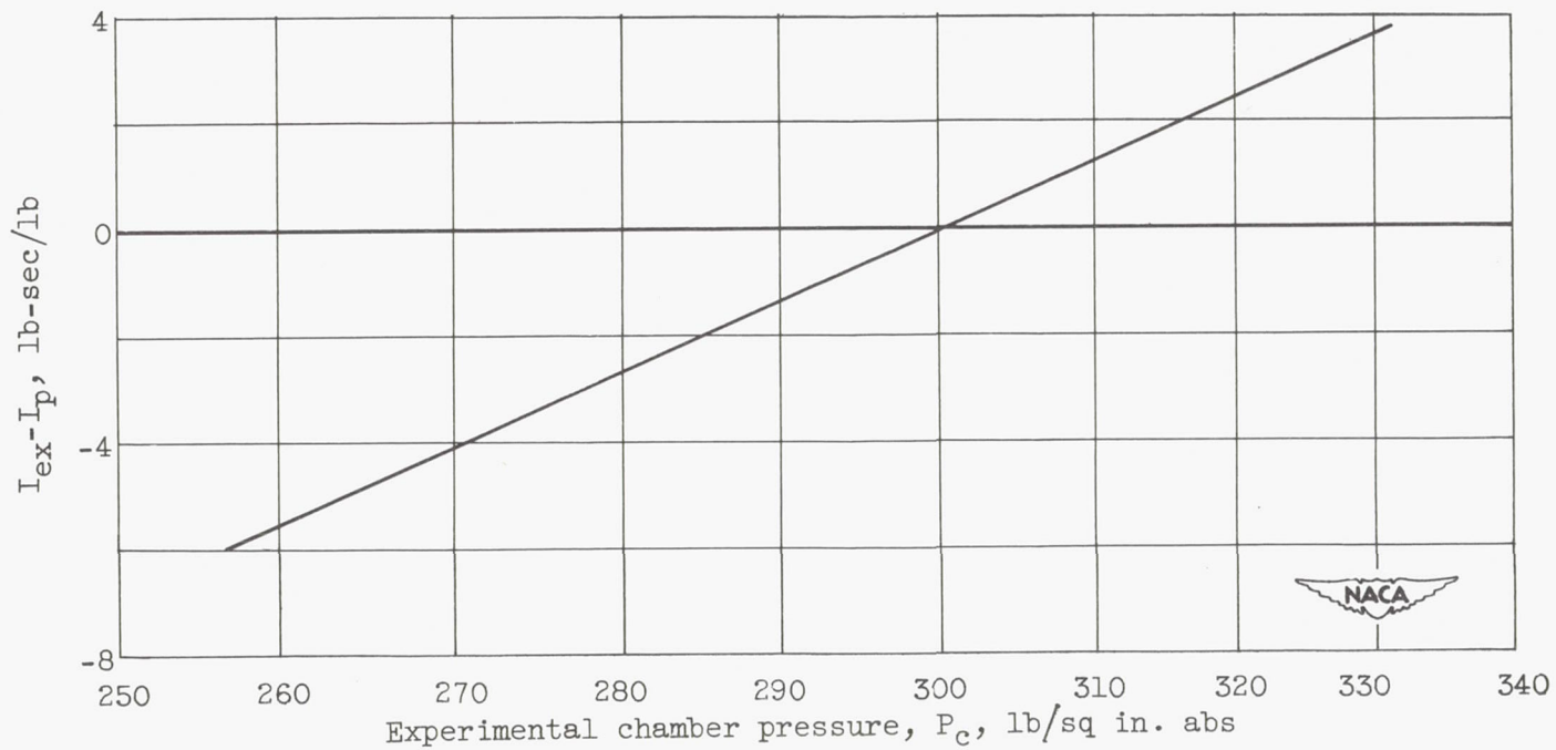
Figure 6. - Theoretical variation of specific impulse with chamber pressure from base of 300 pounds per square inch absolute for liquid fluorine - liquid ammonia propellant combination for ideal nozzle. I_{ex} - I_p = 88.65 \log(P_c/300) .
