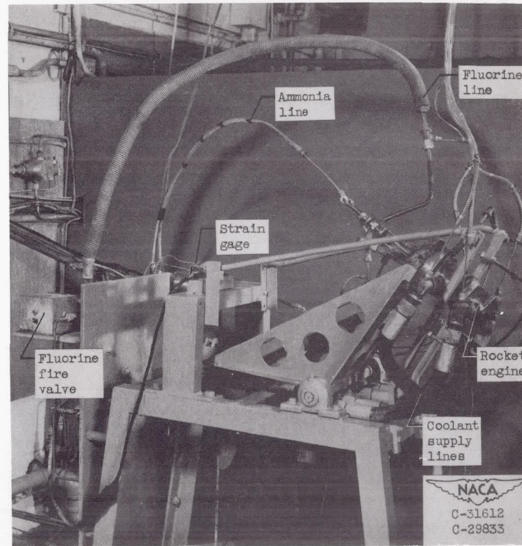
(d) Thrust stand with mounted rocket engine.
