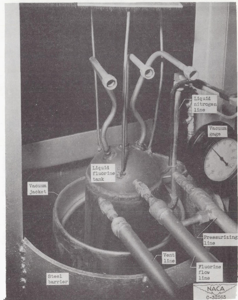
(b) Liquid-fluorine supply tank.
