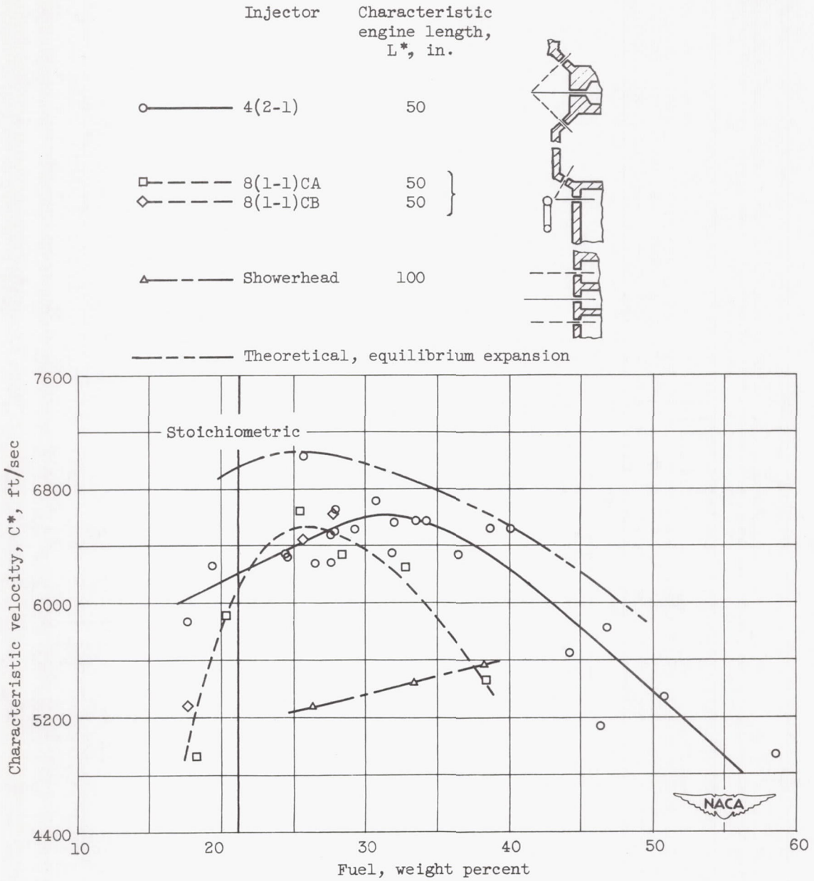
Figure 8. - Theoretical and experimental characteristic velocity of liquid fluorine - liquid ammonia in 100-pound-thrust rocket engines. Chamber pressure, 300 pounds per square inch absolute.
