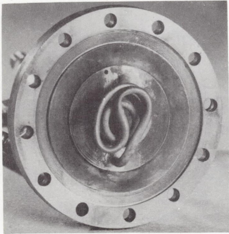
(b) Impinging-jet injector providing for eight sets of one-oxidant-on-one-fuel jets with turbulence coil A (8(1-1)CA).
