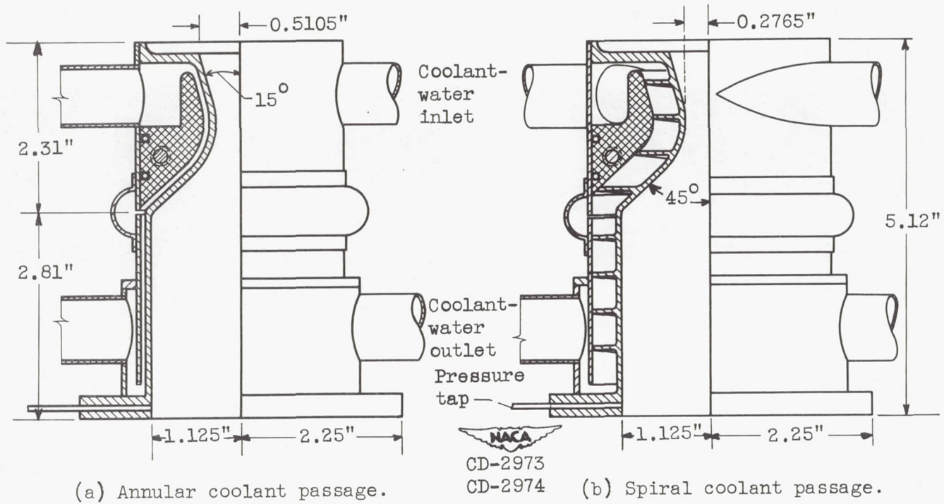
Figure 4. - Diagrammatic sketches of combustion chamber and nozzle assemblies of engines of 50-inch characteristic length.
