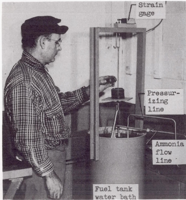
(c) Fuel supply tank.
