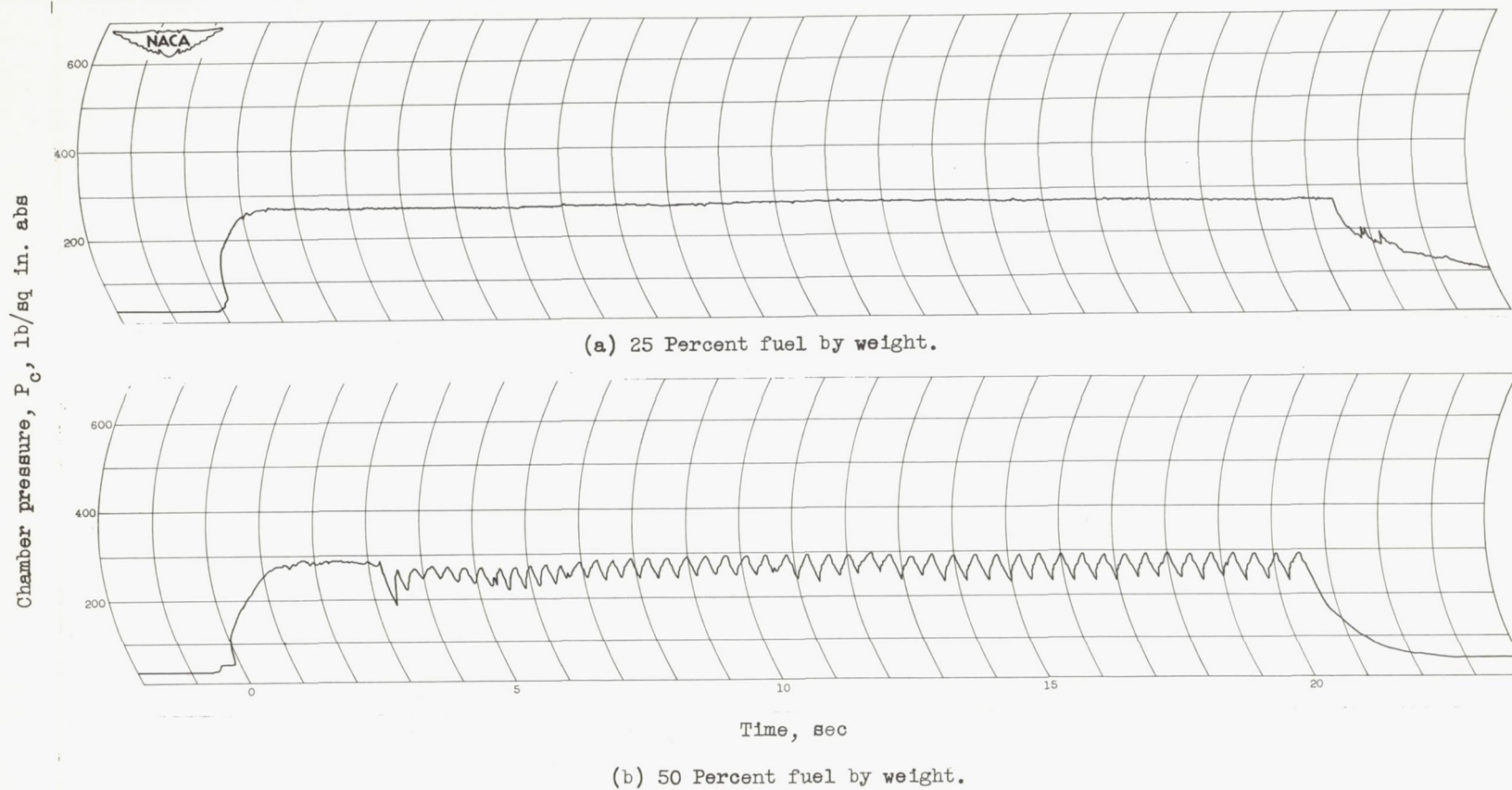
Figure 11. - Chamber-pressure records from runs with 4(2-1) injector at different propellant mixture ratios in 100-pound-thrust rocket engines at chamber pressure of 300 pounds per square inch absolute.
