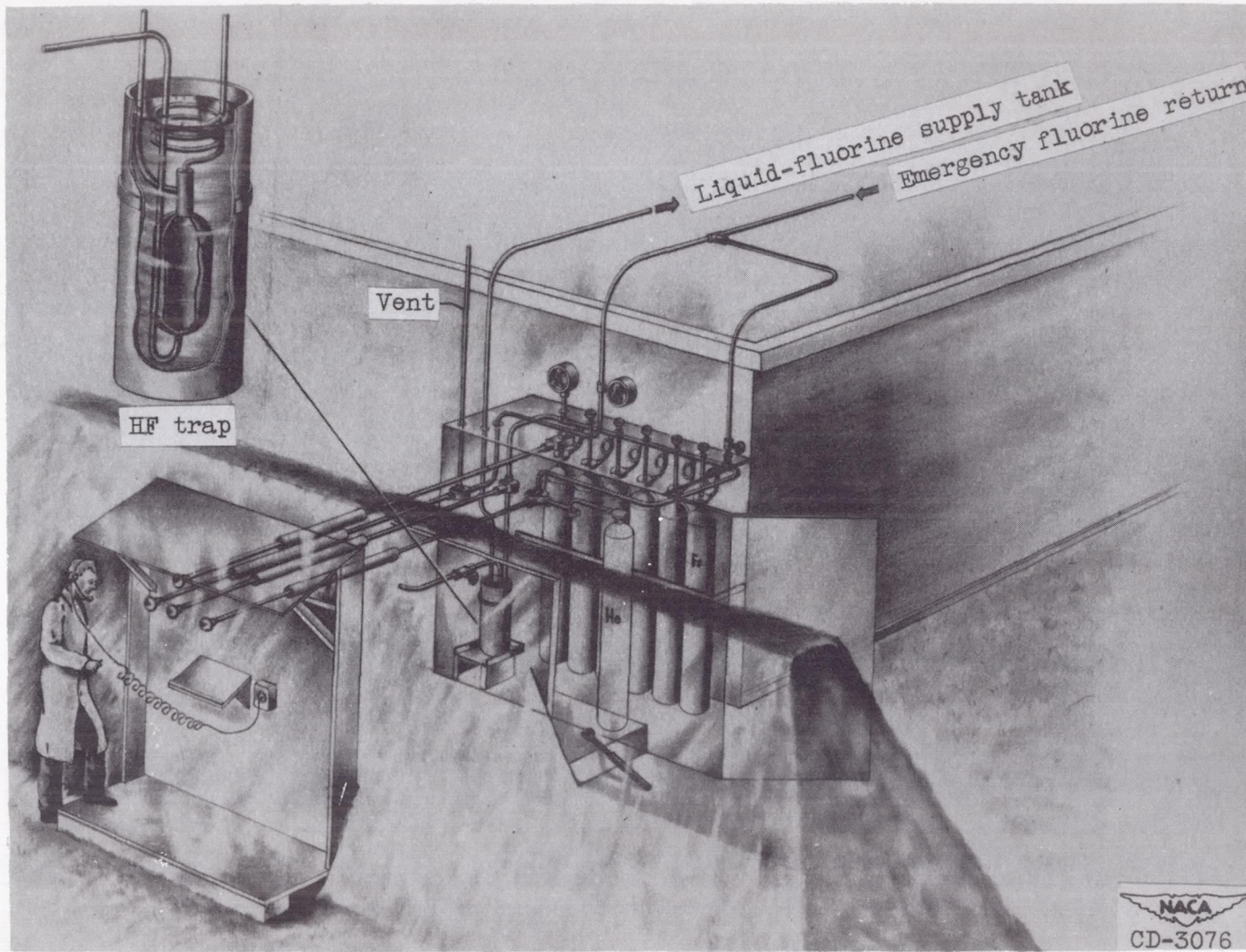
Figure 2. - Gaseous-fluorine supply system.
