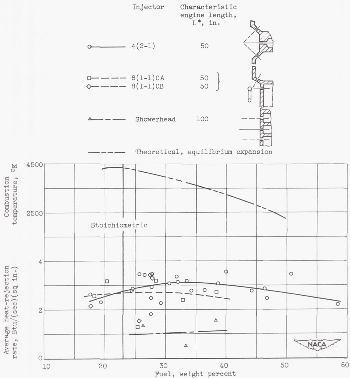
Figure 10. - Theoretical combustion temperature and averaged total experimental heat rejection to complete engine assembly of liquid fluorine - liquid ammonia in 100-pound-thrust rocket engines. Chamber pressure, 300 pounds per square inch absolute.
