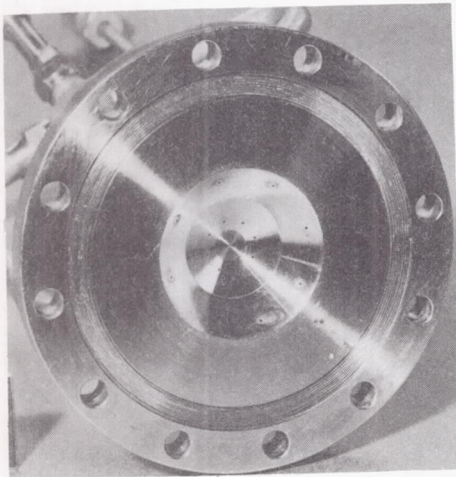
(e) Double-cone injector. Impinging-jet injector providing for impingement of eight fuel jets at common point inside concentric cone formed by eight oxidant streams.
