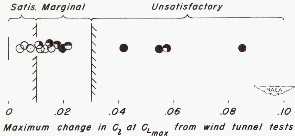
Figure 6.- Correlation of pilots' opinions of stall with changes in C_2 at C_{L_{max}} .
