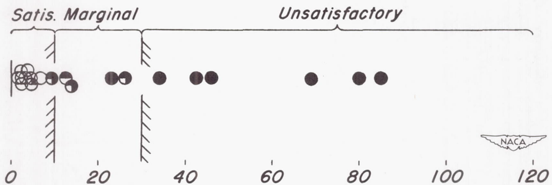
(b) Maximum rolling velocity resulting from initial roll-off, \dot{\phi} , deg/sec.
