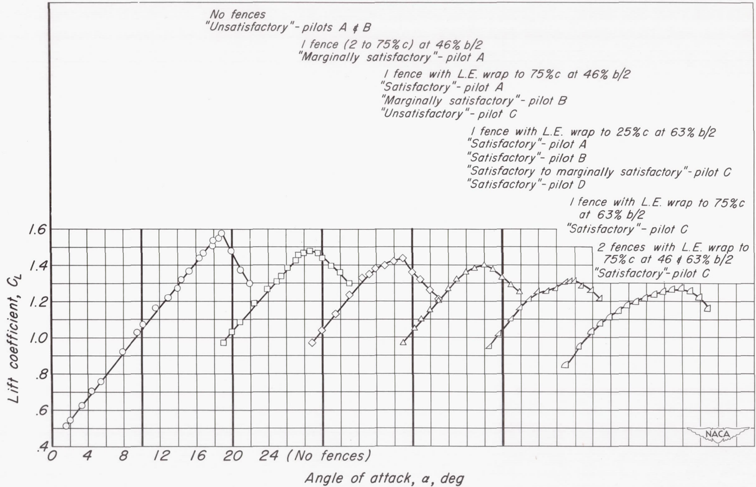
Figure 7.- Lift curves for various configurations measured in flight with cambered leading edge. Flaps down.
