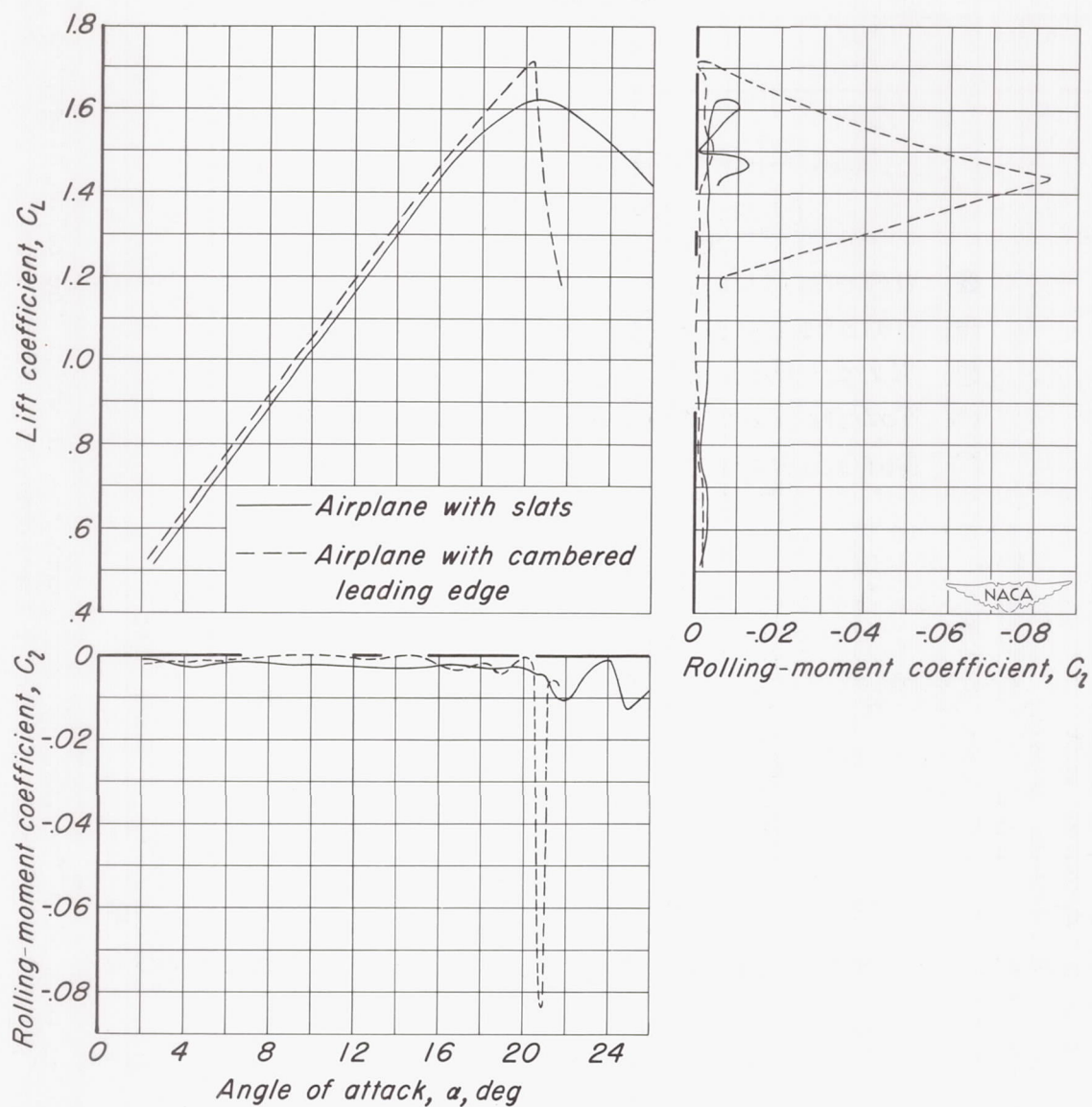
Figure 5.- Lift and rolling-moment characteristics for various configurations.
