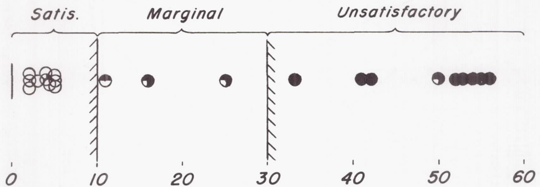
(a) Maximum bank angle resulting from initial roll-off, \phi , deg.
