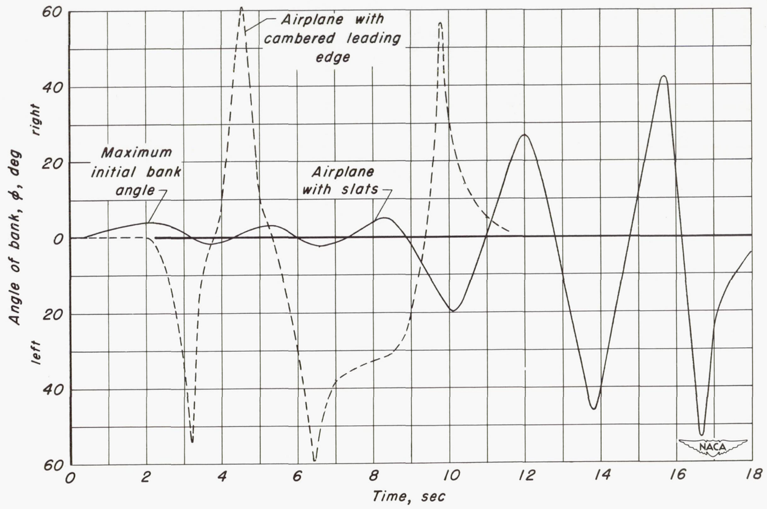
Figure 4.- Time histories of stalls for various configurations in which the pilot attempted to maintain wings level flight by use of the controls. Flaps down.
