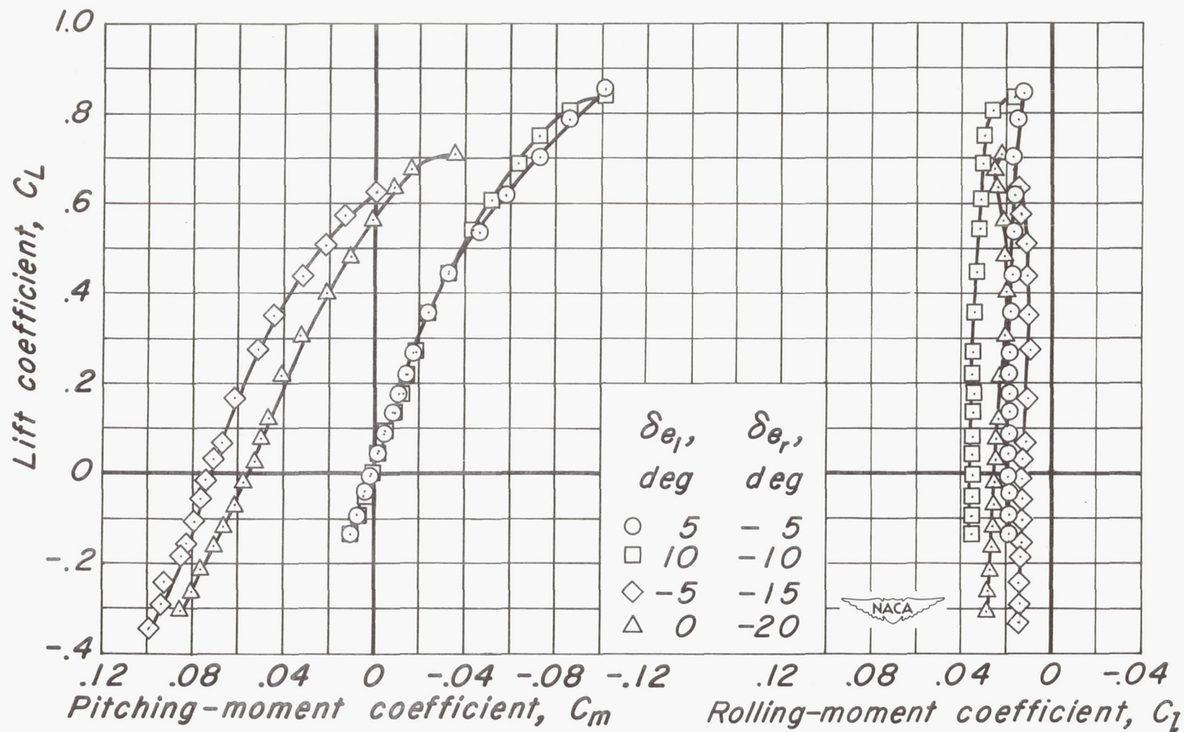
(b) C_L vs C_m , C_L vs C_l Figure 7.- Continued.
