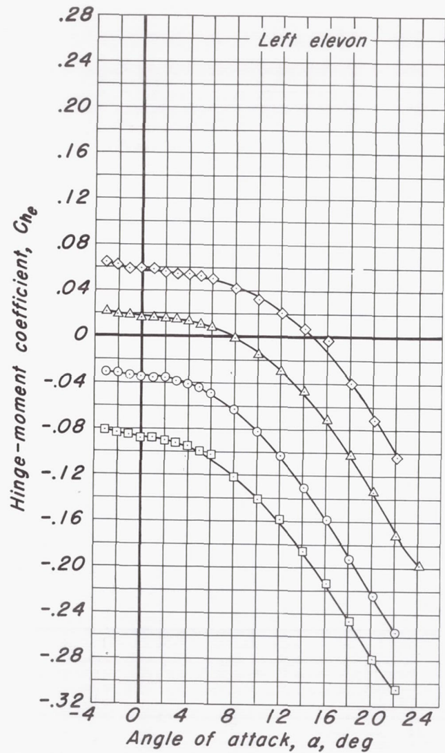
(c) C_{he} vs \alpha Figure 6.- Continued.
