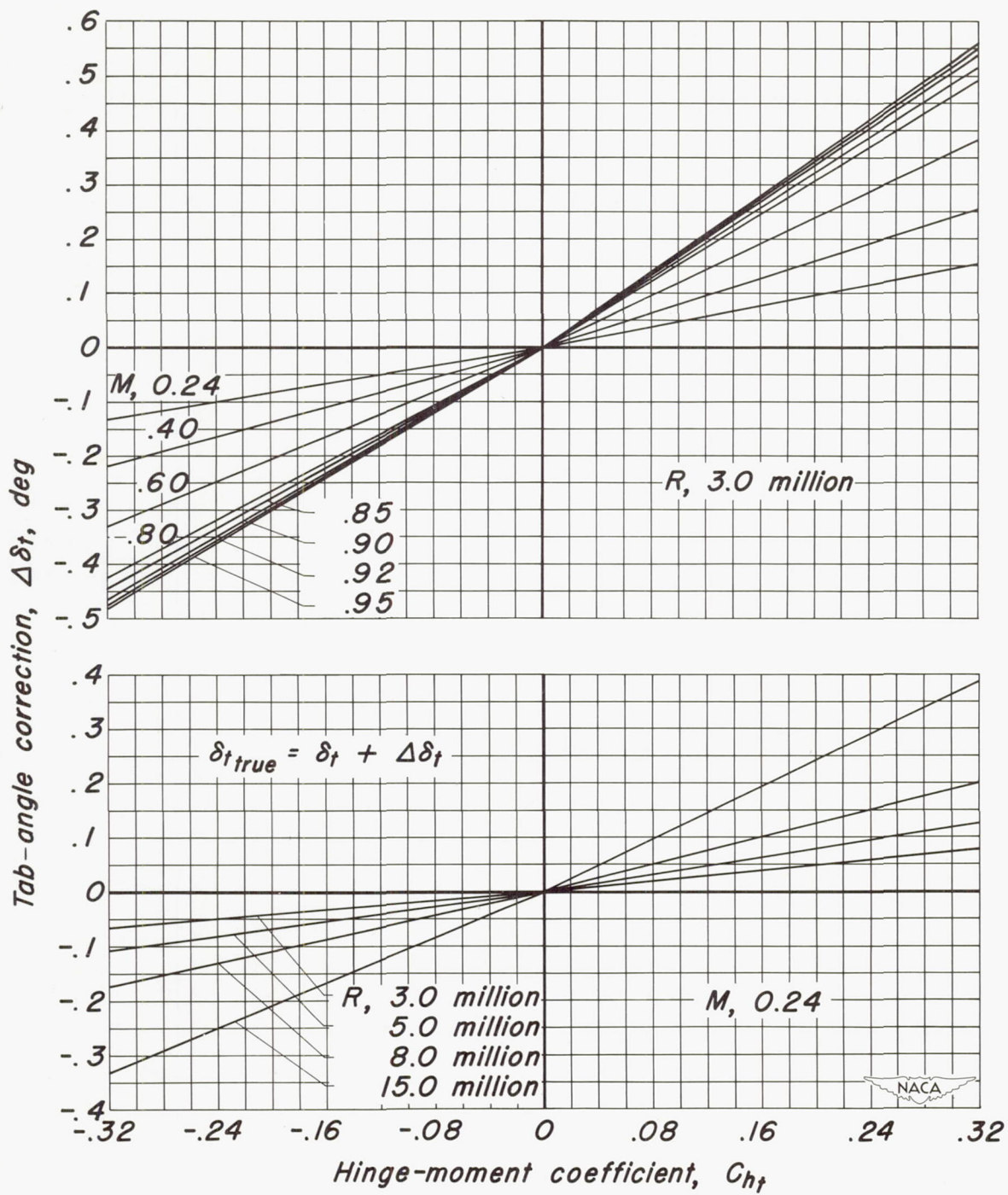
(b) \Delta\delta_t vs C_{h_f}
