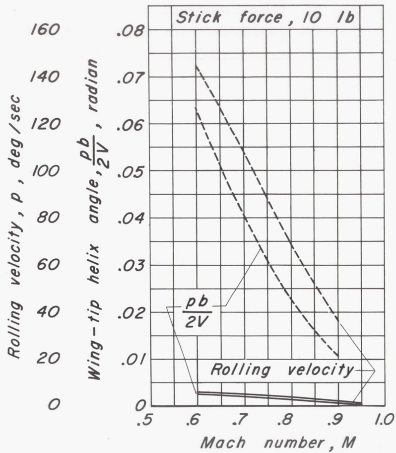
(b) Constant stick force.
