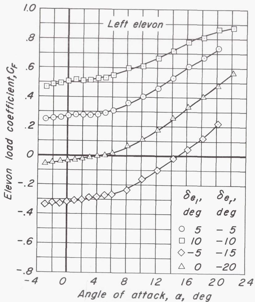
(e) C_F vs \alpha Figure 7.- Continued.
