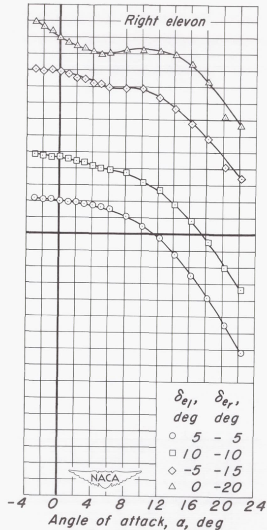
(c) C_{he} vs \alpha Figure 6.- Continued.
