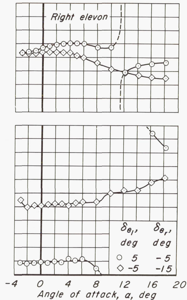
(f) 2y/b vs \alpha , x/c_r vs \alpha
