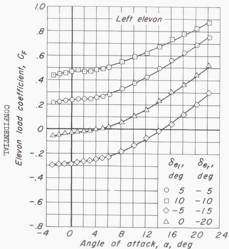
(e) C_F vs \alpha Figure 6- Continued.
