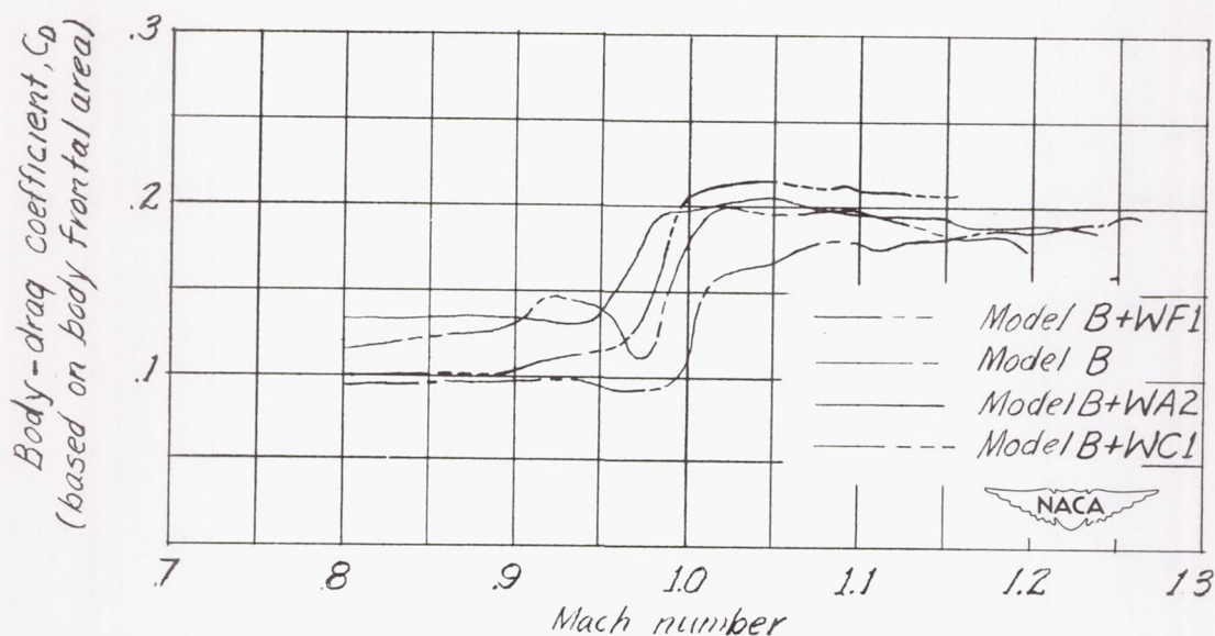
Figure 11.- Comparison of variations with Mach number of body drag coefficient for several configurations illustrating the effect of wing position on wing-body interference.
