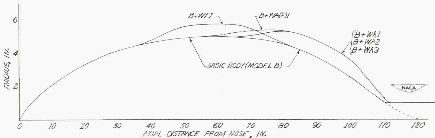
Figure 13.- Comparison of the shapes of bodies of revolution having the same axial distribution of cross-sectional area as wing-body configurations B + WA1 , B + WA2 , B + WA3 , B + WF1 , and B + WA(F) with the basic body shape (model B).
