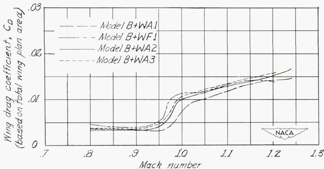
Figure 7.- Comparison of results for models B + WA2 and B + WA3 with results for similar models tested previously. Variation of wing drag coefficient with Mach number.
