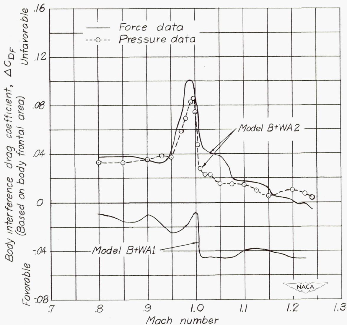
Figure 10.- Variation of Mach number of the body interference drag coefficient for model B + WA2 obtained from two independent measurements. Data for model B + WA1 is included for comparison.
