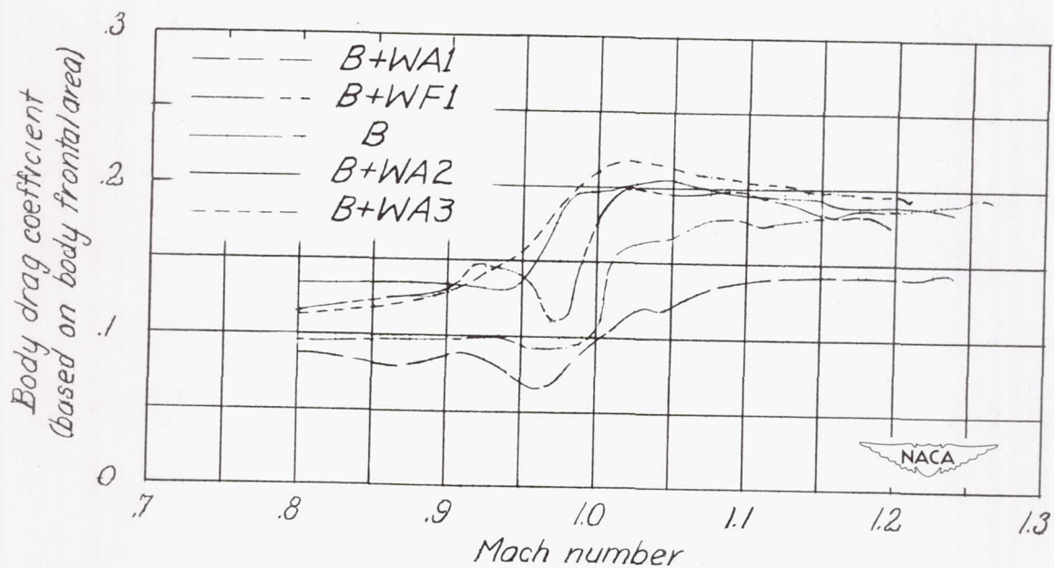
Figure 9.- Comparison of results for models B + WA2 and B + WA3 with results for similar models tested previously. Variation of body drag coefficient with Mach number.
