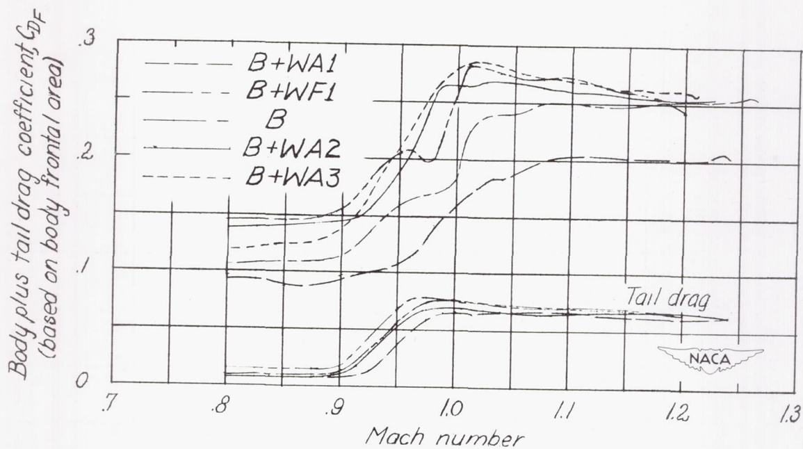
Figure 8.- Comparison of results for models B + WA2 and B + WA3 with results for similar models tested previously. Variation with Mach number of the drag coefficient of the body-tail combination.
