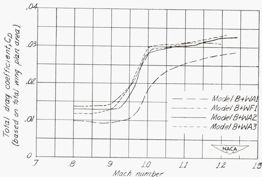
Figure 6.- Comparison of results for models B + WA2 and B + WA3 with results for similar models tested previously. Variation of total drag coefficient with Mach number.
