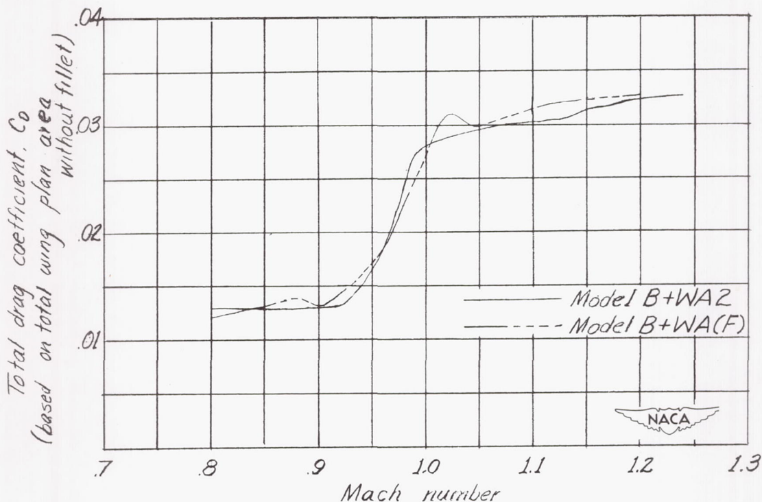
Figure 12.- Comparison of variations with Mach number of total drag coefficient for a wing-body combination with (model B + WA(F)) and without (model B + WA2) a large wing fillet.
