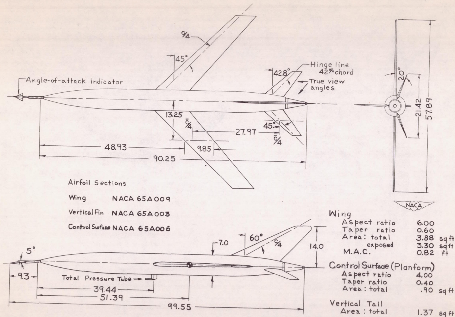
Figure 1.- Physical characteristics of model. All linear dimensions in inches.
