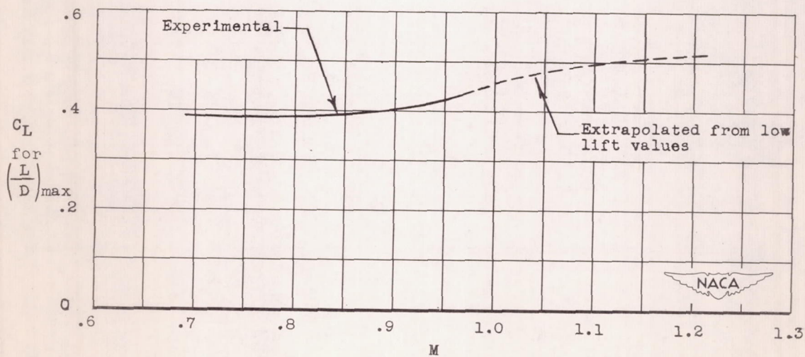
Figure 17.- Lift coefficients for maximum lift-drag ratios.
