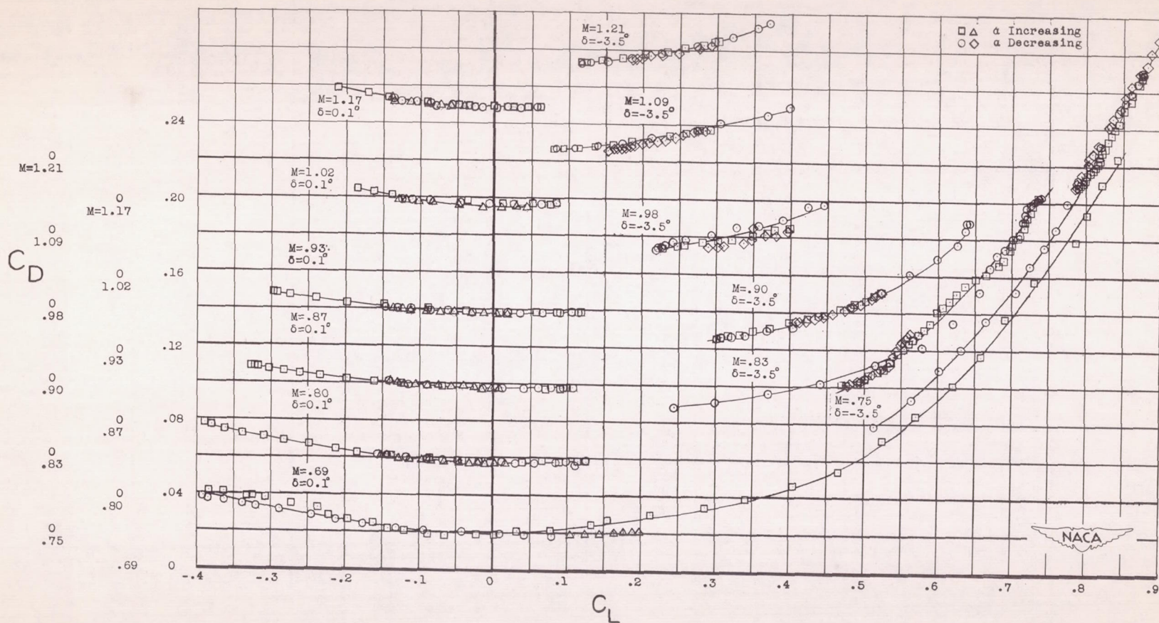
Figure 13.- Variation of drag with lift.
