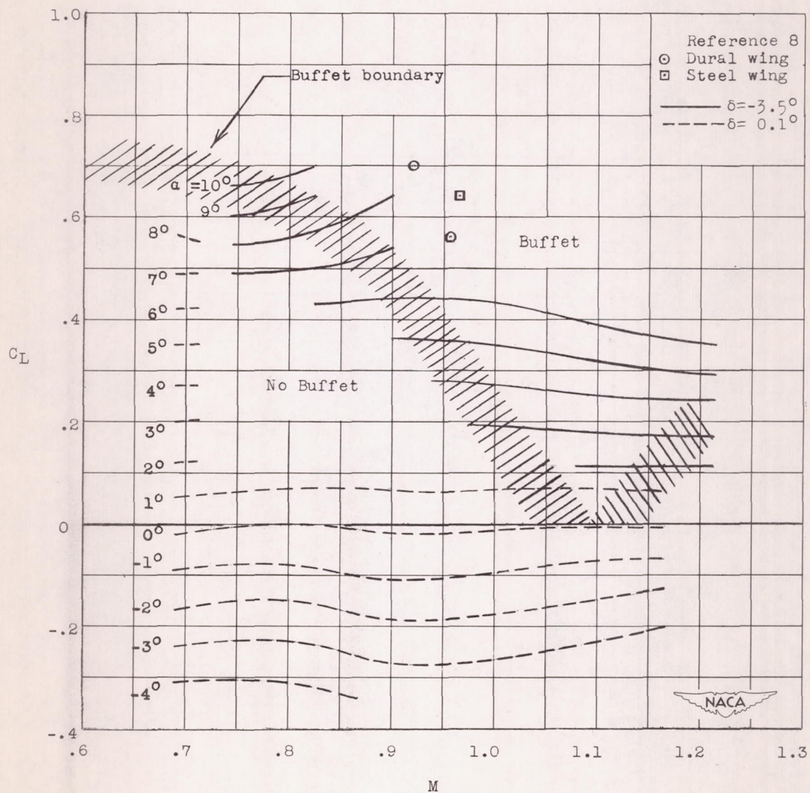
Figure 9.- Lift coefficients for constant angles of attack plotted against Mach number.
