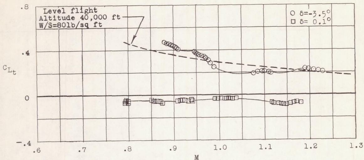
(a) Trim lift coefficient plotted against Mach number.
