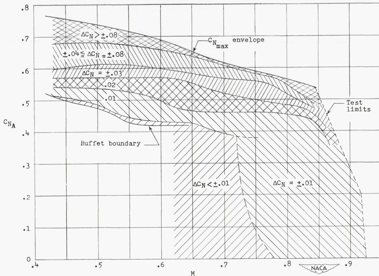
Figure 8.- The variation of buffet intensities with airplane normal-force coefficient and Mach number. Northrop X-4 airplane; h_p \approx 30,000 feet.
