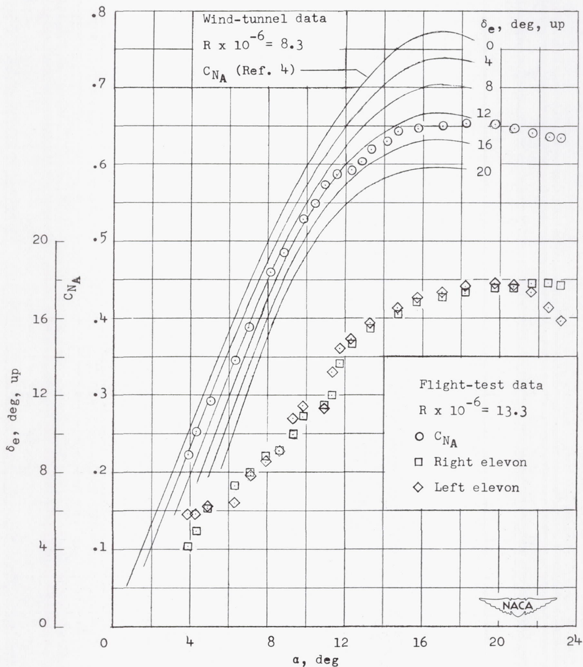
Figure 5.- Variation of flight-determined airplane normal-force coefficient and elevon positions with angle of attack and comparison with wind-tunnel normal-force coefficients at various elevon positions. M \approx 0.6 .
