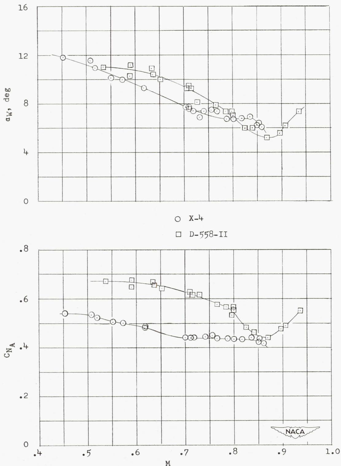
Figure 10.- Comparison of the buffet intensity-rise boundaries of the Northrop X-4 and Douglas D-558-II airplanes. h_p \approx 30,000 feet.
