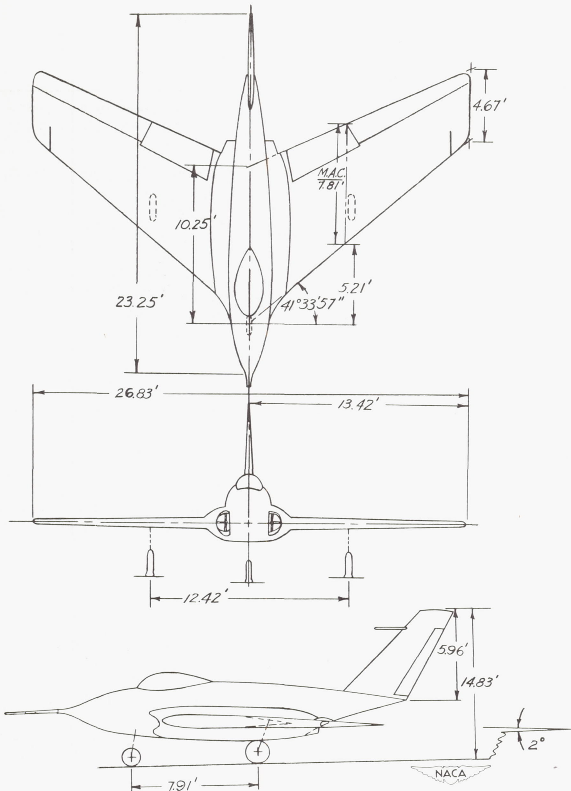
Figure 2.- Three-view drawing of Northrop X-4 airplane.
