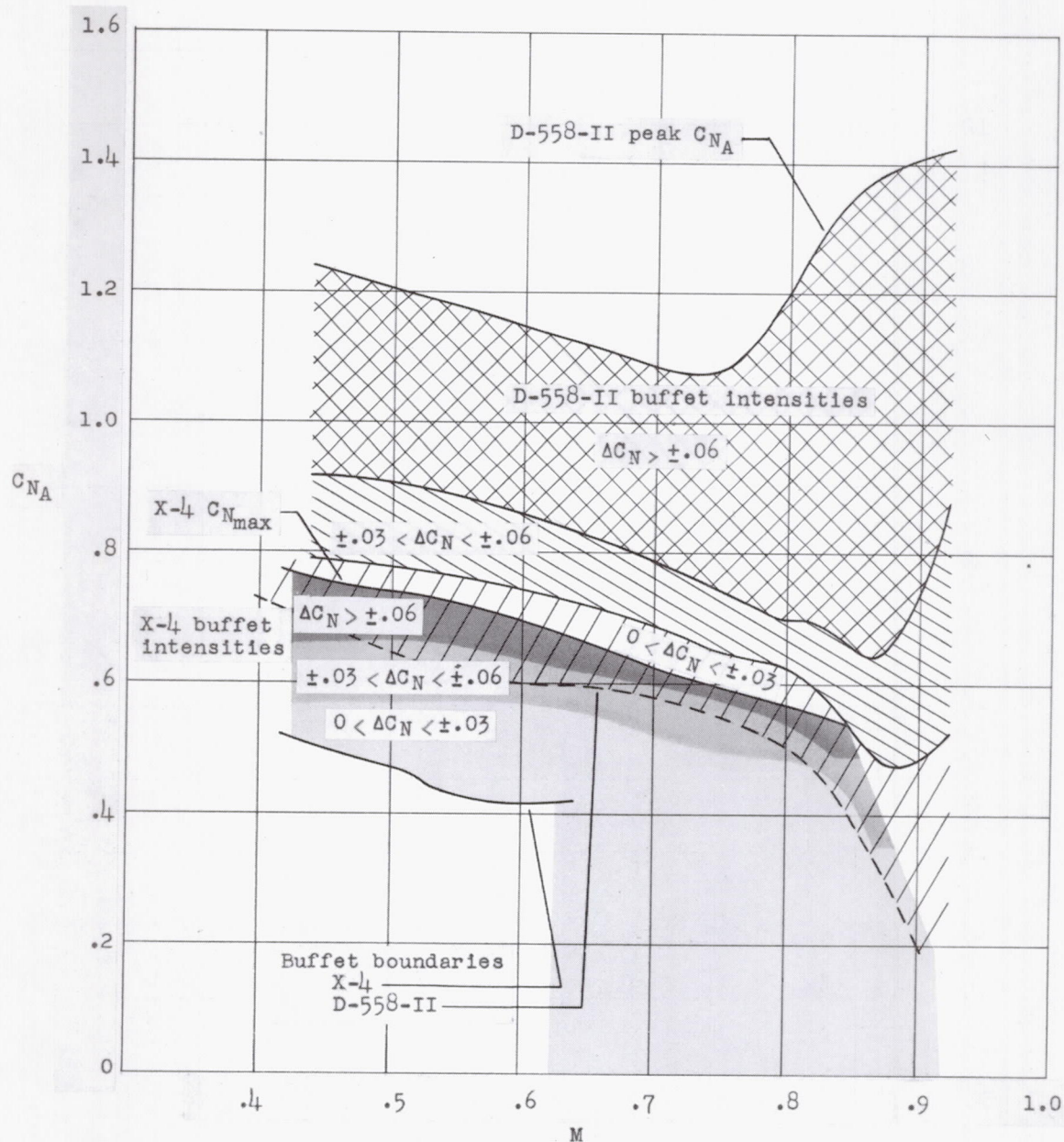
Figure 9.- Comparison of the buffet intensities experienced by the Northrop X-4 airplane with those encountered by the Douglas D-558-II airplane. h_p \approx 30,000 feet.
