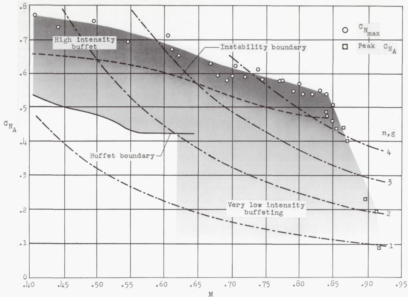
Figure 4.- Operational region of the Northrop X-4 airplane.
