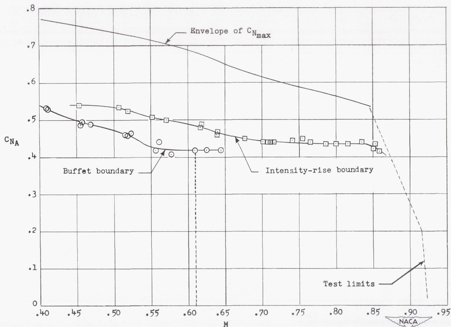
Figure 7.- The buffet boundary and buffet intensity-rise boundary for the Northrop X-4 airplane. h_p \approx 30,000 feet.
