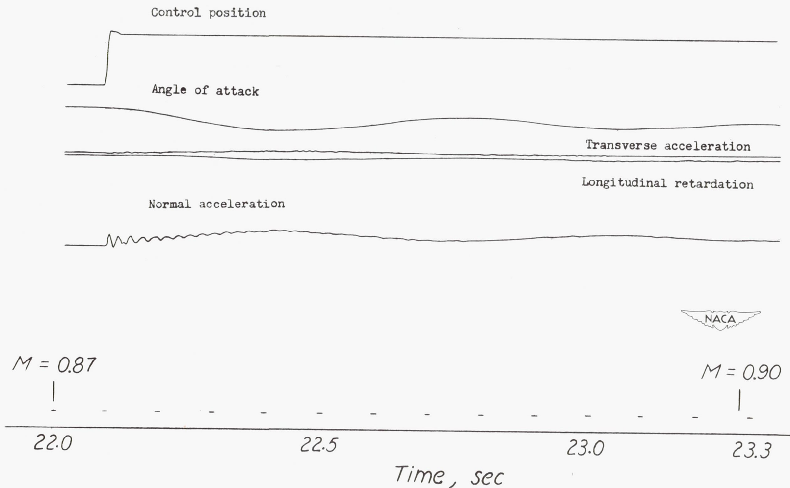
Figure 7.- Full-size reproduction of a section of the record film.
