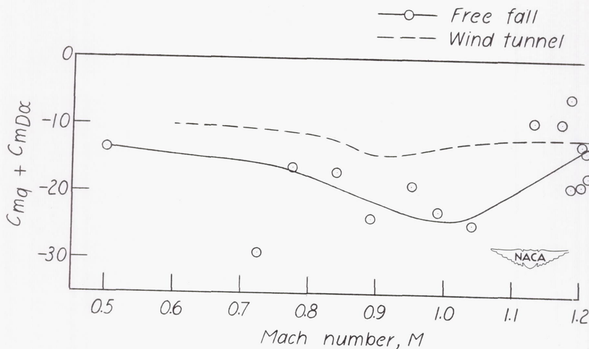
Figure 16.- Variation with Mach number of the damping derivative C_{mq} + C_{mD\alpha} .
