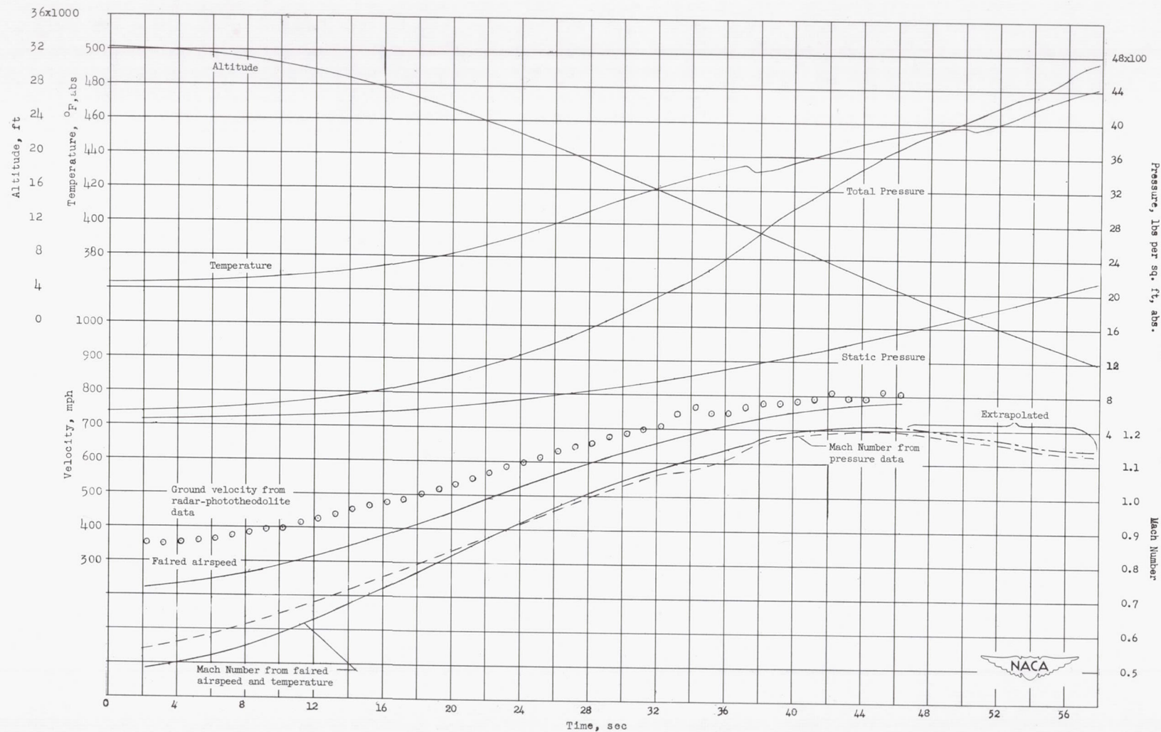
Figure 6.- Quantities used to determine Mach number.
