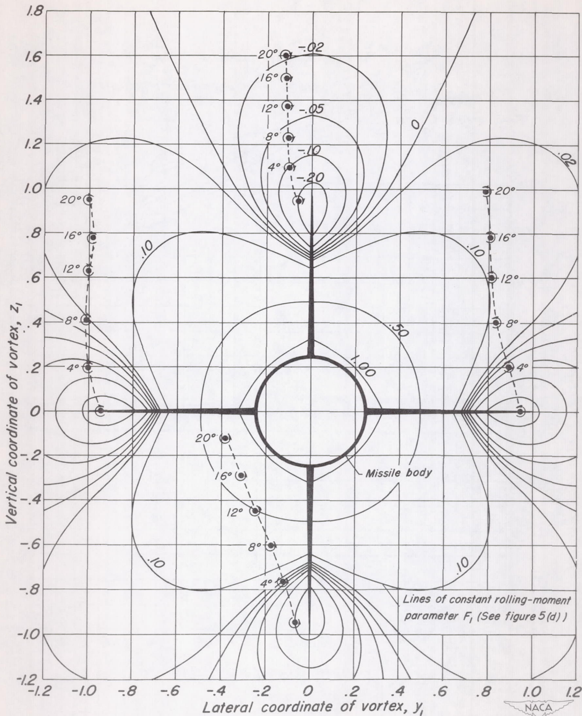
Figure 18.- Relationship between the position of the vortex cores at various angles of attack and lines of constant rolling-moment parameter, F_1 , in the cross-flow plane at the center of pressure of the trailing wing of missile C at 1.4 Mach number.
