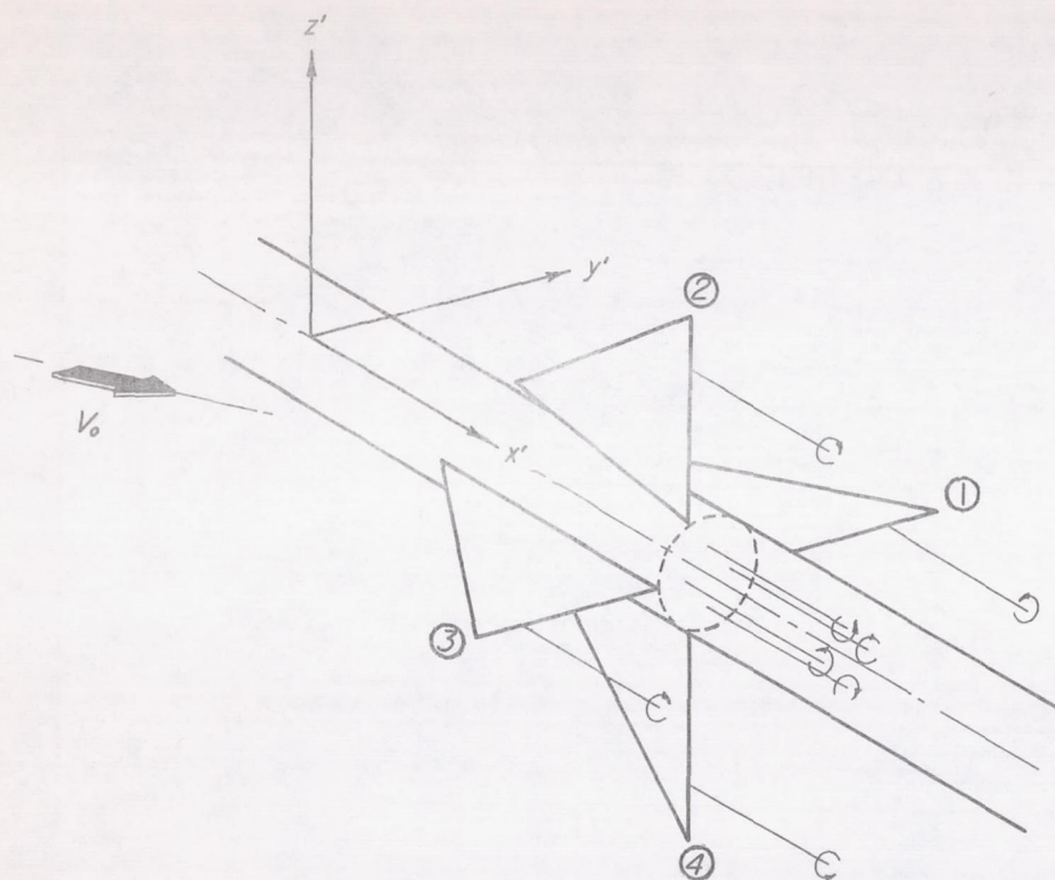
(a) Three-dimensional view showing wing and body and vortex filament arrangement.
