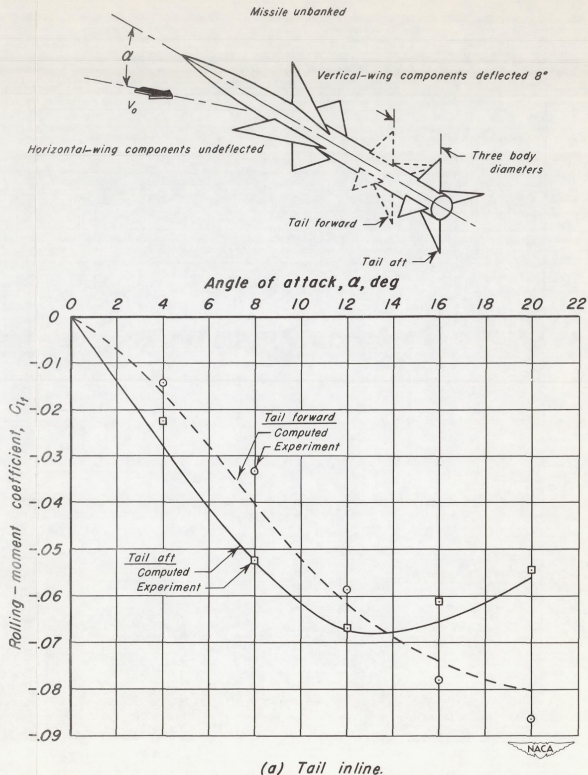
Figure 8.- Calculated and experimental tail rolling moments at 1.4 Mach number for Missile A.
