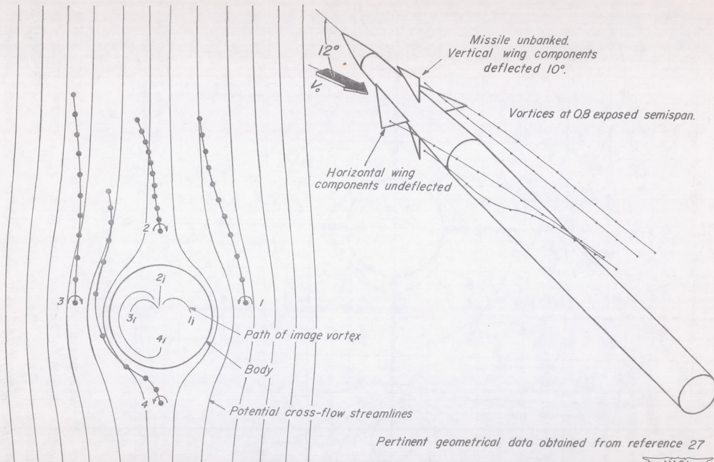
Figure 20.-Vortex paths downstream of the control fins of missile D at 12° angle of attack.
