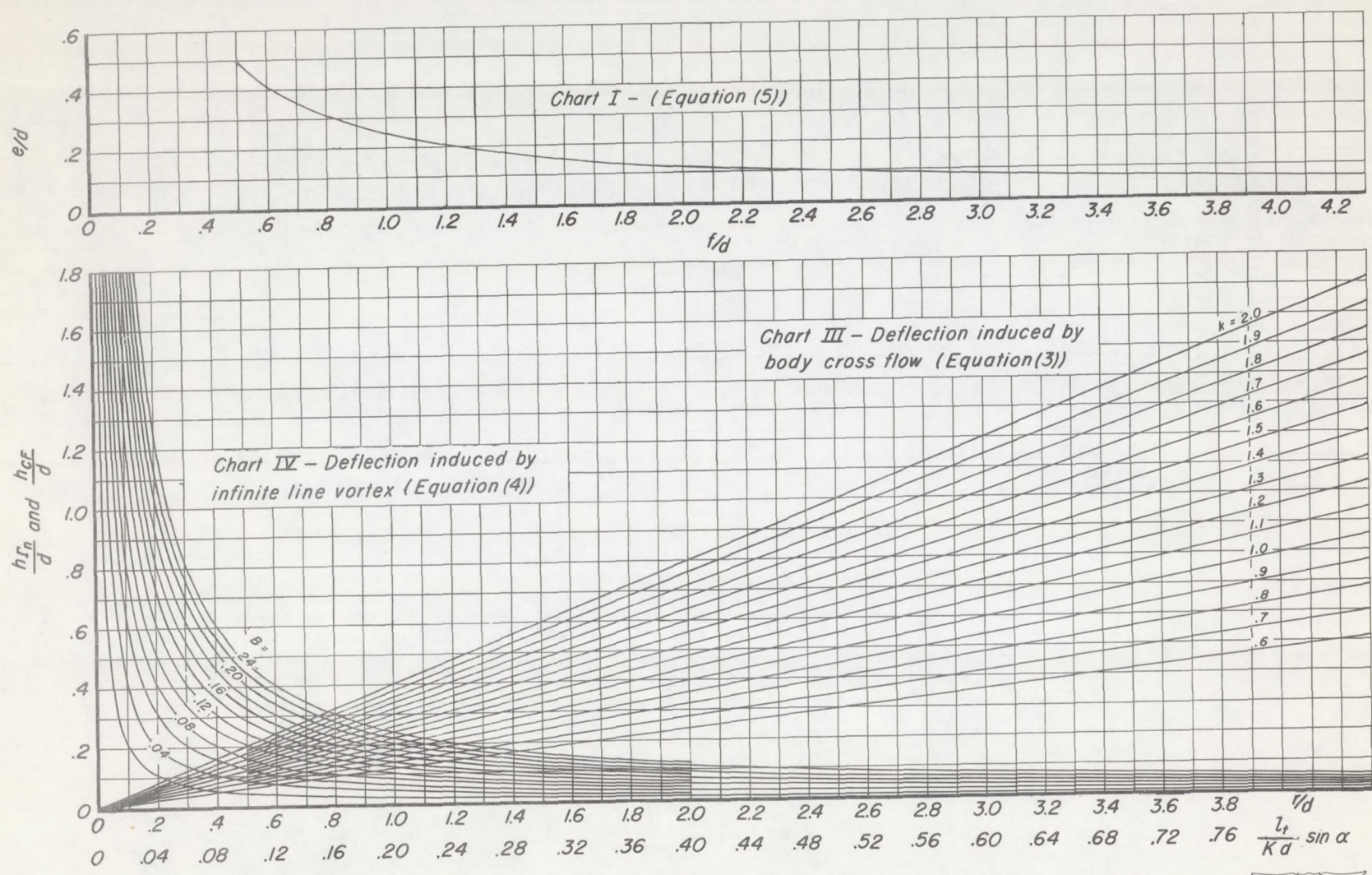
(a) Graphs of the aerodynamic and geometric parameters given in equations (3), (4), and (5).
