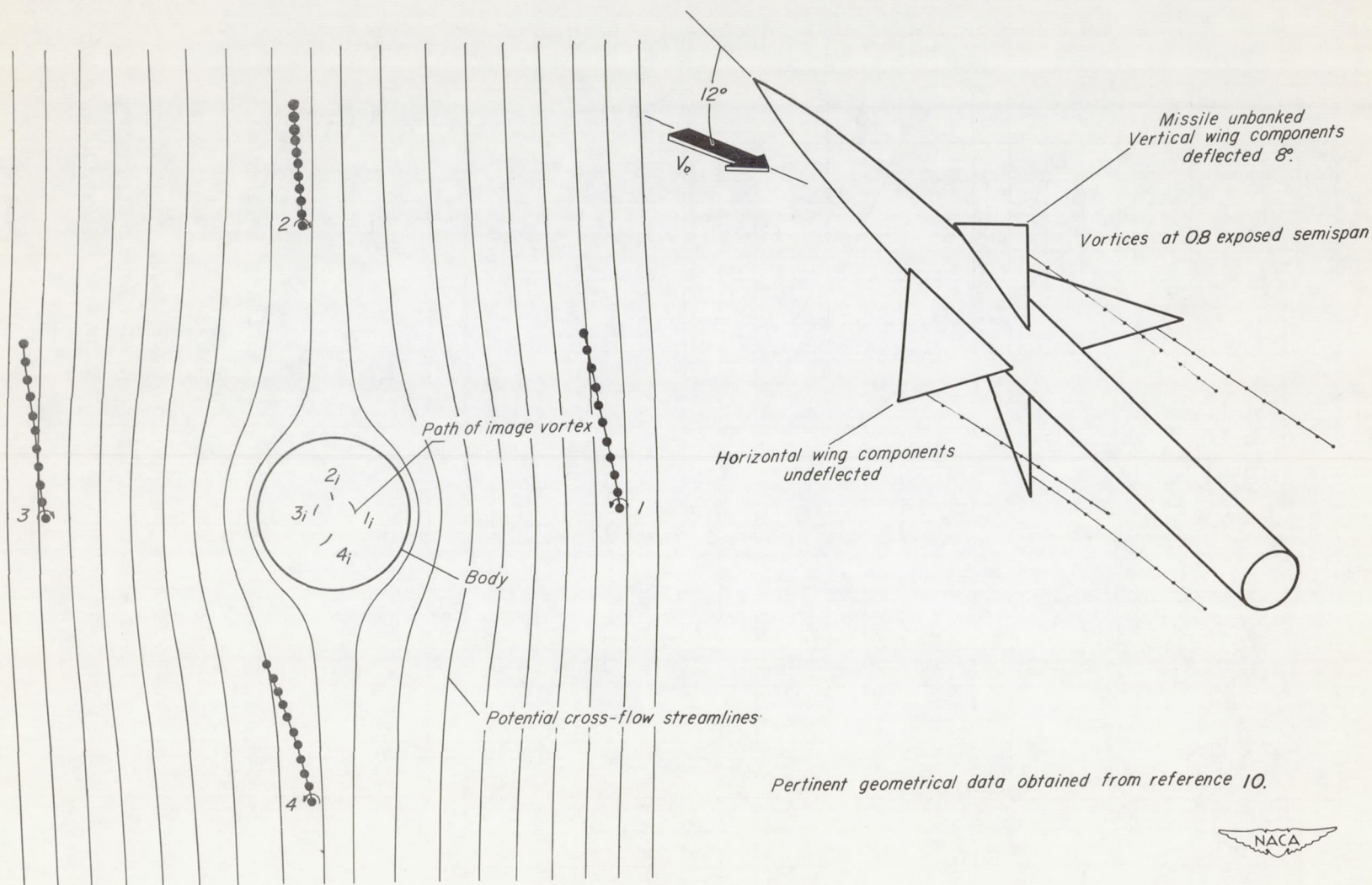
Figure 17. - Vortex paths downstream of the control fins of missile C at 12° angle of attack.
