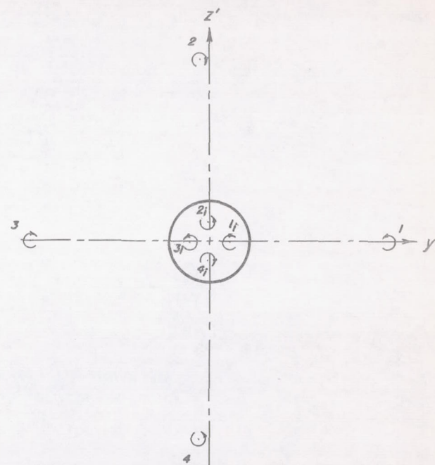
(b) Vortex positions in the plane of the wing trailing edge.
