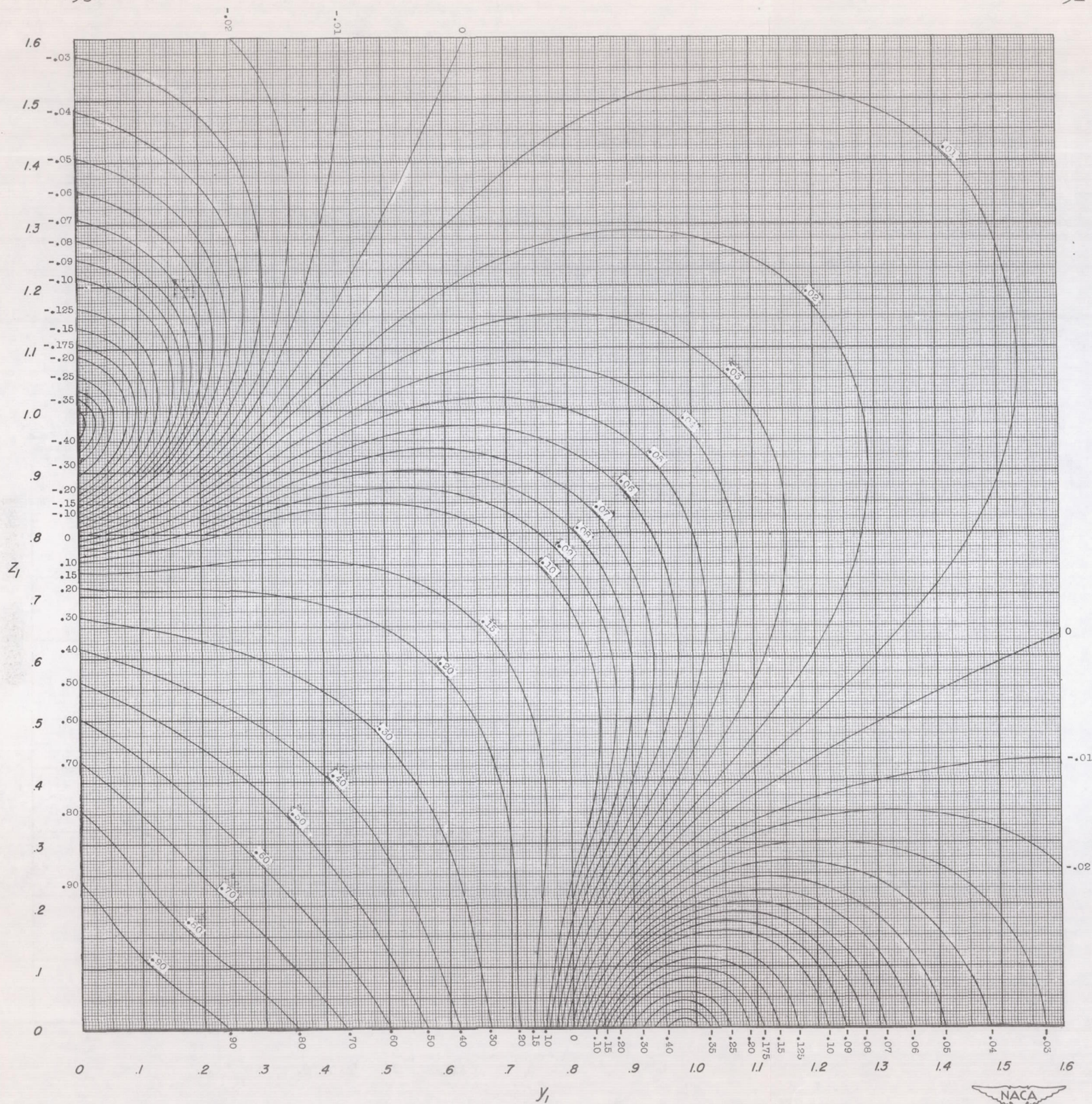
Figure 7.- Chart for determining values of the rolling-moment parameter, F_B , as a function of the vortex coordinates (y_1, z_1) .
