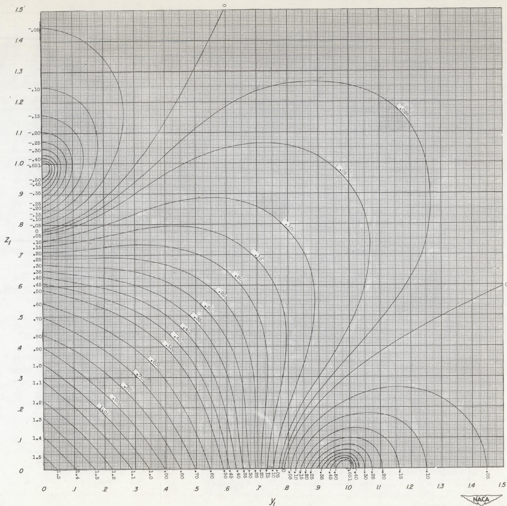
Figure 6.- Chart for determining values of the rolling-moment parameter, F_A , as a function of the vortex coordinates (y_1, z_1) .
