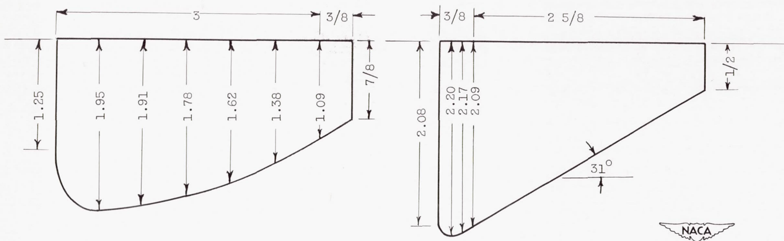
(a) Diffuser contour A.
