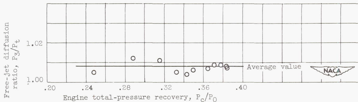
Figure 6. - Effect of supercritical engine recovery on free-jet diffusion. Mach number, 2.98; nozzle size, 1.85; over-all pressure ratio, 6.8.
