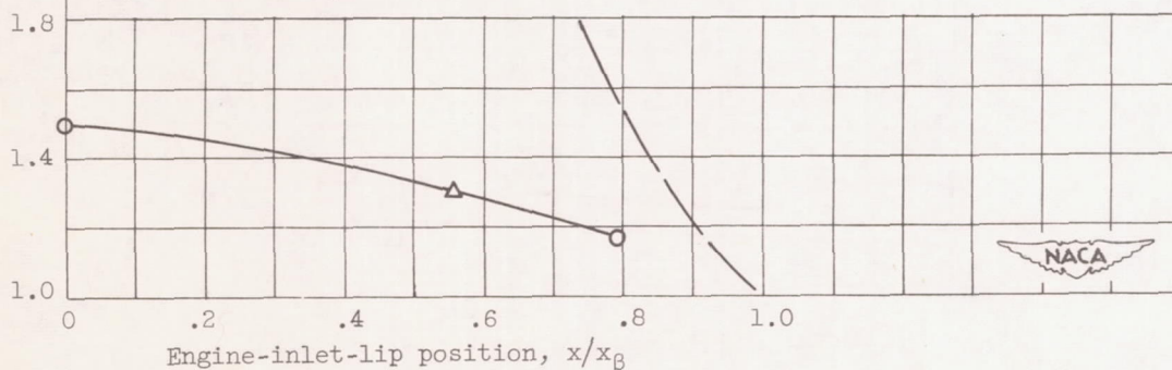
(c) Mach number, 2.18; nozzle size, 1.35.
