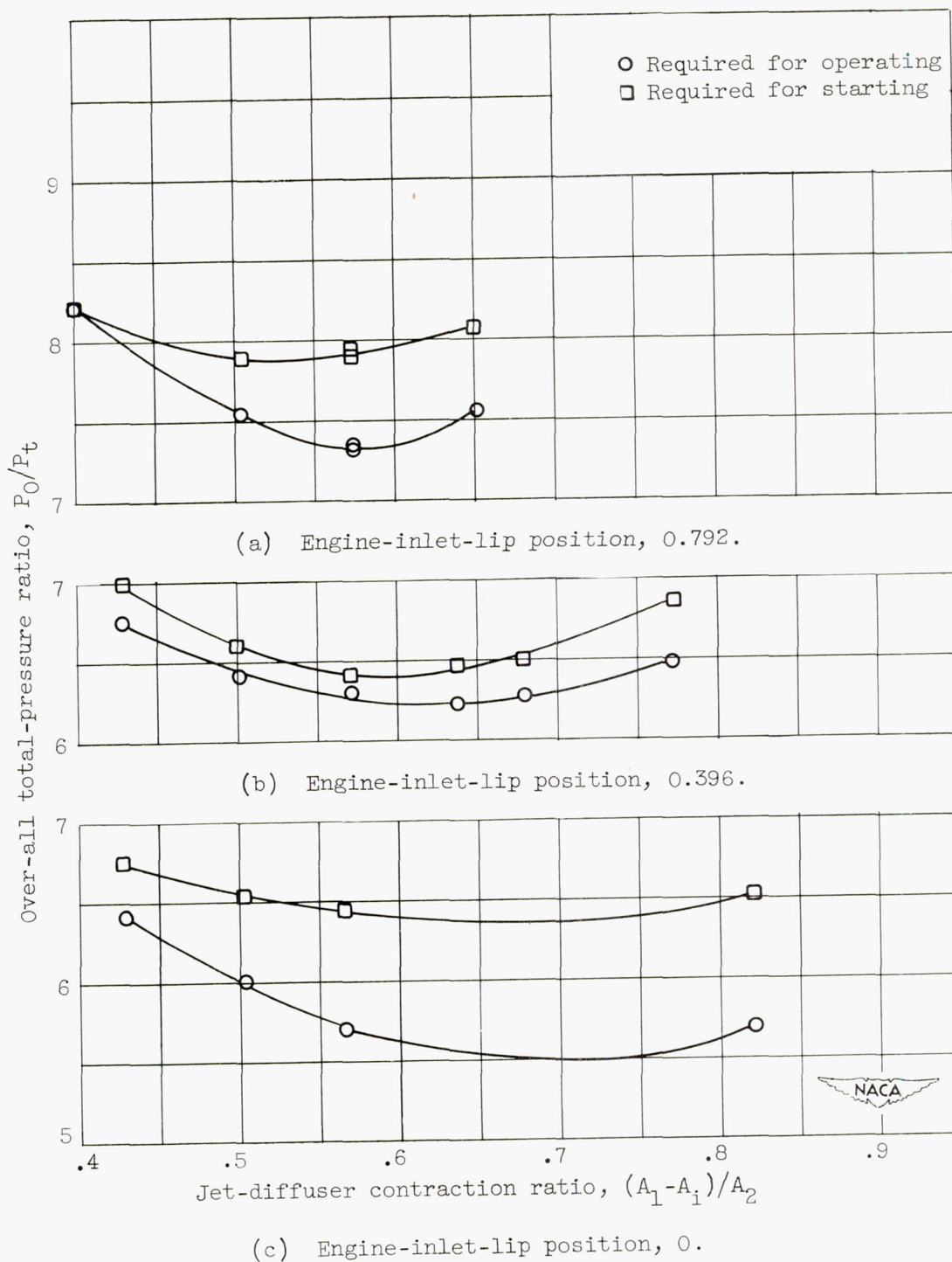
Figure 8. - Variation of required over-all starting and operating pressure ratio with jet-diffuser contraction ratio for several engine-inlet-lip positions. Mach number, 2.98; nozzle size, 1.85.
