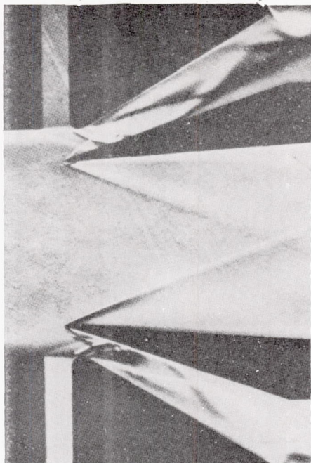
(a) Over-all total-pressure ratio, 13.8; plenum pressure, 0.90.
