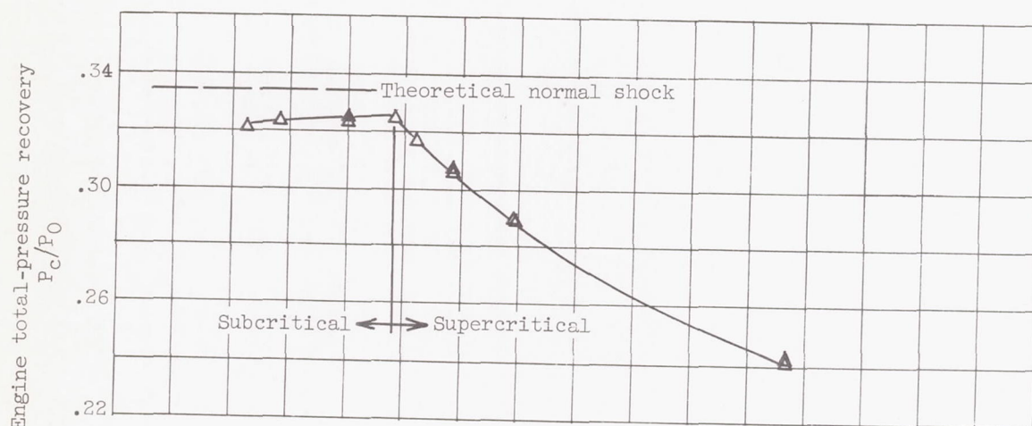
(a) Engine pressure recovery.
