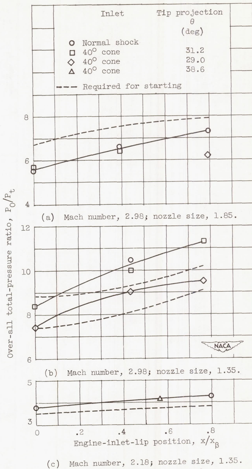
Figure 14. - Required over-all total-pressure ratios for shock-free flow into engine inlet.
