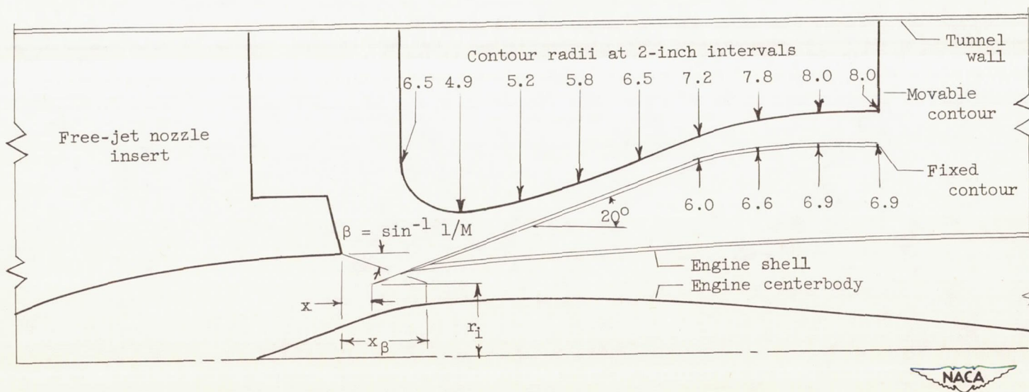
Figure 2. - Scale diagram of diffuser contour, one-fourth size.
