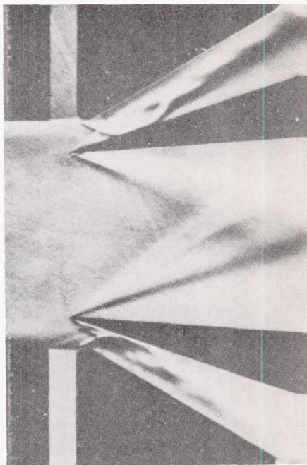
(b) Over-all total-pressure ratio, 8.06; plenum pressure, 0.90.
