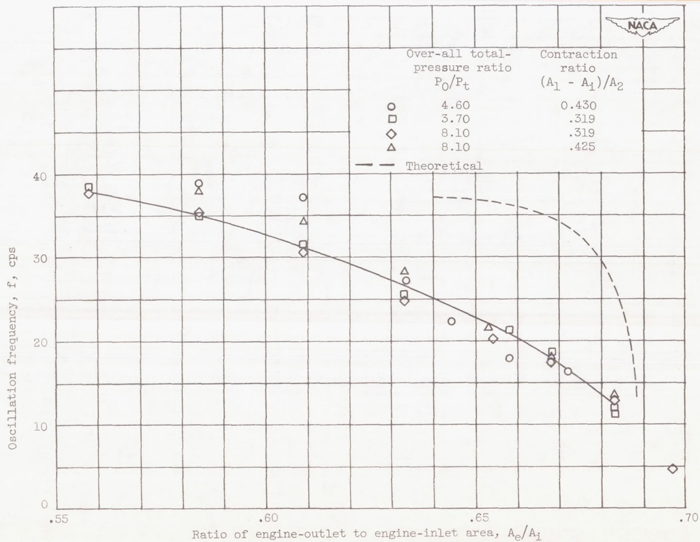
Figure 16. - Engine combustion-chamber-pressure oscillation for subcritical inlet flow. Mach number, 2.18; nozzle size, 1.35; engine-inlet-lip position, 0.557.
