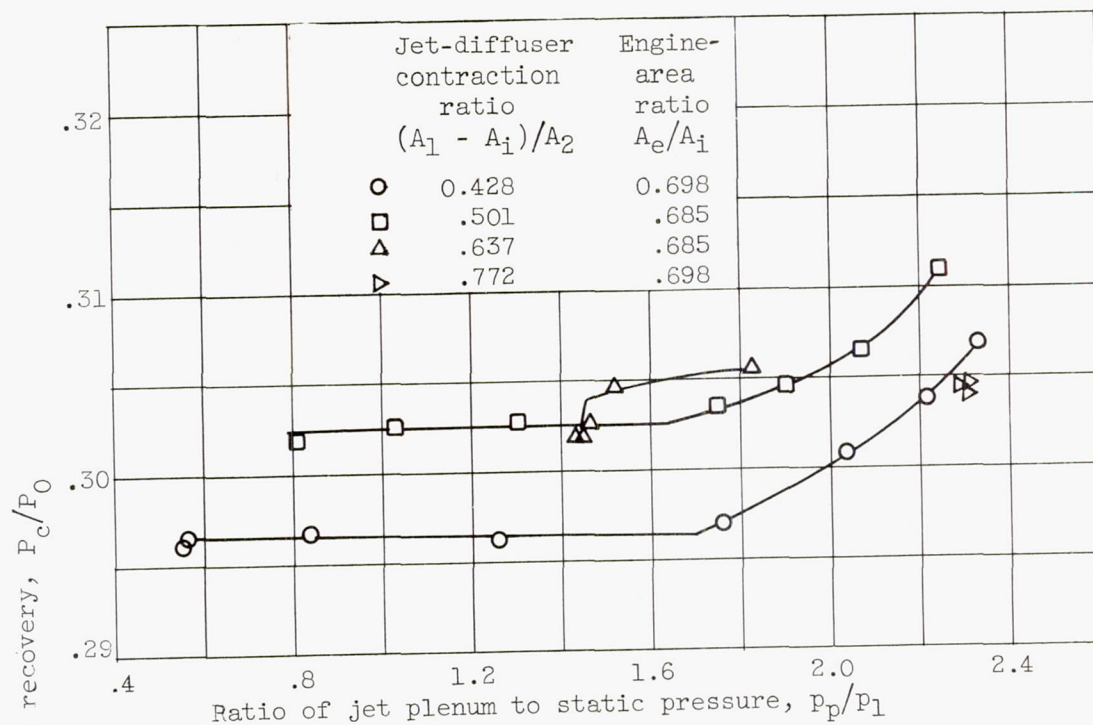
(a) Jet plenum pressure.
