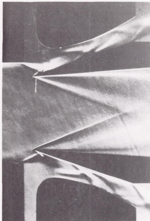
(b) Contraction ratio, 0.852; plenum pressure, 1.502.
