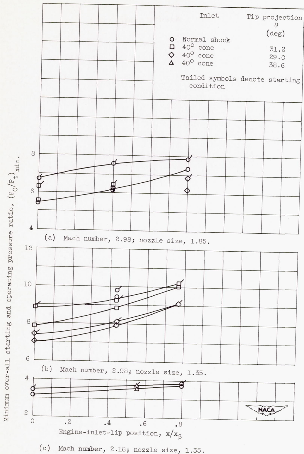
Figure 9. - Minimum over-all starting and operating pressure ratios as affected by engine-inlet-lip position.
