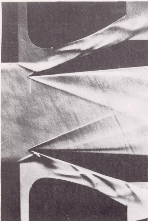
(a) Contraction ratio, 0.795; plenum pressure, 1.408.
