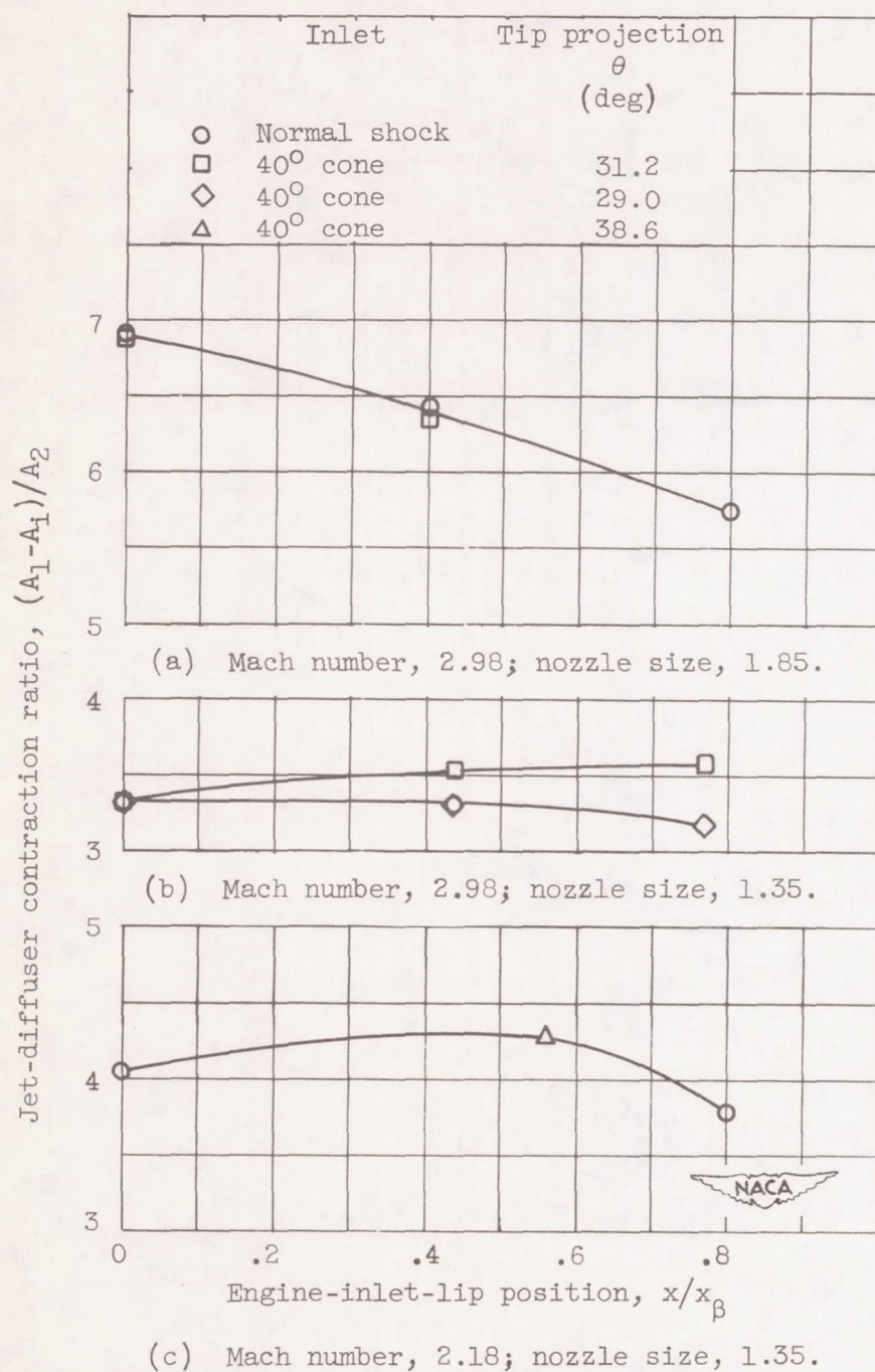
Figure 15. - Optimum jet-diffuser contraction ratio.
