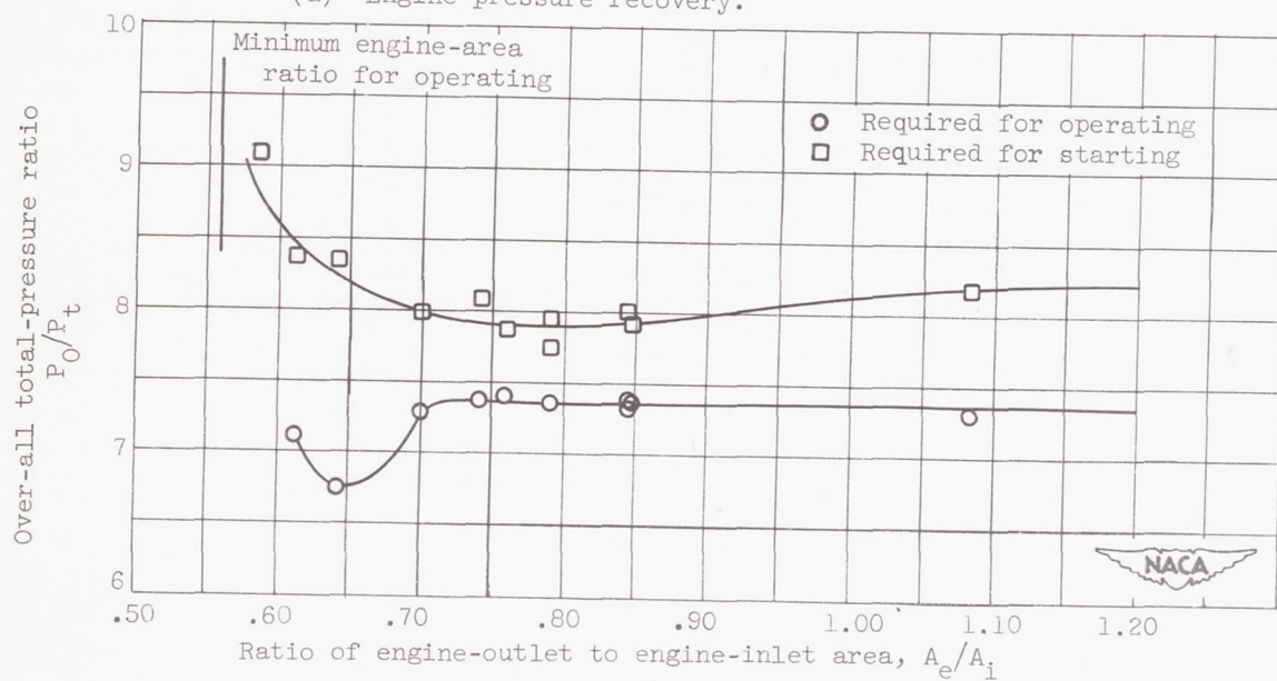
(b) Starting and operating pressure ratios.
