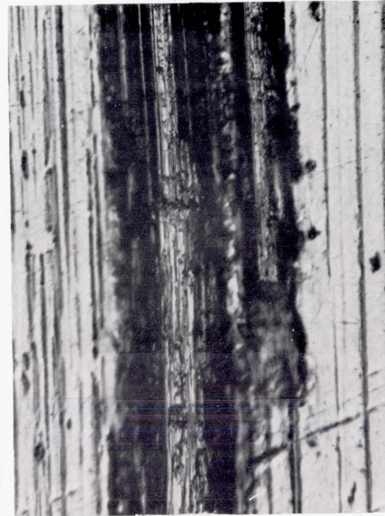
(d) Damage type d, similar materials (stainless steel against stainless steel); coefficient of friction \mu , 0.96.
