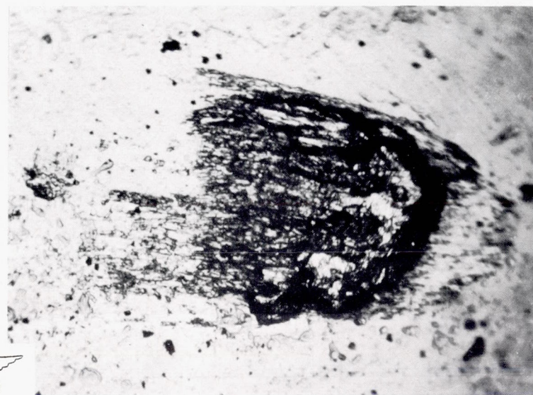
(b) Mating surface of tungsten carbide slider after sliding several hundredths of inch.
