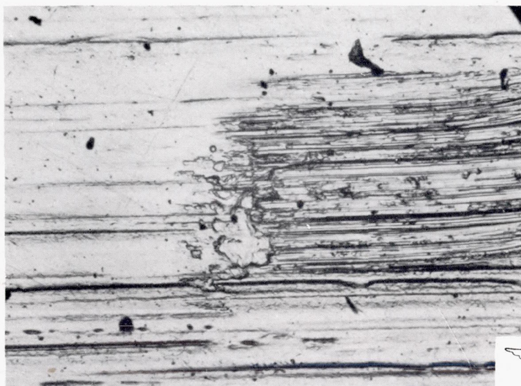
(a) Wear track on stainless-steel plate.
