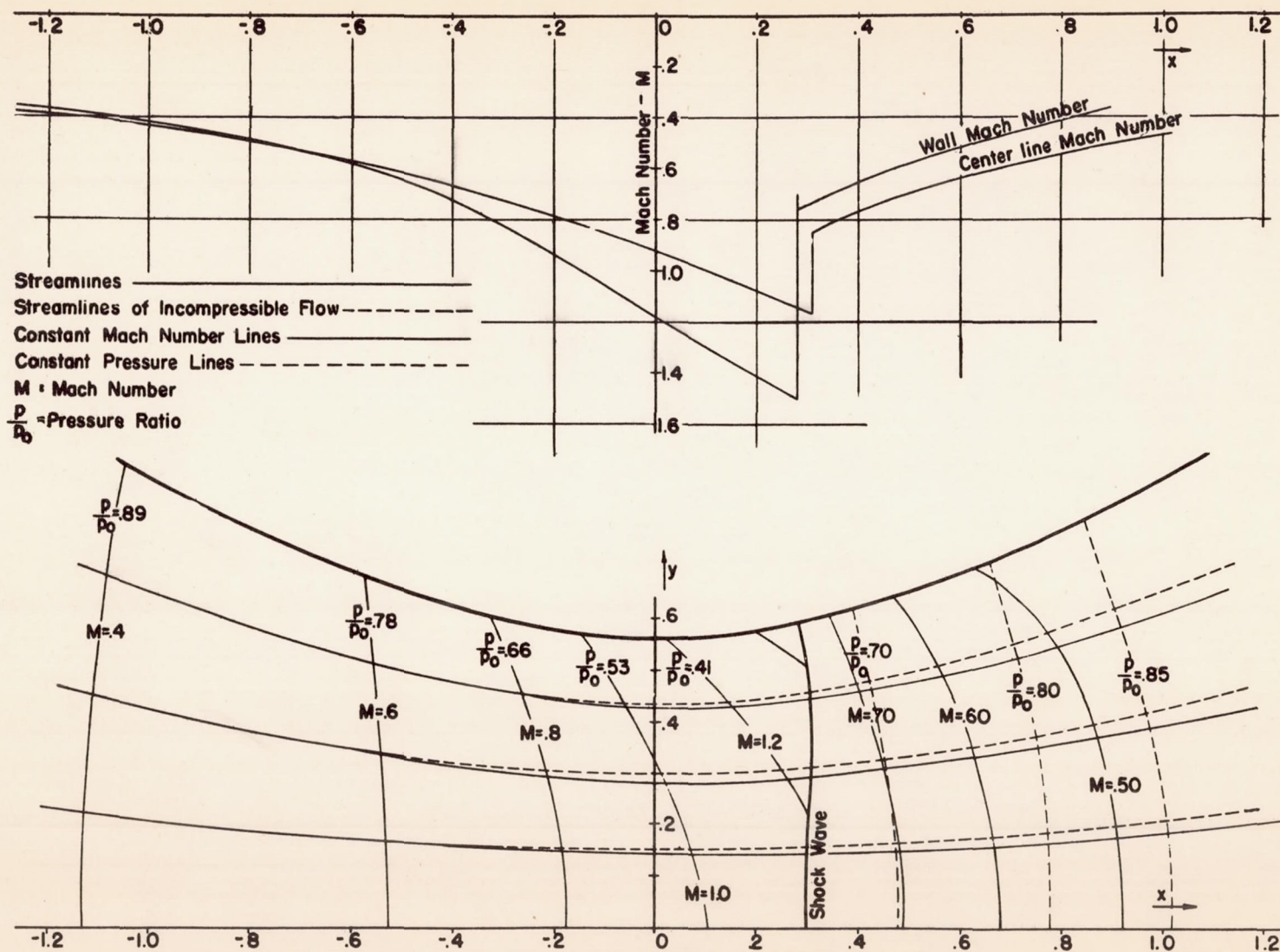
Figure 14.- Flow of compressible fluid in hyperbolic channel.
