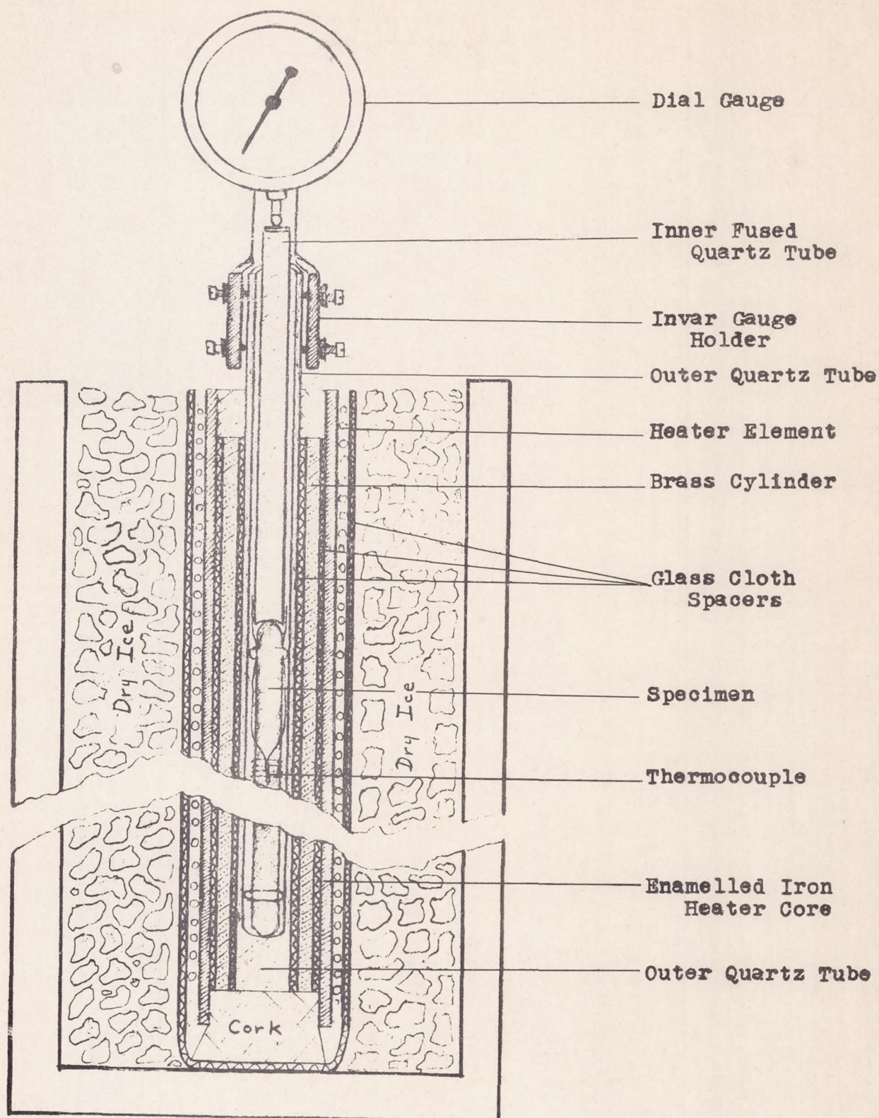
Figure 1. Thermal Expansion Apparatus
