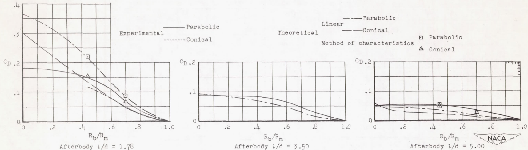
Figure 6.- Comparison of experimental and theoretical afterbody pressure drags at M = 1.2 .
