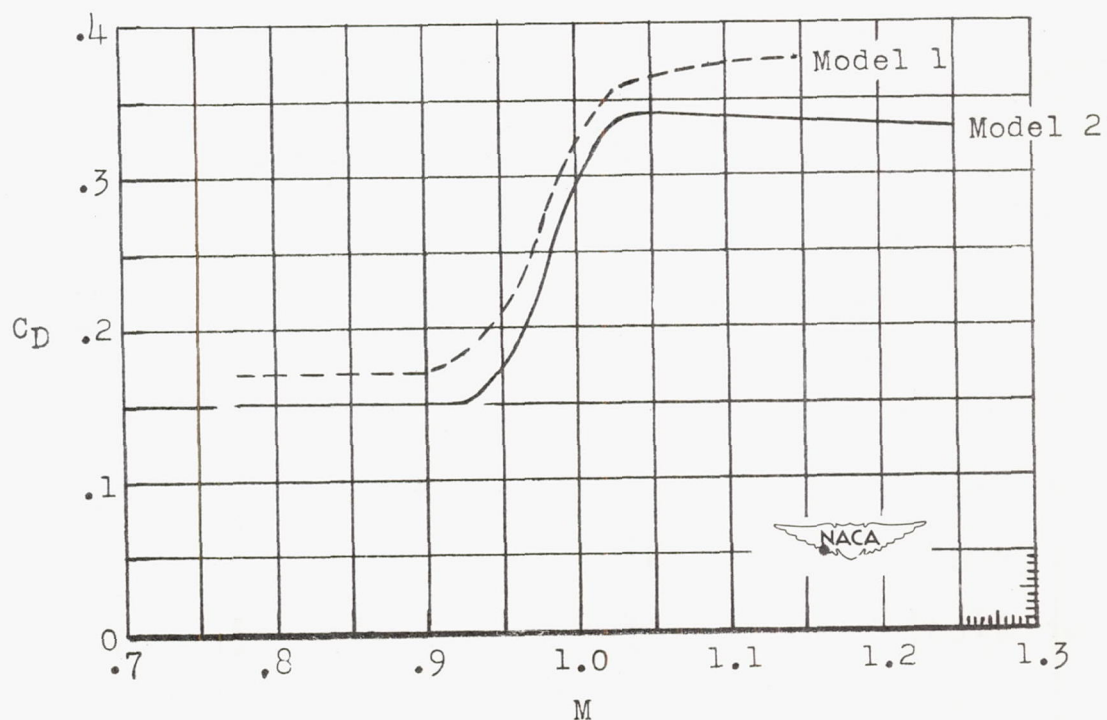
Figure 13.- Drag coefficients of fin-interference test models.
