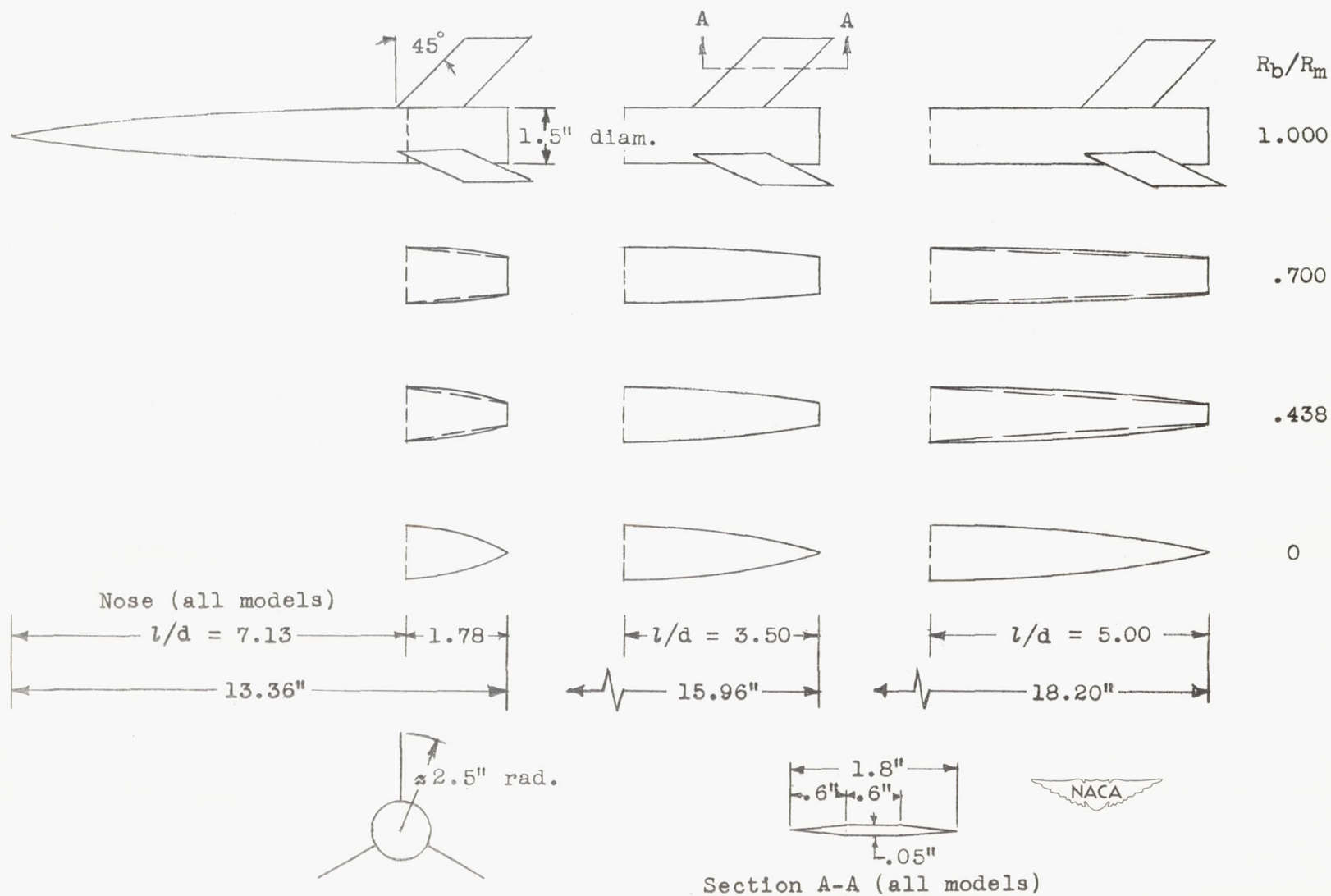
Figure 1.- Test configurations.
