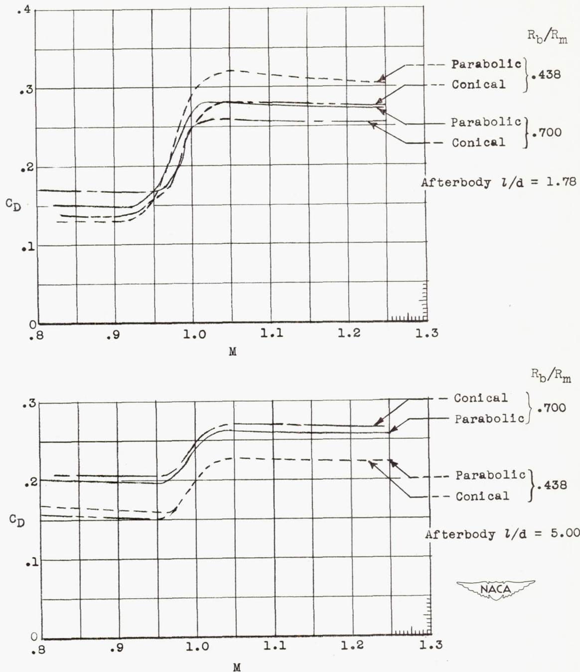
Figure 4.- Comparison of total drag coefficients of parabolic and conical afterbody models.
