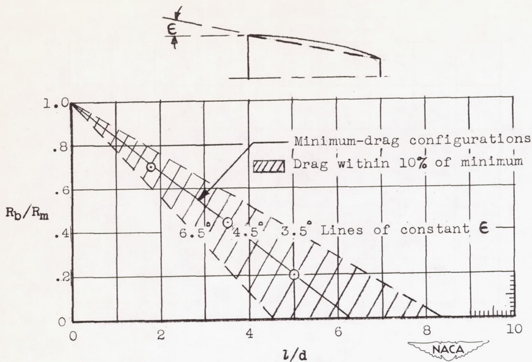
Figure 9.- Minimum-drag configurations at M = 1.2 .
