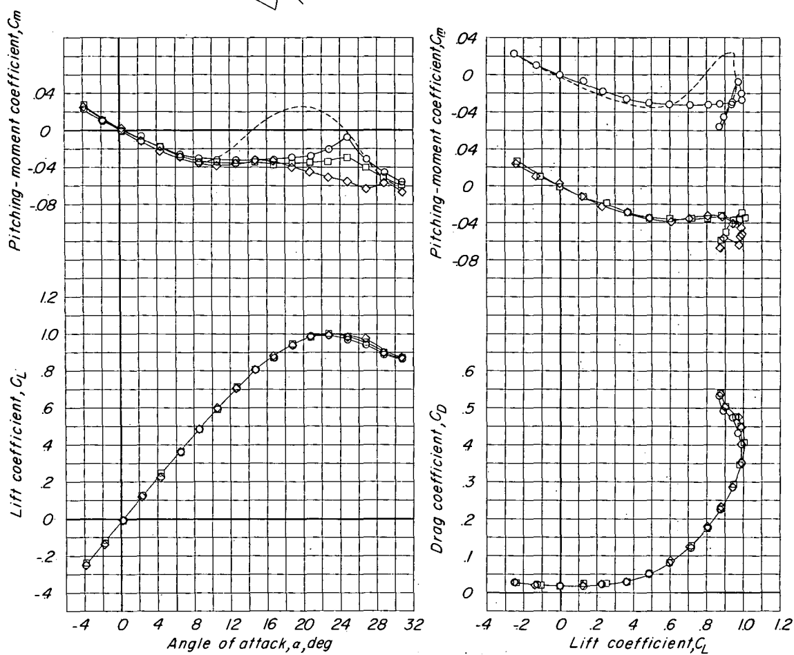
Figure 8.- Effect of notching inboard end of tapered partial-span chord-extension.
