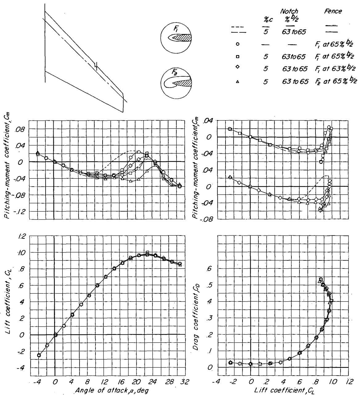
Figure 6.- Notch-fence combinations.
