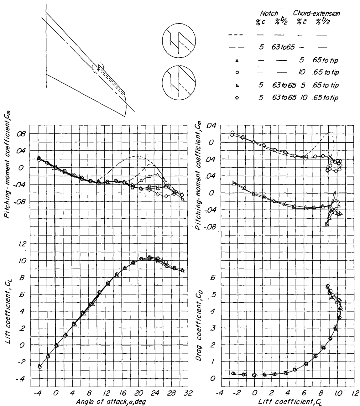
Figure 7.- Notch—chord-extension combinations.
