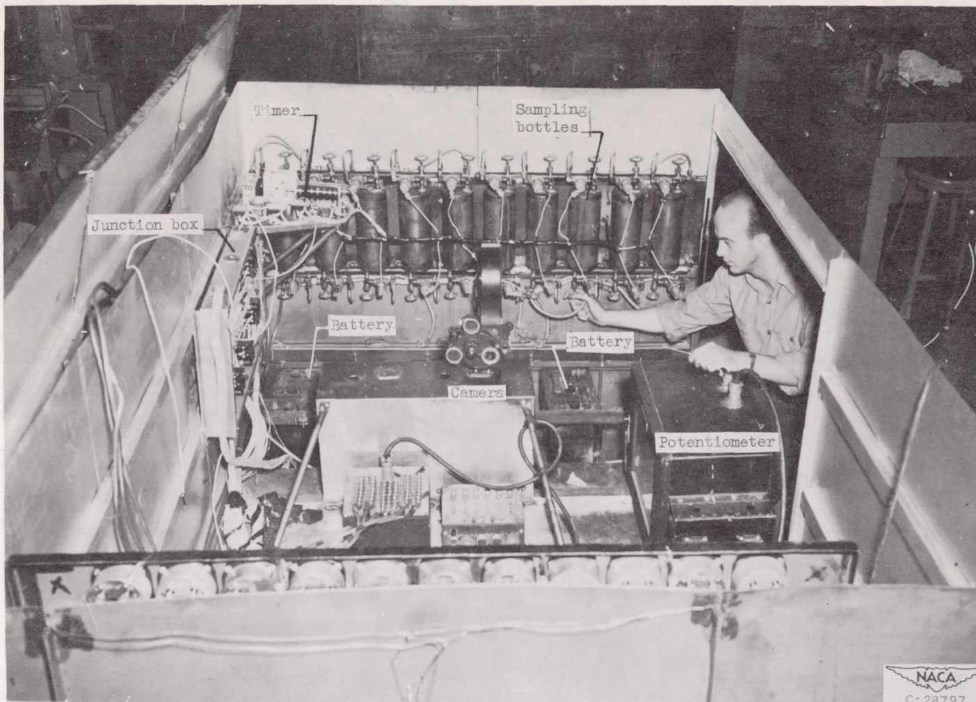
Figure 23. - Installation of cabin-air sampling bottles, camera, junction box, batteries, potentiometer, and timer in fireproof instrument box.
