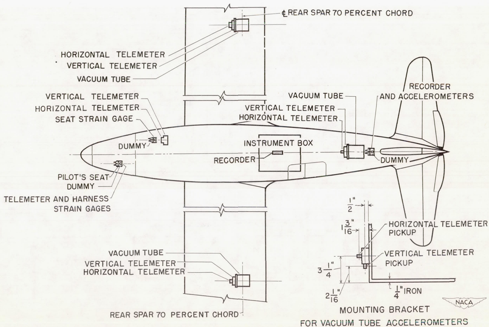
Figure 36. - Recorder, accelerometer-pickup, and strain-gage locations in C-46 airplane.
