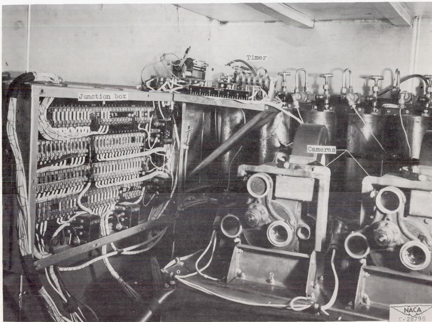
Figure 24. - Closeup view of installation of cameras, junction box, and timer in fireproof instrument box.
