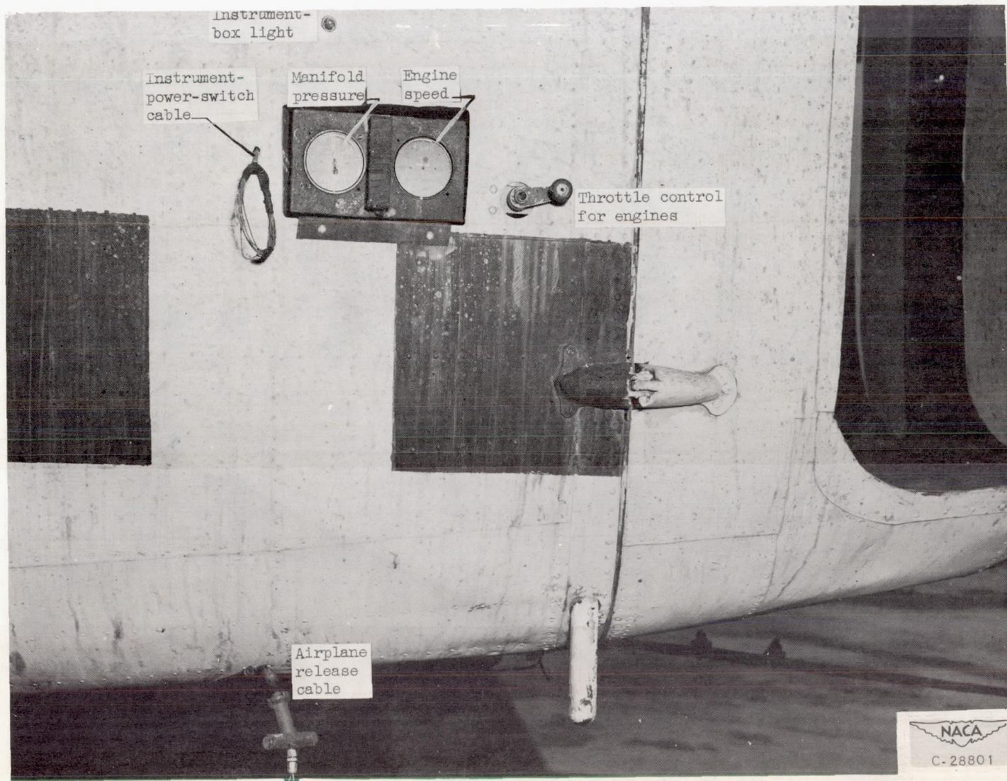
Figure 16. - Controls for operating engines, instrument box power, and airplane release located at rear of fuselage in C-82 airplane.
