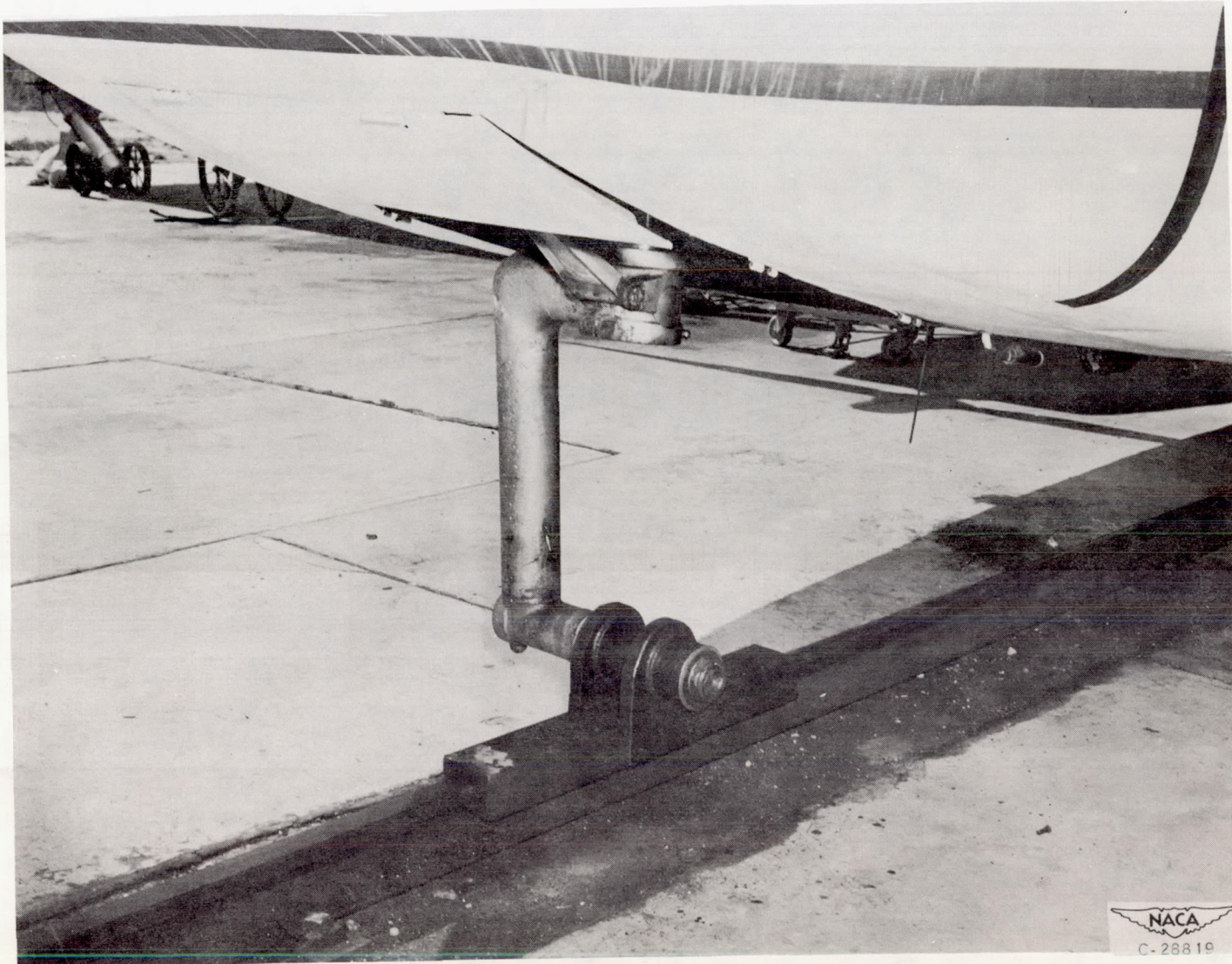
Figure 9. - Guide slipper attached to nose-gear axle of C-82 airplane.
