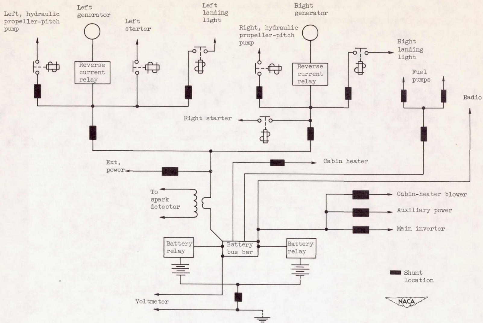
Figure 35. - Shunt locations in electric system of C-46 airplane for third crash.
