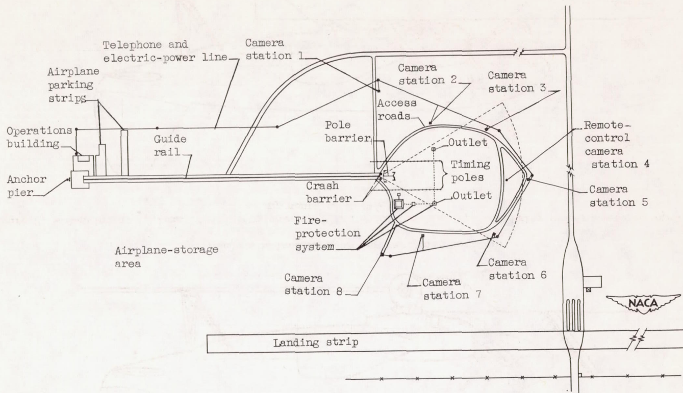
Figure 3. - Plan view of test site for conducting full-scale crash-fire investigation.
