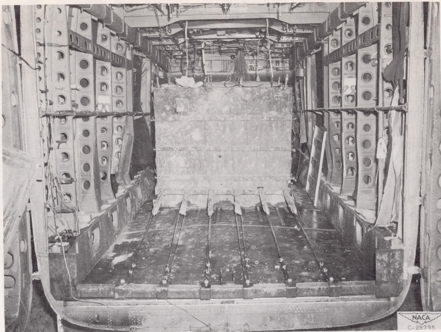
Figure 25. - Rear view of instrument box and shock absorbing system installed in rear of fuselage of a C-82 airplane
