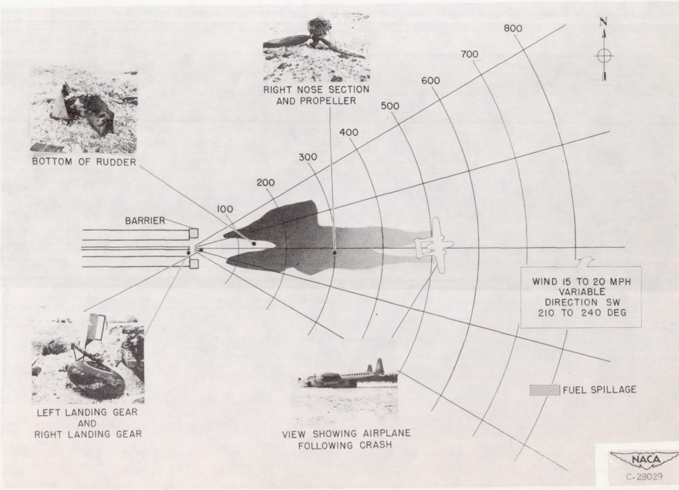
Figure 40. - Distribution of wreckage of C-82 airplane following simulated take-off accident. Test No. Y-4.
