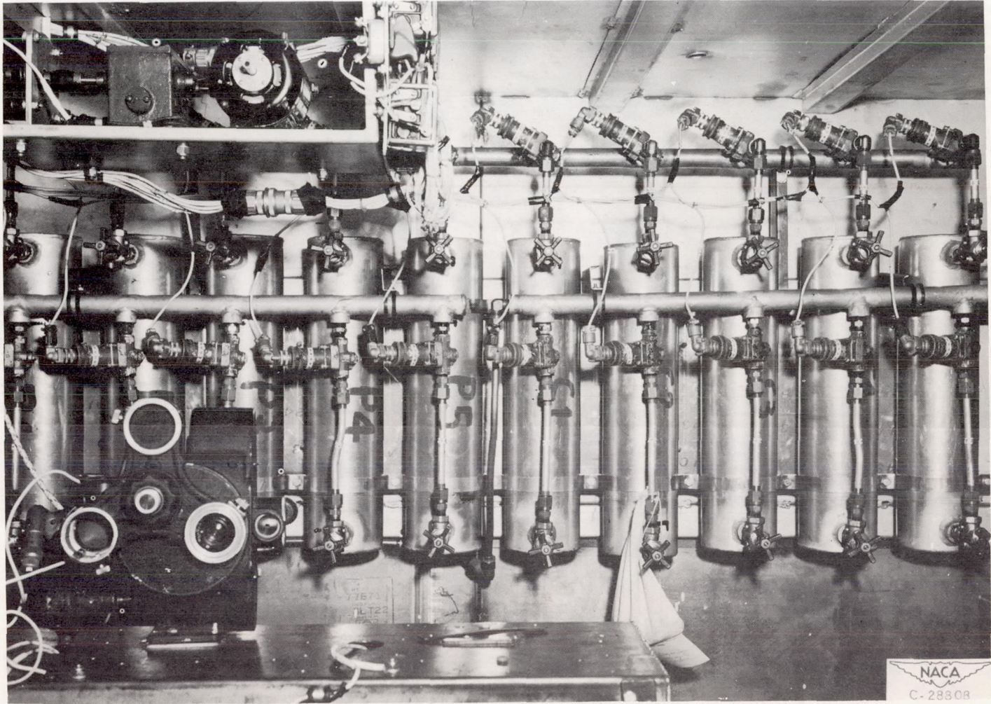
Figure 32. - Cabin-air sampling system installed in fireproof instrument box.
