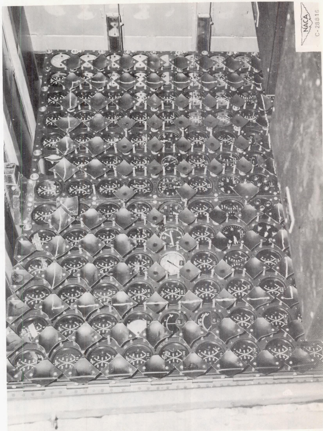
Figure 22. - Instrument panel located at one end of fireproof instrument box.
