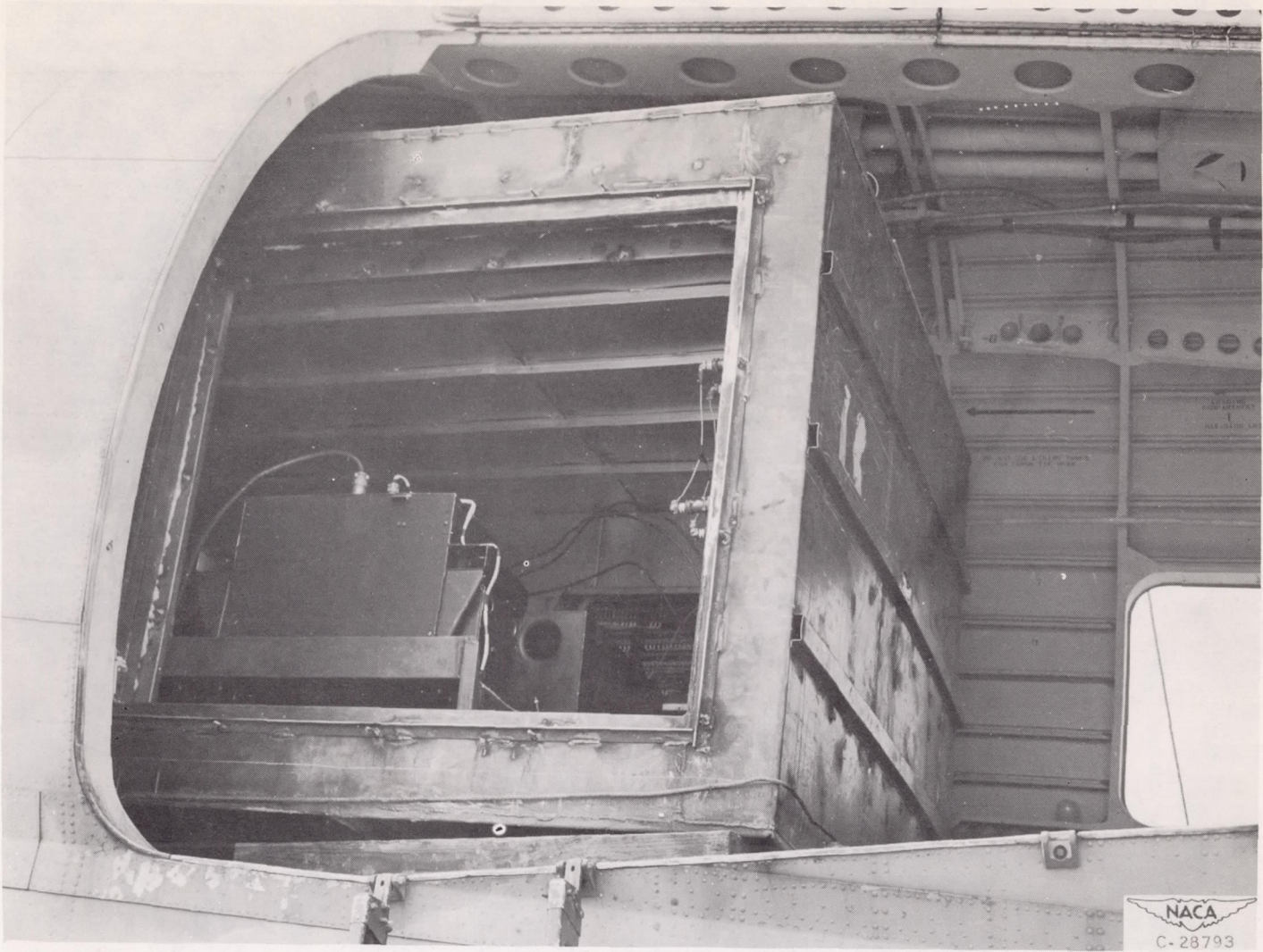
Figure 27. - Fireproof instrument box installation in C-46 airplane; side view.
