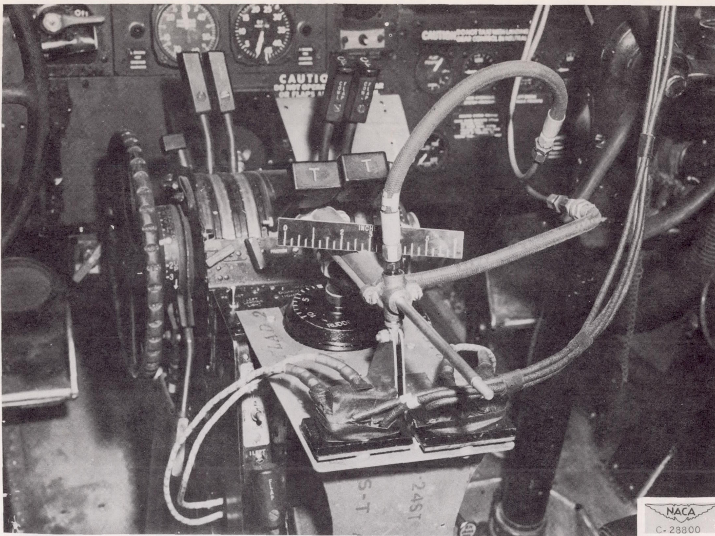
Figure 17. - Remote-control throttle mechanism located in cockpit of C-82 airplane.
