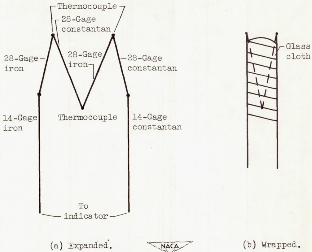
Figure 30. - Construction of thermopiles.
