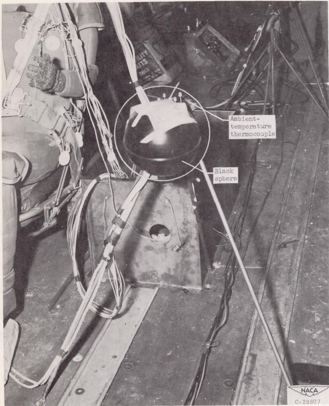
Figure 31. - Installation of radiant and ambient temperature thermocouples in fuselage of C-46 airplane.
