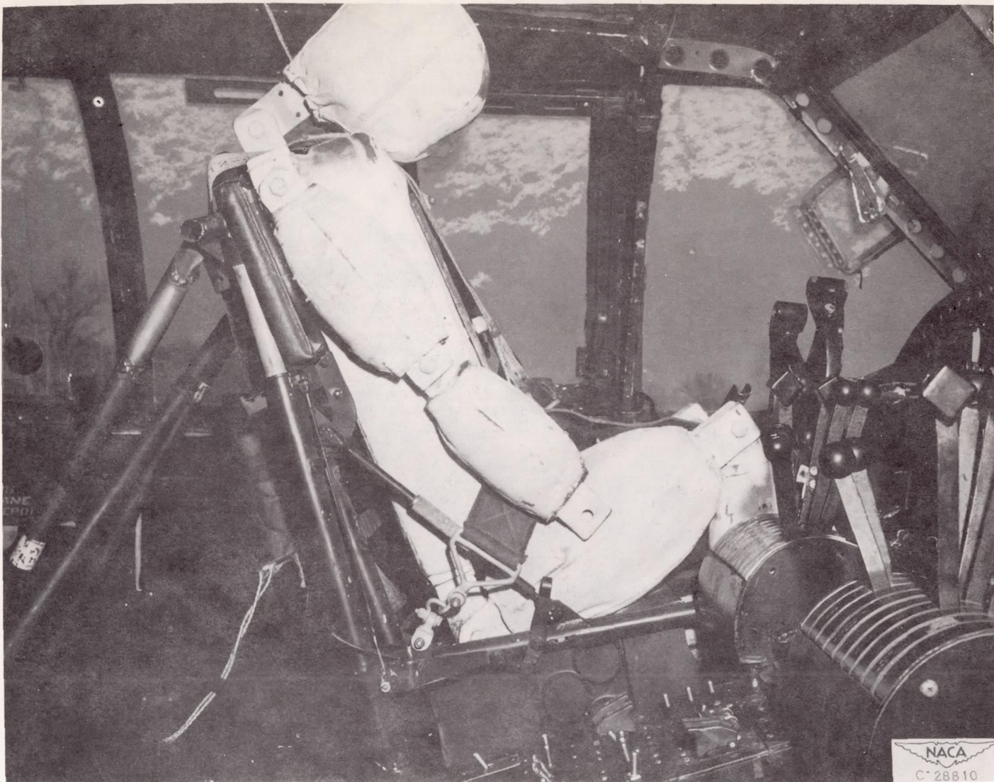
Figure 37. - Typical seat and dummy installation in pilot compartment of C-82 airplane.
