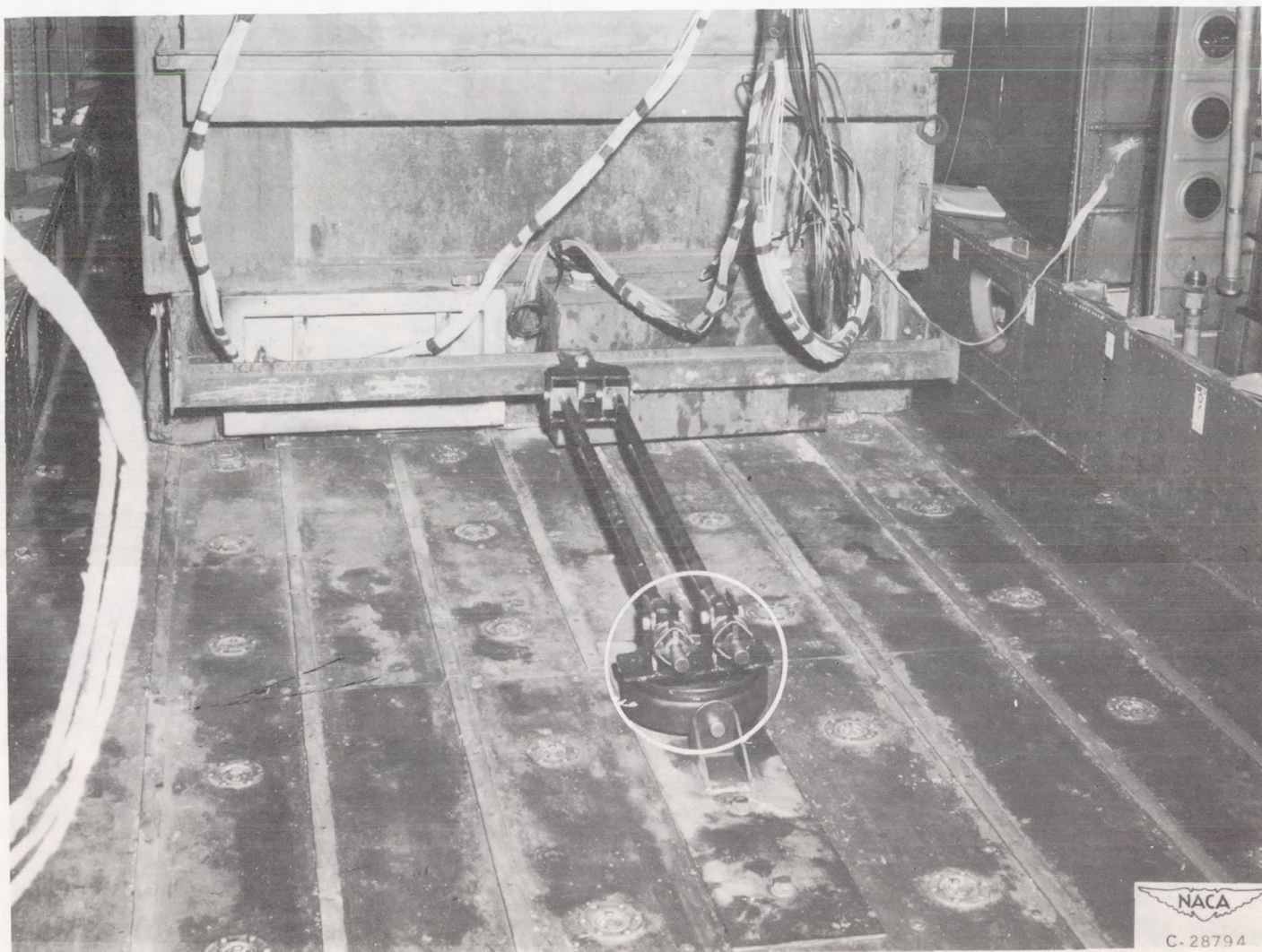
Figure 26. - Installation of restraining mechanism in front of fireproof instrument box in C-82 airplane.
