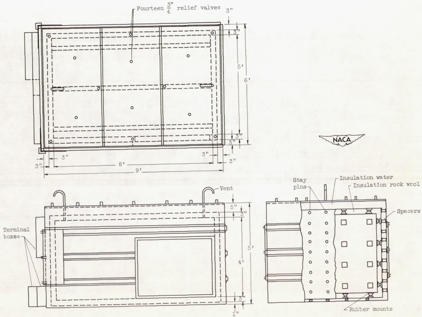
Figure 20. - Sketch showing construction of fireproof instrument box. Material, 1/16-inch black iron; water capacity, 310 gallons; total weight, 6575 pounds.
