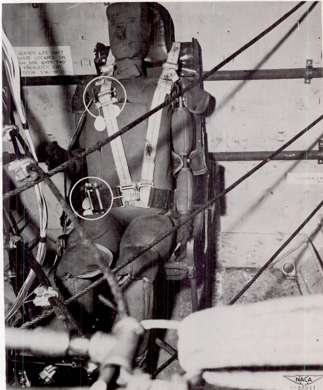
Figure 38. - Strain-gage links installed on shoulder and seat harness of dummy at rear of fuselage in C-46 airplane.
