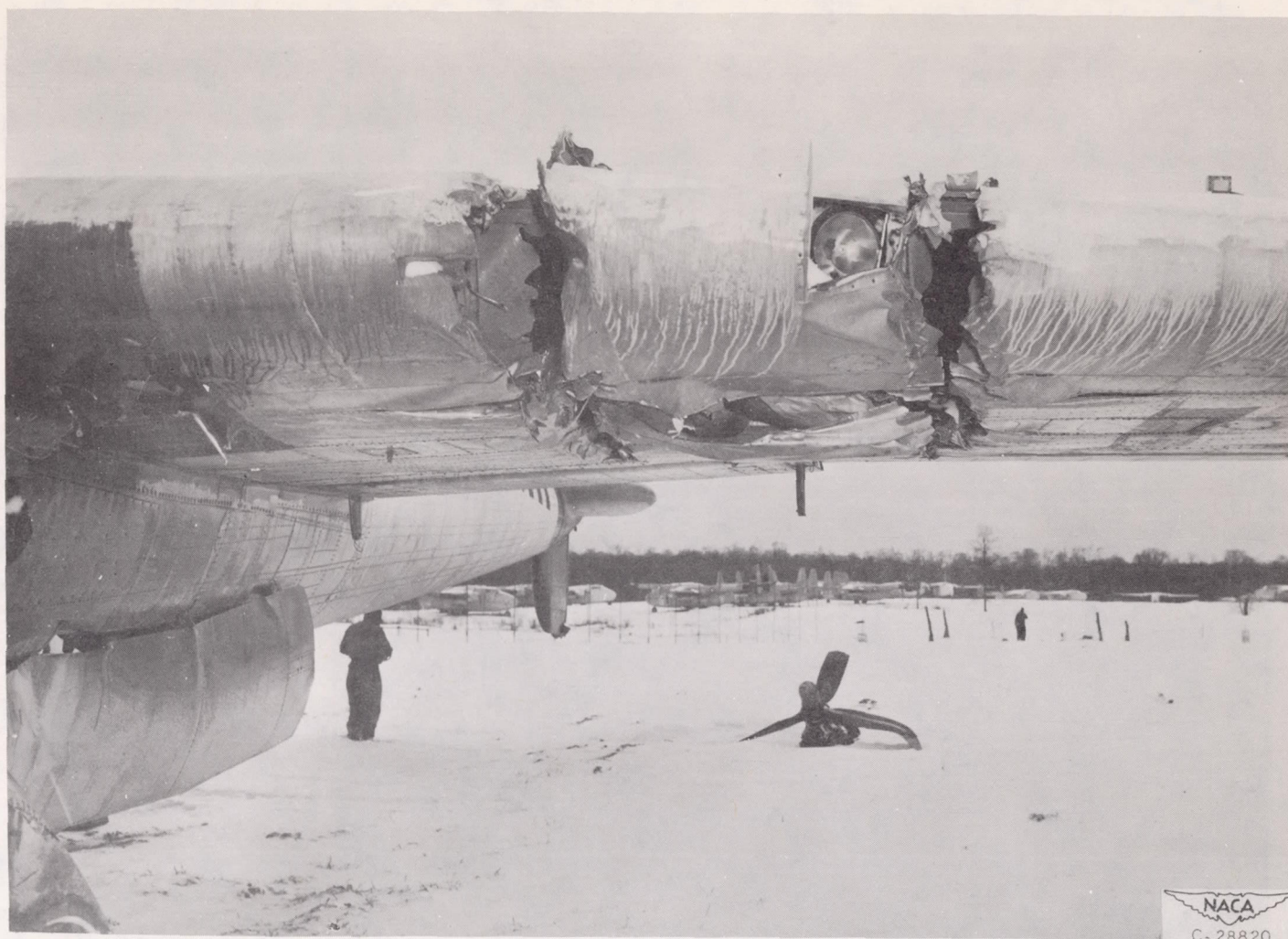
Figure 15. - Damage to left wing and fuel tanks of C-82 airplane produced by pole barriers.
