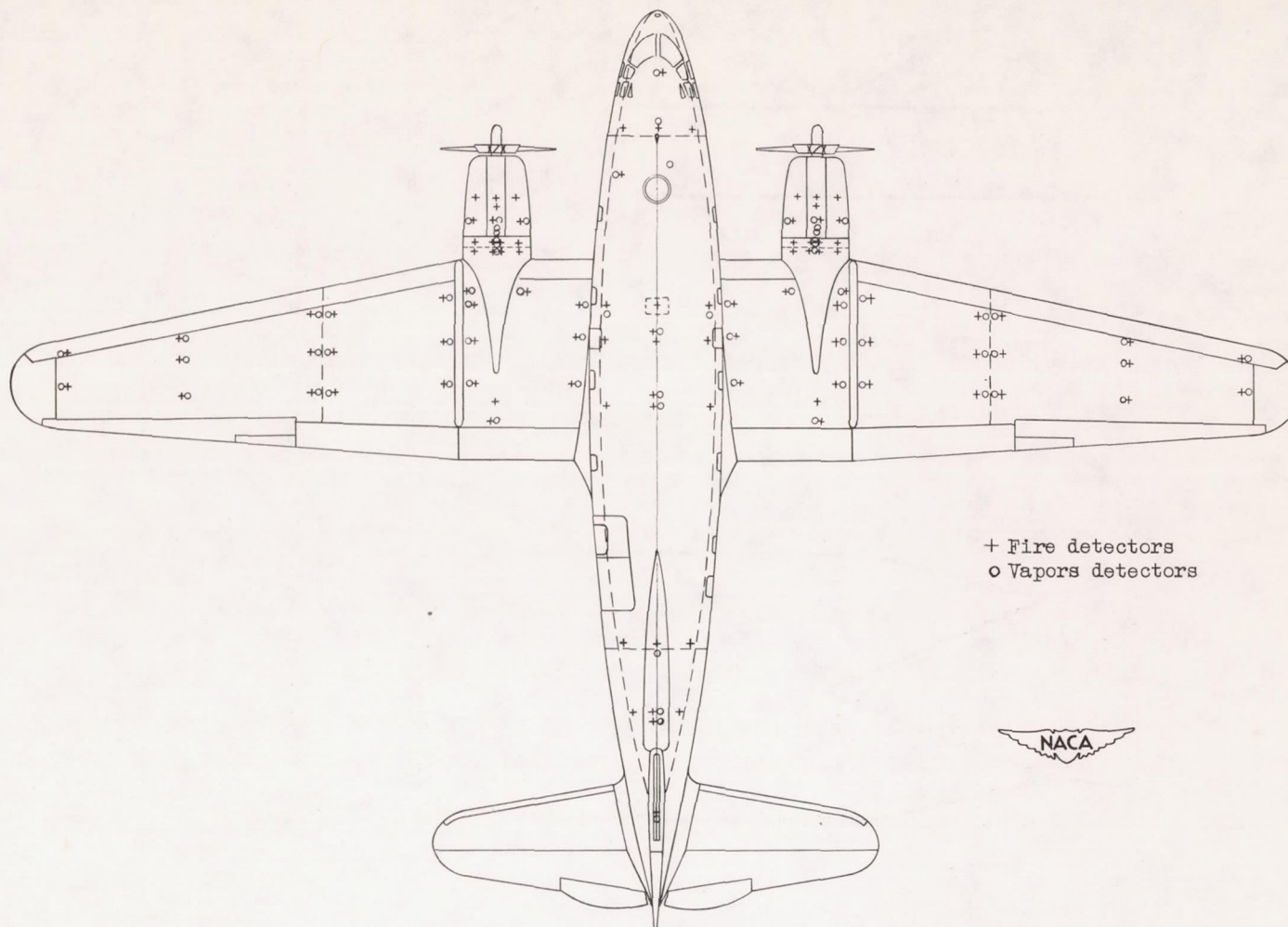
Figure 29. - Location of fire and vapor detectors installed in C-46 airplane.
