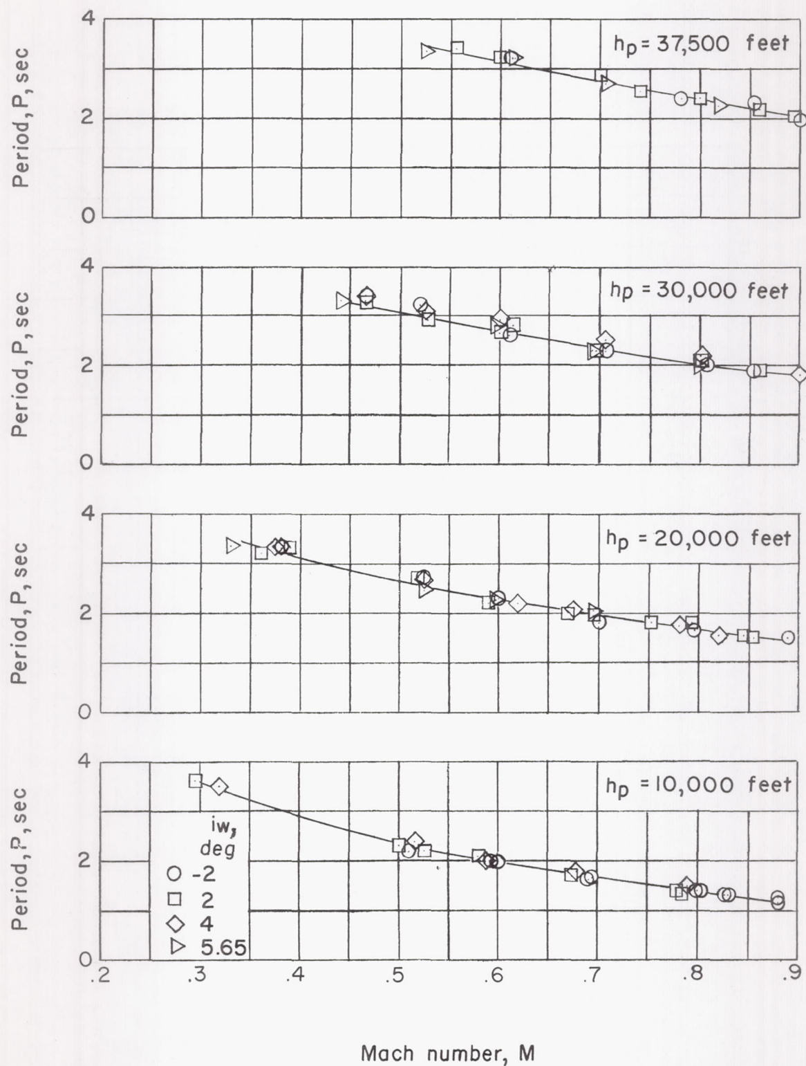
Figure 5.- Variation of period of the lateral oscillation with Mach number.
