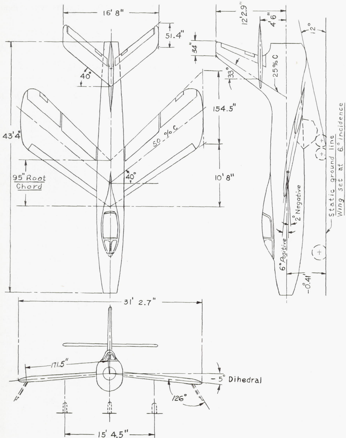
Figure 1.- Three-view drawing of the Republic XF-91 airplane.
