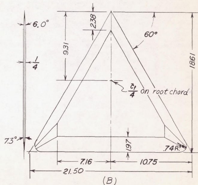
(c) Details of horizontal tails and tail locations tested.
