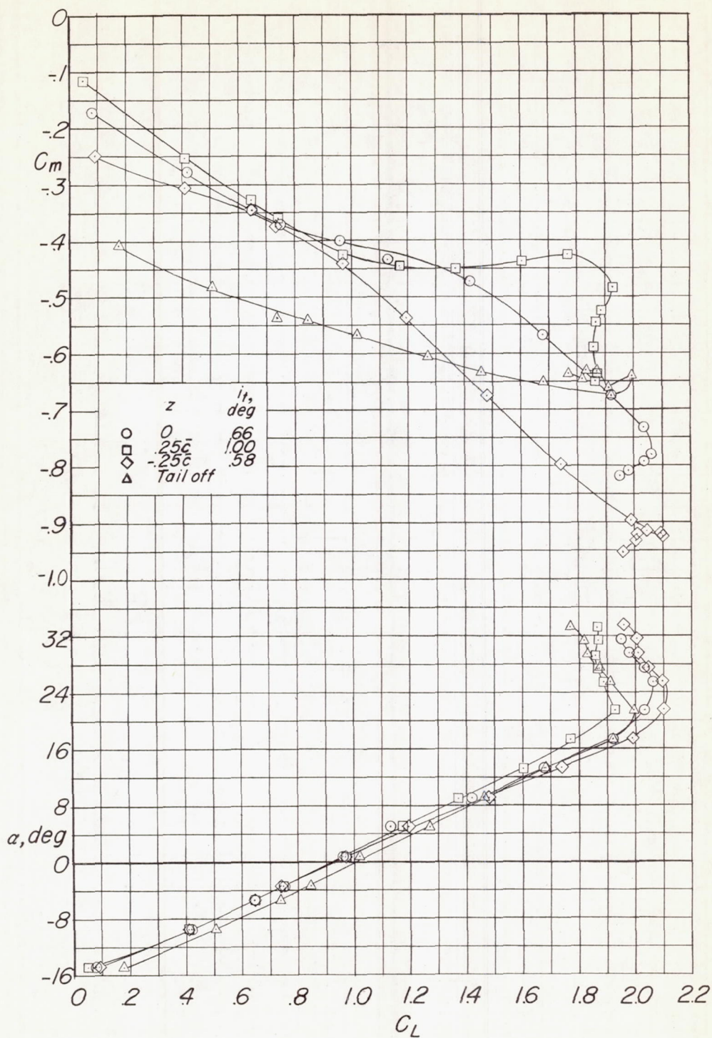
Figure 7.- Effect of location of the delta horizontal tail on the longitudinal aerodynamic characteristics in pitch of the delta-wing-fuselage model with extended double slotted flaps deflected 56.2^\circ . \lambda = 2.0\bar{c} .
