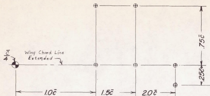
Tail Locations Tested (Taper Ratio 0.394 Tail)
