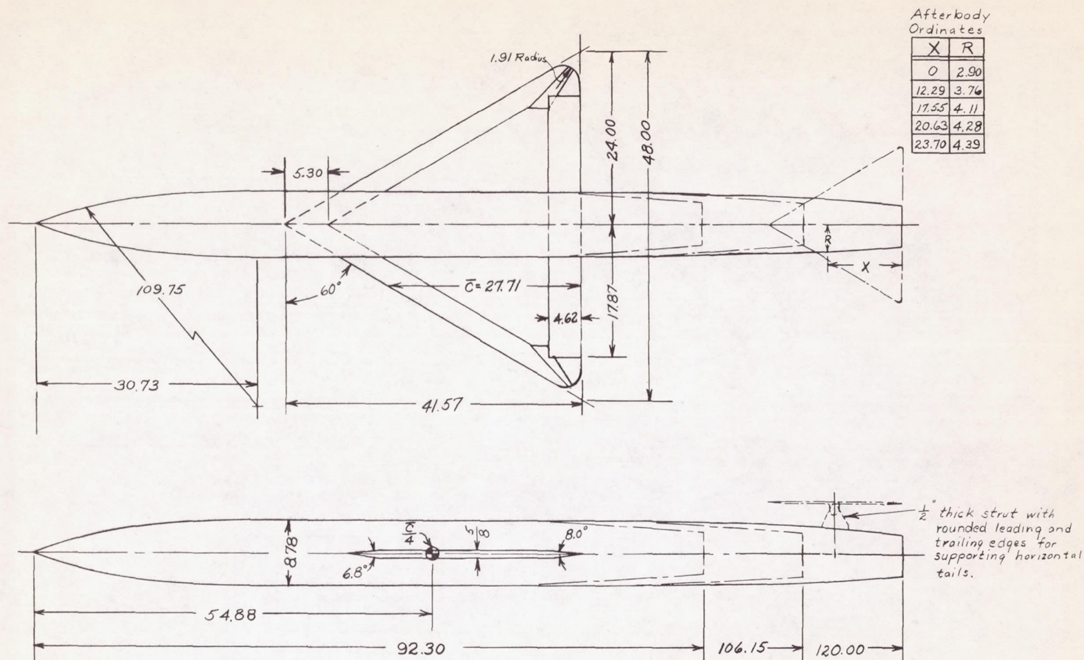
(a) Details of fuselage and wing.
