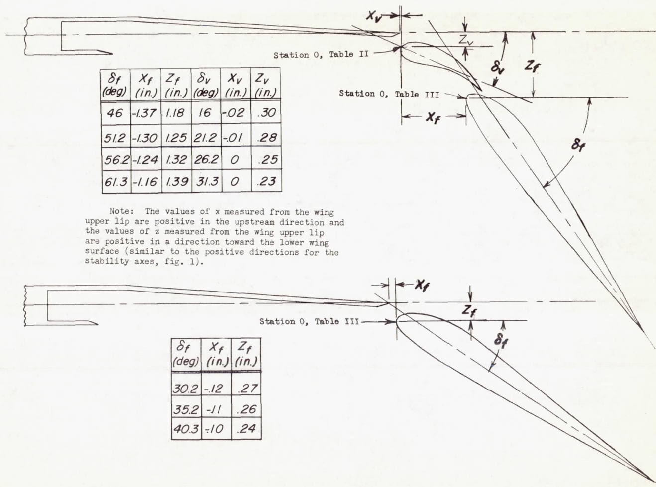
(b) Details of flaps.
