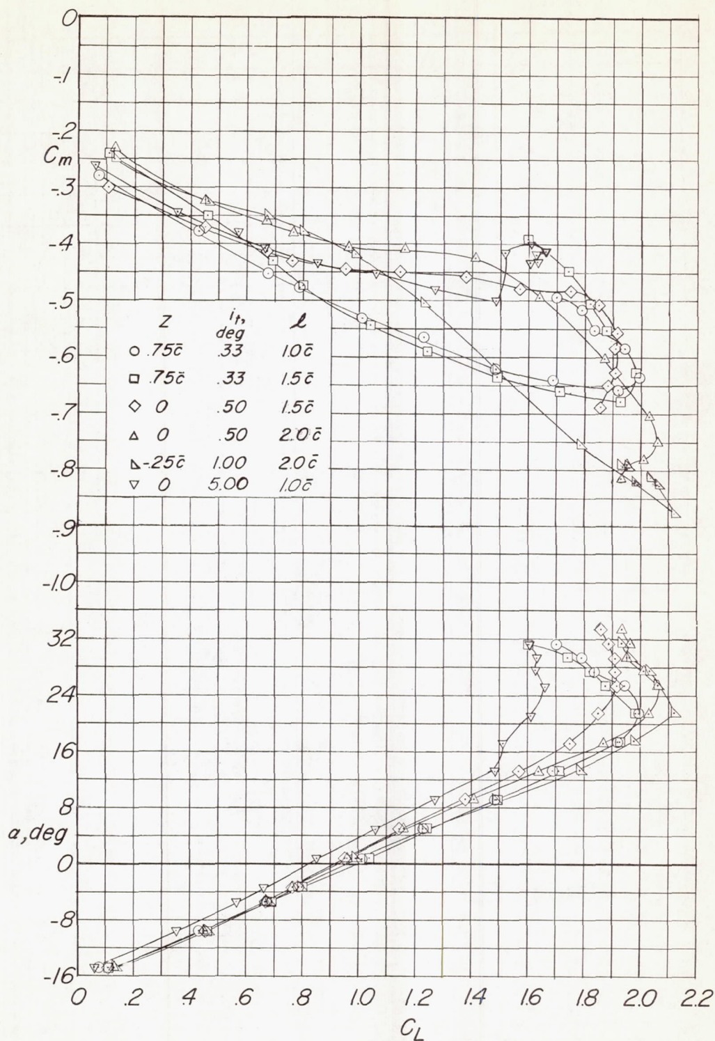
Figure 9.- Effect of location of the tail with a taper ratio of 0.394 on the longitudinal aerodynamic characteristics in pitch of the delta-wing-fuselage model with extended double slotted flaps at 56.2^\circ .
