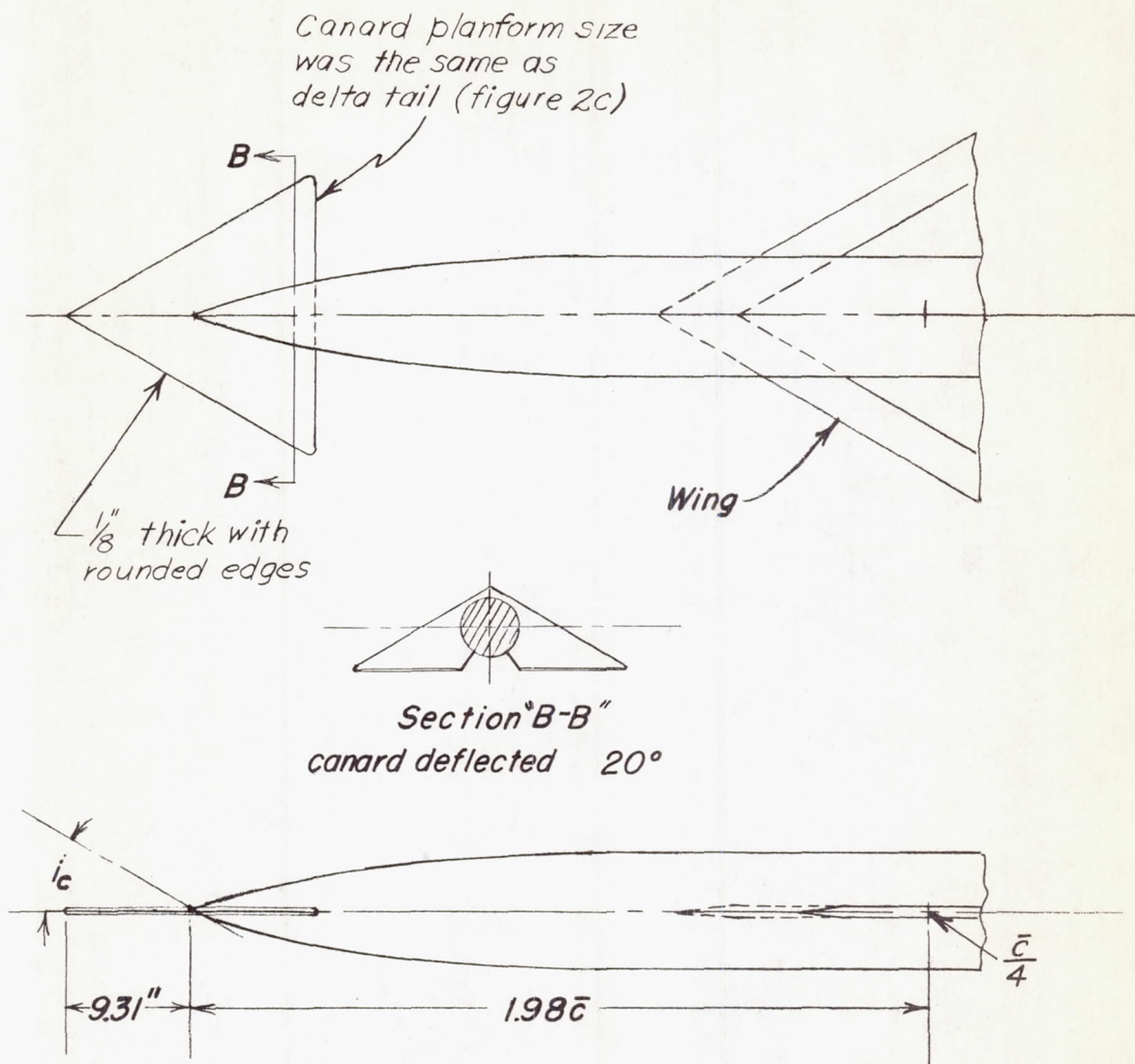
Figure 3.- Canard details.
