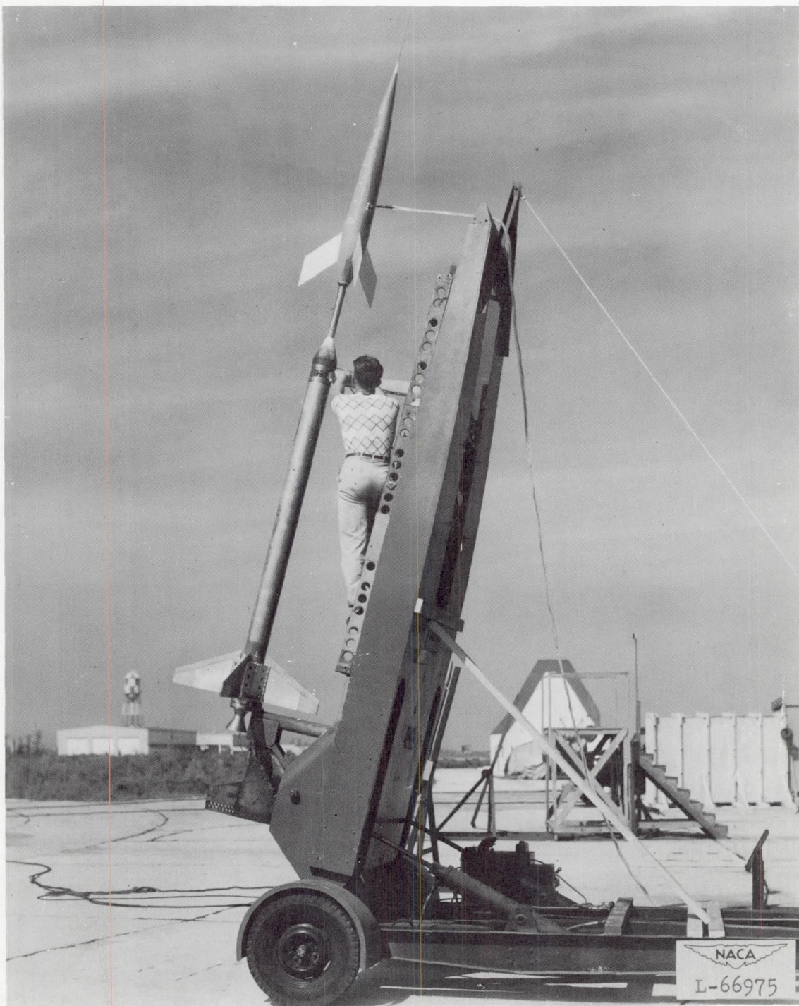
(a) Model and booster on zero length launcher.
