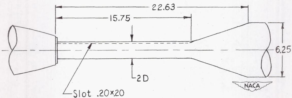
(b) Sting between model and booster.
