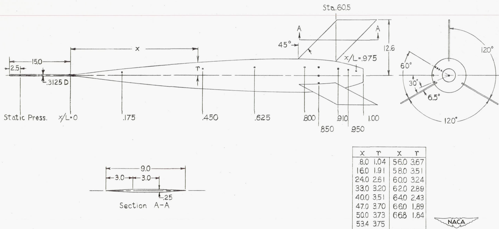
(a) Location of pressure orifices.
