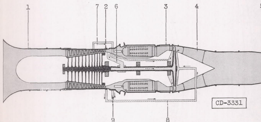
(b) Turbojet engine with axial-flow compressor.
