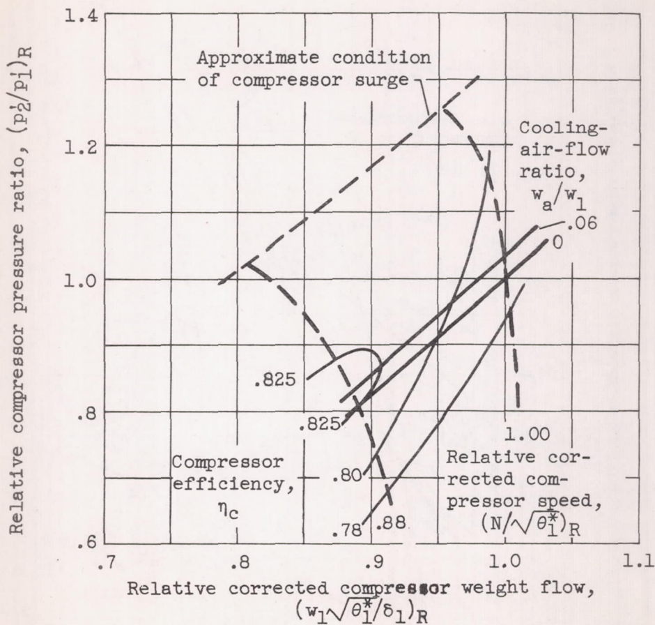
(a) Compressor map.
