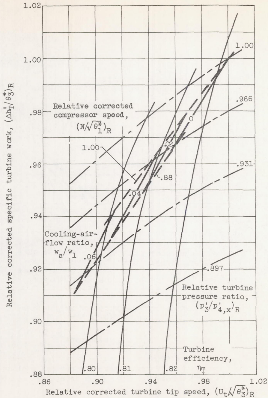
(b) Turbine map.
