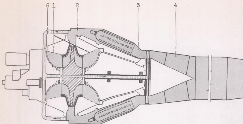
(a) Turbojet engine with centrifugal compressor.
