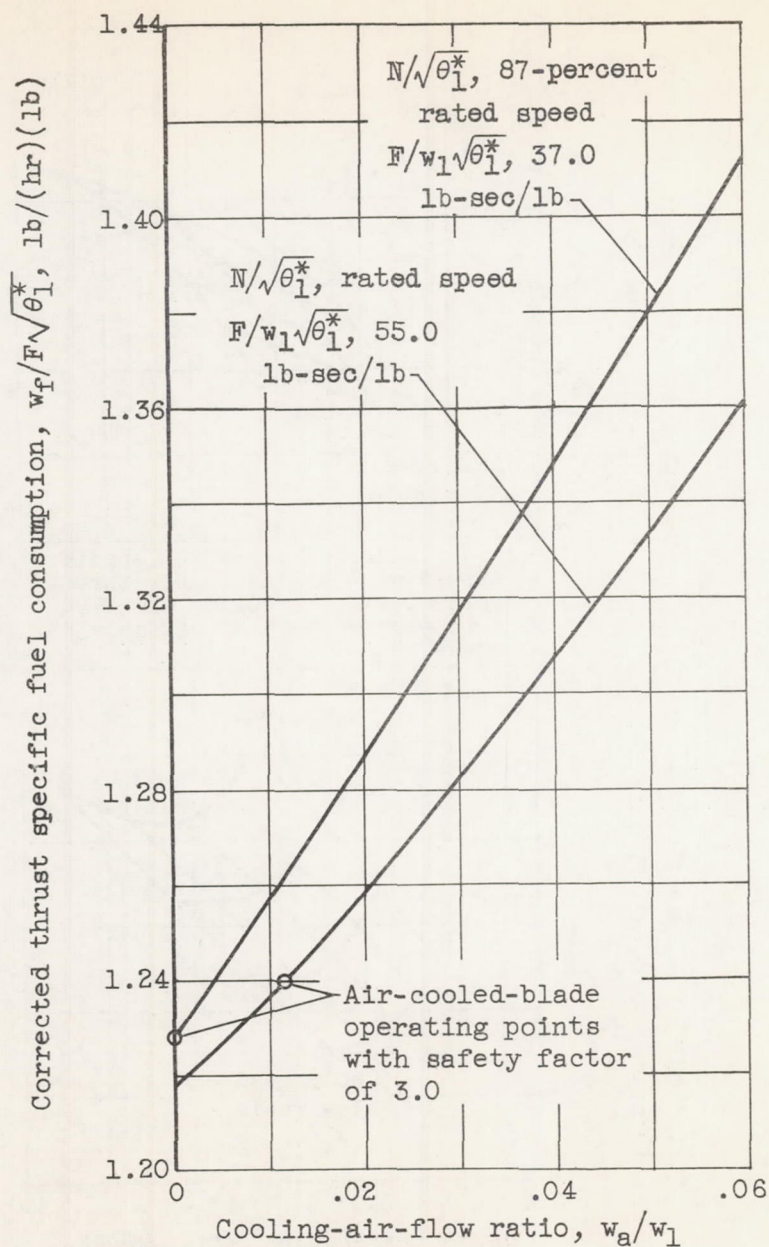
Figure 12. - Variation of thrust specific fuel consumption with cooling-air-flow ratio for constant values of corrected specific thrust at two corrected engine speeds. Centrifugal-flow compressor.
