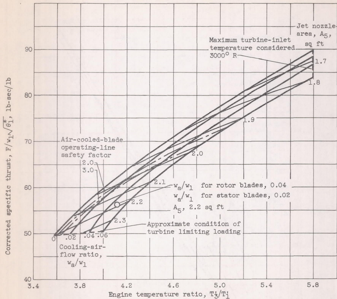
(a) Variation of corrected specific thrust with engine temperature ratio for four cooling-air-flow ratios over range of jet nozzle areas.
