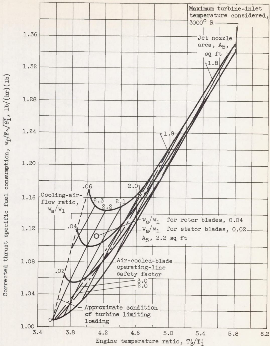
(b) Variation of corrected thrust specific fuel consumption with engine temperature ratio for four cooling-air-flow ratios over range of jet nozzle areas.
