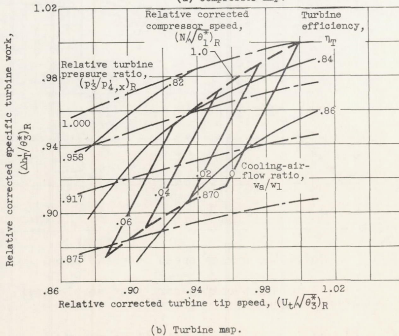
Figure 6. - Centrifugal-flow-engine operating lines on relative performance maps for several cooling-air-flow ratios. Jet nozzle area, 1.80 square feet.
