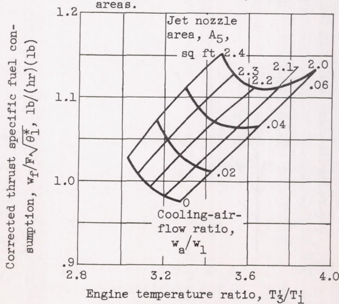
(b) Variation of corrected thrust specific fuel consumption with engine temperature ratio for four cooling-air-flow ratios over range of jet nozzle areas.
