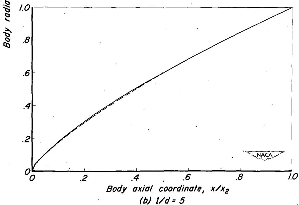
Figure 8. - Comparison of profiles of minimum drag bodies of revolution for given lengths and base diameters with the approximate profiles employed in the present tests.
