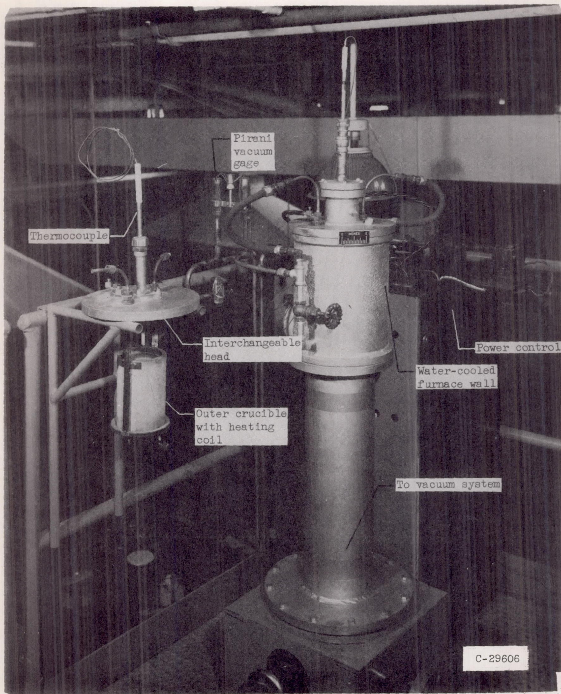
Figure 4. - Vacuum furnace and automatic control. Extra furnace head at left.
