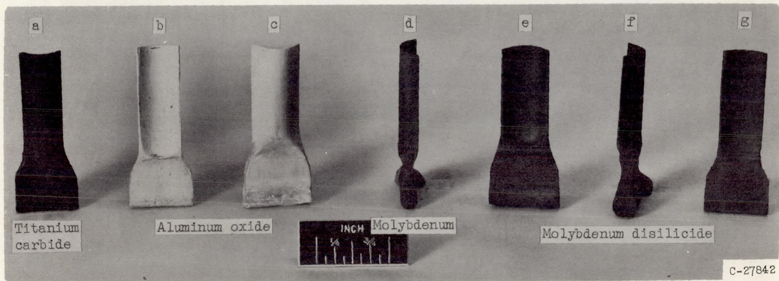
Figure 3. - Freeze-cast turbosupercharger blades as cast.
