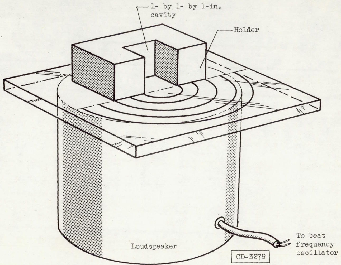
Figure 5. - Plate and cavity arrangement used for measuring the effect of vibratory frequency on speed of flow of thick slips.
