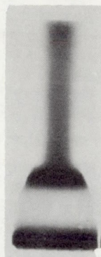
Figure 7. - Radiograph of molybdenum disilicide sintered blade.
