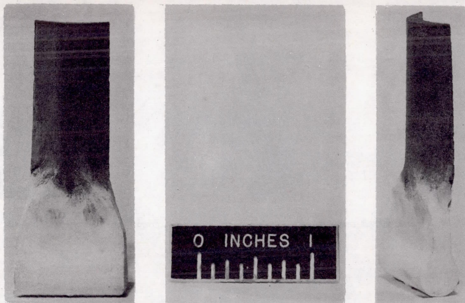
Figure 6. - Composite freeze-cast turbosupercharger blade in as-cast condition. Titanium carbide blade, alumina root.
