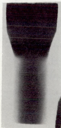
(a) Radiograph of blade after presintering for 2 hours at 2300° F.
