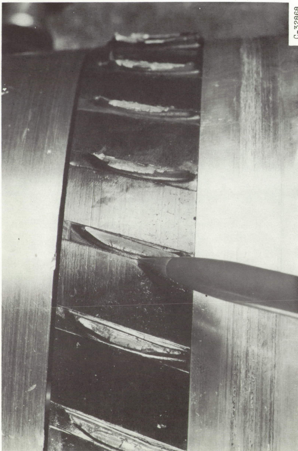
(b) Blade having fatigue failure over 95 percent of cross section.
