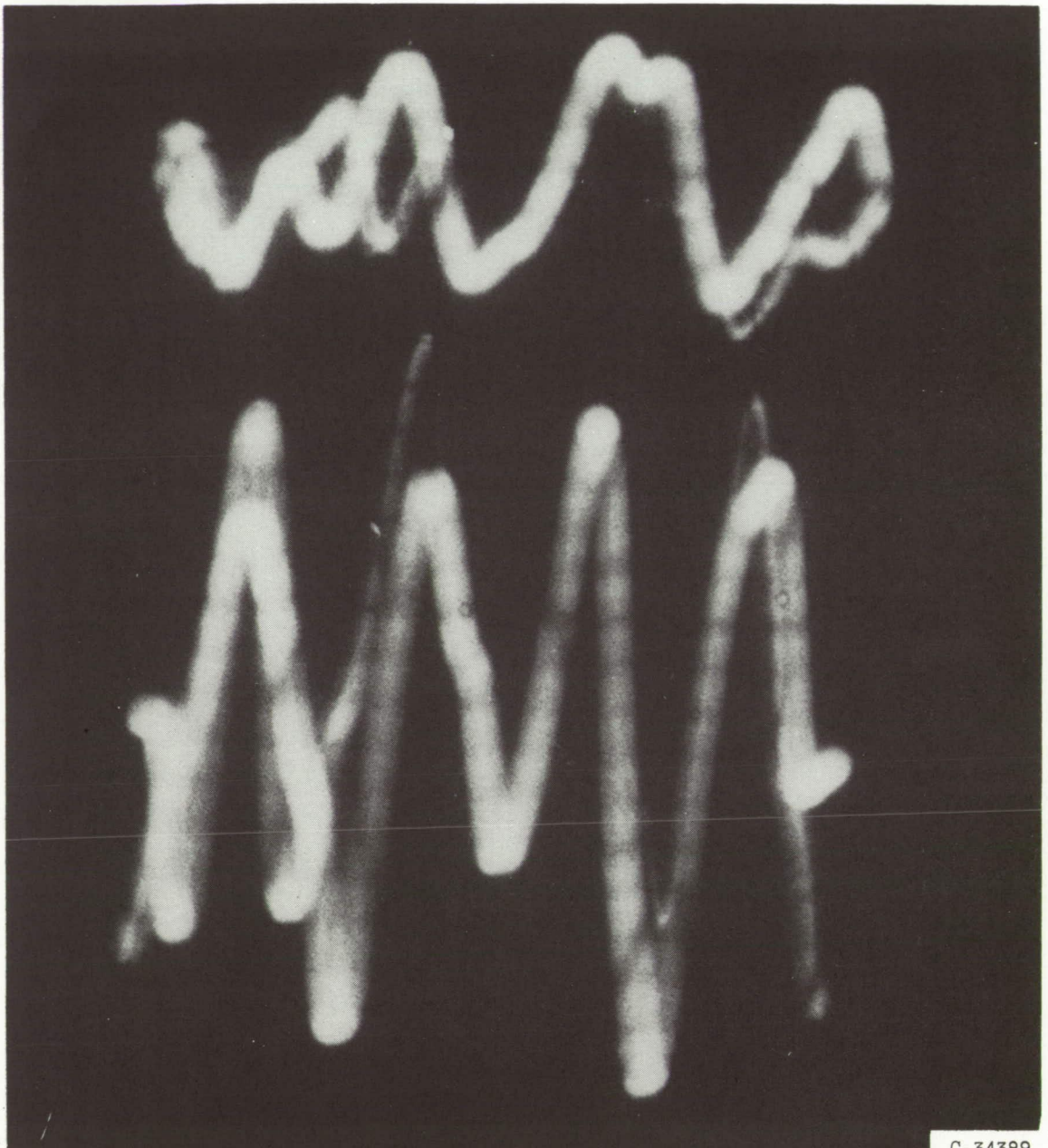
Figure 3. - Typical stall patterns observed on cathode-ray oscilloscope.
