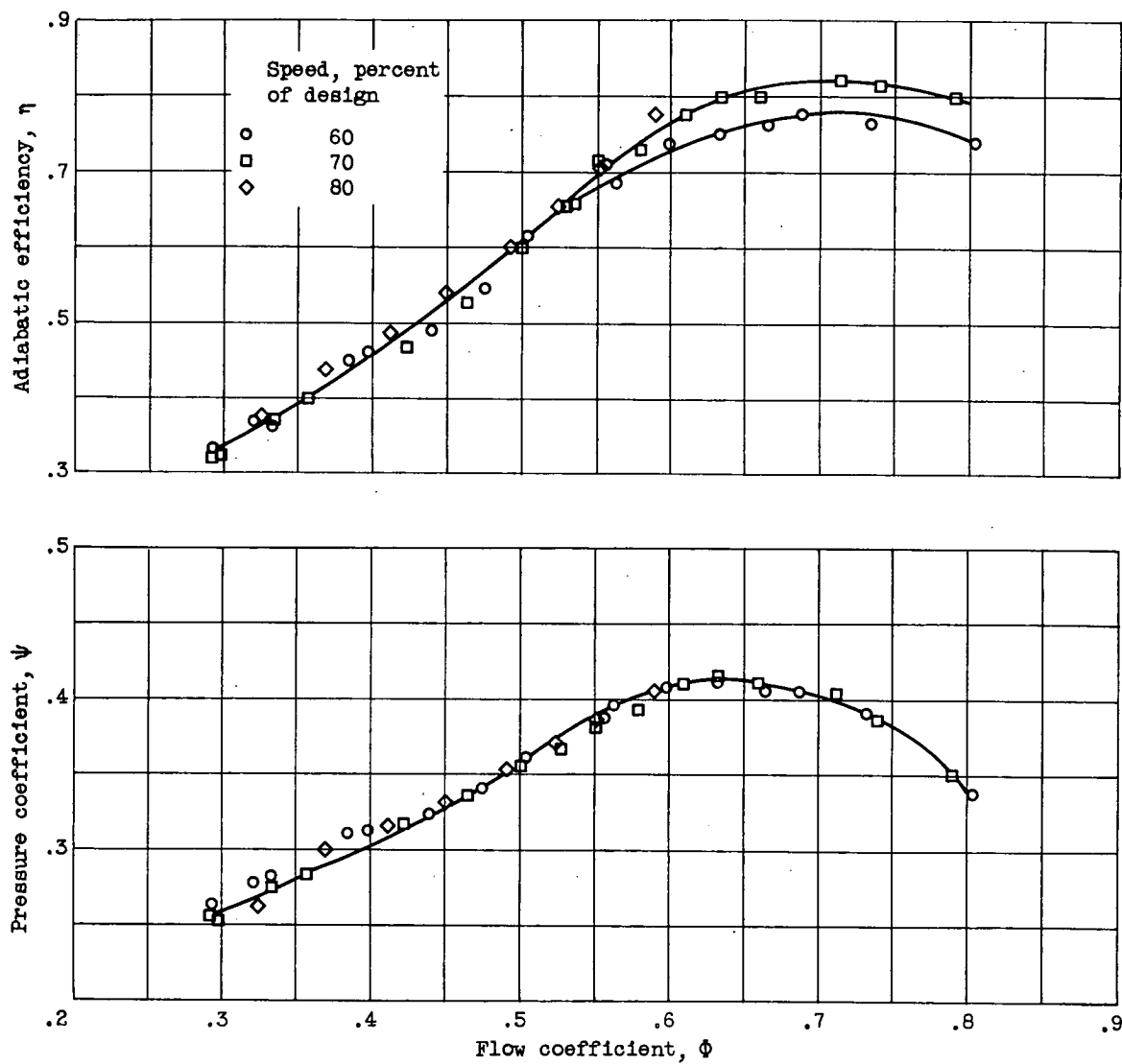
Figure 1. - Performance map of single-stage compressor.
