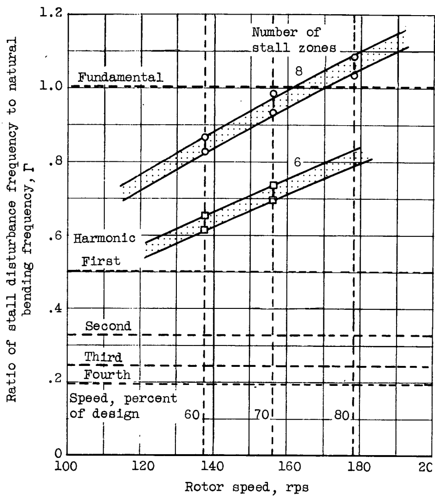
Figure 5. - Dimensionless blade excitation parameter as a function of compressor speed.
