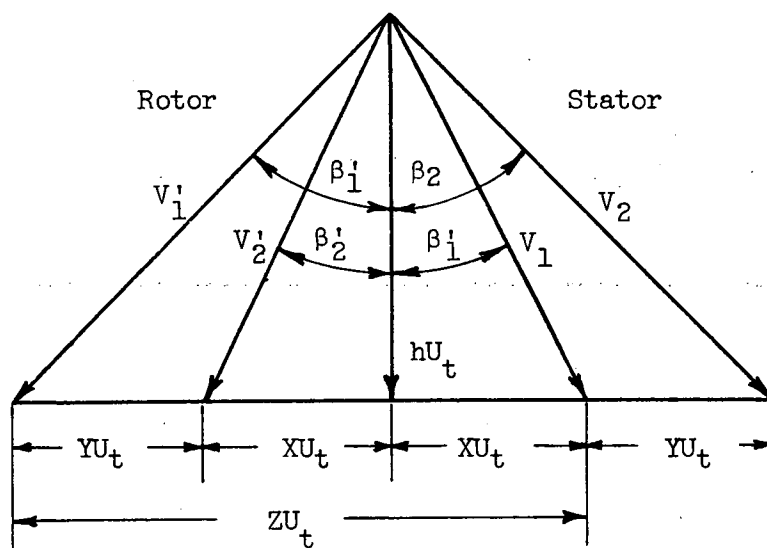
Symmetrical axial-velocity diagram
