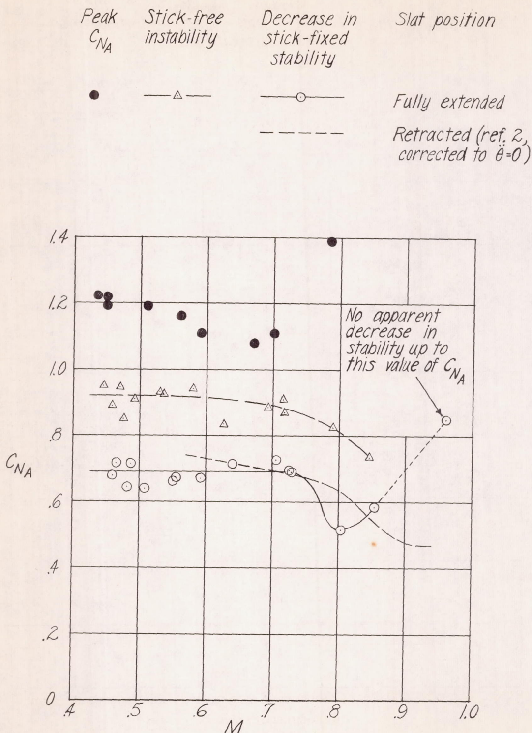
Figure 19.- Normal-force coefficient for decay in longitudinal stability as a function of Mach number for the airplane with inboard fences on the wing.
