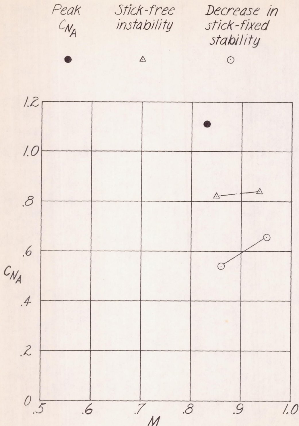
Figure 21.- Normal-force coefficient for decay in longitudinal stability as a function of Mach number for the airplane with half-extended slats and inboard wing fences removed.
