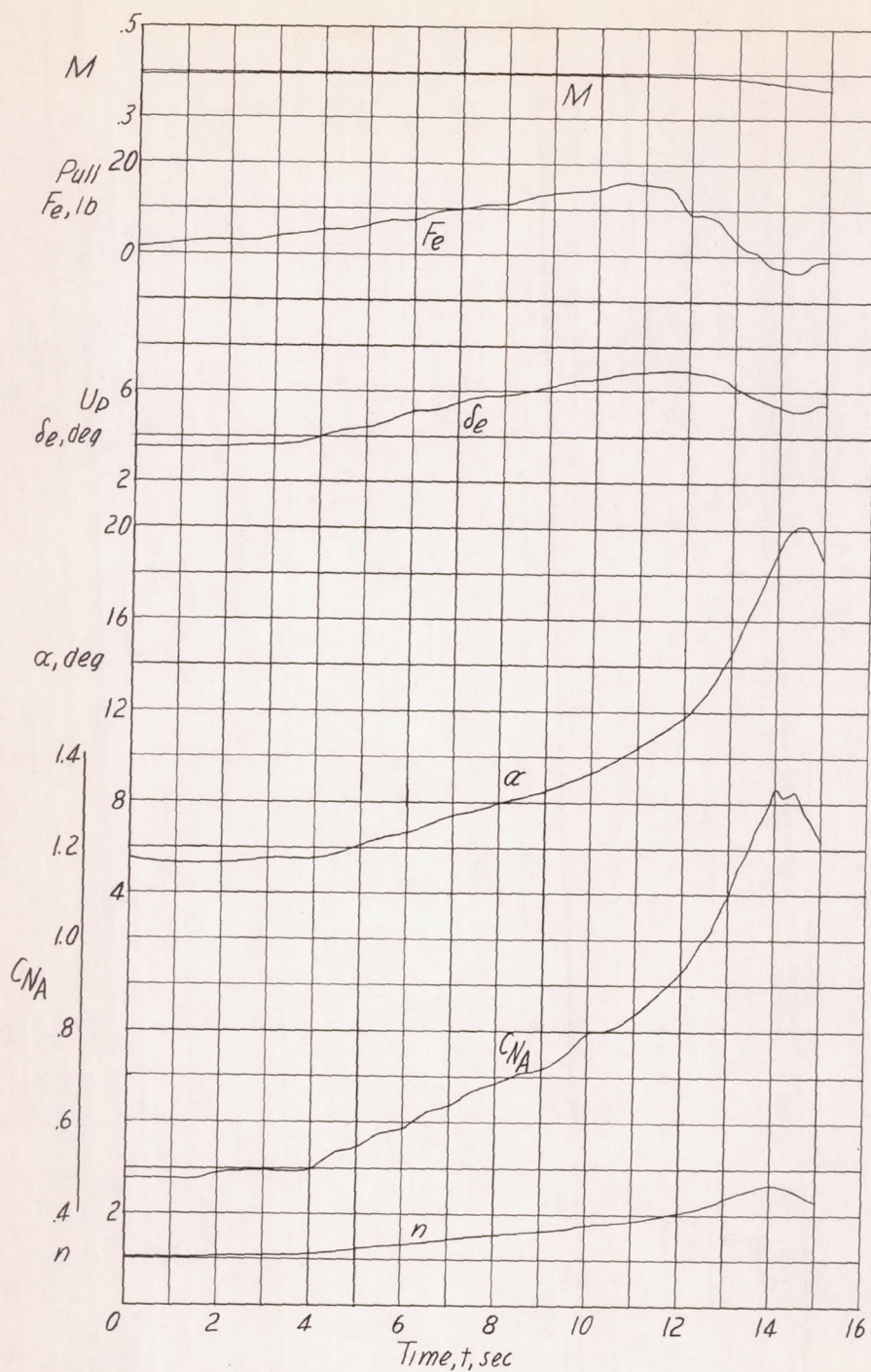
(a) h_p \approx 12,700 feet; i_t = 1.5^\circ ; center of gravity at 26.6 percent mean aerodynamic chord.
