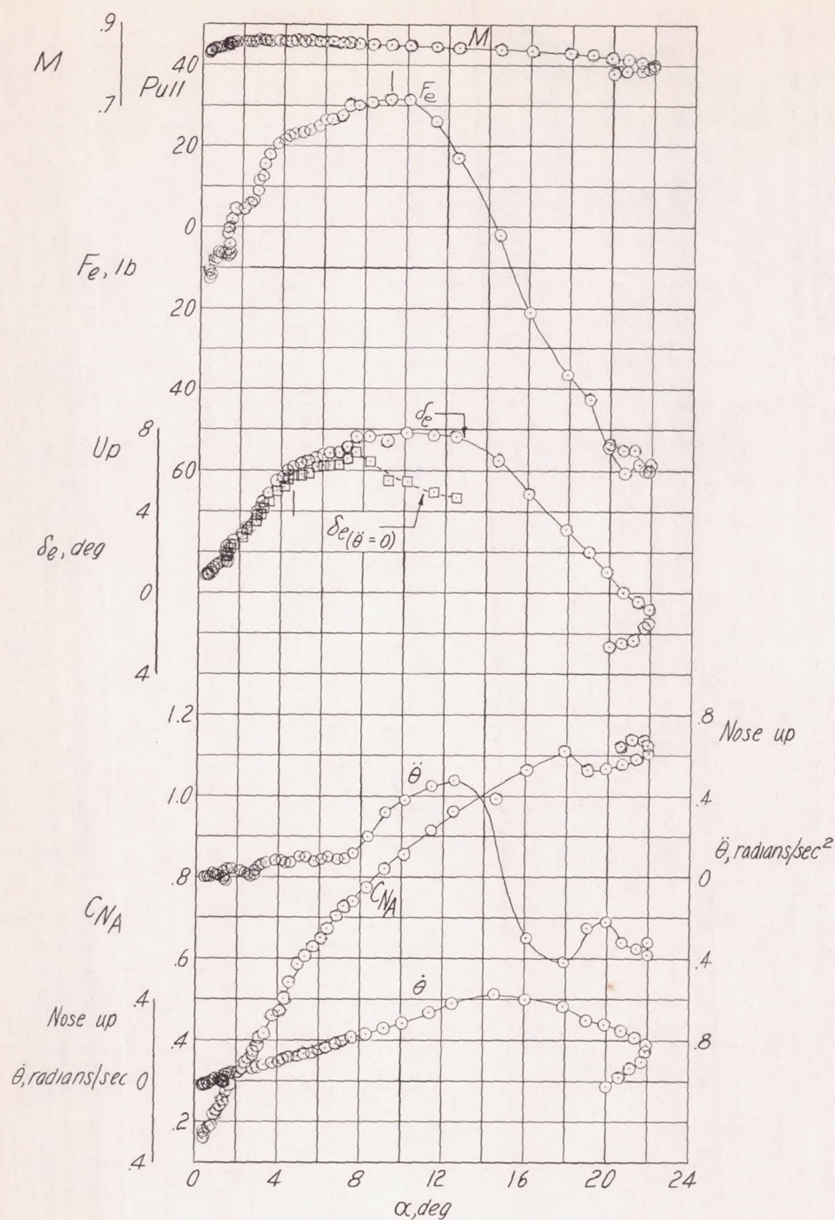
(a) h_p \approx 29,000 feet; i_t = 1.6^\circ ; center of gravity at 28.6 percent mean aerodynamic chord.
