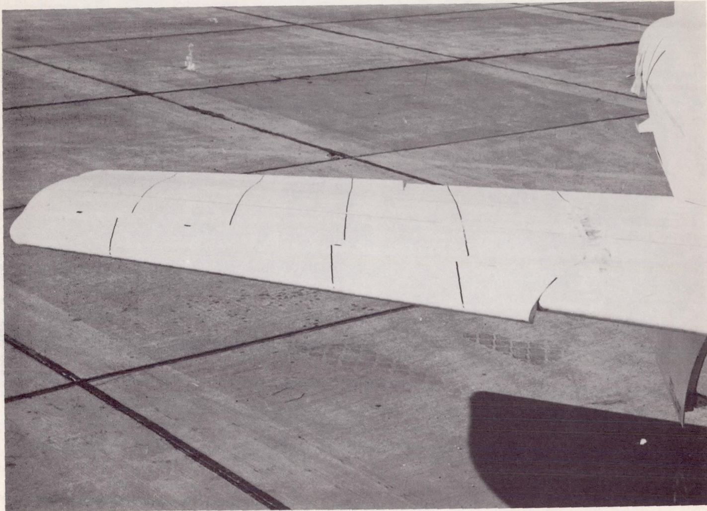
Figure 6.- Photograph of right wing of D-558-II airplane, showing slat in half-extended position with inboard wing fences removed.
