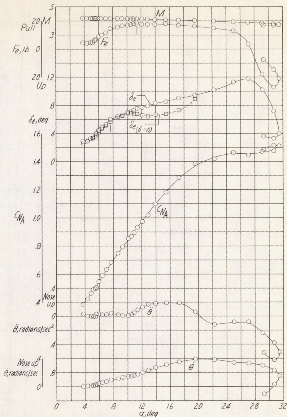
(a) h_p \approx 14,900 feet; i_t = 1.3^\circ ; center of gravity at 26.4 percent mean aerodynamic chord.
