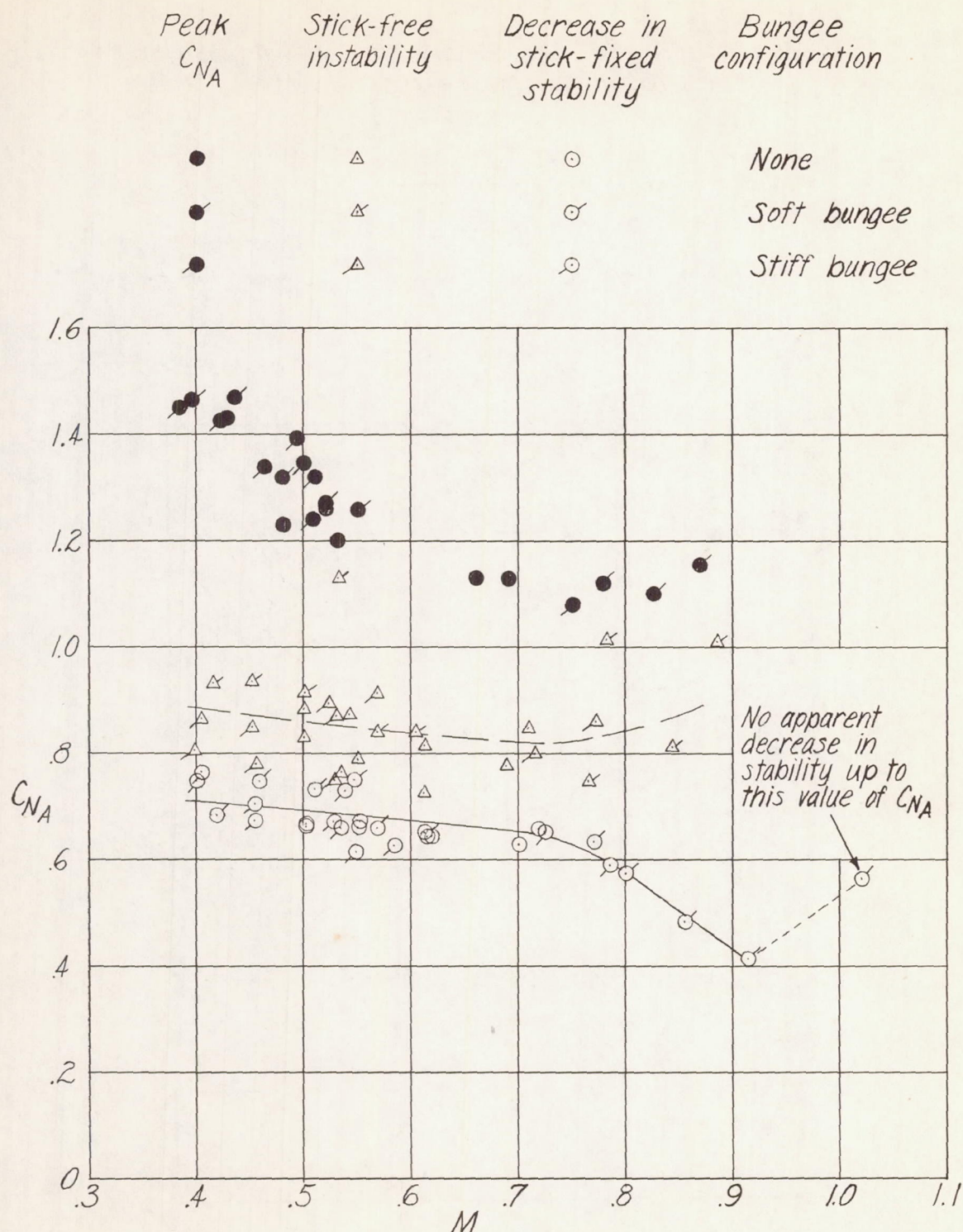
Figure 20.- Normal-force coefficient for decay in longitudinal stability as a function of Mach number for the airplane with fully extended slats and inboard wing fences removed.
