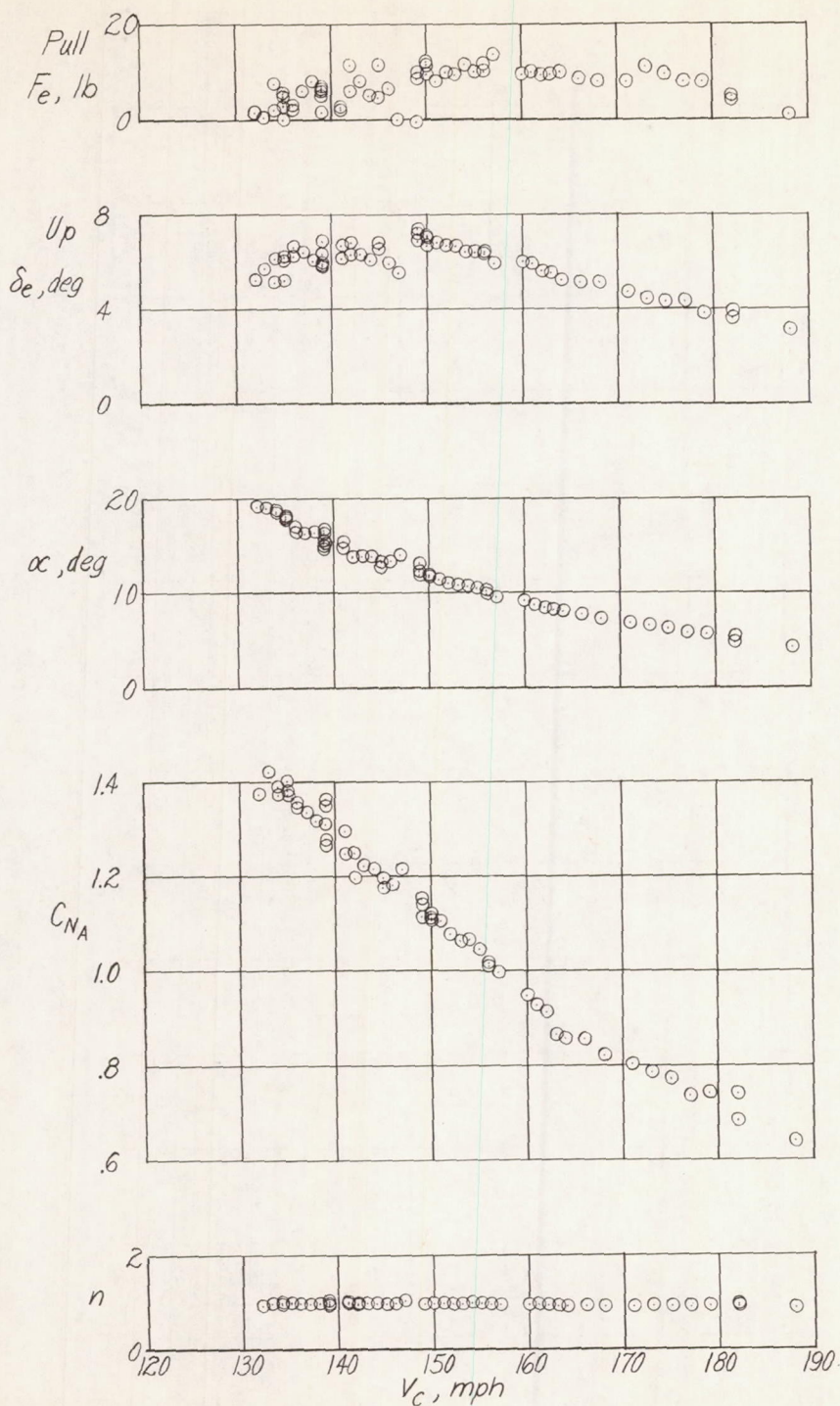
Figure 16.- Low-speed steady-flight static longitudinal stability characteristics of the Douglas D-558-II research airplane with slats fully extended and inboard wing fences removed. Flaps and landing gear extended; h_p \approx 19,250 feet; i_t = 1.6^\circ ; center of gravity at 24.9 percent mean aerodynamic chord.
