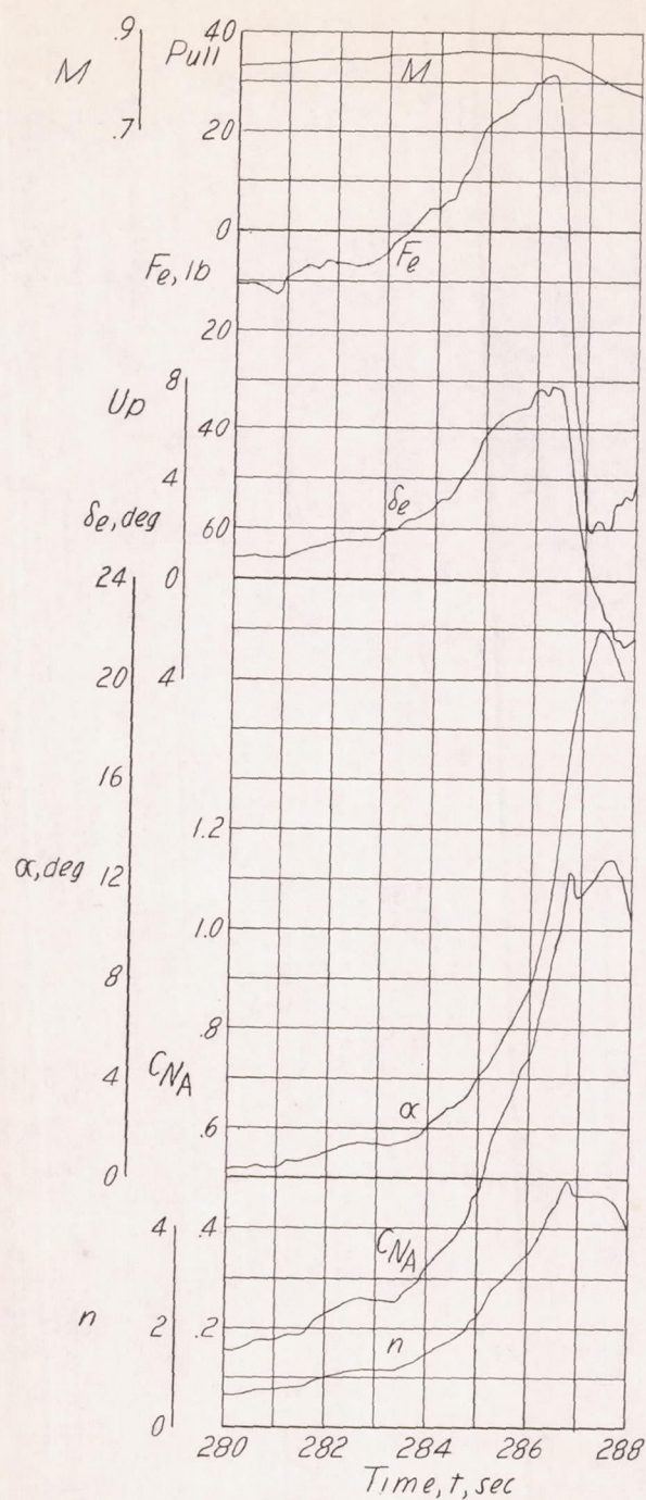
(a) h_p \approx 29,000 feet; i_t = 1.6^\circ ; center of gravity at 28.6 percent mean aerodynamic chord.
