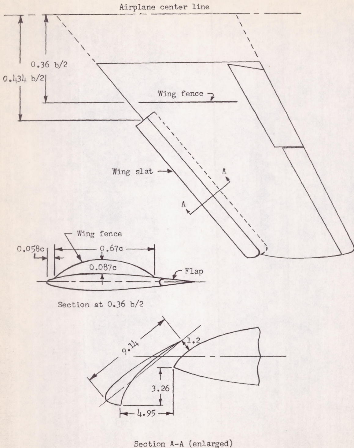
Figure 3.- Plan form and section of the wing of the Douglas D-558-II airplane showing the location of the slat in the fully extended position. All dimensions in inches except as noted.
