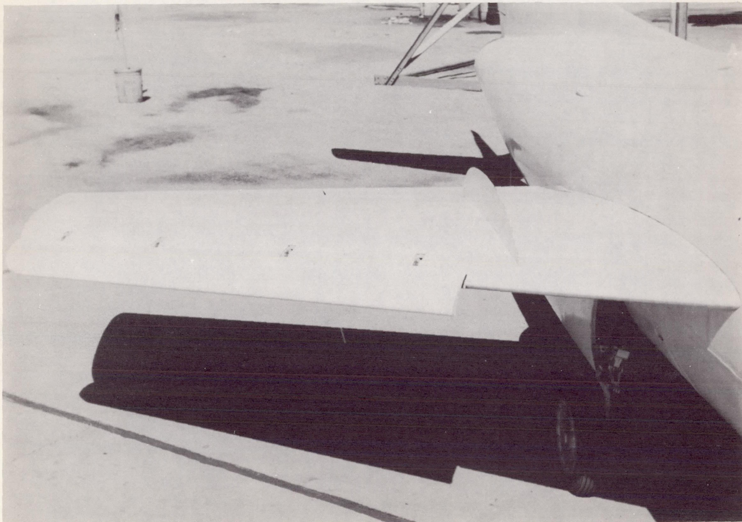
Figure 4.- Photograph of right wing of D-558-II airplane, showing slat in fully extended position and inboard fence on wing.
