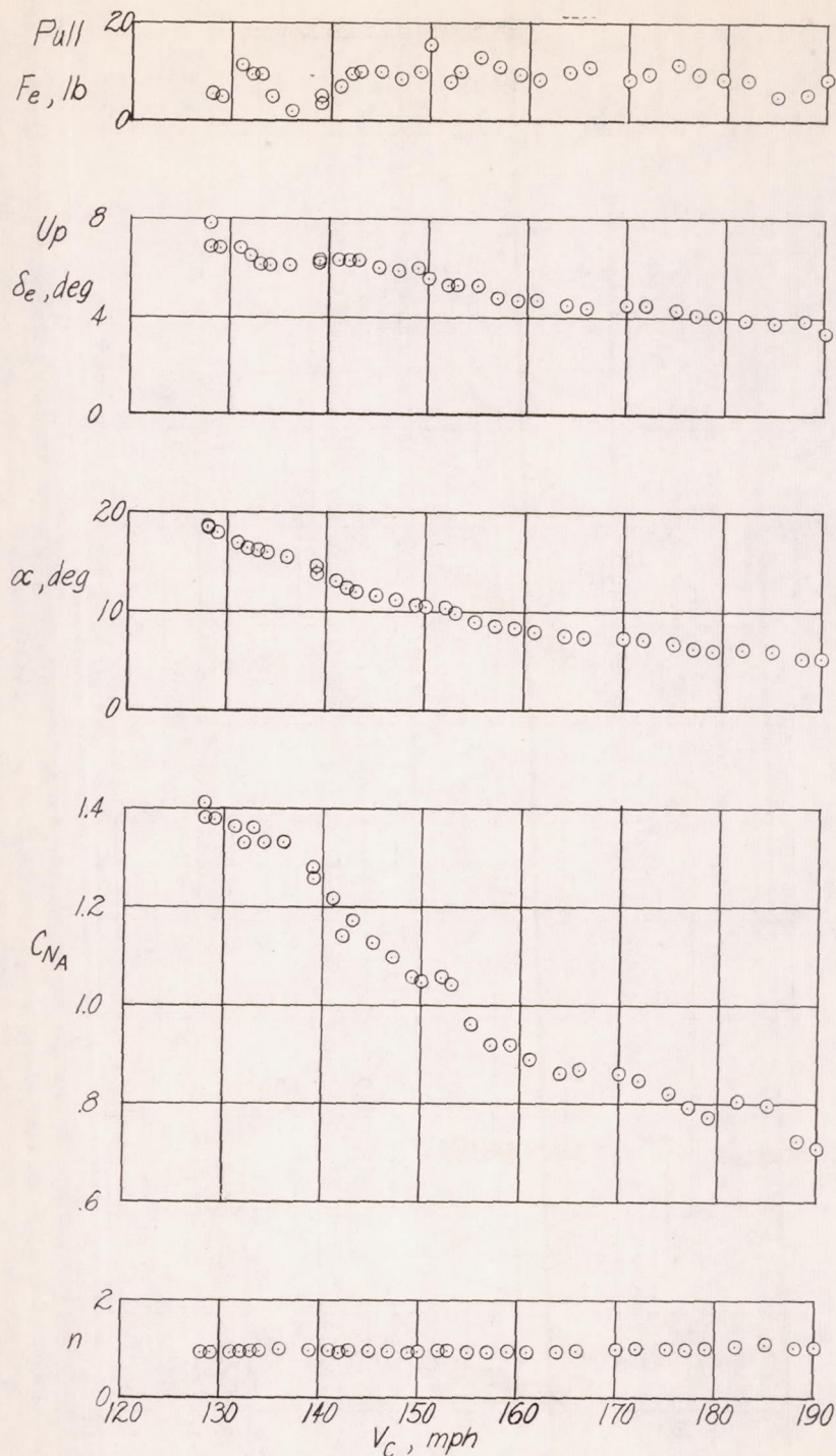
Figure 15.- Low-speed steady-flight static longitudinal stability characteristics of the Douglas D-558-II research airplane with slats fully extended and inboard wing fences on. Flaps and landing gear extended; h_p \approx 20,000 feet; i_t = 1.6^\circ ; center of gravity at 25.2 per cent mean aerodynamic chord.
