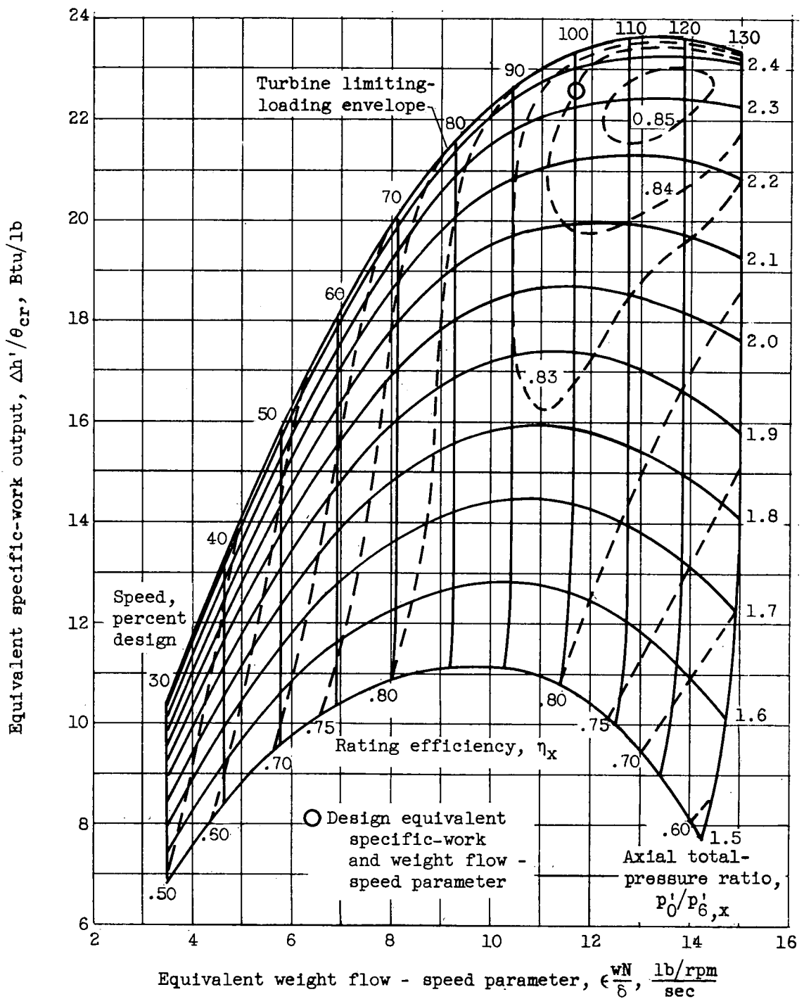
Figure 9. - Experimentally obtained performance map.
