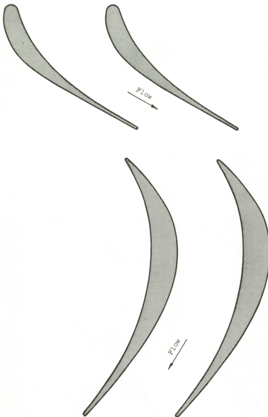
Figure 2. - Continued. Stator- and rotor-blade passages and profiles.
