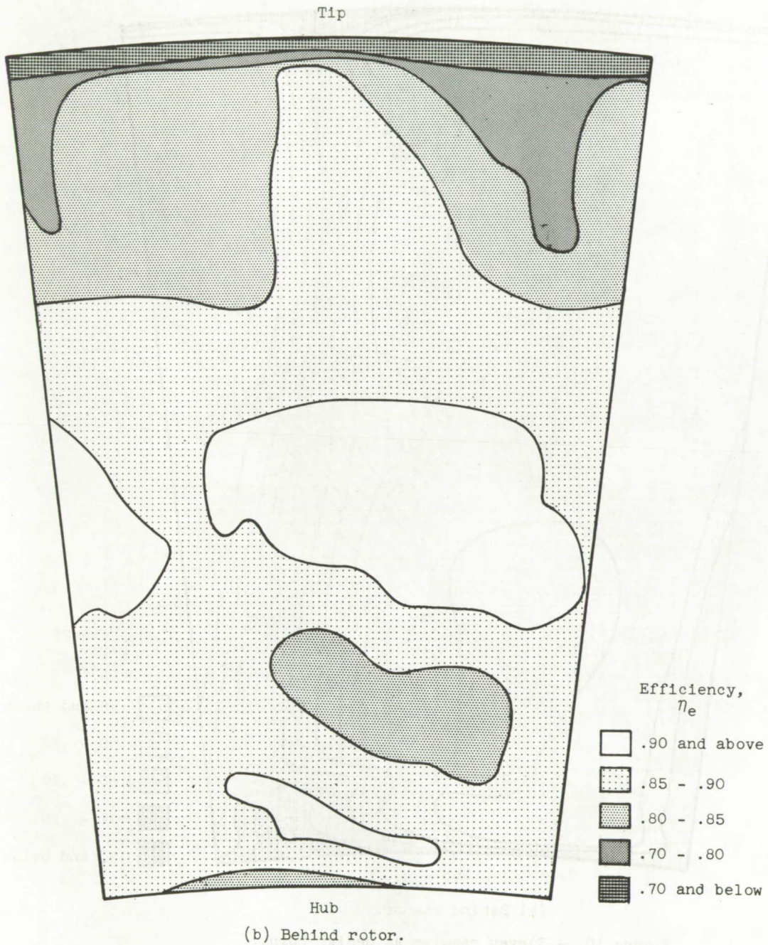
Figure 10. - Concluded. Survey results at design point.
