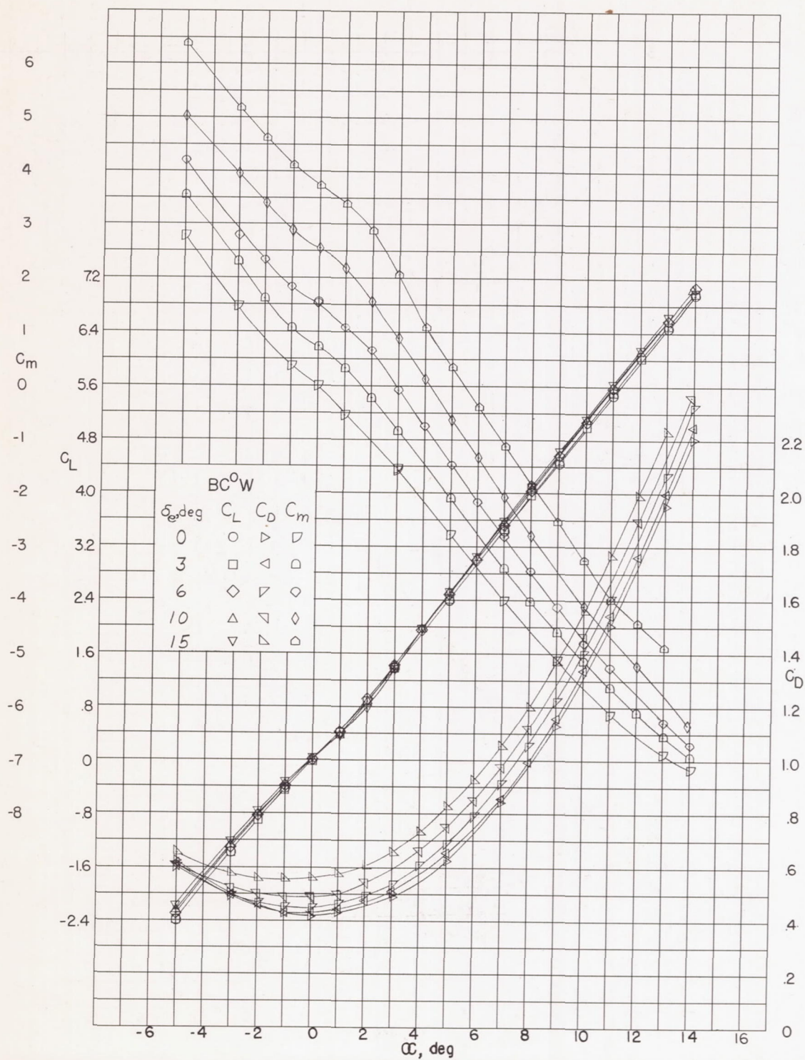
Figure 6.- Aerodynamic characteristics of inline BCW configuration for various deflections of the pitch canard fins. M = 1.62 ; \delta_r = \phi = 0^\circ .
