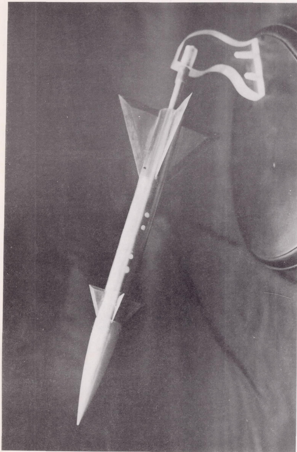
Figure 2.- Photograph of model.
