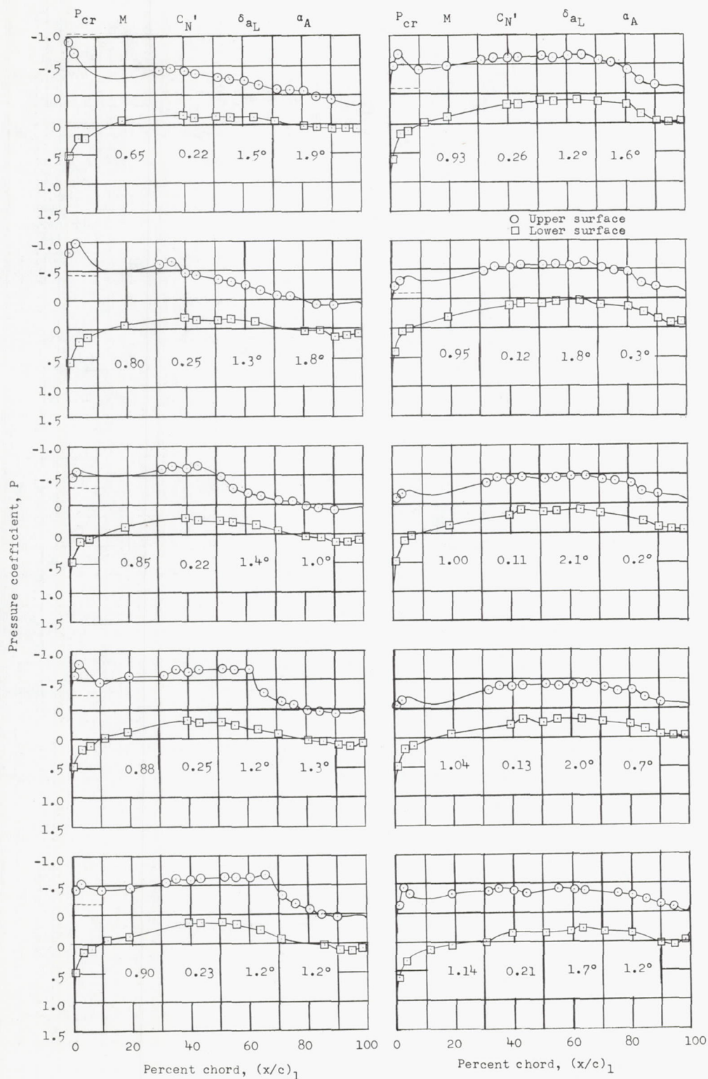
Figure 7.- Chordwise pressure distribution at midspan station located normal to 30-percent-common chord line.
