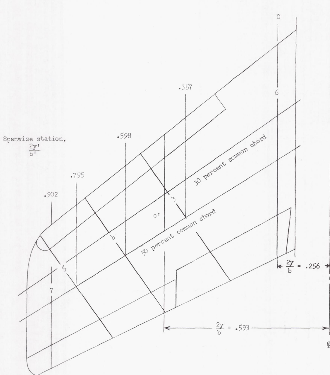
Figure 3.- Location of pressure-orifice stations.
