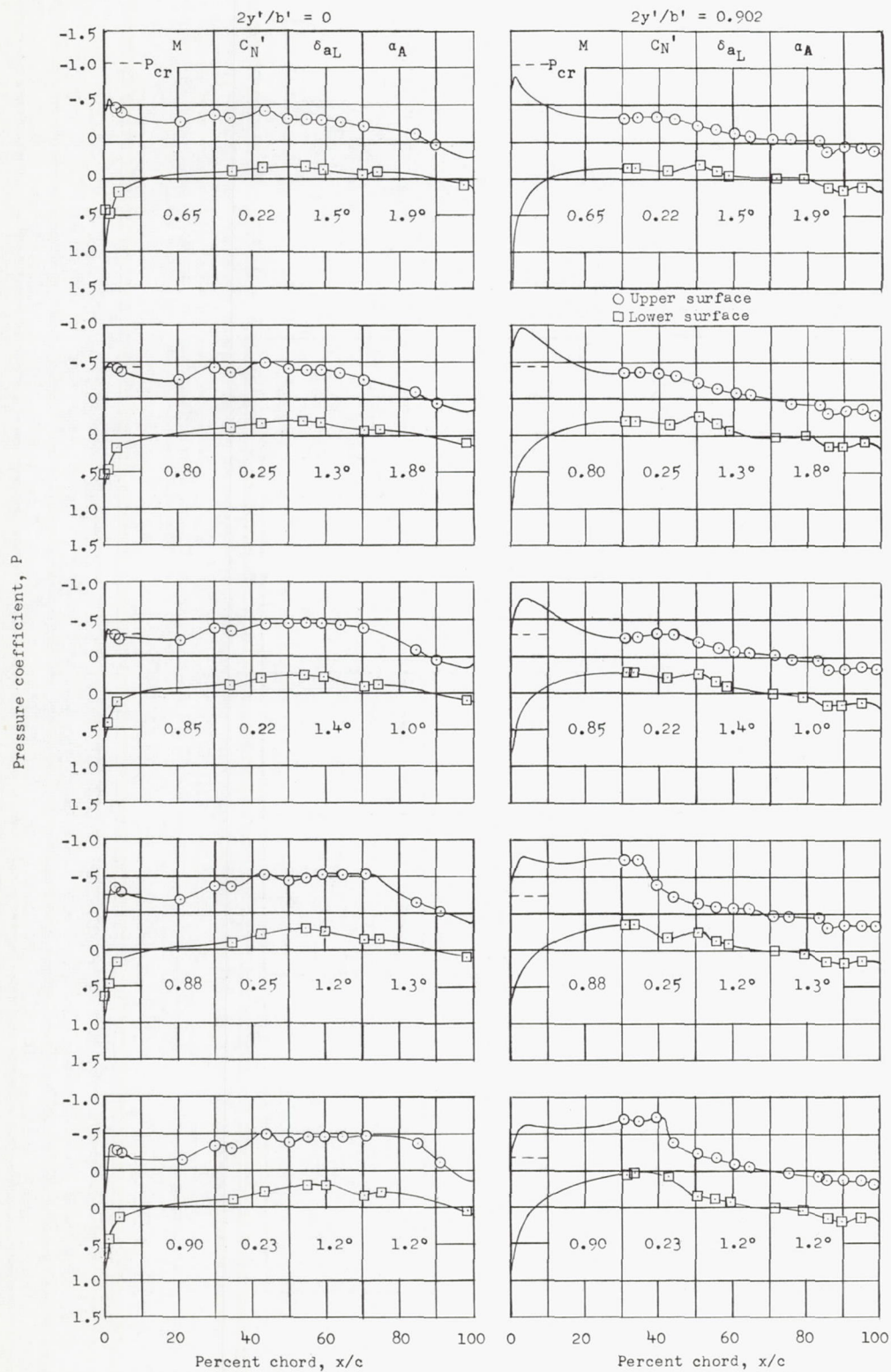
Figure 6.- Chordwise pressure distribution at root and tip stations.
