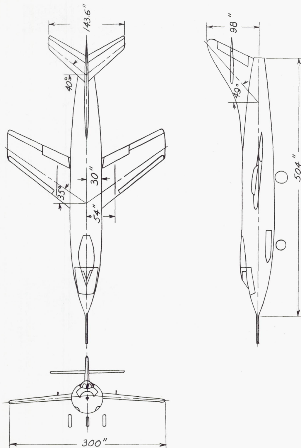
Figure 2.- Three-view drawing of Douglas D-558-II airplane.
