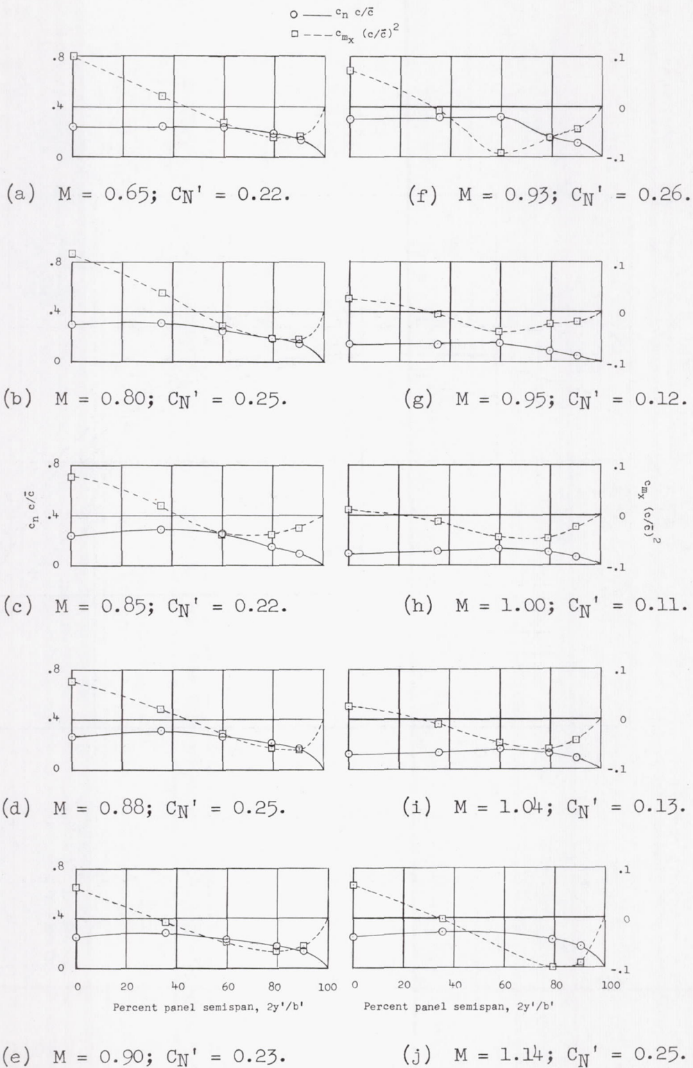
Figure 10.- Span load and pitching-moment distributions over the wing panel.
