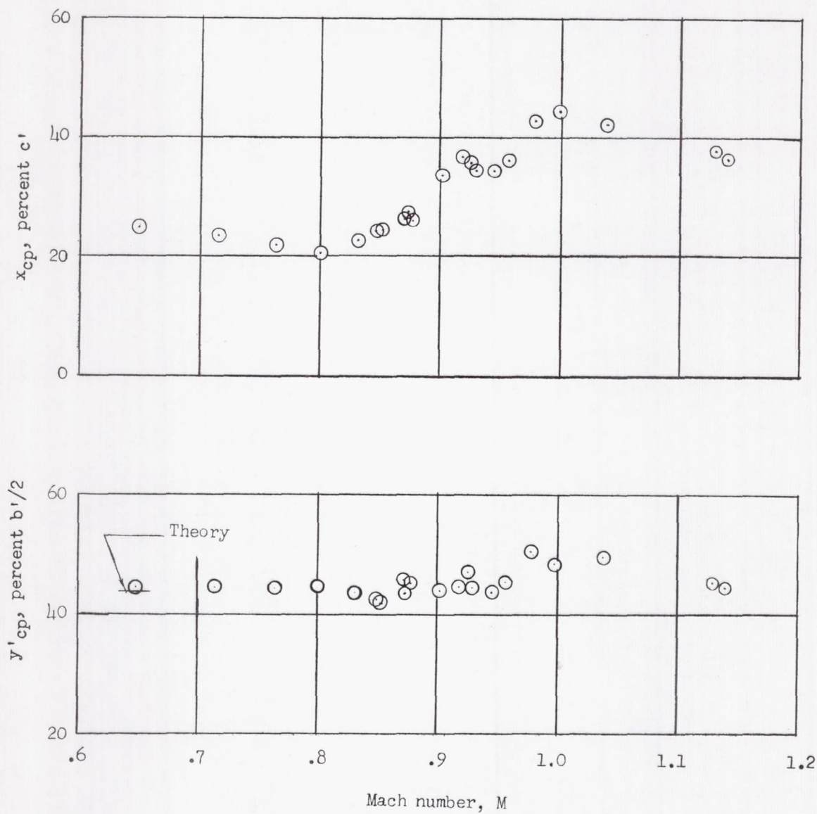
Figure 12.- Variation of spanwise and chordwise centers of pressure of the wing panel with Mach number.
