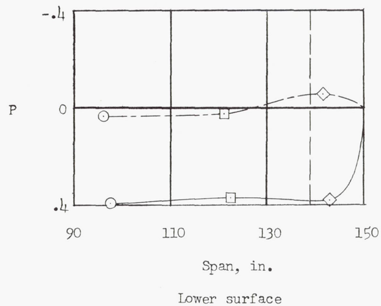
Figure 4.- Example of spanwise plot of individual pressure coefficients over leading edge of wing tip.
