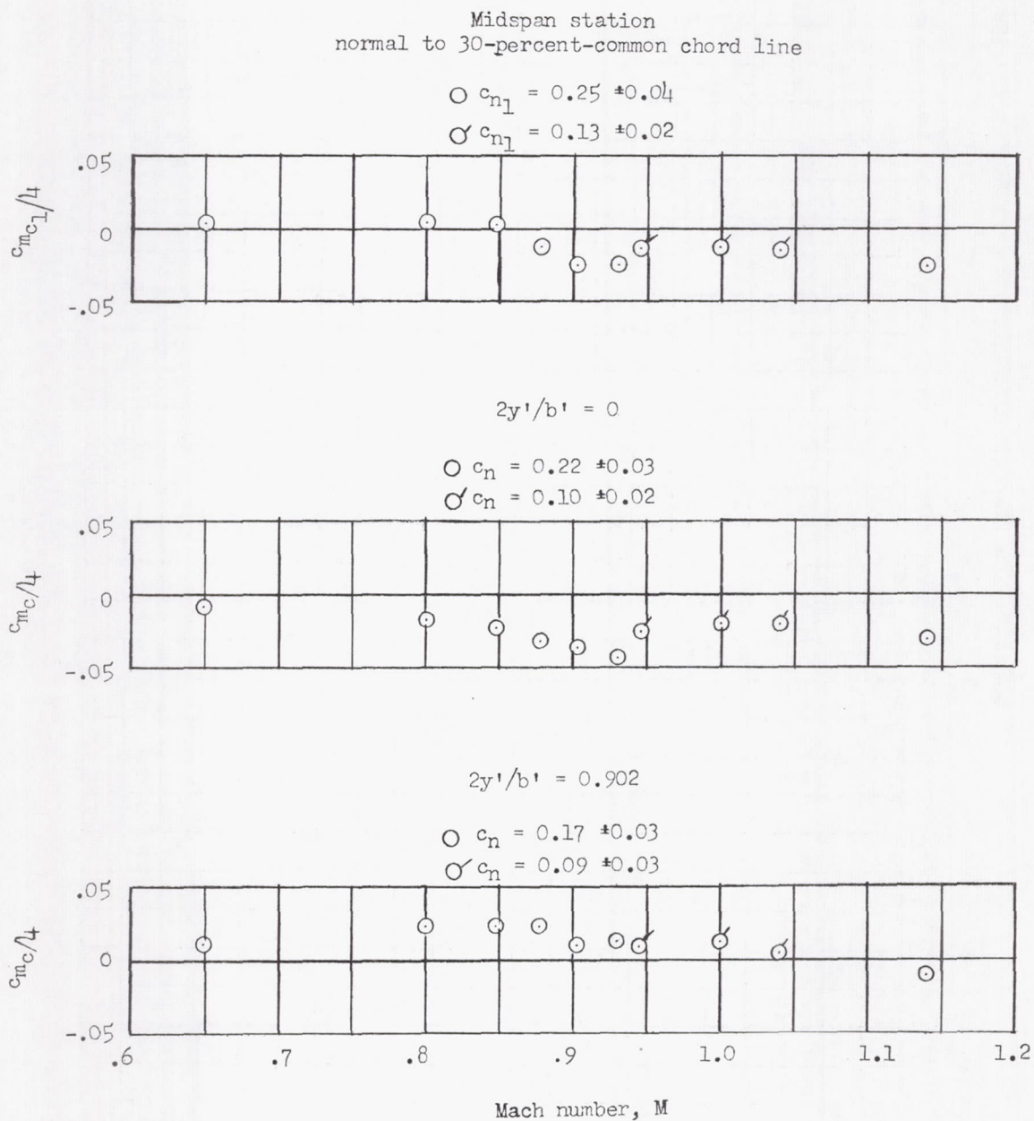
Figure 8.- Variation of the section pitching-moment coefficient with Mach number.
