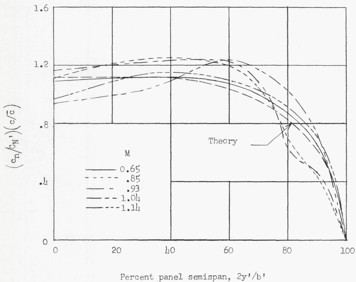
Figure 11.- Relative span loading of wing panel.
