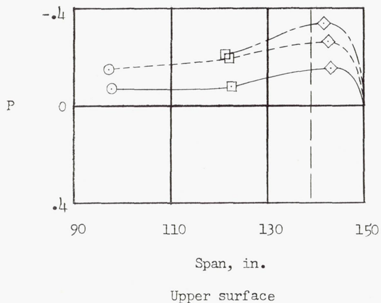
Figure 4.- Example of spanwise plot of individual pressure coefficients over leading edge of wing tip.
