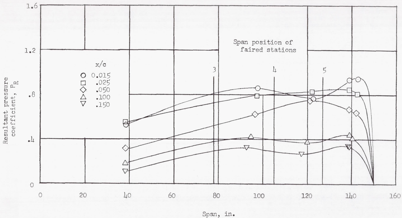
Figure 5.- Typical spanwise plot of resultant pressure coefficients over the wing panel.
