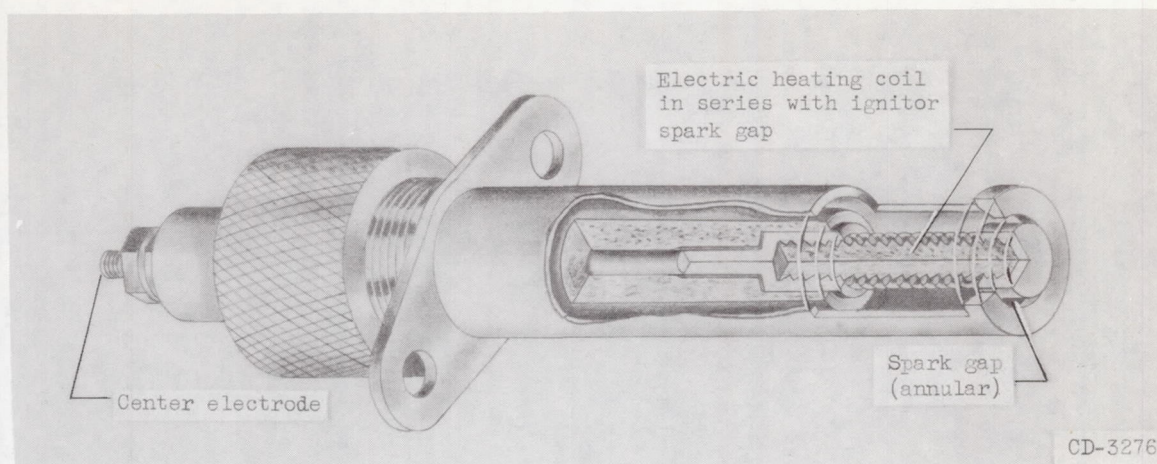
(g) Ignitor F (no cooling-air hole).
