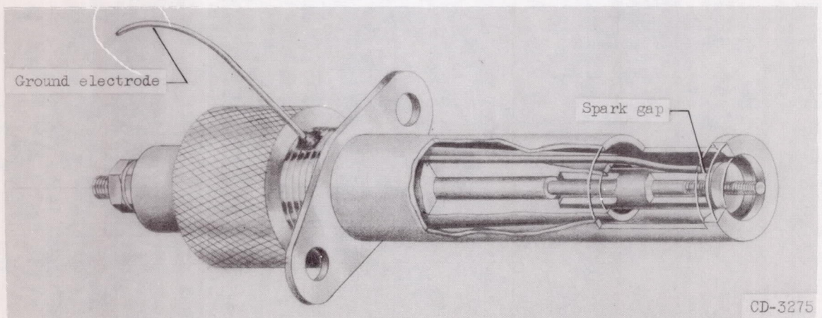
(f) Ignitor E (no cooling-air hole).
