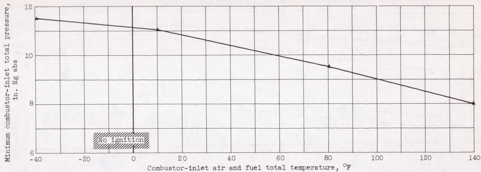
Figure 20. - Effect of inlet-air and fuel temperature on minimum inlet pressure for ignition in single tubular combustor. Triggered commercial ignition system; ignitor 0; fuel, NACA 52-288; air flow, 1.87 pounds per second per square foot; spark energy, 2.12 joules.
