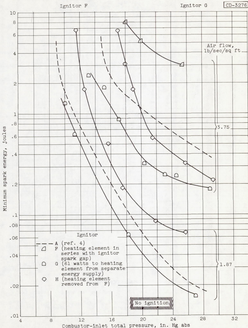
Figure 8. - Effect of fuel heating at spark electrodes on ignition-energy requirements of single tubular combustor. Fuel-spray nozzle, variable-area type; experimental ignition system; fuel, NACA 50-197; inlet-air and fuel temperature, 10° F.
