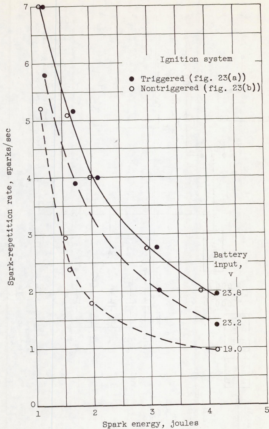
Figure 24. - Variation of spark-repetition rate with spark-energy level and battery-input voltage. Commercial ignition systems.
