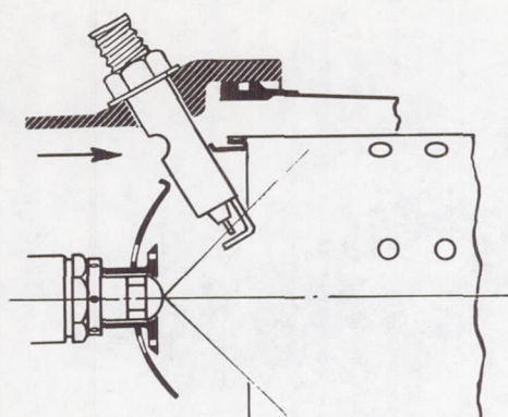
(a) Standard installation; \frac{1}{16} -inch diametral clearance between ignitor and combustor; cooling-air hole open.
