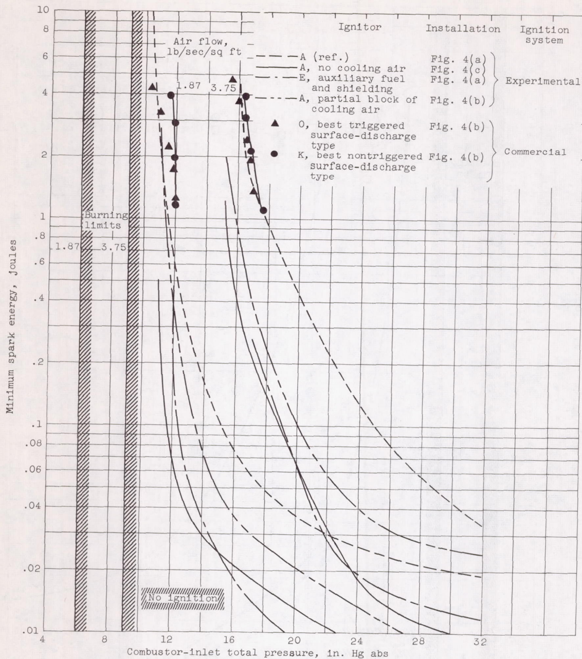
Figure 16. - Comparison of combustor ignition-energy requirements with experimental and commercial ignition systems. Fuel, NACA 50-197; inlet-air and fuel temperature, 10° F.
