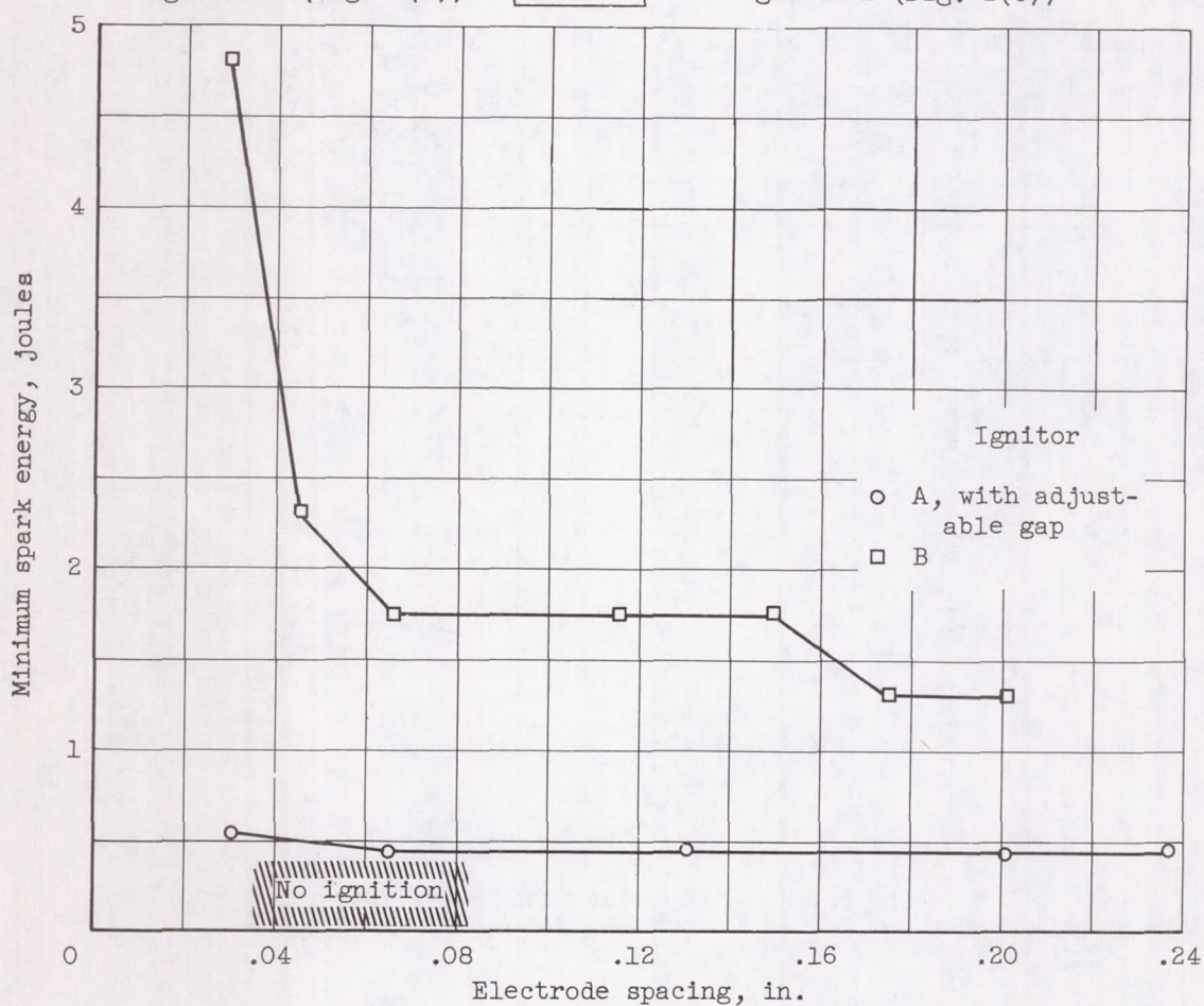
Figure 5. - Effect of electrode spacing on ignition-energy requirements of single tubular combustor. Experimental ignition system; fuel, NACA 50-197; inlet-air pressure, 12 inches of mercury absolute; air flow, 1.87 pounds per second per square foot; inlet-air and fuel temperature, 100° F.
