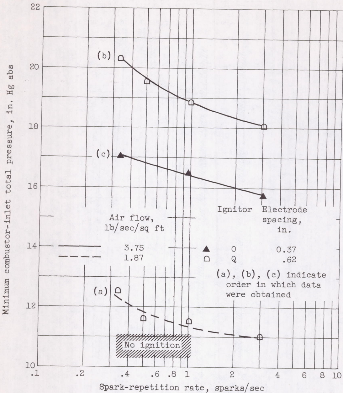
Figure 14. - Effect of spark-repetition rate on ignition limits of single tubular combustor at two air-flow rates. Fuel, NACA 52-288; inlet-air and fuel temperature, 10^{\circ}\text{F} ; spark energy, 2.32 joules.
