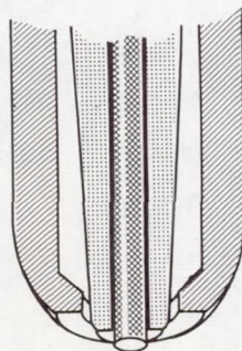
(m) Sectional view of experimental air-gap ignitor S. (Cooling-air entrance in outer shell of ignitor.)
