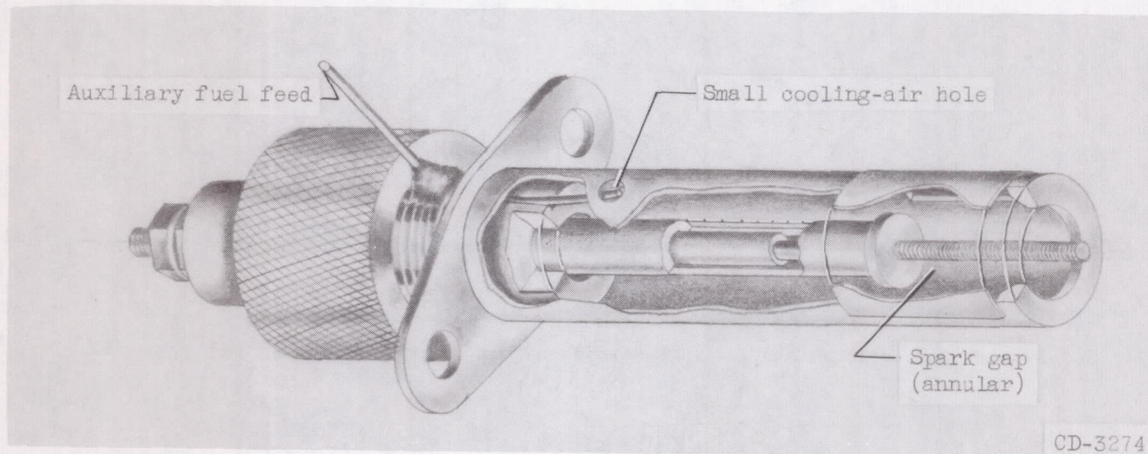
(k) Ignitor J (full shield).
