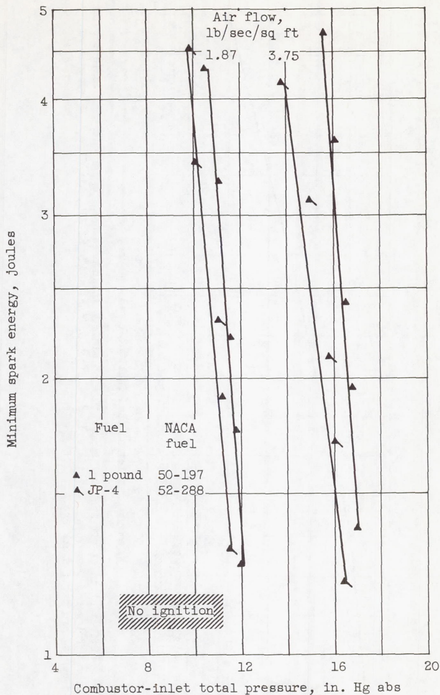
Figure 21. - Effect of fuel volatility on ignition limits obtained in single tubular combustor. Triggered surface-discharge ignitor 0; inlet-air and fuel temperature, 10^{\circ} F; fuel nozzle, 10.5 gallons per hour, 80^{\circ} spray-cone angle.
