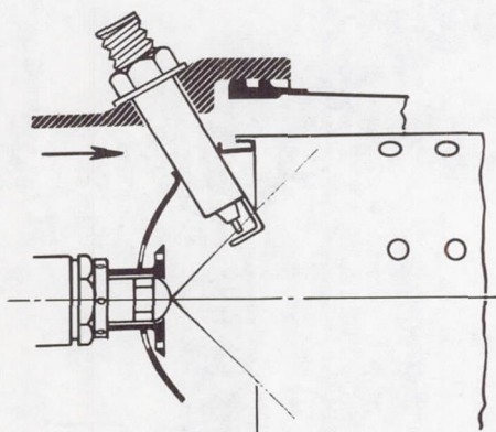
(c) No cooling air; no diametral clearance or cooling-air hole.
