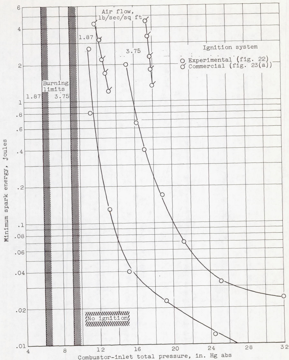
Figure 17. - Comparison of combustor ignition-energy requirements in single tubular combustor with experimental and commercial ignition systems. Ignitor A with partial block of cooling air (fig. 4(b)); fuel, NACA 50-197; inlet-air and fuel temperature, 10° F.
