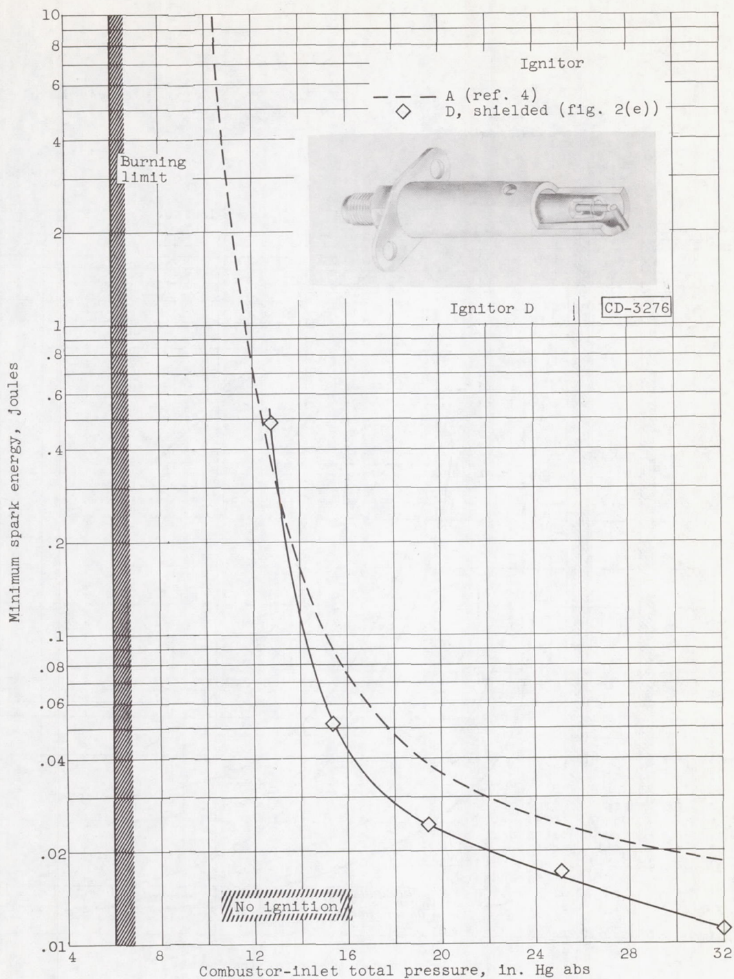
(b) Ignitor D; air flow, 1.87 pounds per second per square foot.
