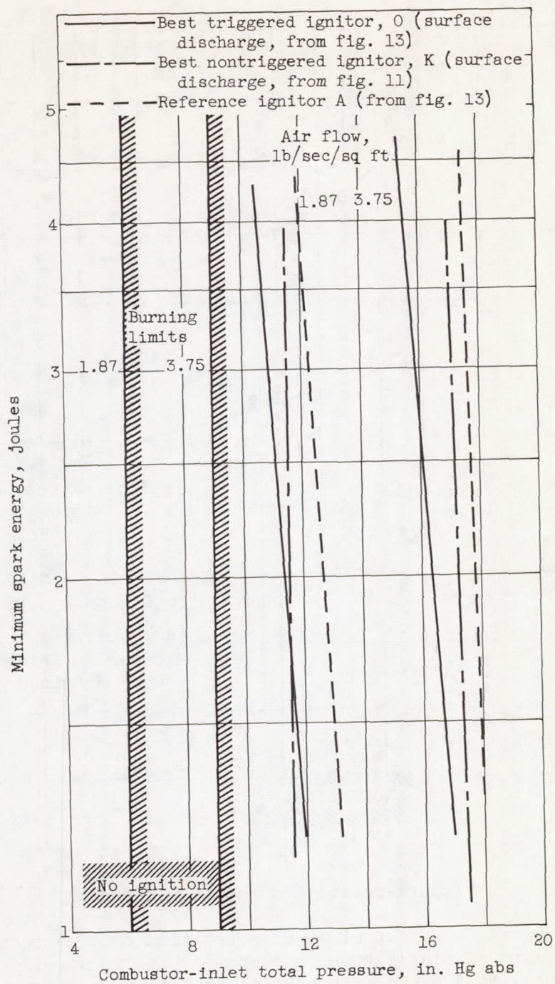
Figure 15. - Comparison of ignition limits of single tubular combustor with the best non-triggered and triggered surface-discharge ignitors and with reference air-gap ignitor A. Commercial ignition system; ignitor installation, figure 4(b); fuel, NACA 50-197; inlet-air and fuel temperature, 10° F.
