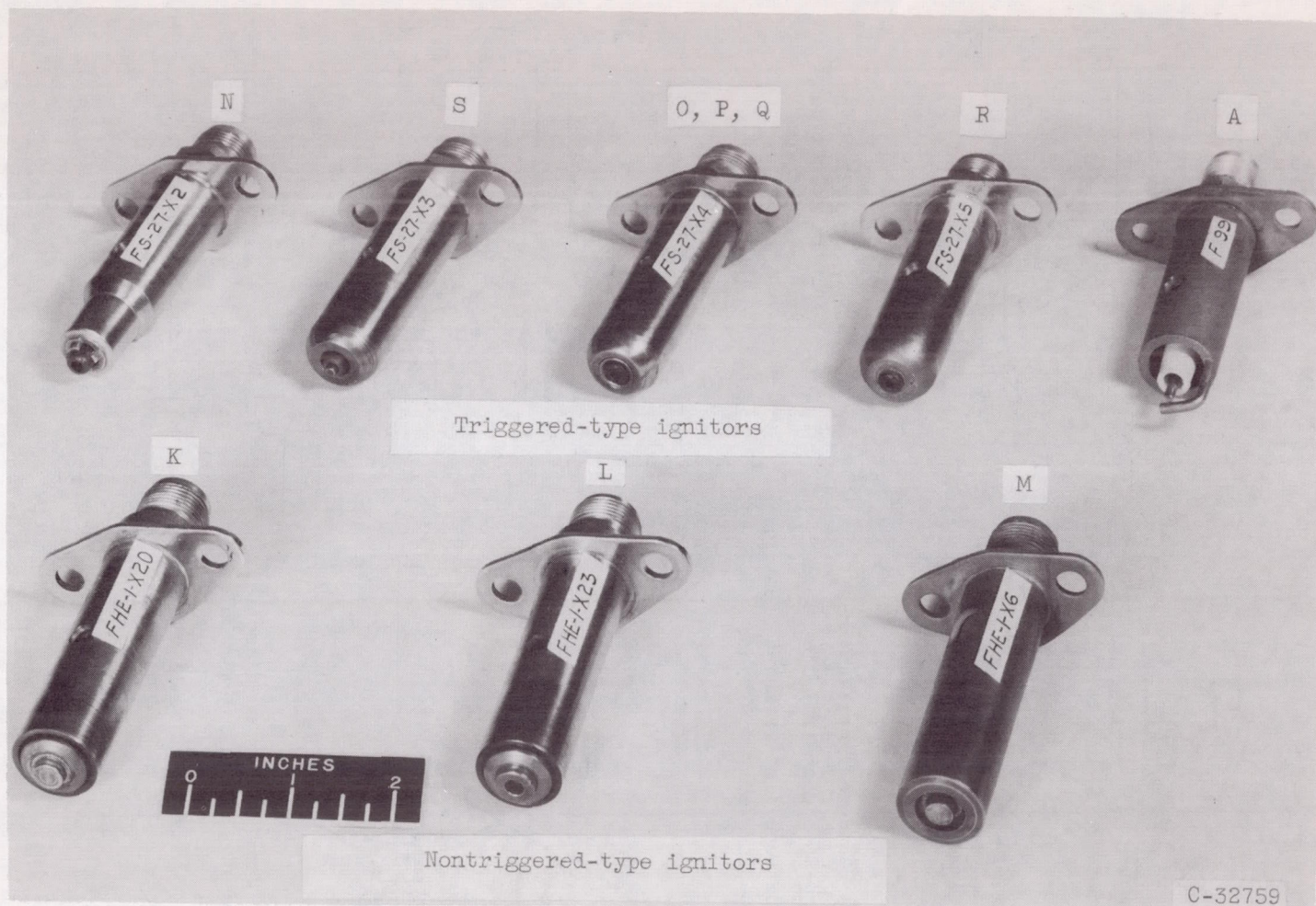
Figure 3. - Experimental ignitors K through R; reference ignitor A.
