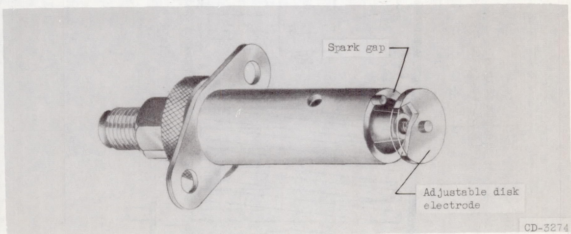
(c) Ignitor B.
