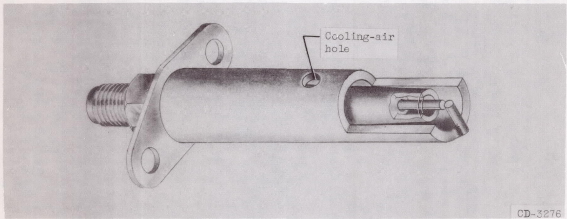
(e) Ignitor D (partial shield).
