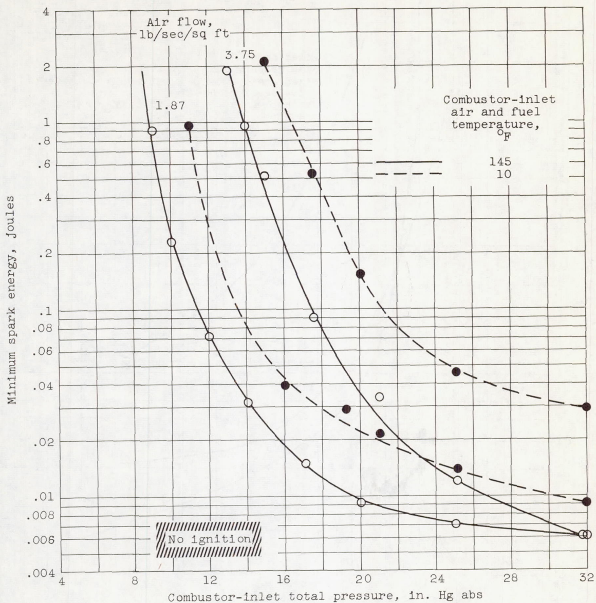
Figure 19. - Effect of inlet-air and fuel temperature on spark energy required for ignition in single tubular combustor. Experimental ignition system; ignitor A, with partial block of cooling air (fig. 4(b)); fuel, NACA 50-197.
