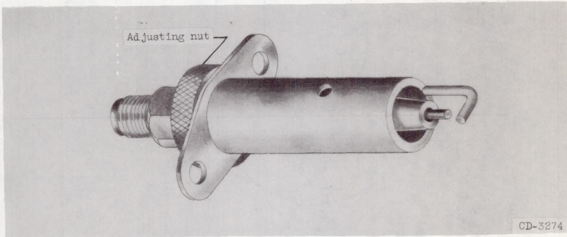
(b) Ignitor A with adjustable spark gap.
