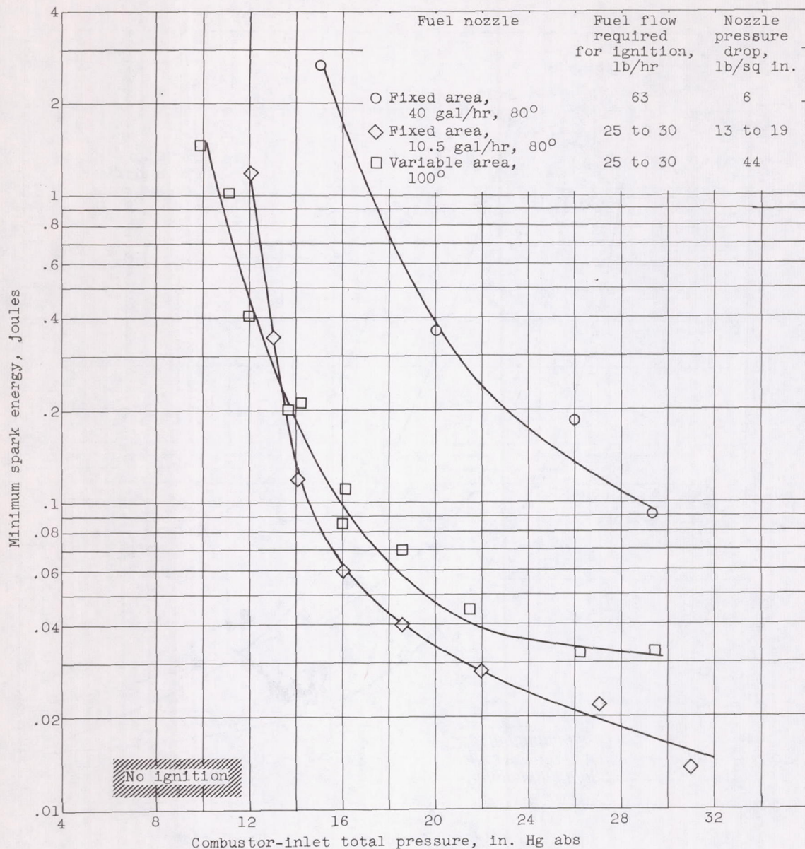
Figure 18. - Effect of fuel-spray nozzle on spark energy required for ignition in single tubular combustor. Experimental ignition system; ignitor A; fuel, NACA 51-192 (ref. 4); air flow, 1.87 pounds per second per square foot; inlet-air and fuel temperature, 10° F.
