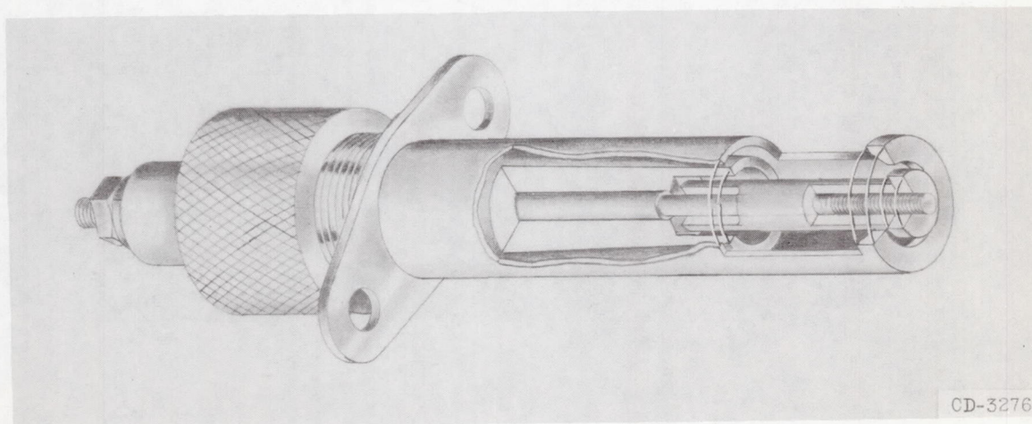
(i) Ignitor H (no heating element, no cooling-air hole).
