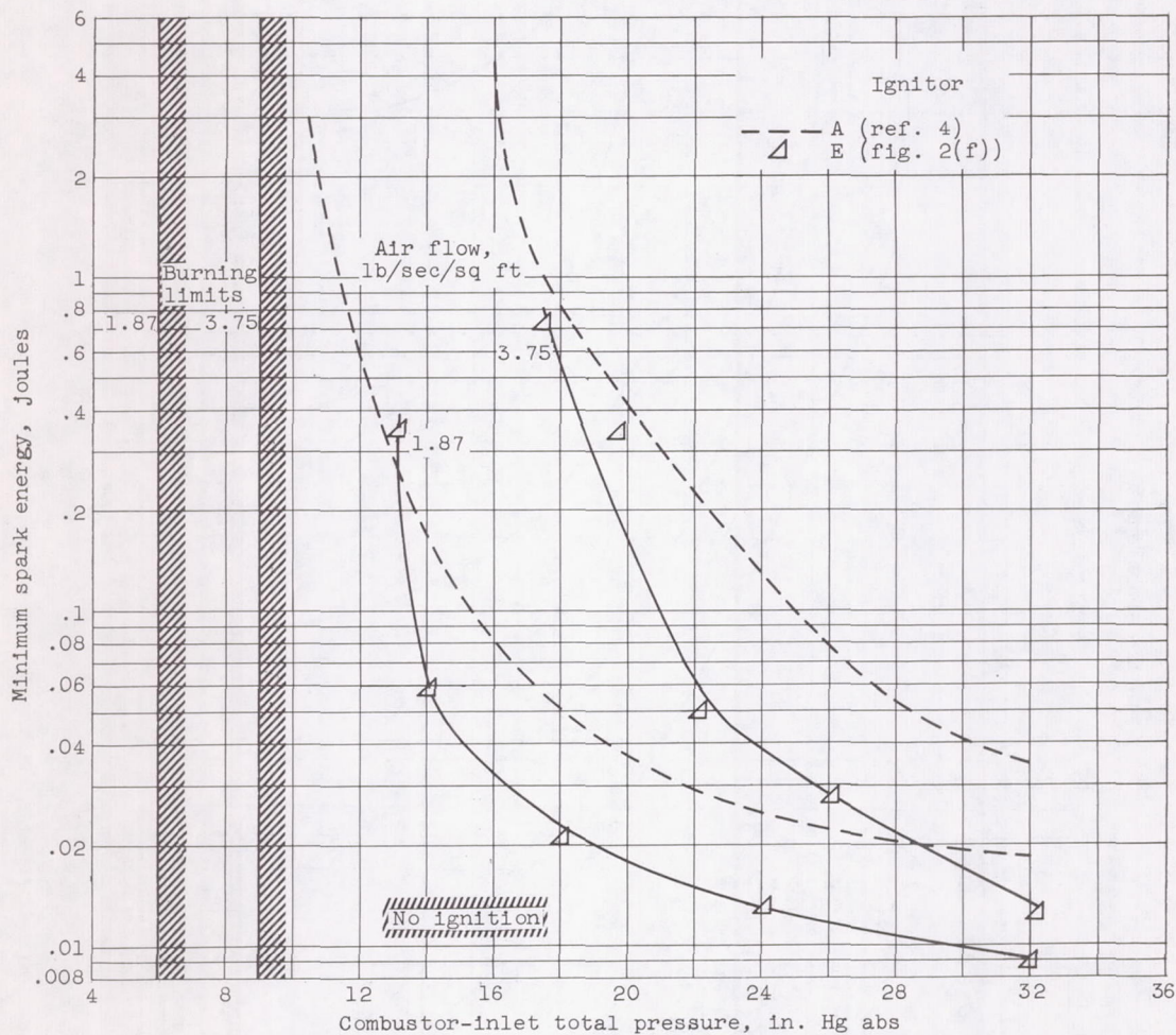
(c) Ignitor E; air flow, 1.87 and 3.75 pounds per second per square foot.
