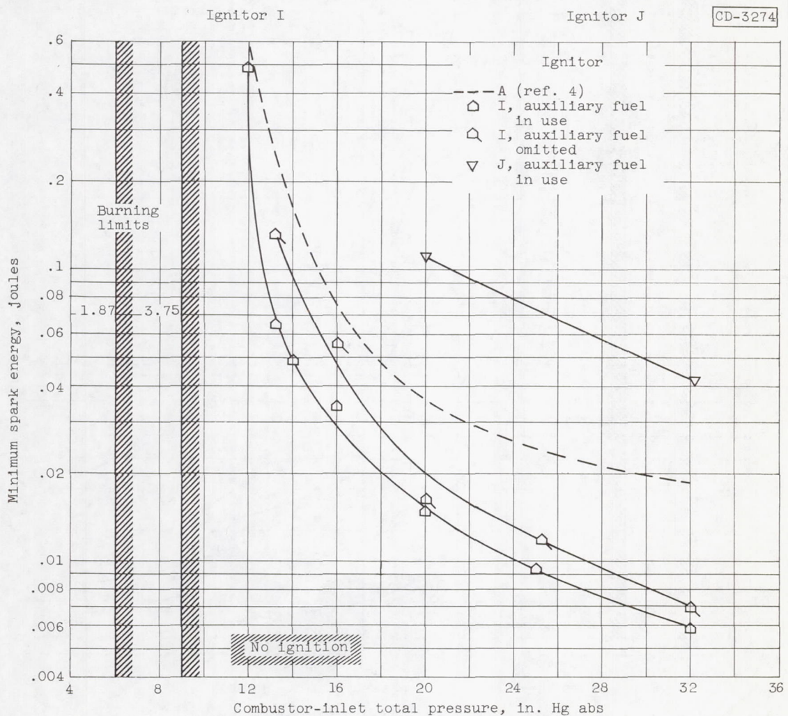
(b) Ignitors I and J; air flow, 1.87 pounds per second per square foot.
