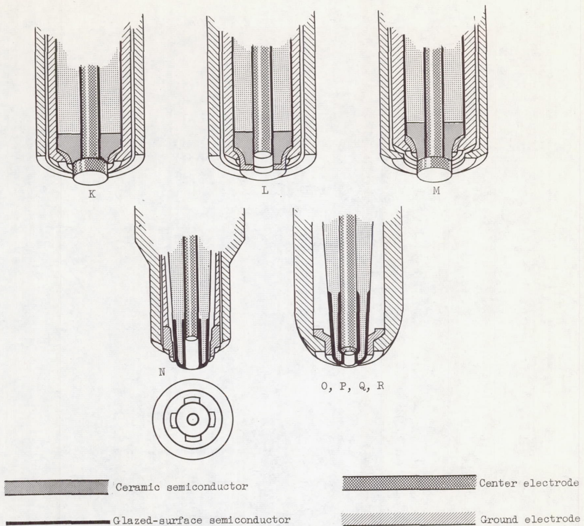
(l) Sectional views of experimental surface-discharge ignitors. (Cooling-air entrance in outer shell of ignitors.)
