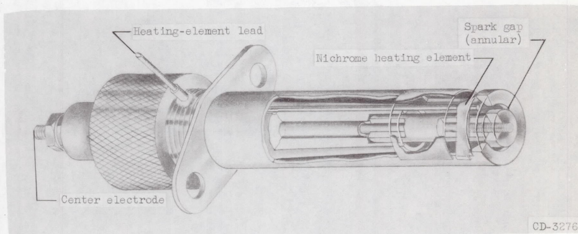
(h) Ignitor G (no cooling-air hole).
