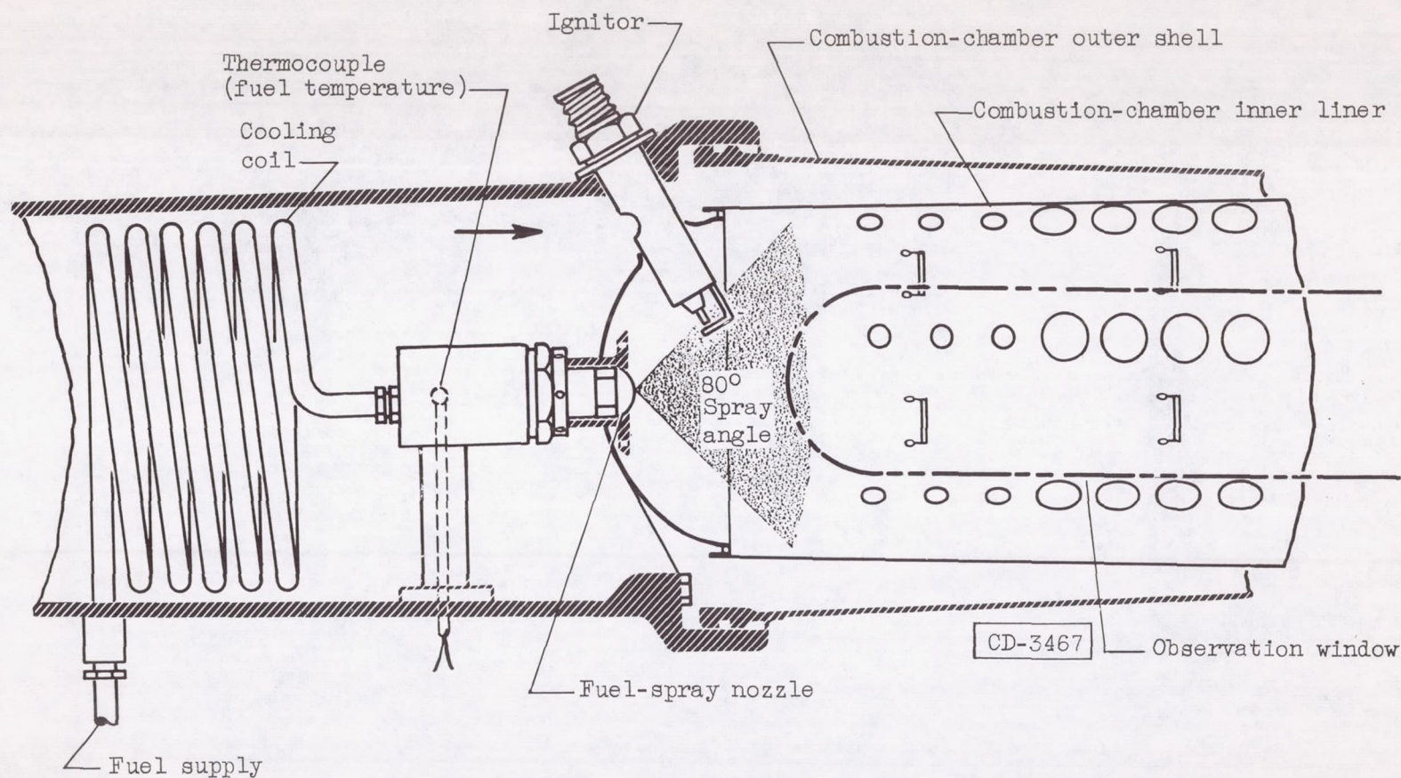
Figure 1. - Diagrammatic cross section of single tubular combustor (ref. 4).
