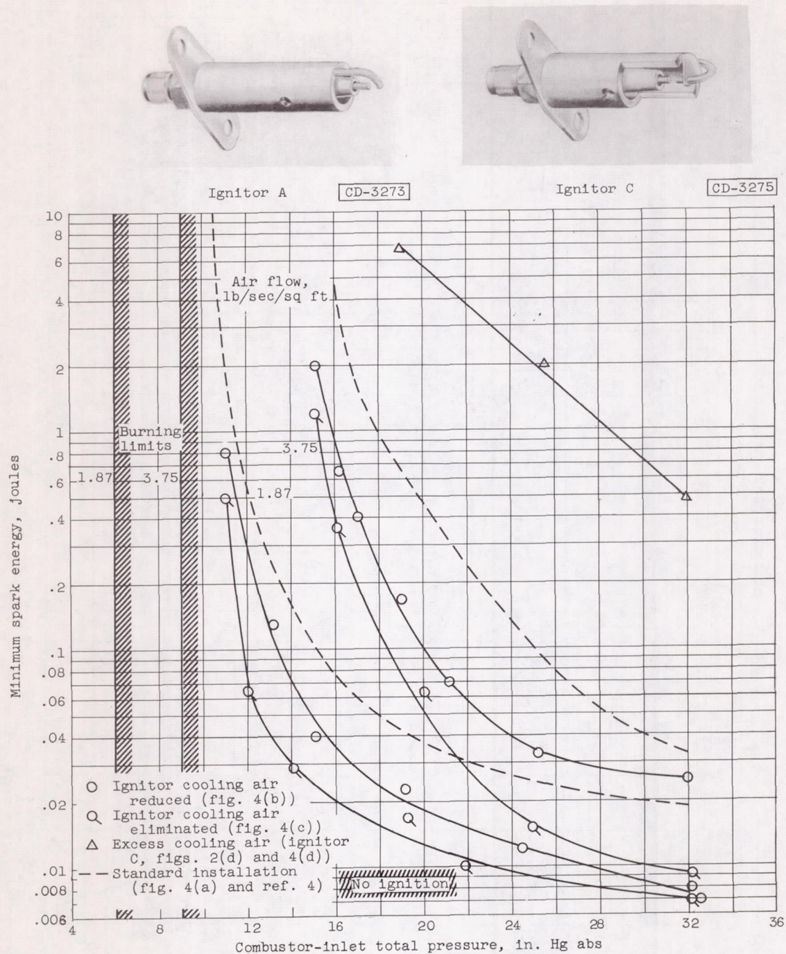
(a) Ignitors A and C; air flow, 1.87 and 3.75 pounds per second per square foot.
