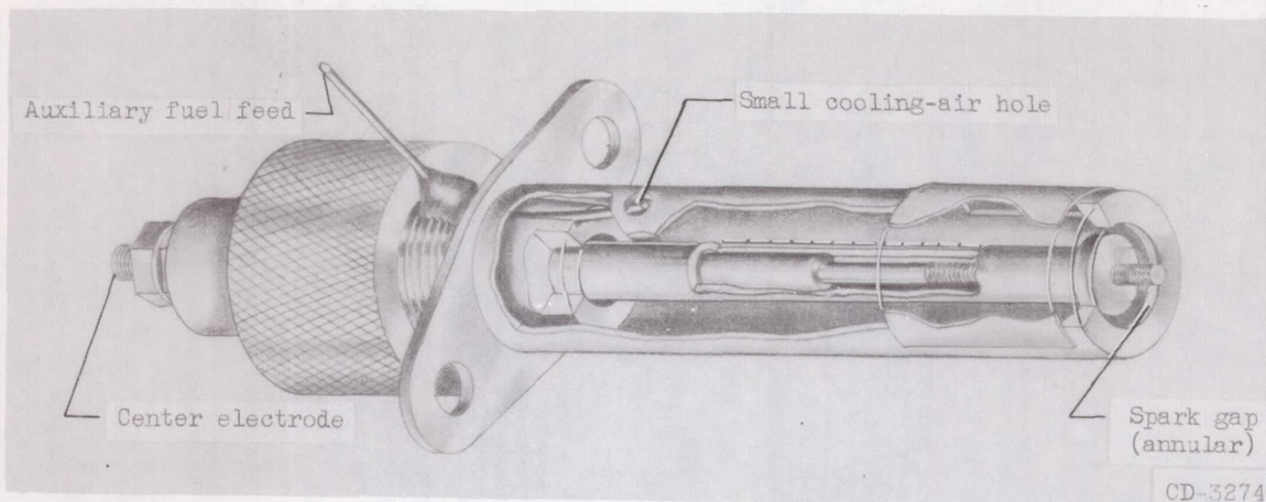
(j) Ignitor I (full shield).
