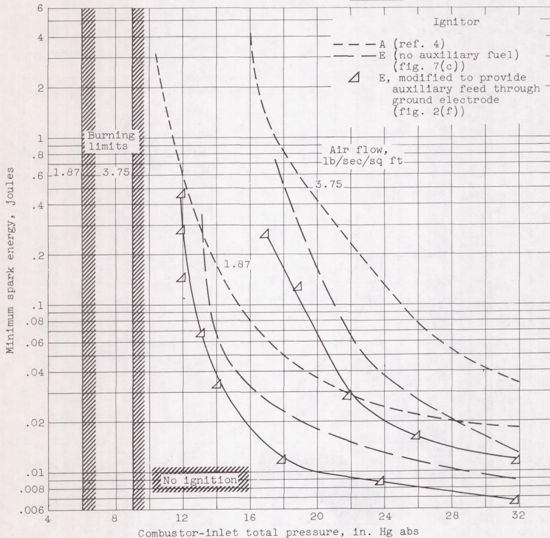
(a) Ignitor E modified; air flow, 1.87 and 3.75 pounds per second per square foot.
