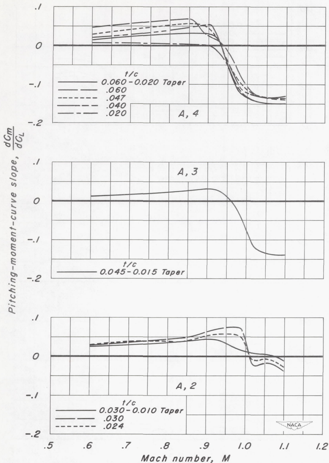
Figure 11.- The variation of pitching-moment-curve slope with Mach number. C_L = 0 .
