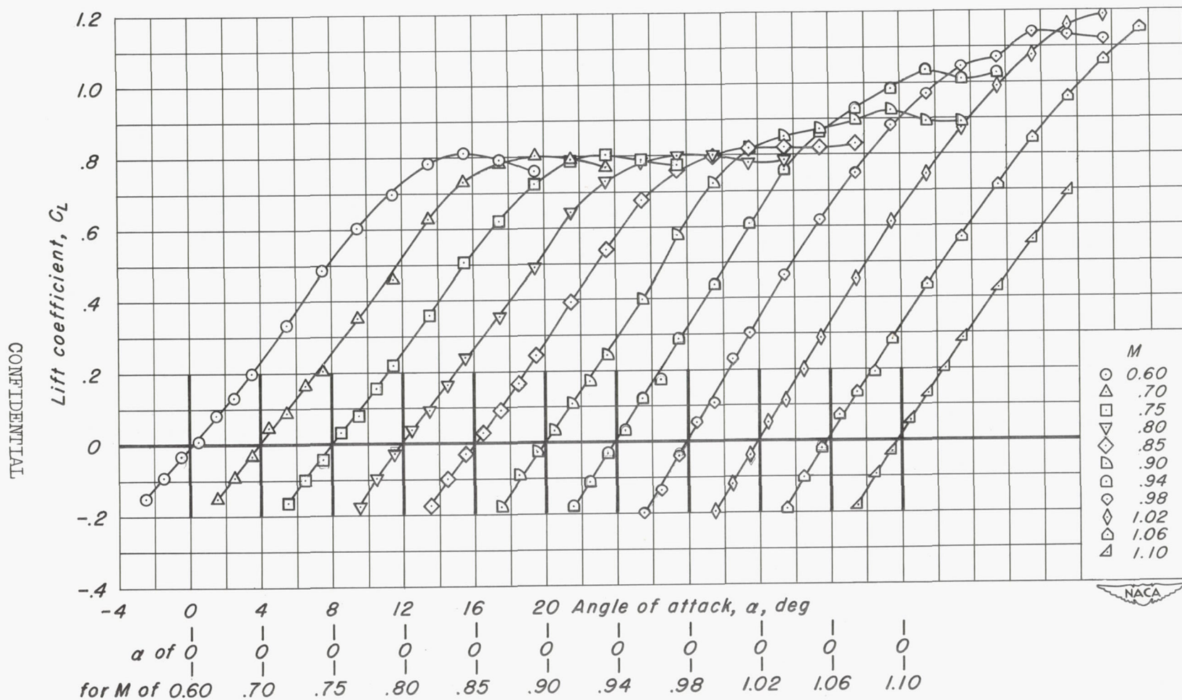
(a) Lift characteristics.
