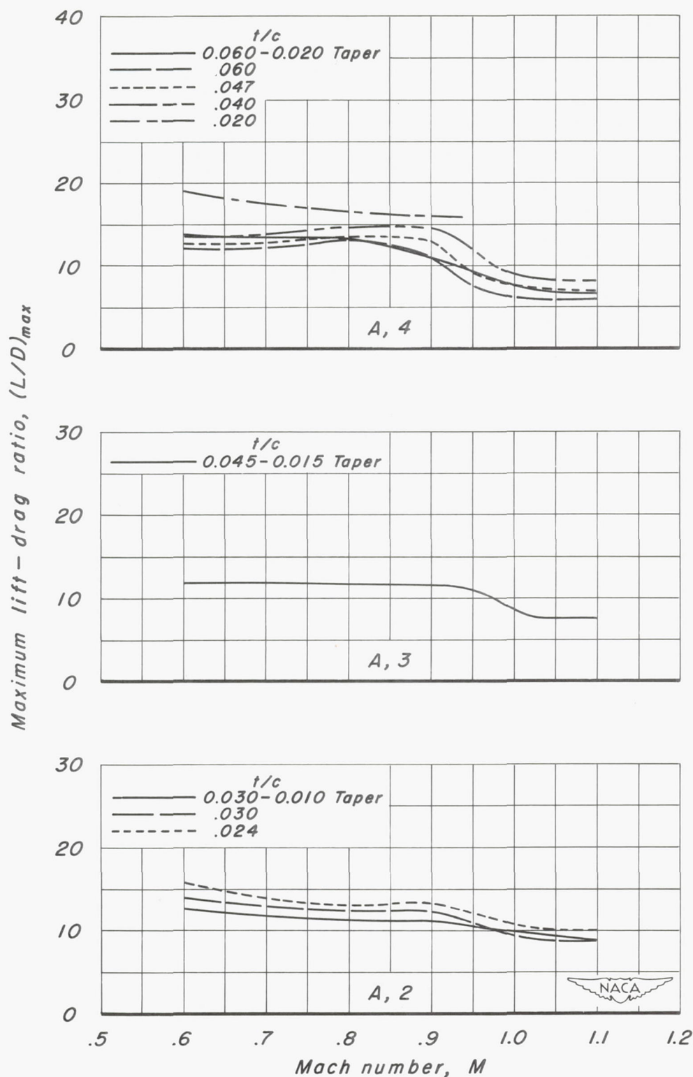
Figure 13.- The variation of maximum lift-drag ratio with Mach number.
