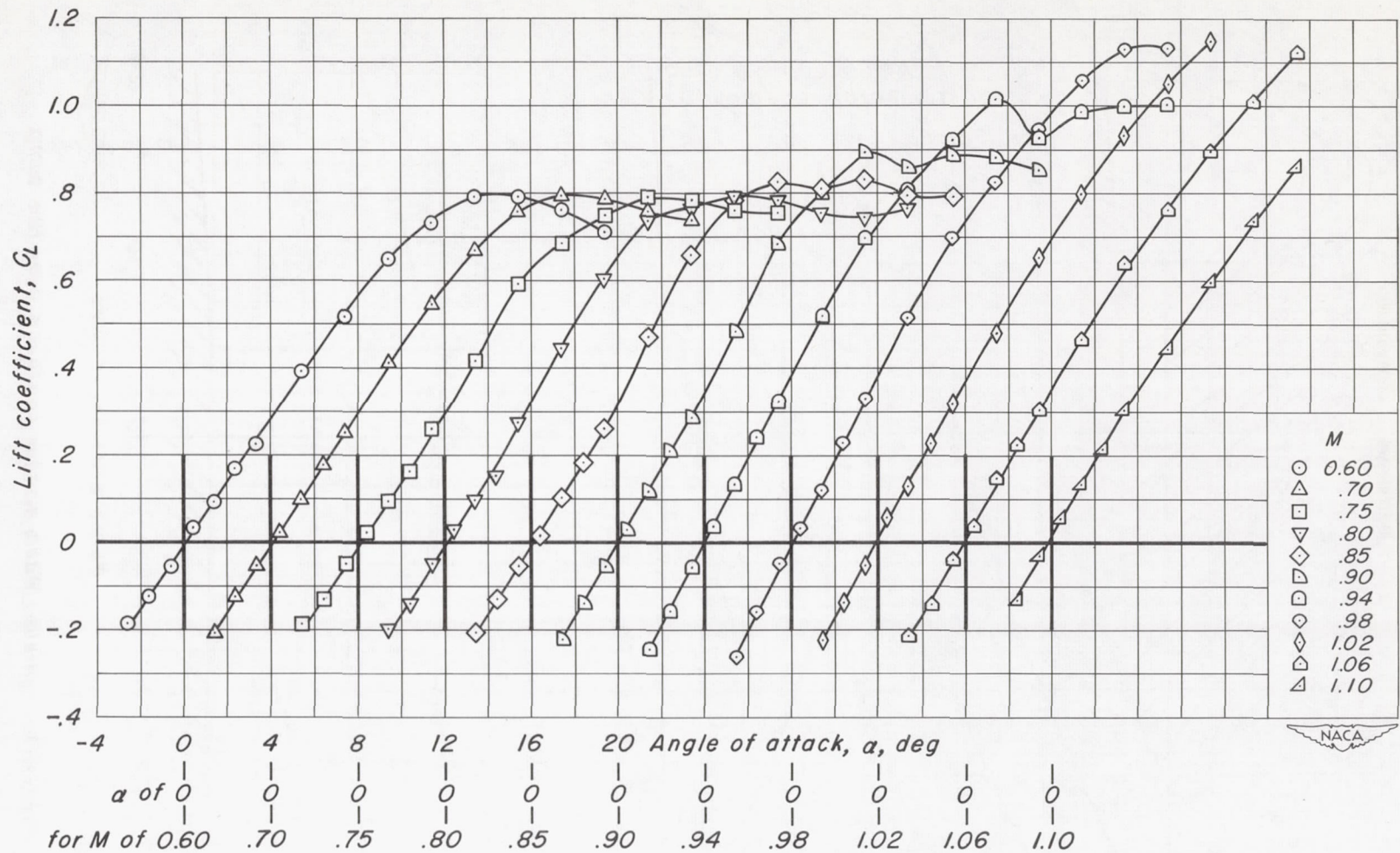
(a) Lift characteristics.
