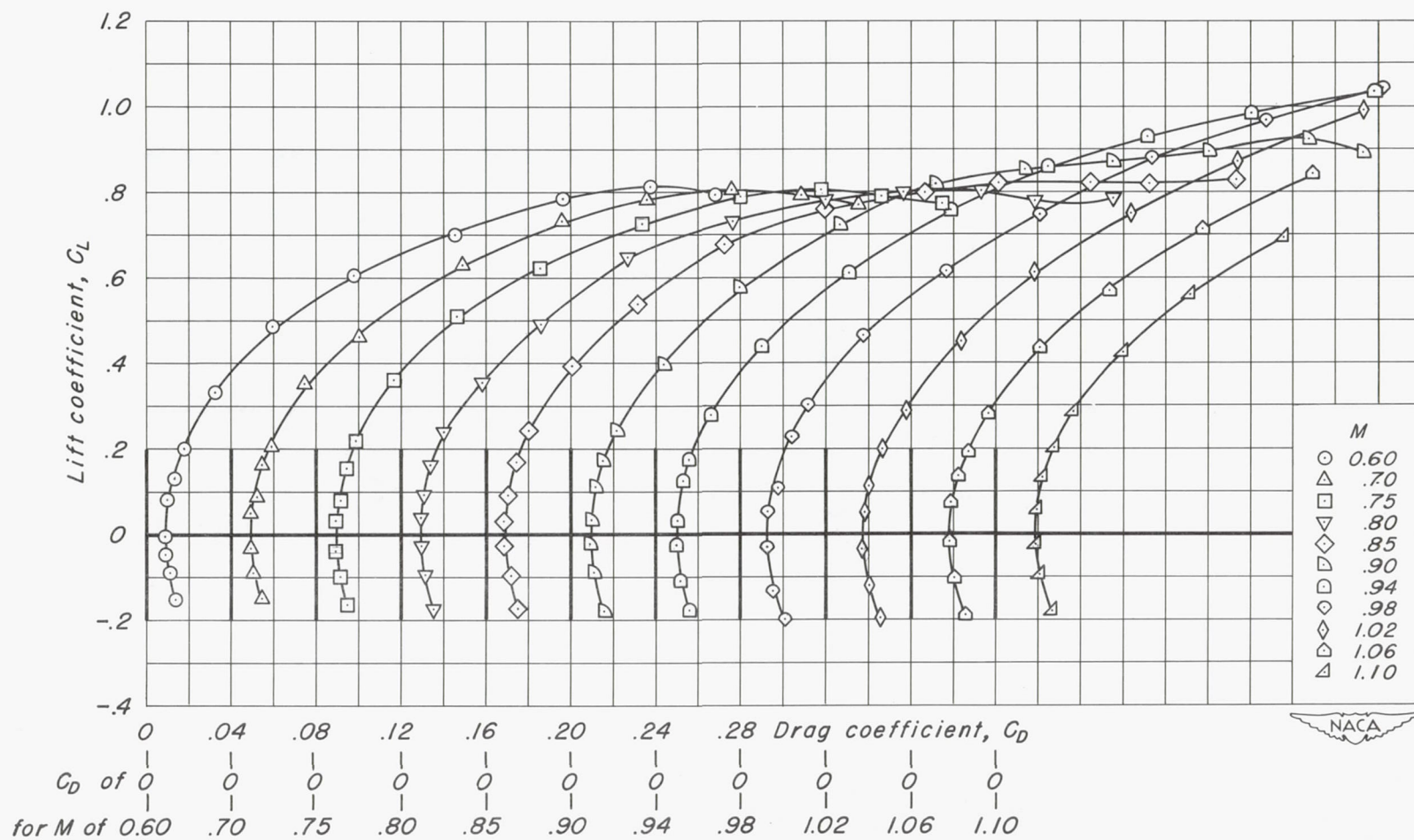
(c) Drag characteristics.
