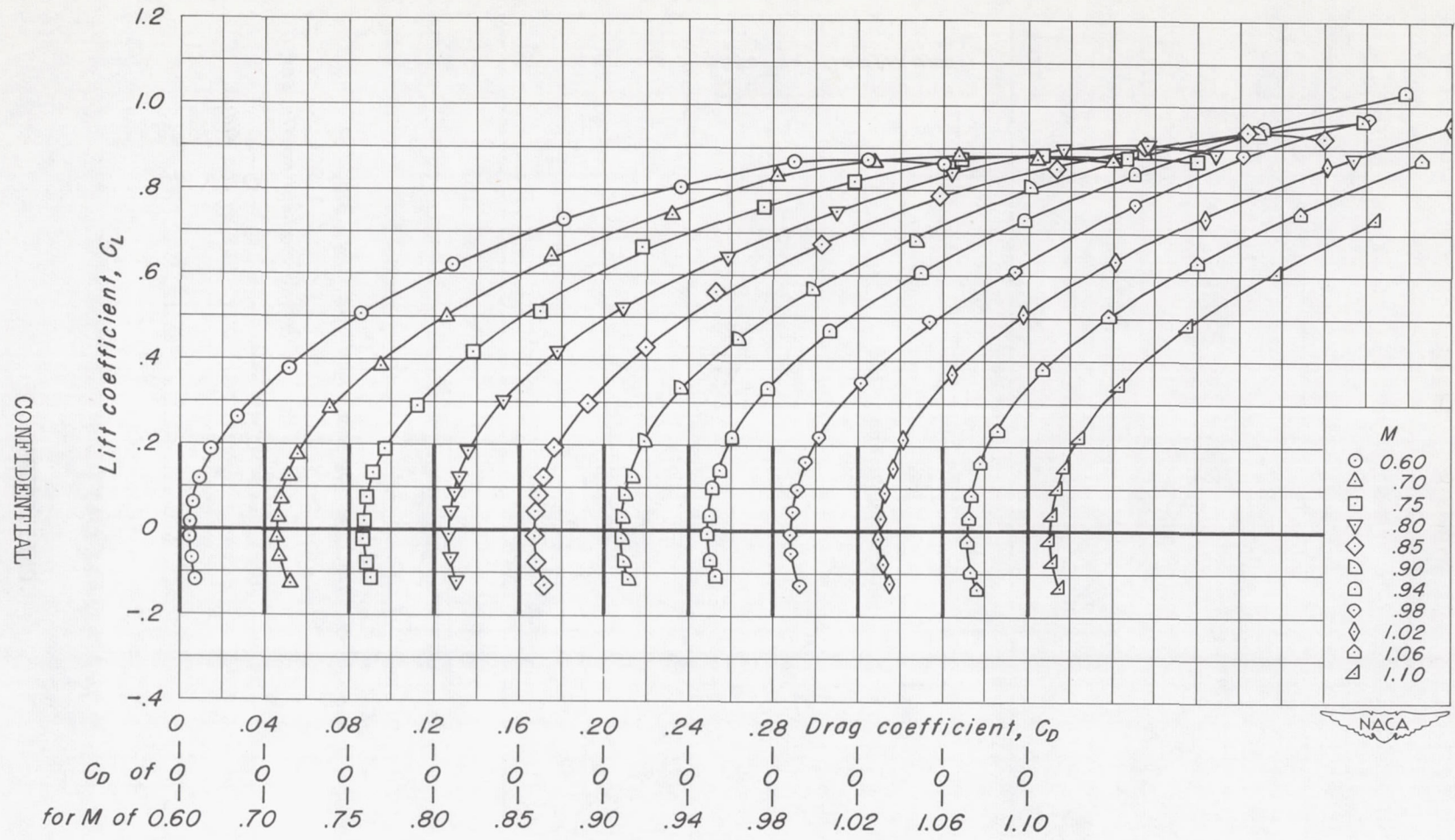
(c) Drag characteristics. Figure 7.- Concluded.
