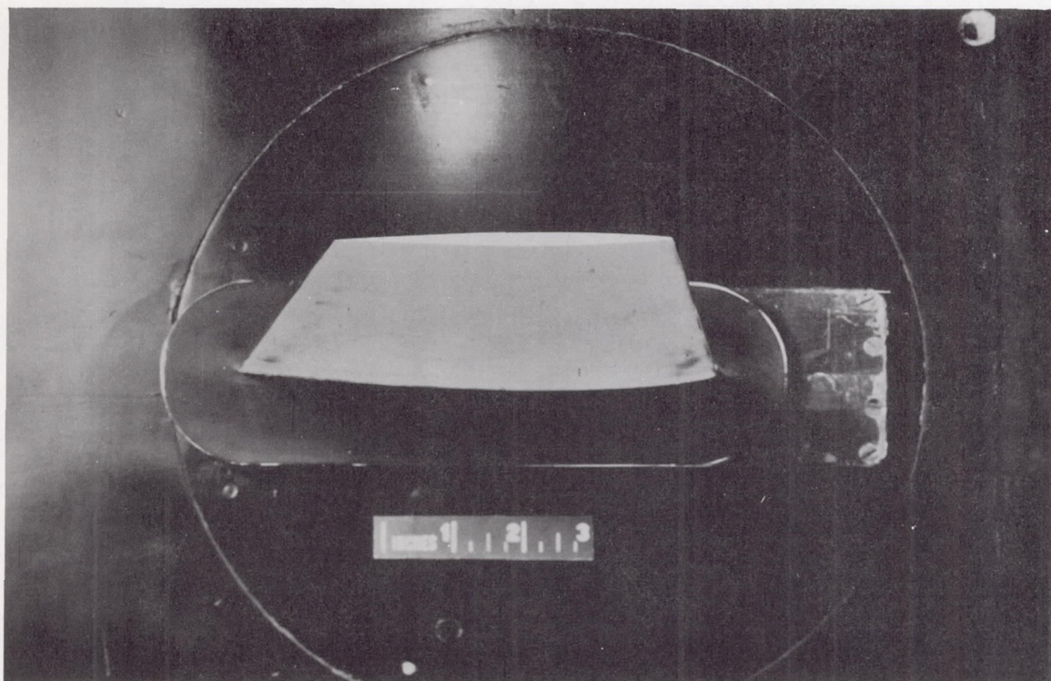
Figure 3.- The wing having an aspect ratio of 4 mounted on the transonic bump in the Ames 16-foot high-speed wind tunnel.
