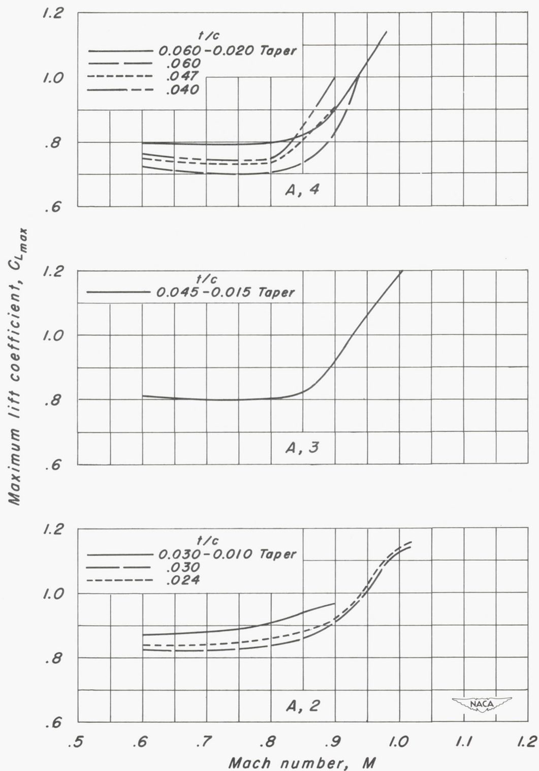
Figure 10.- The variation of maximum lift coefficient with Mach number.
