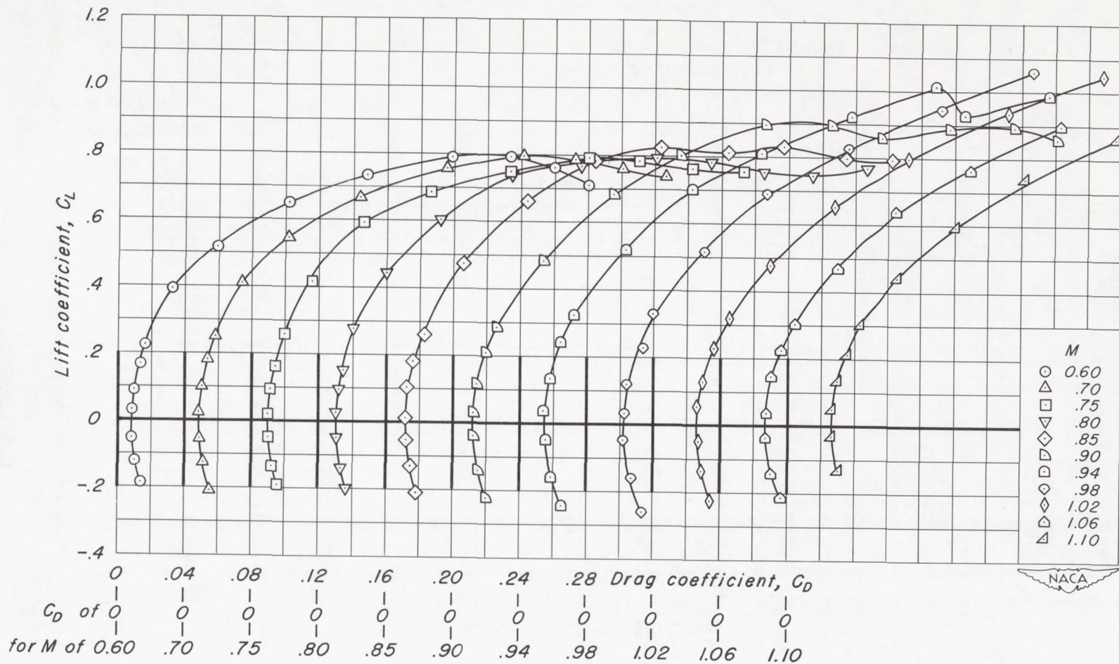
(c) Drag characteristics. Figure 5.- Concluded.
