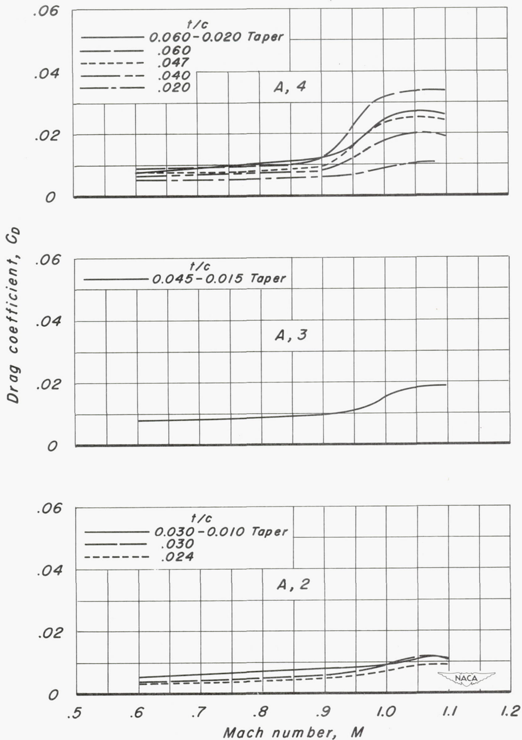
Figure 12.- The variation of drag coefficient with Mach number.
