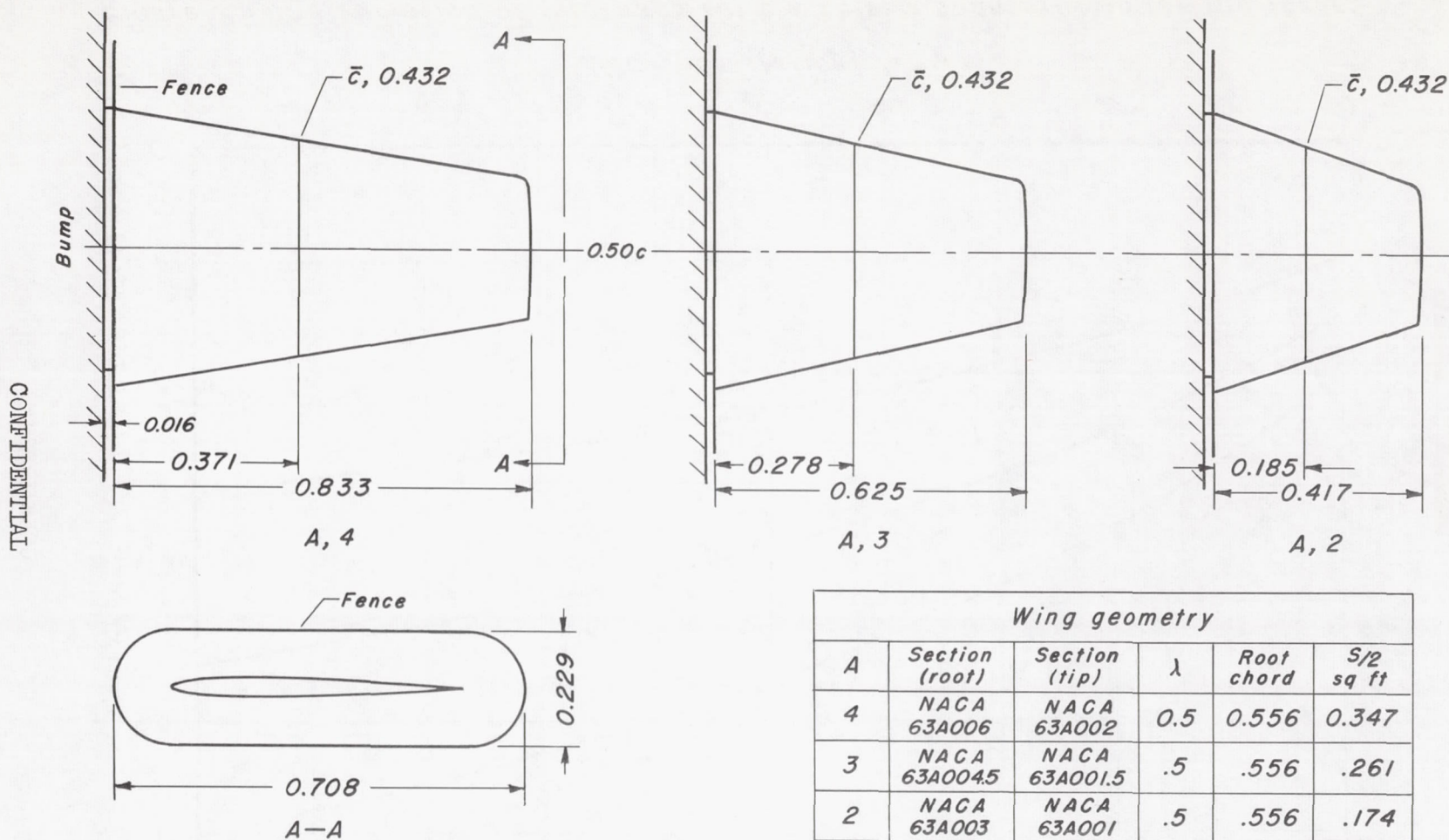
Figure 1.- Dimensions and plan forms of the three wings.
