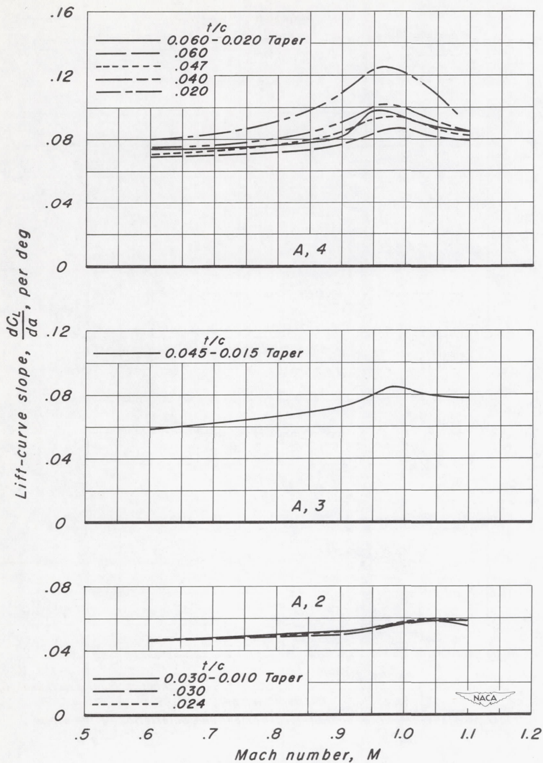
Figure 9.- The variation of lift-curve slope with Mach number. C_L = 0 .
