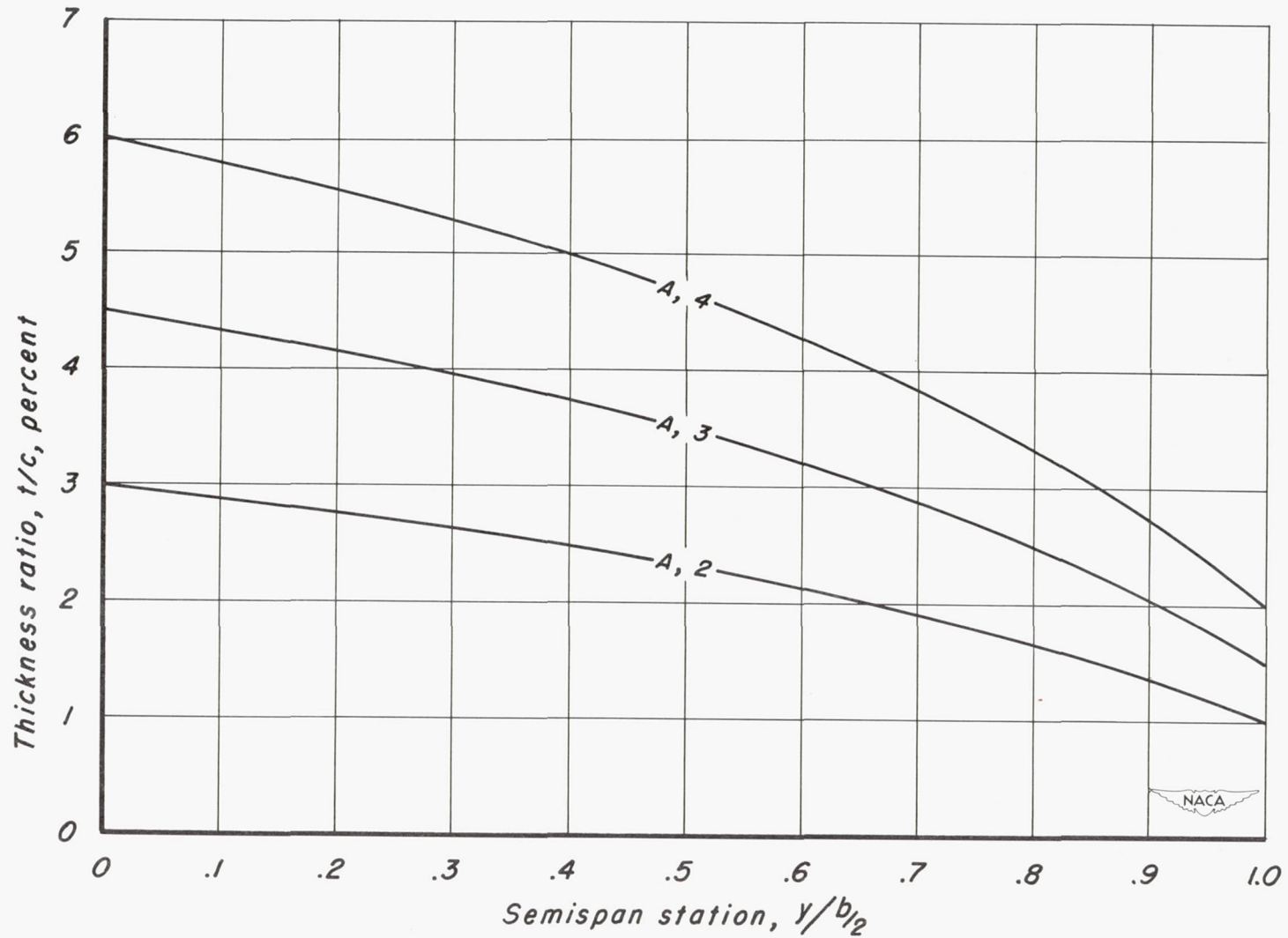
Figure 2.- The variation of thickness ratio with semispan station for the three wings.
