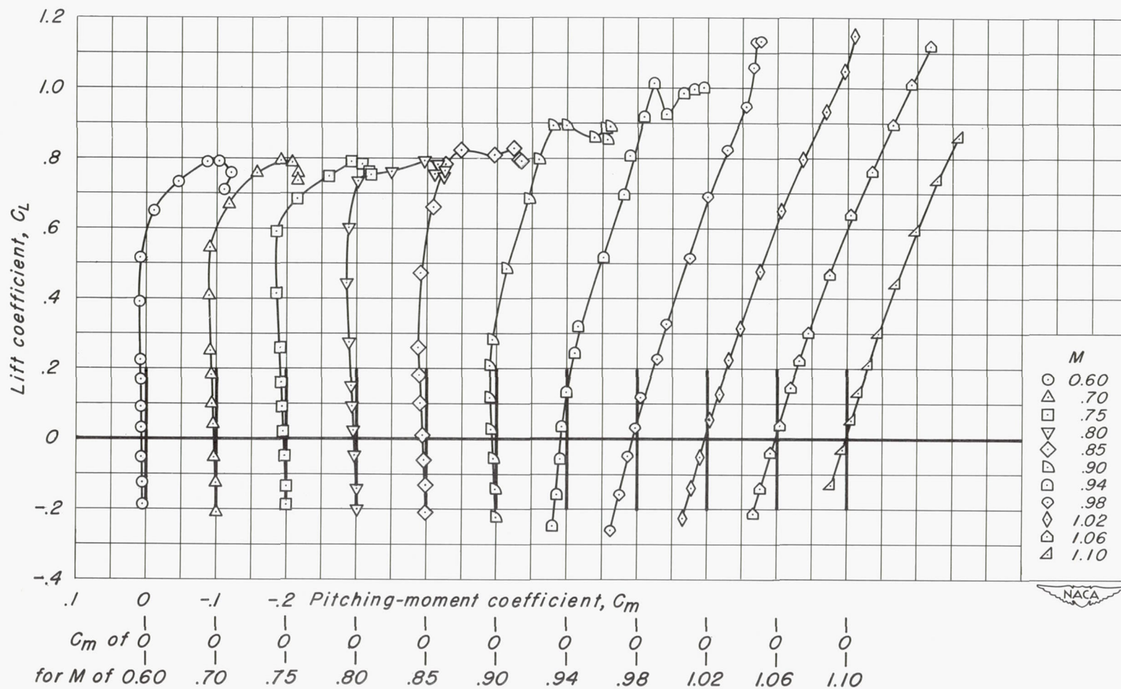
(b) Pitching-moment characteristics.
