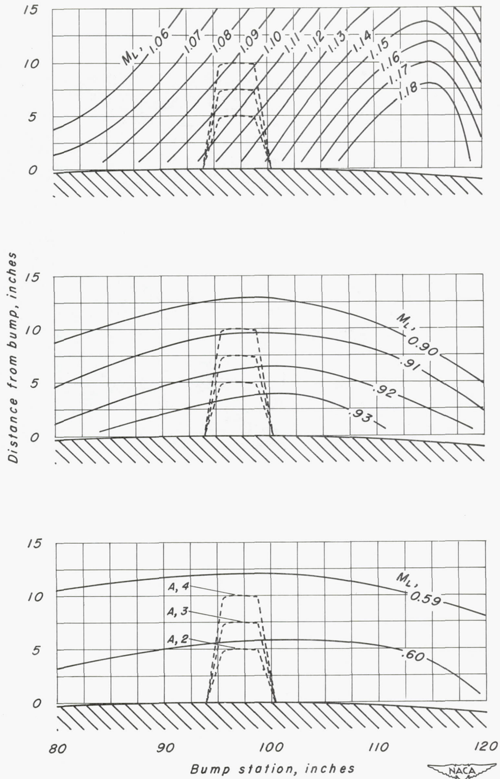
Figure 4.- Typical Mach number contours over the bump.
