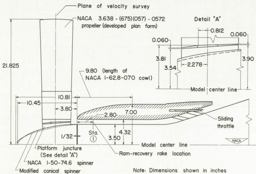
Figure 2.- Model arrangement.
