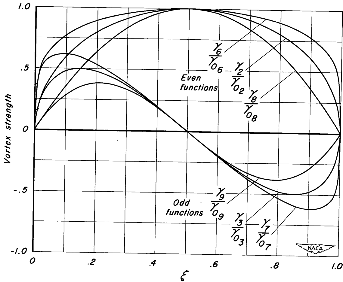
Figure 13.-Vortex distributions.
