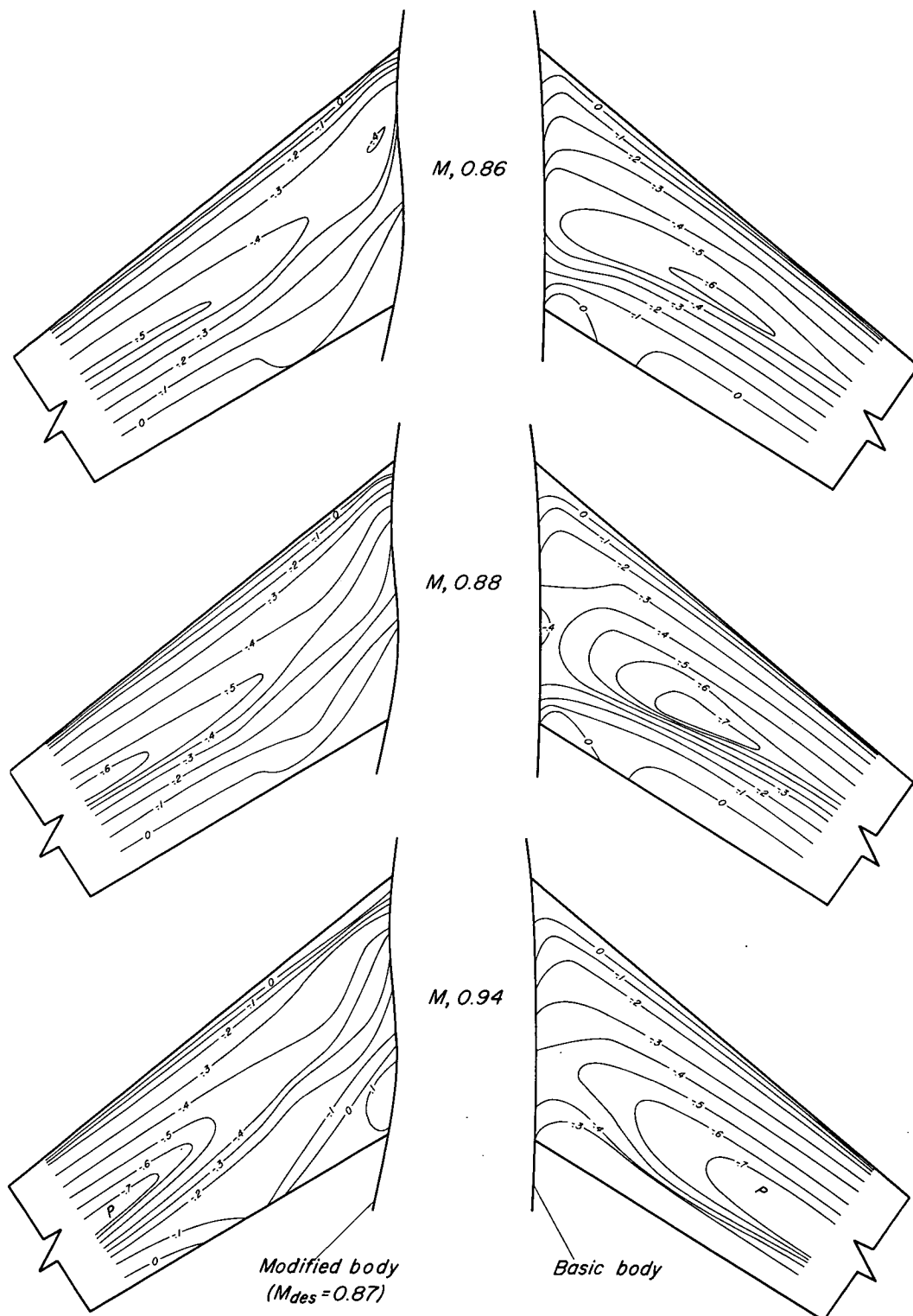
Figure 10.—Lines of constant pressure on the sweptback wing in combination with basic and modified bodies at zero lift.
