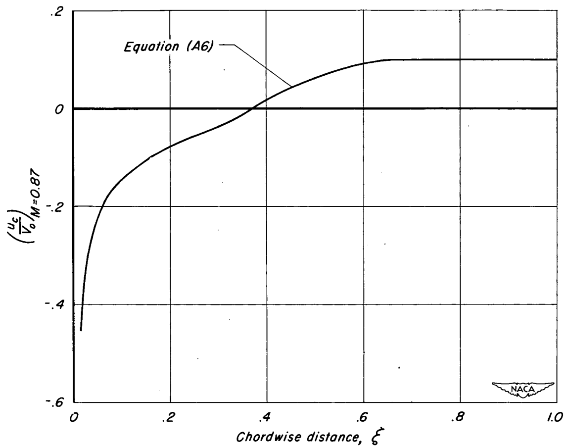
Figure 12.- Distortion velocity at the root of a 35° sweptback, untapered wing having 64 2 AO15 sections normal to the leading edge (Mach number of 0.87).
