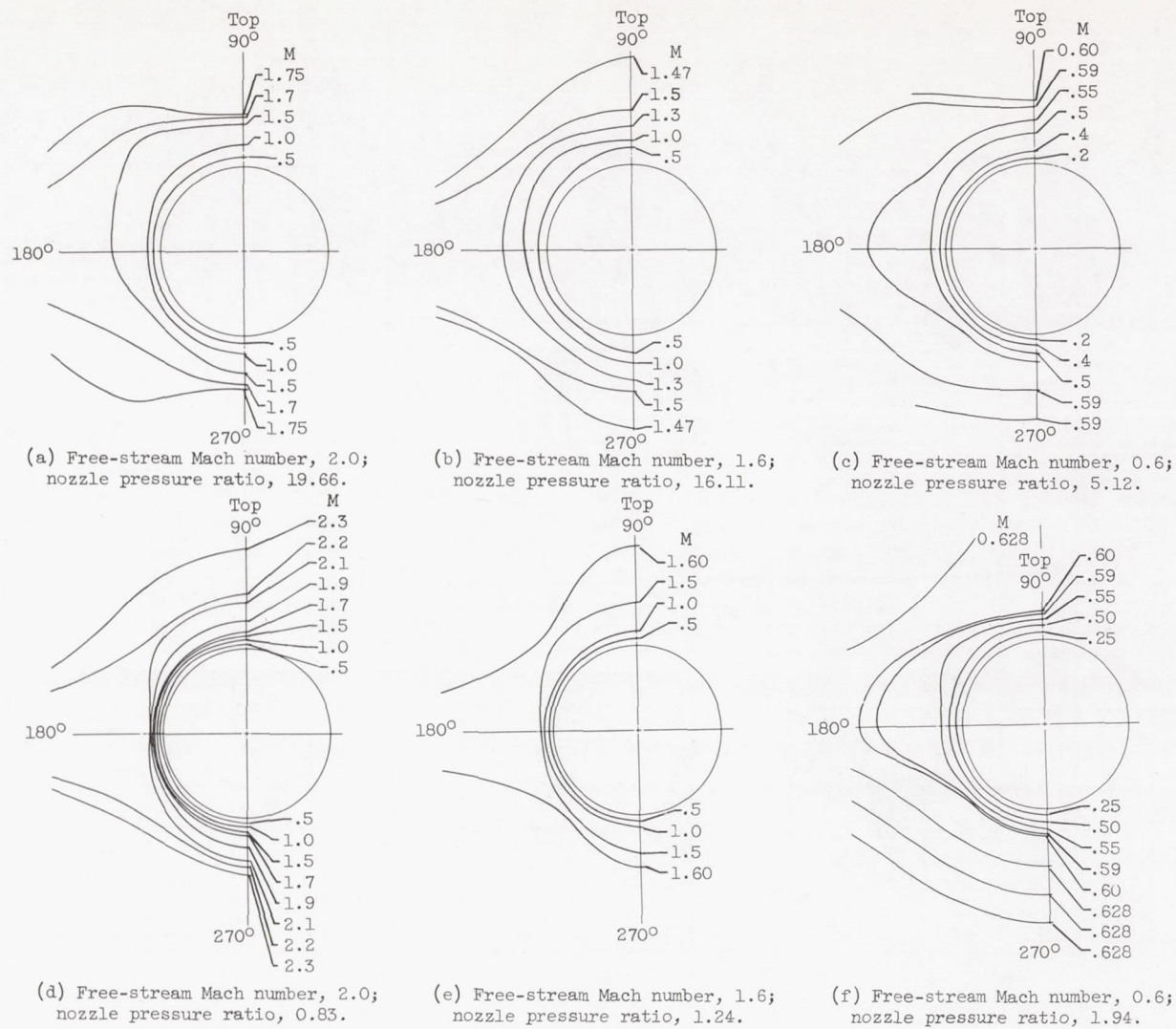
Figure 8. - Contour maps of Mach number M taken at wake survey station. Nozzle B; zero angle of attack.
