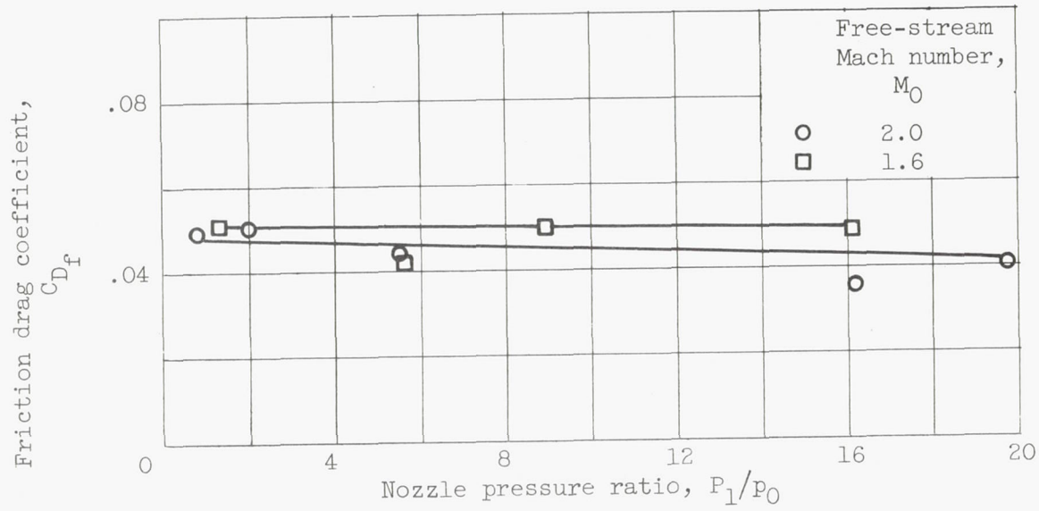
Figure 7. - Effect of jet interference on friction drag coefficient.
