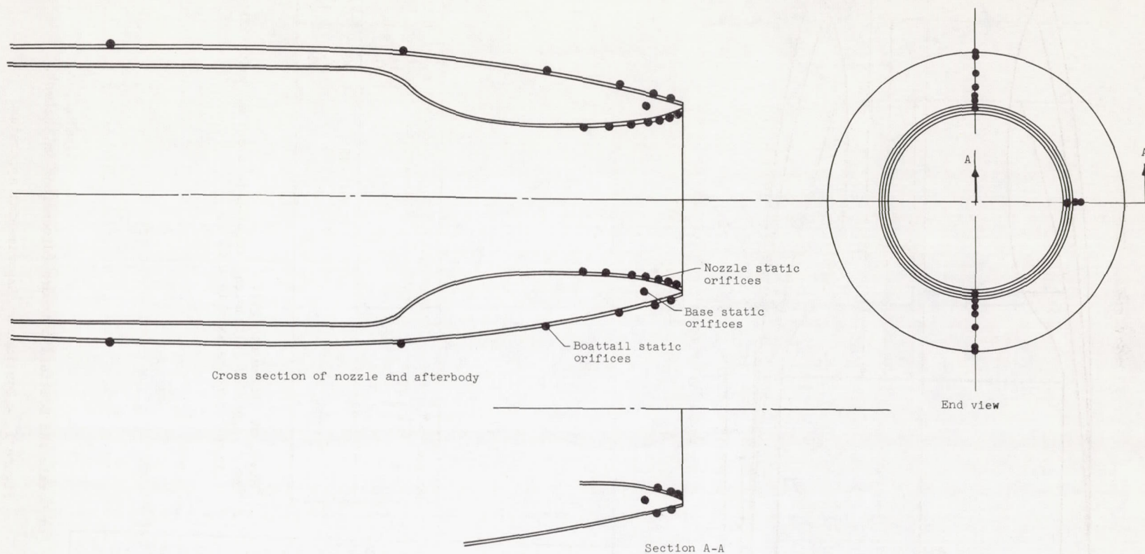
(d) Location of pressure-measuring orifices on nozzle and afterbody.
