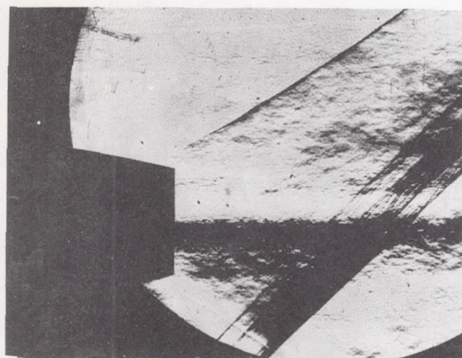
(c) Free-stream Mach number, 1.6; nozzle pressure ratio, 1.09.
