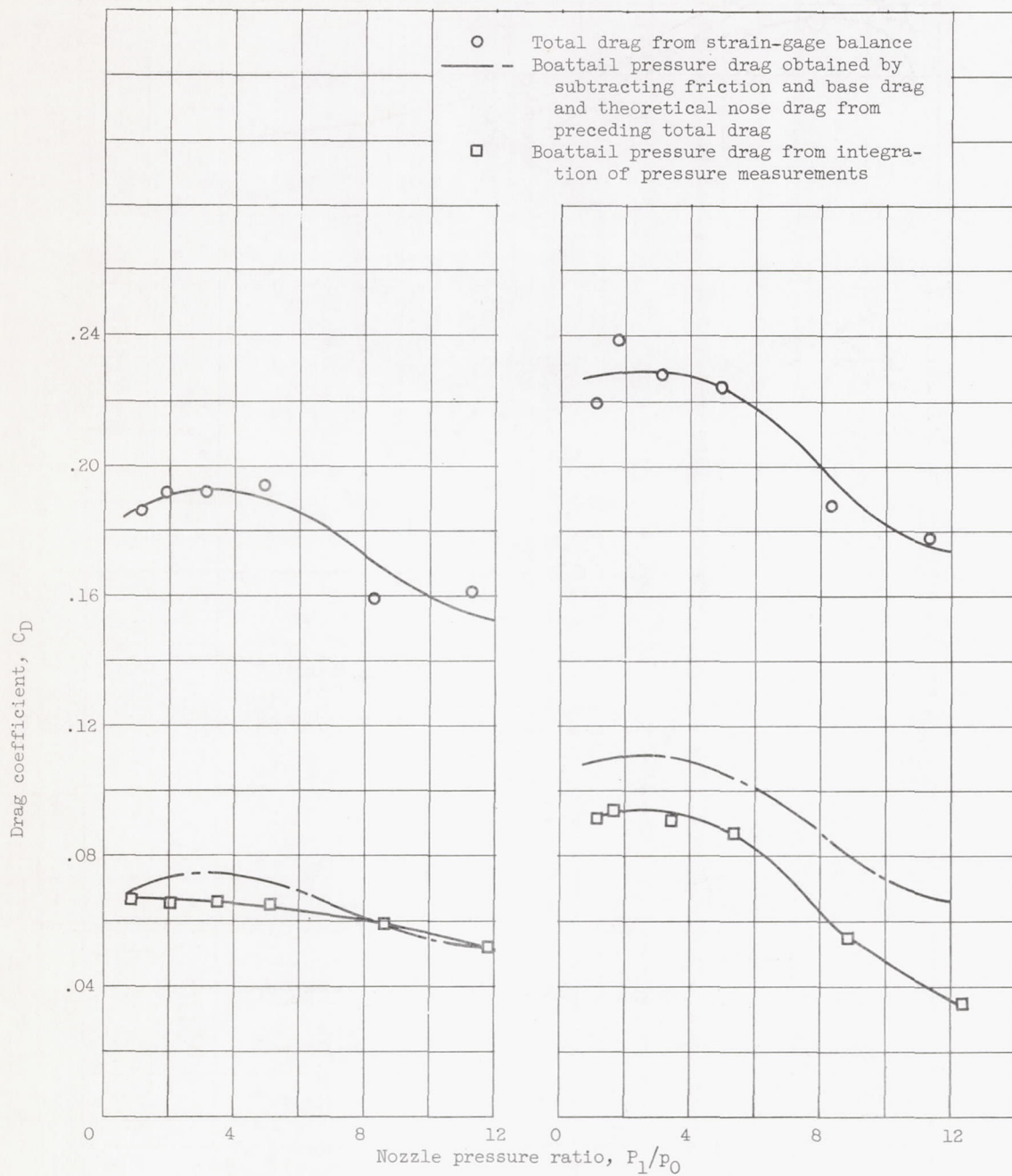
Figure 10. - Comparison of boattail pressure drag obtained from two independent methods for convergent-divergent nozzle B.
