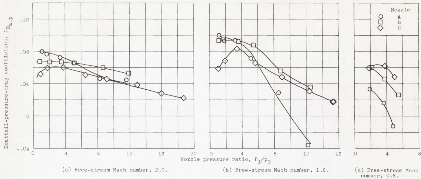
Figure 2. - Effect of jet interference on boattail-pressure-drag coefficient at zero angle of attack.
