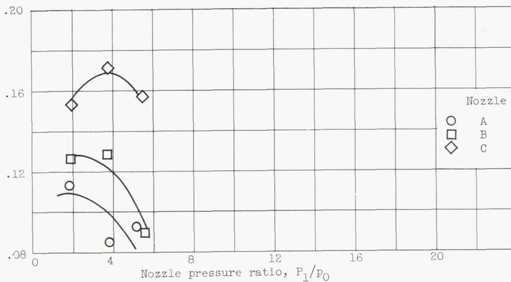
(c) Free-stream Mach number, 0.6.
