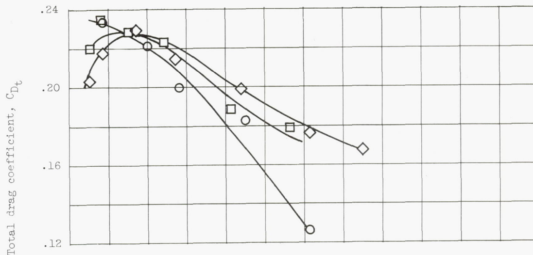
(b) Free-stream Mach number, 1.6.
