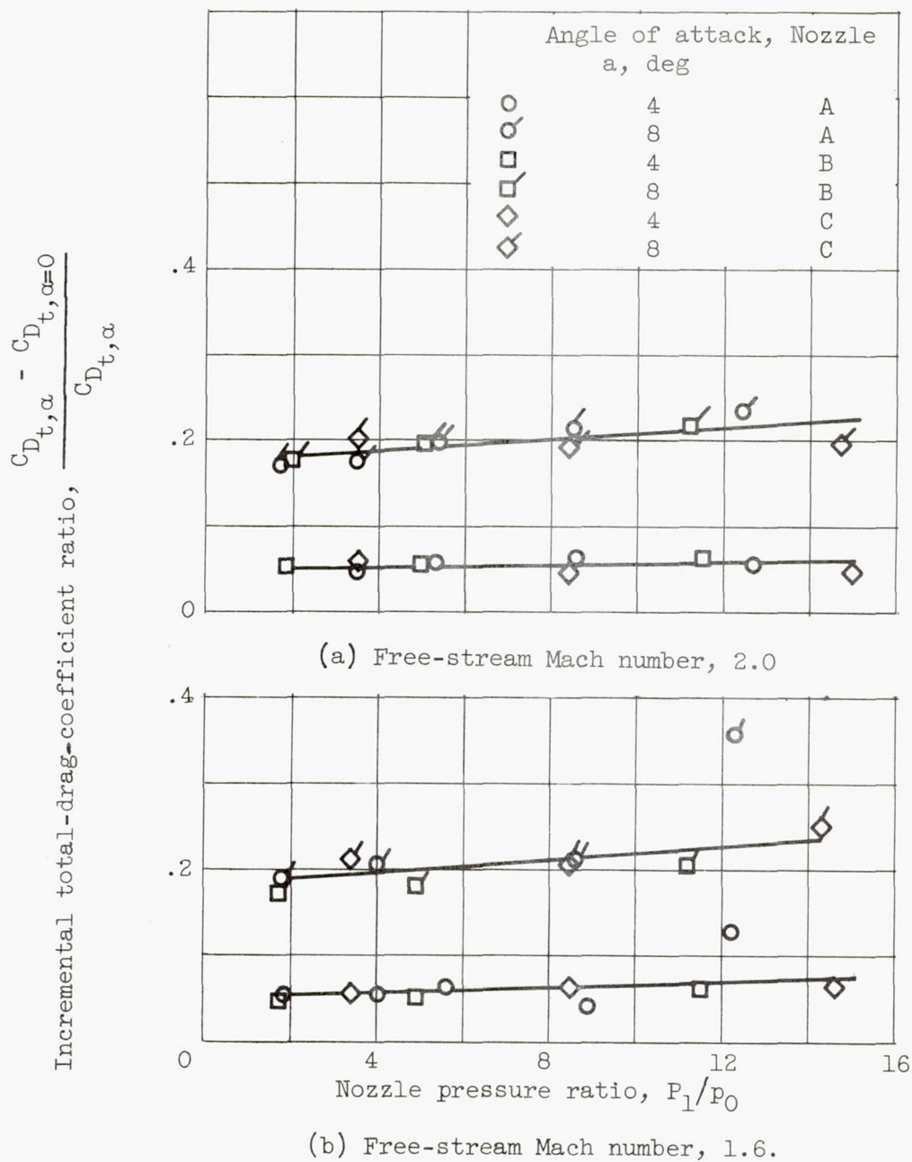
Figure 11. - Effect of jet interference on total drag at angle of attack.
