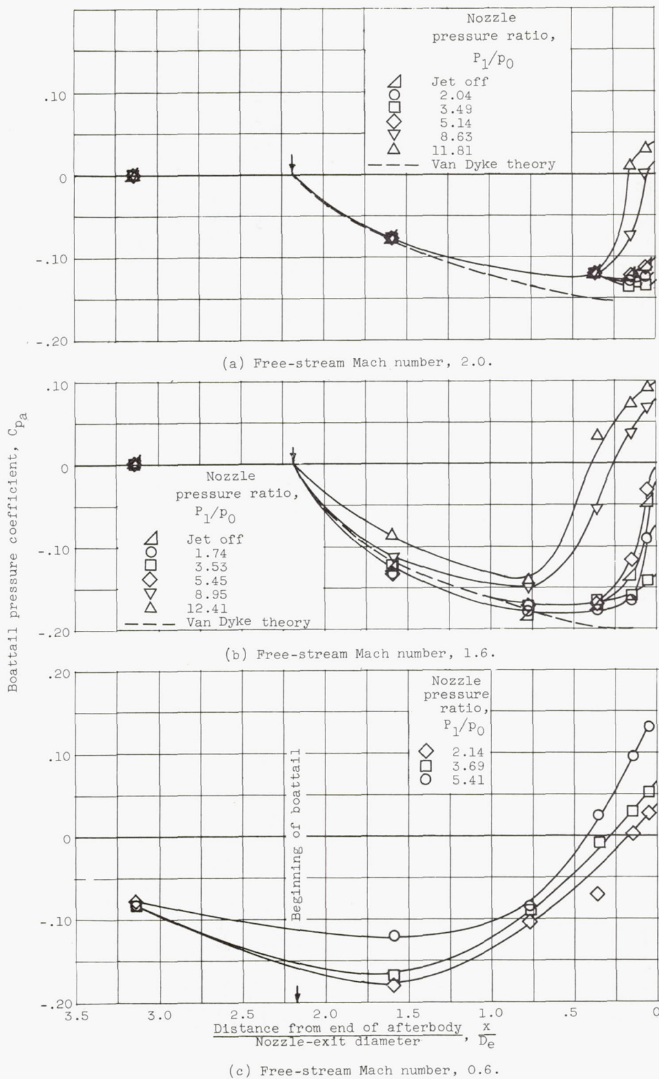
Figure 3. - Effect of jet interference on pressure distribution for convergent-divergent nozzle B.
