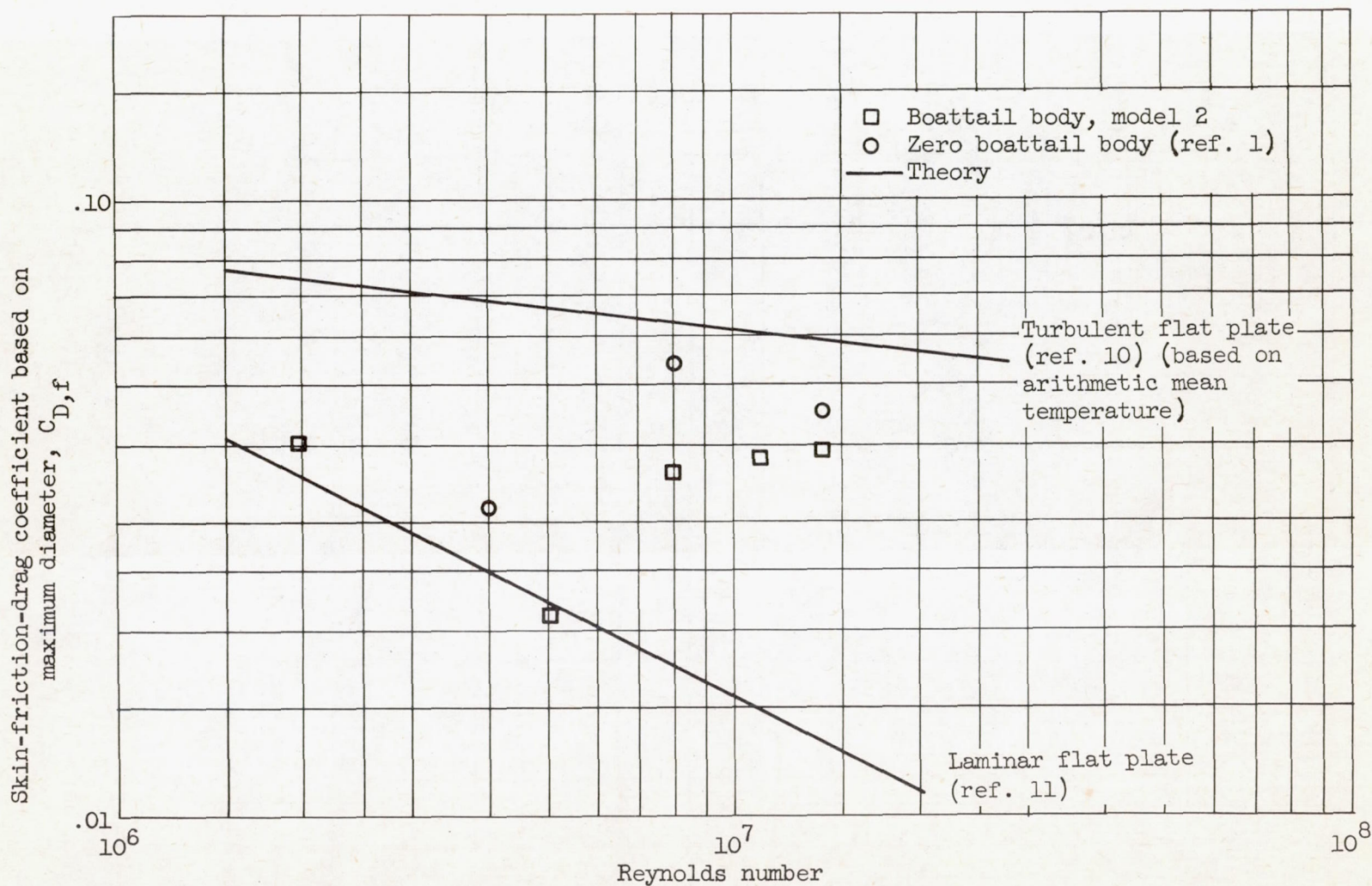
Figure 10. - Comparison of skin-friction drag between boattailed model 2 and zero boattailed body of reference 1.
