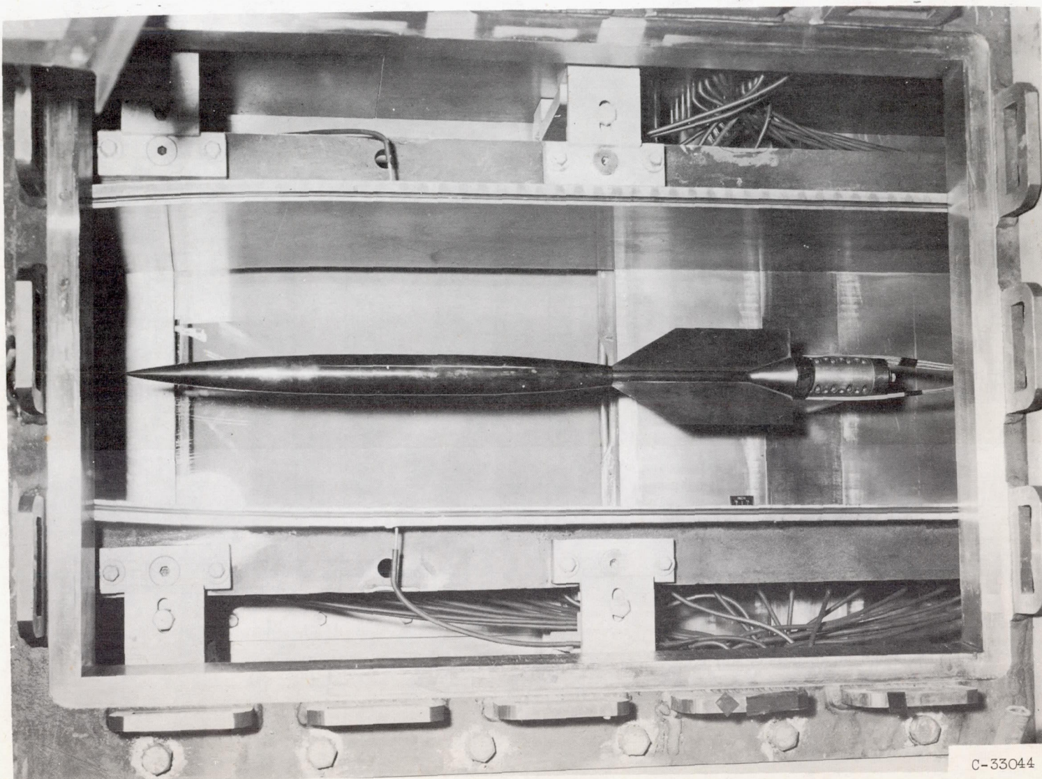
Figure 2. - Representative model 2 installed in Lewis 1- by 1-foot supersonic tunnel.
