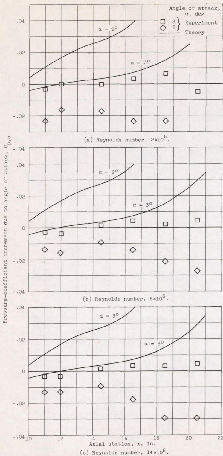
Figure 7. - Effect of Reynolds number on top surface pressure distribution of model 2 for two angles of attack, meridian angle, 180^\circ .
