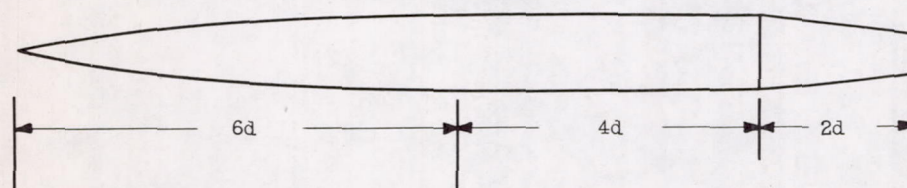
Figure 1. - Schematic drawing of models. Maximum body diameter d , 1.75 inches.
