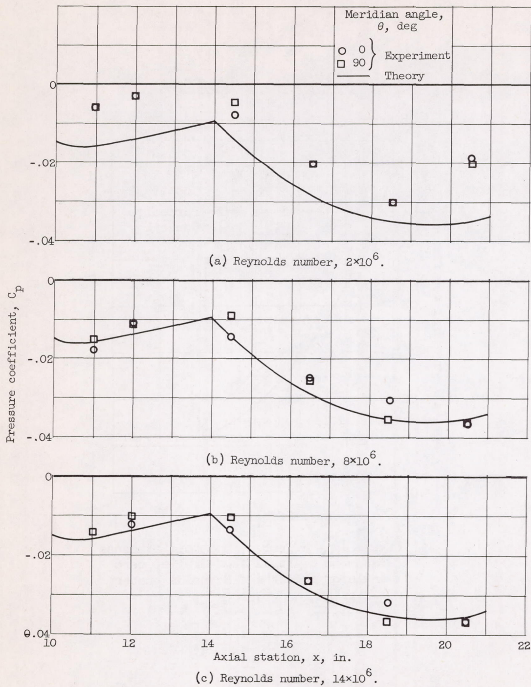
Figure 5. - Effect of Reynolds number on boattail pressure distribution for model 2 at zero angle of attack.
