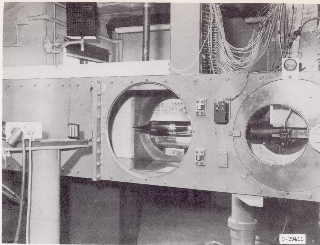
(a) Isentropic inlet installed in 2- by 2-foot supersonic tunnel.
