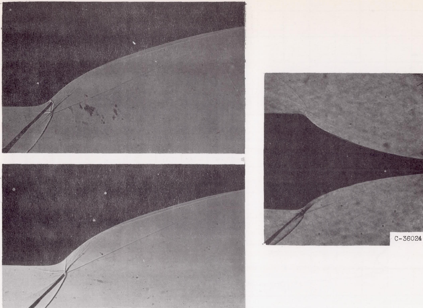
Figure 5. - Typical photographs showing probe in flow field of original isentropic spike.
