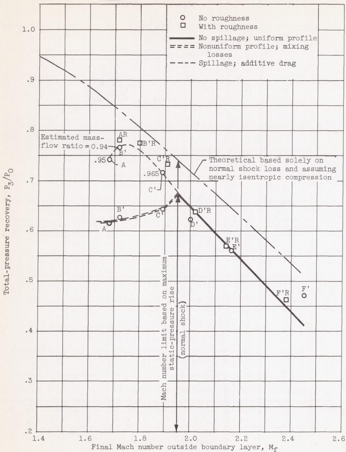
Figure 14. - Summary of potential pressure recoveries available for all-external-compression inlets designed to accommodate flow fields of various isentropic spikes.
