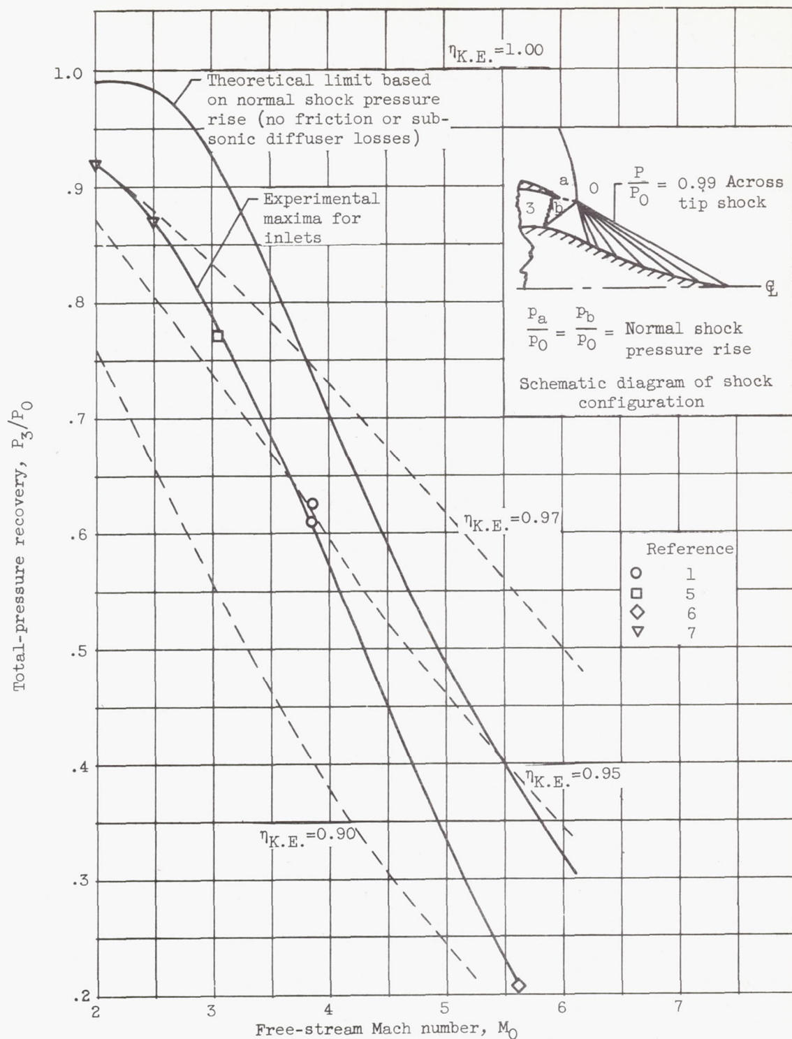
Figure 15. - Comparison of current experimental maximum recoveries with theoretical limits for all-external-compression isentropic inlets at several Mach numbers.
