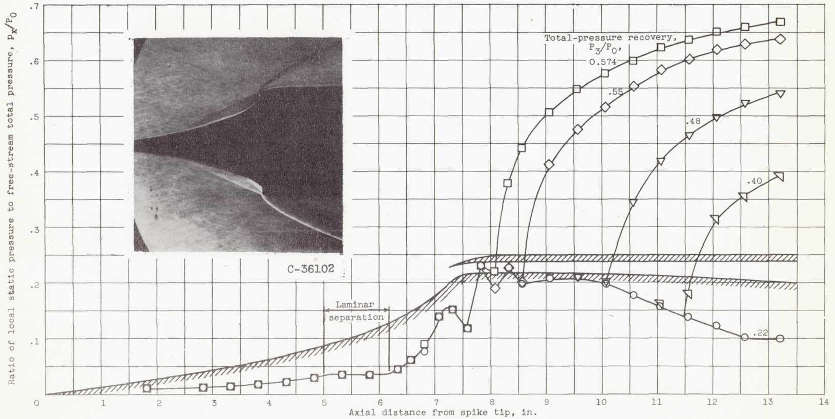
Figure 2. - Static-pressure distributions along spike of isentropic inlet for several supercritical operating conditions. Zero angle of attack and no tip roughness.
