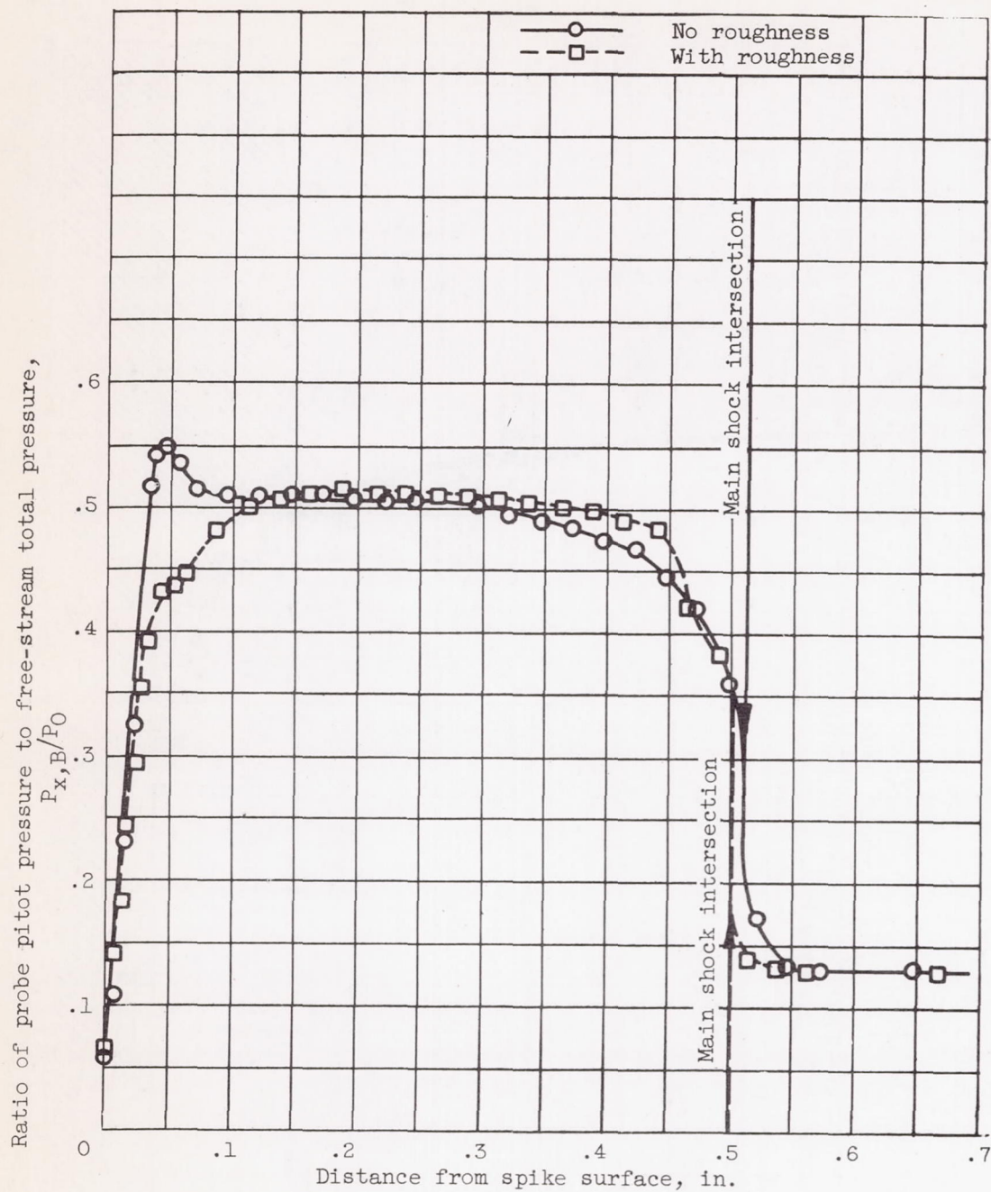
(f) Configurations F' and F'(R).
