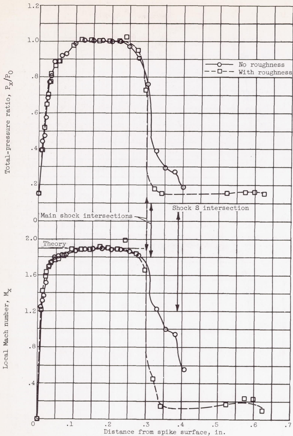
(c) Configurations C' and C'(R).
