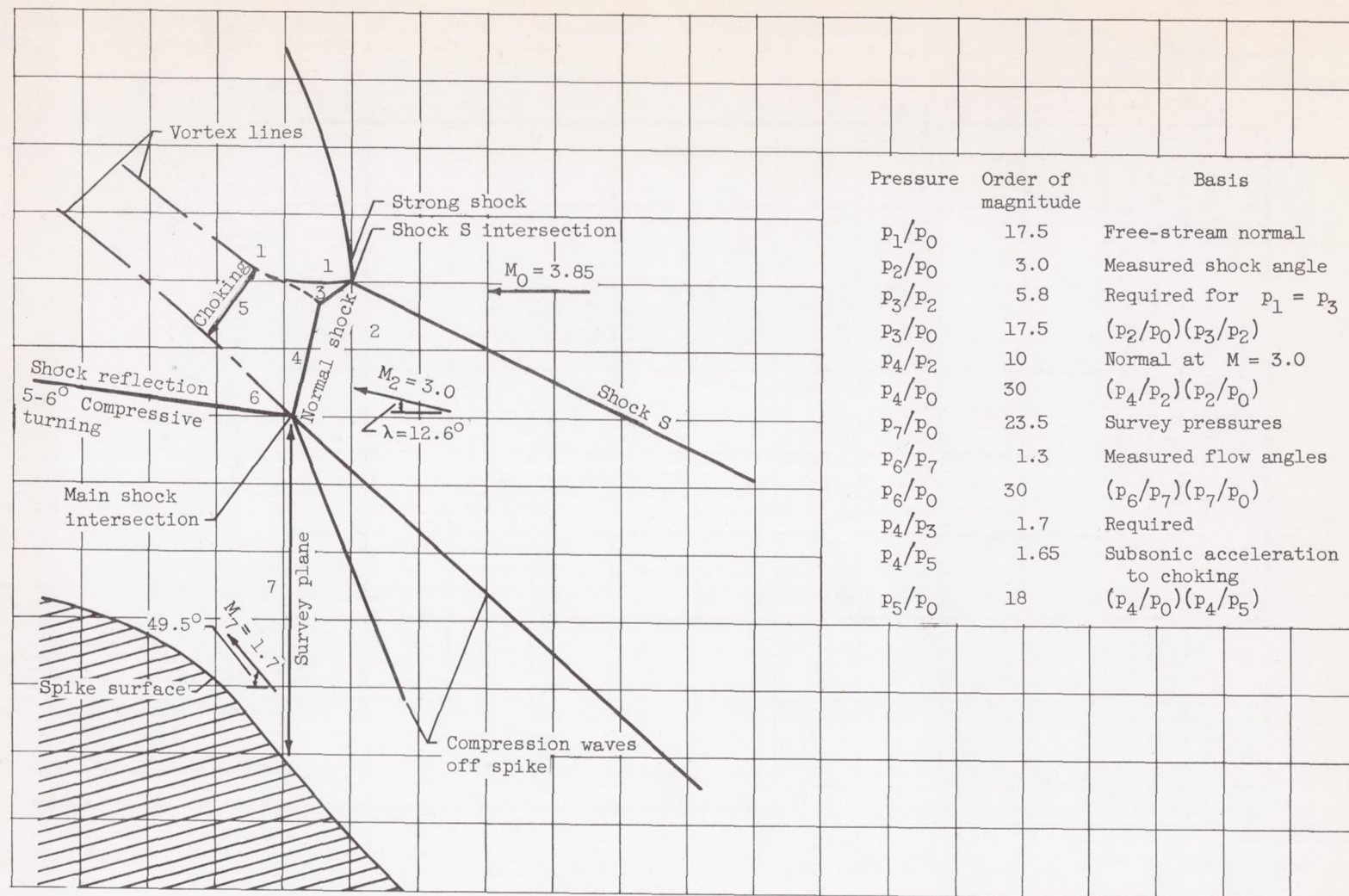
Figure 12. - Experimental and analytical approximation of shock structure and flow fields obtained for configuration A of isentropic survey spike.
