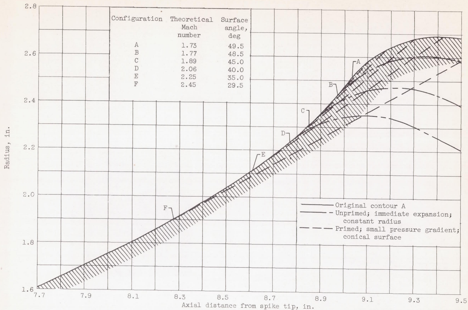
(g) Isentropic survey spike configurations.
