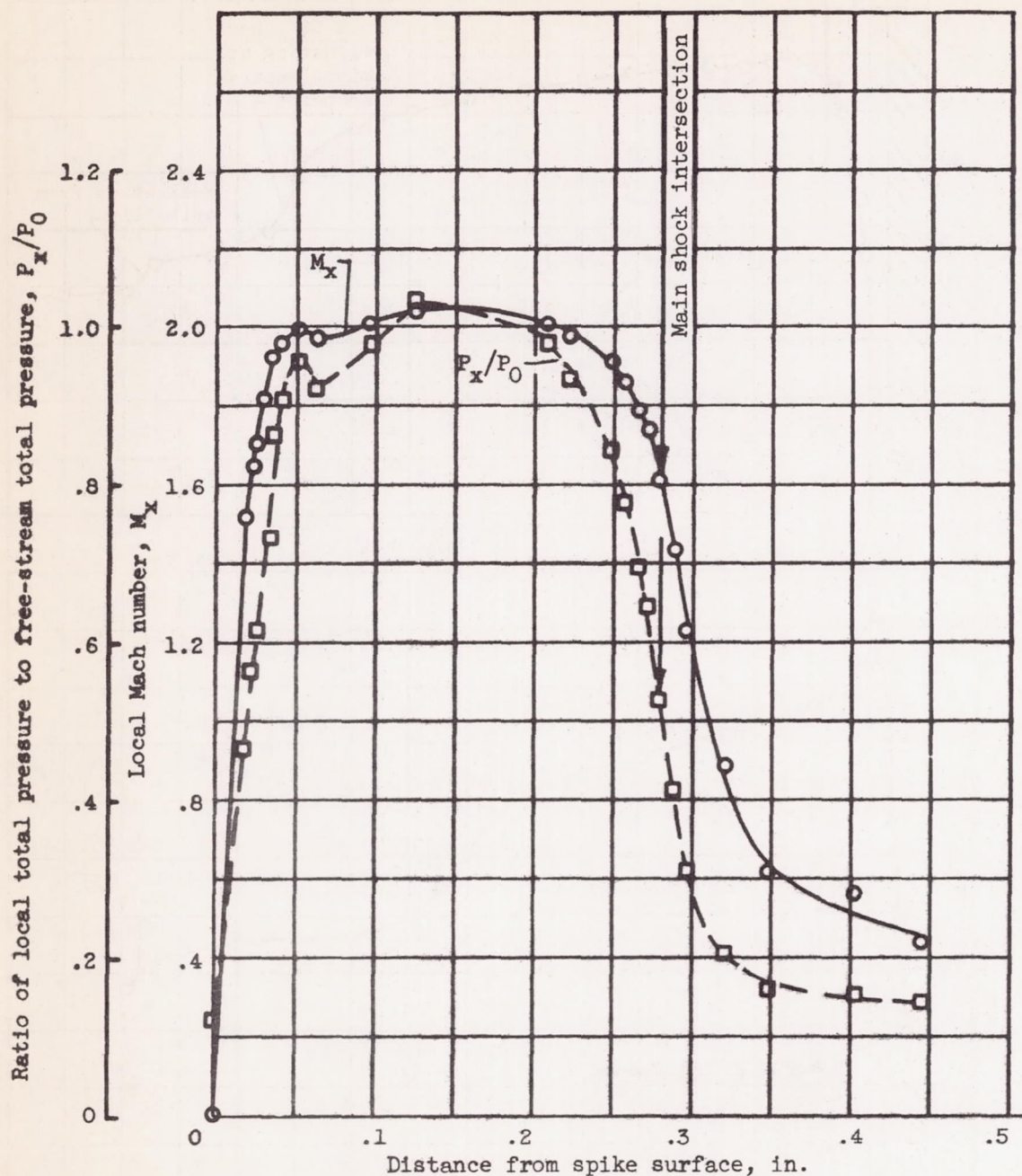
(b) Mach number and total-pressure profiles.
