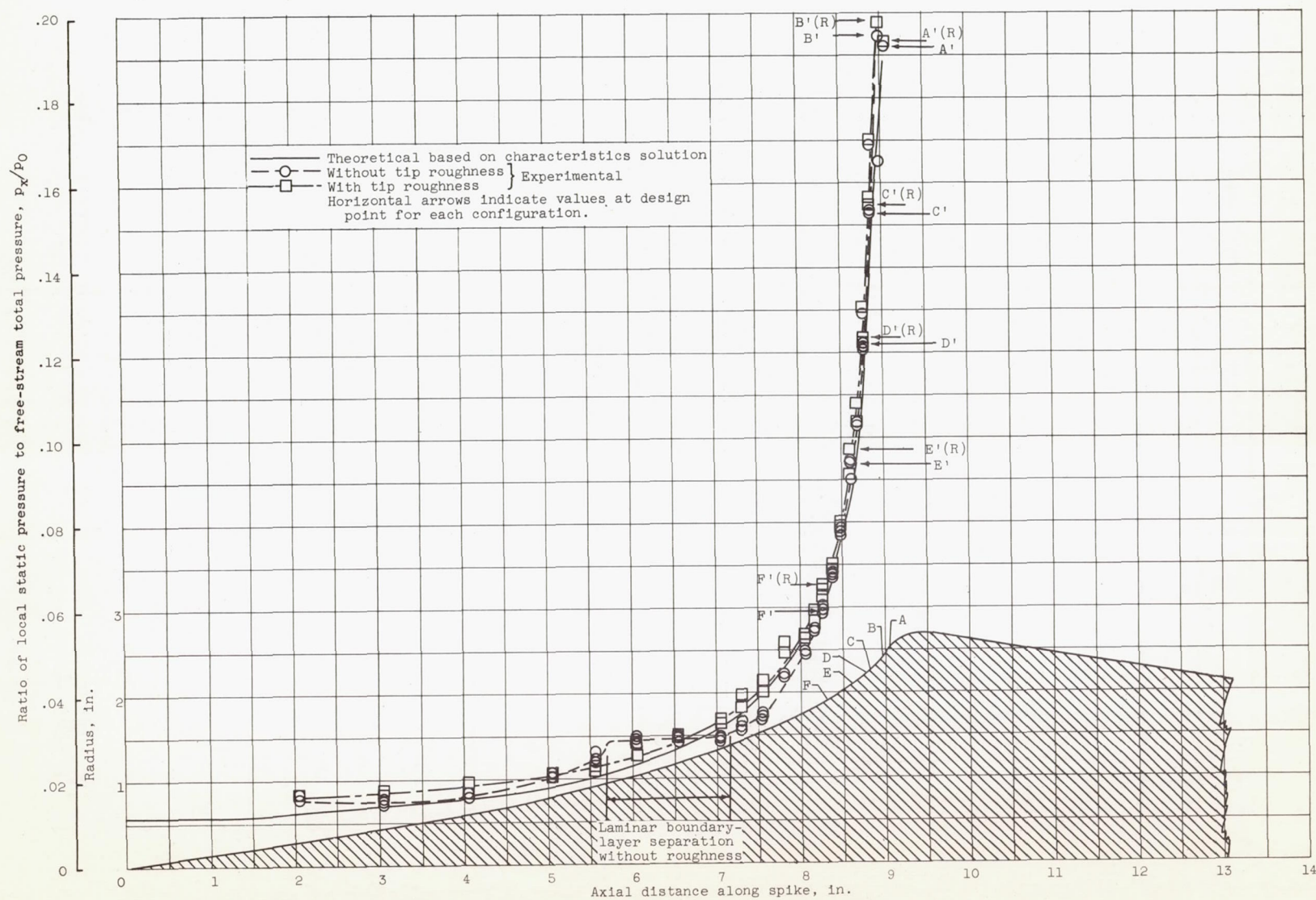
Figure 10. - Static-pressure distributions along surfaces of various isentropic survey-spike configurations.
