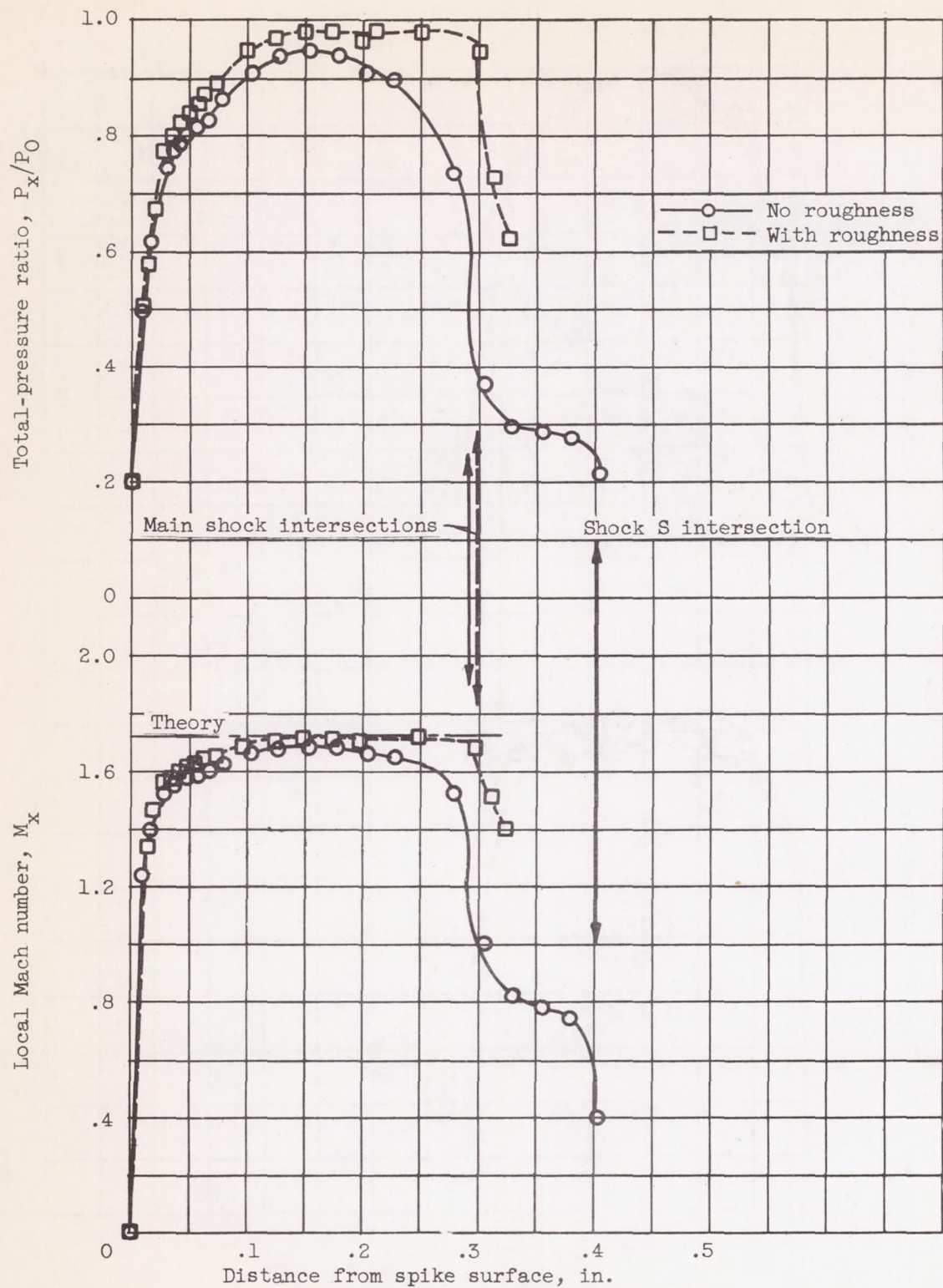
(a) Configurations A and A(R).
