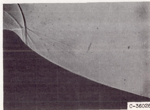
With tip roughness
