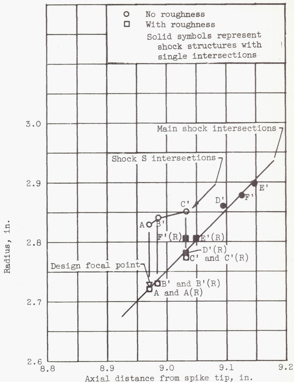
Figure 13. - Relative positions of shock intersections encountered in survey plane.
