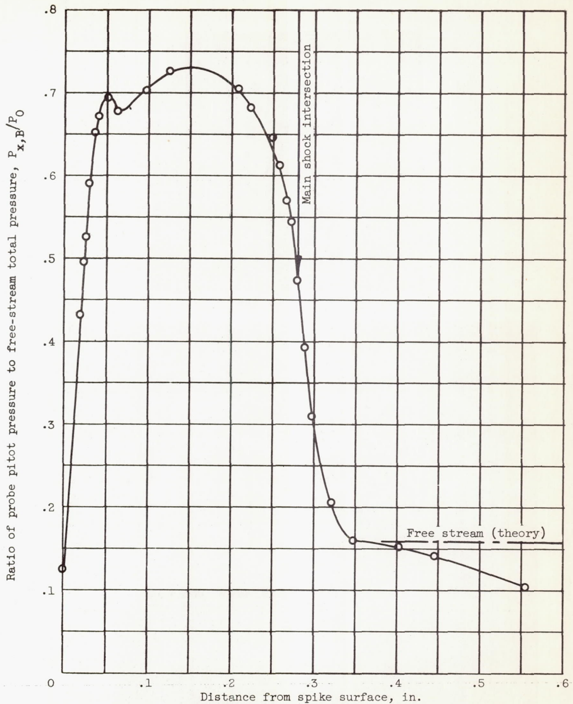
(a) Pitot-pressure profile.
