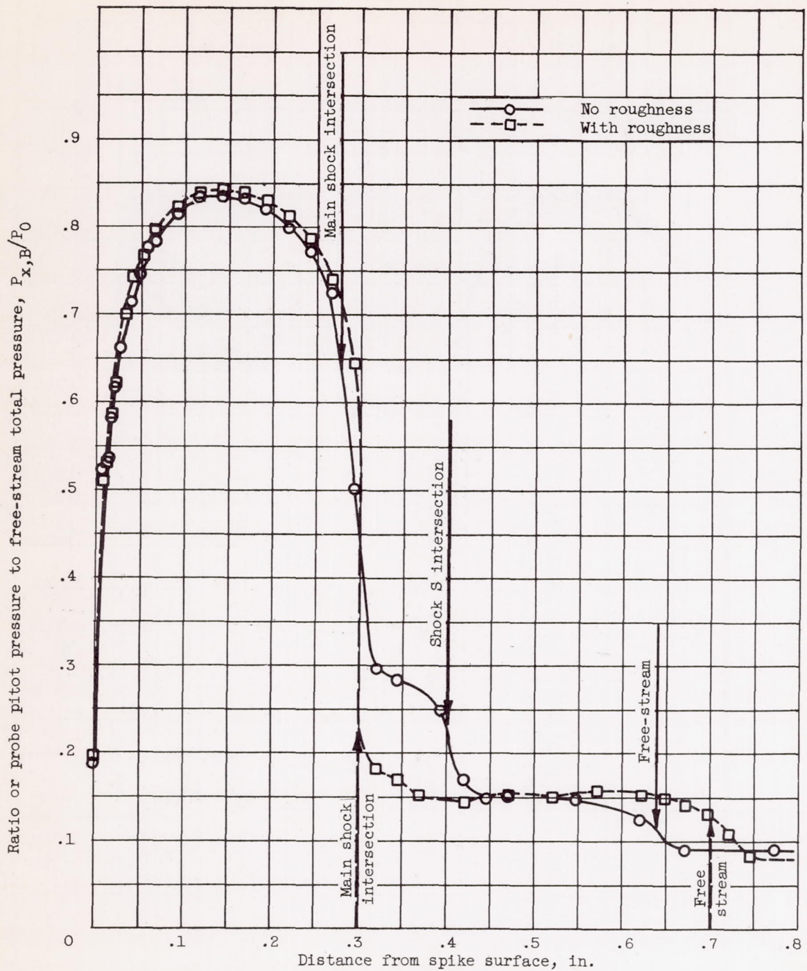
(b) Configurations B' and B'(R).
