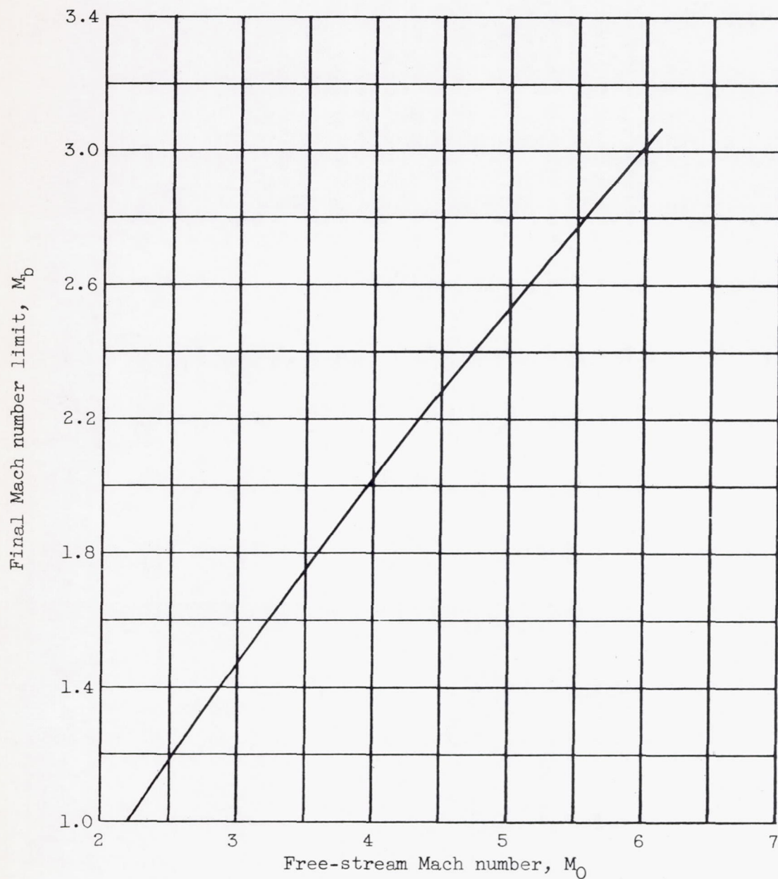
Figure 16. - Effect of free-stream Mach number on final Mach number limit.
