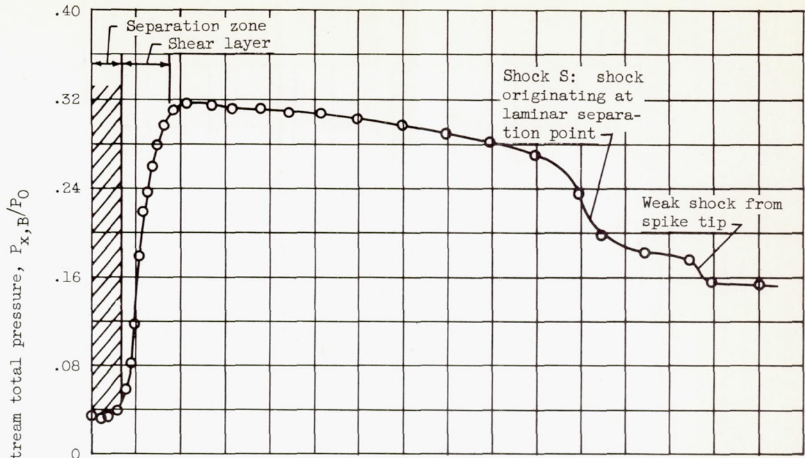
(a) No roughness.
