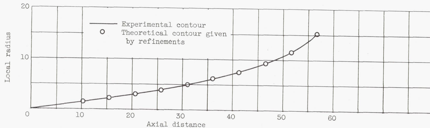
(e) Isentropic spike contours plotted in arbitrary units.
