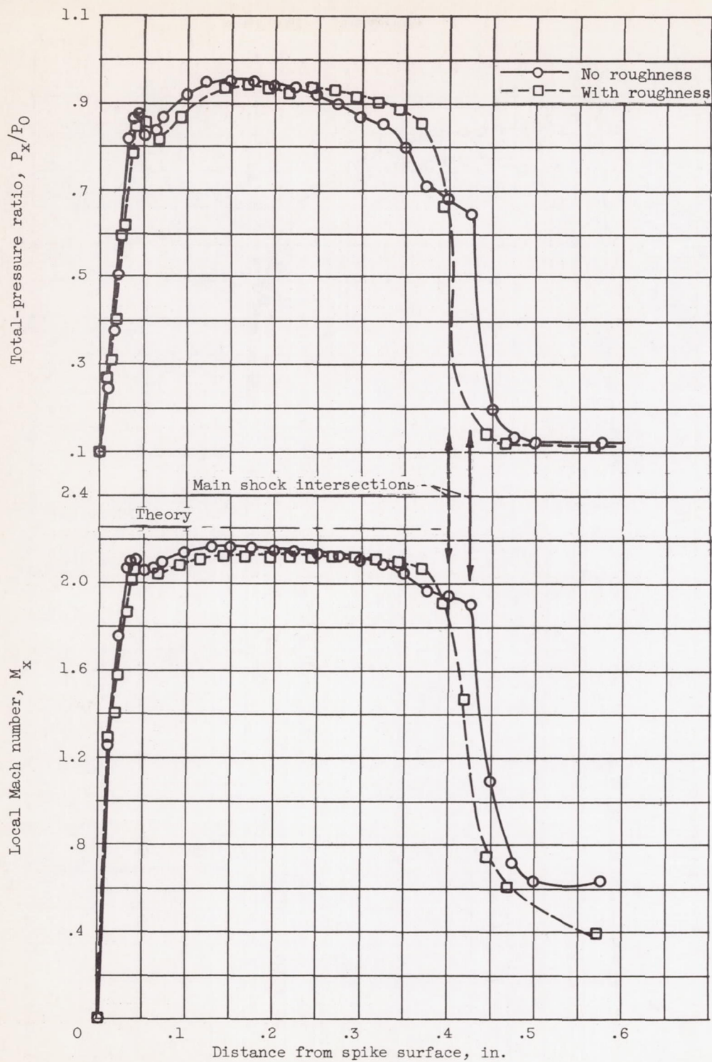
(e) Configuration E' and E'(R).
