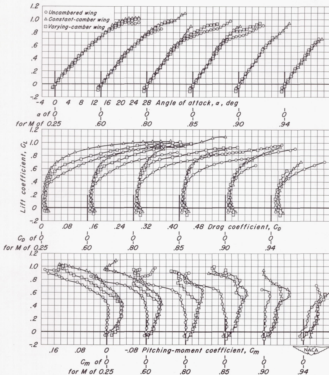
Figure 4.- Comparison of the lift, drag, and pitching-moment characteristics of the model with the three different wings.
