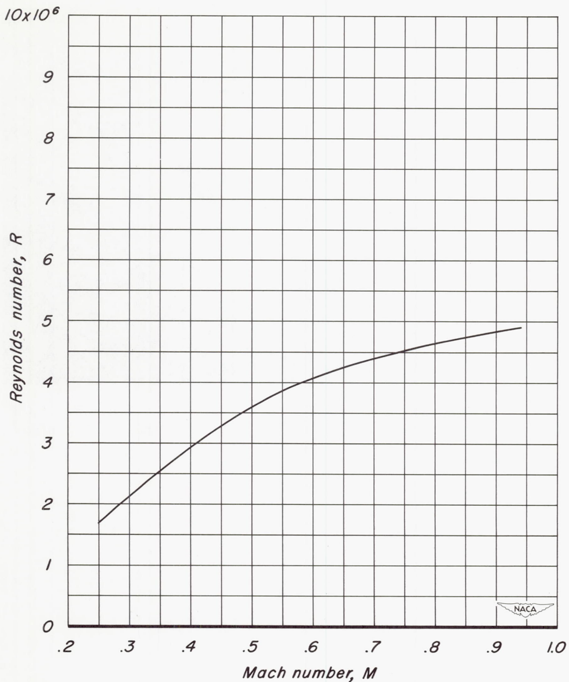
Figure 3.- The variation of Reynolds number with Mach number.
