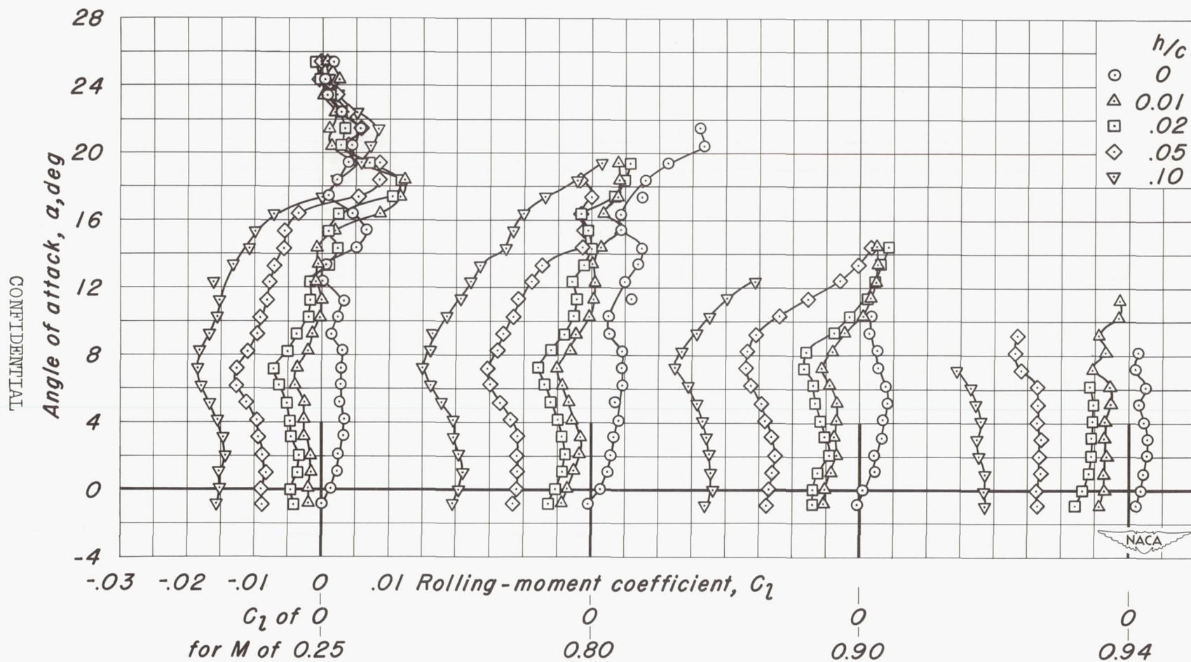
Figure 12.-The rolling-moment characteristics of the continuous spoiler.
