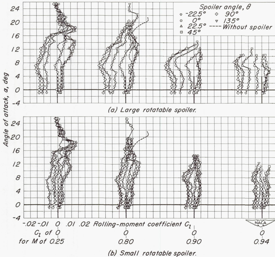
Figure 18.—The rolling-moment characteristics of the rotatable spoilers.
