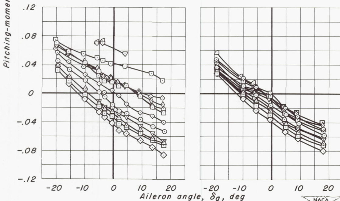
Figure 9.-The variation of pitching-moment coefficient with aileron angle.
