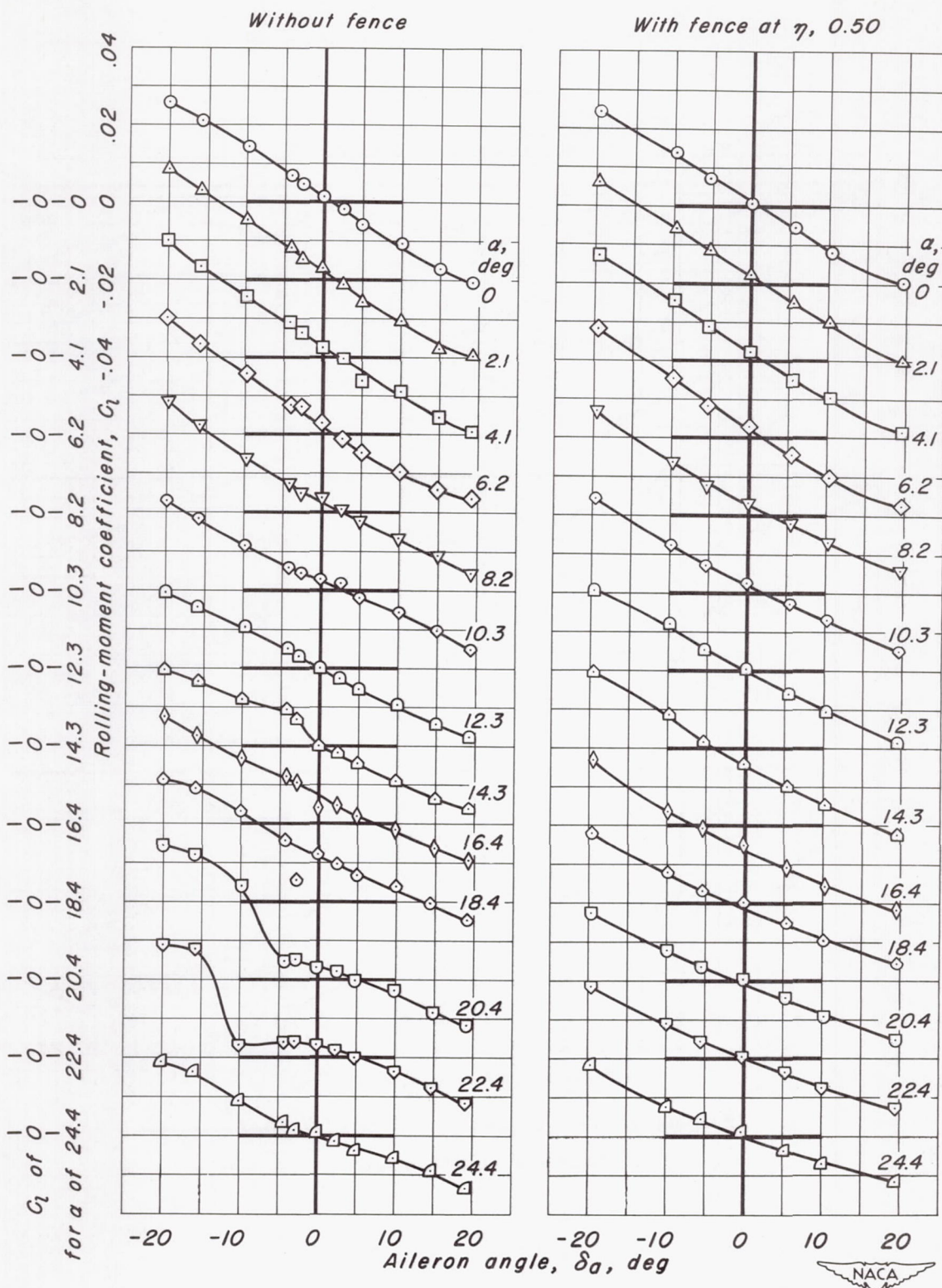
Figure 8.-The variation of rolling-moment coefficient with aileron angle.
