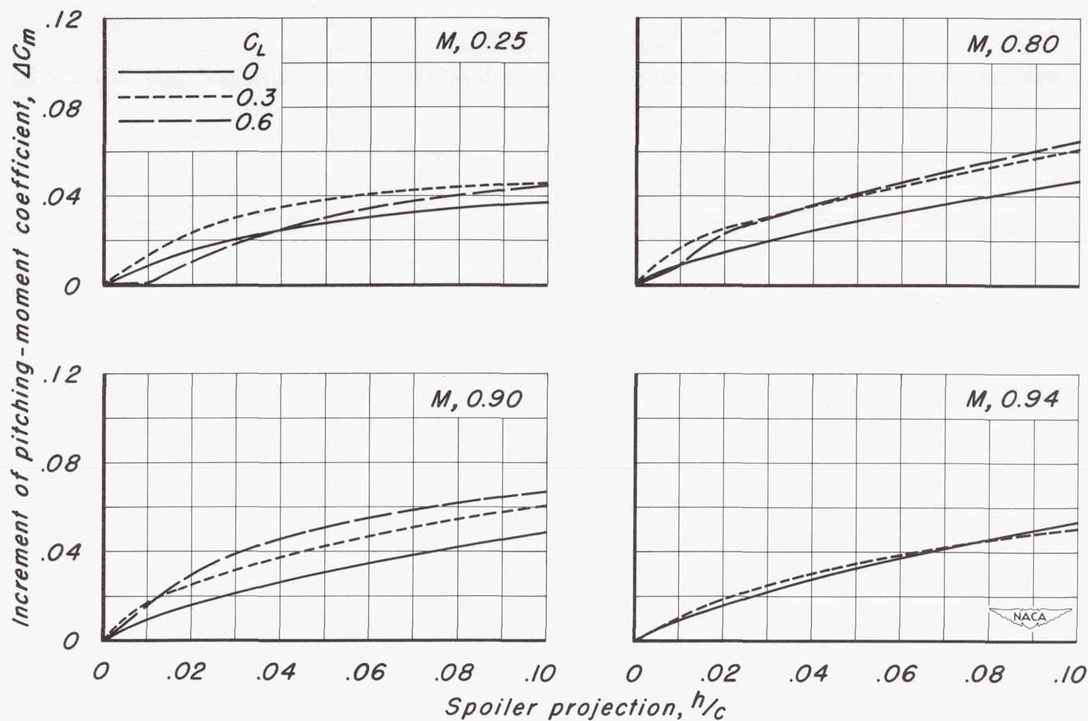
Figure 16.-The variation of incremental pitching-moment coefficient with projection of the continuous spoiler.
