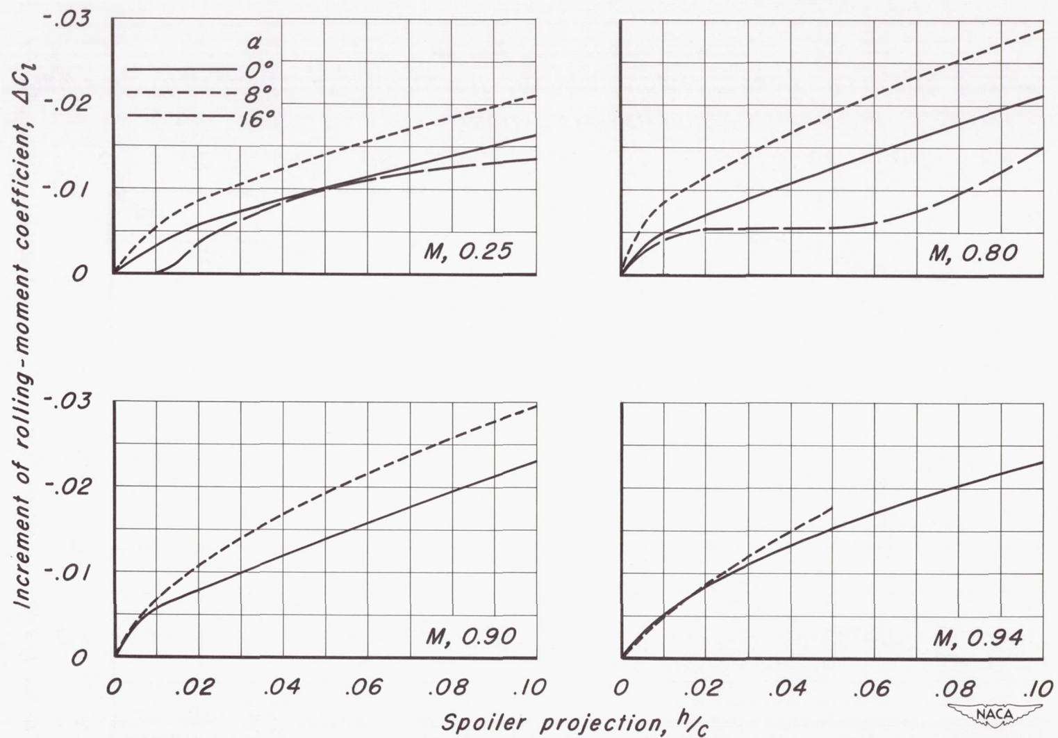
Figure 15.—The variation of incremental rolling-moment coefficient with projection of the continuous spoiler.
