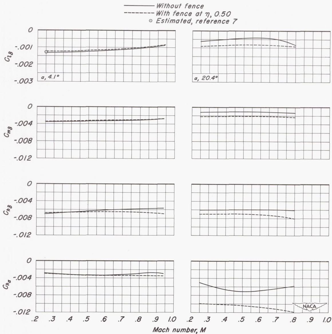
Figure 11.- The variation of the aileron effectiveness and hinge-moment parameters with Mach number.
