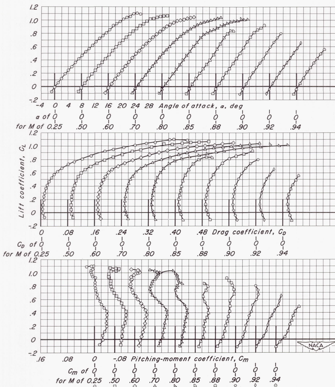
(a) Fence at \eta of 0.50.
