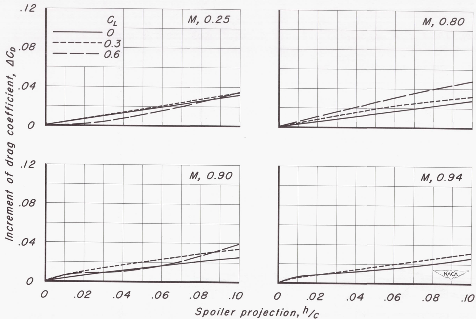
Figure 17.—The variation of incremental drag coefficient with projection of the continuous spoiler.
