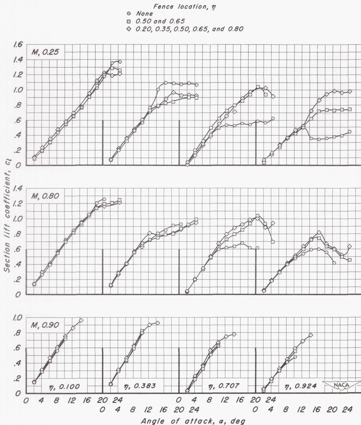
Figure 7.—The effect of different combinations of fences on the section lift and pitching-moment characteristics of four sections of the varying-camber wing.
