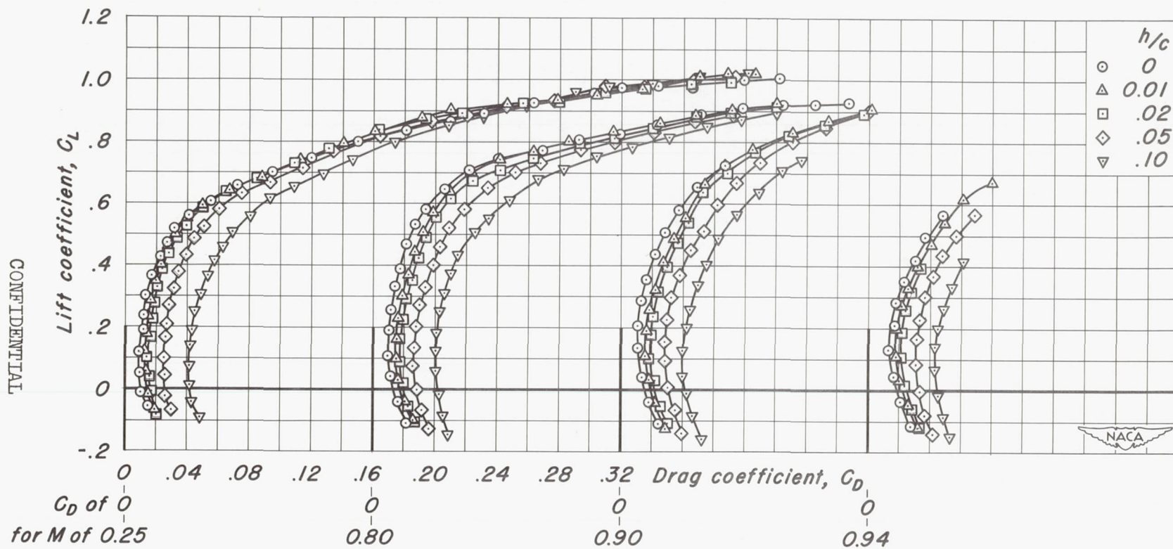
Figure 14.-The drag characteristics of the continuous spoiler.
