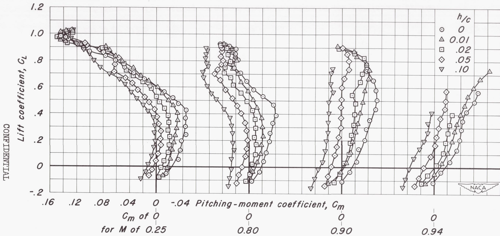
Figure 13.—The pitching-moment characteristics of the continuous spoiler.
