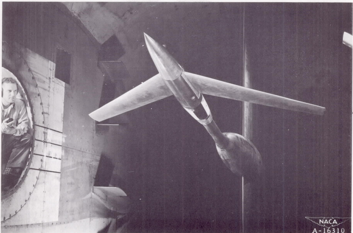
Figure 2.- Photograph of the model supported in the Ames 16-foot high-speed wind tunnel.
