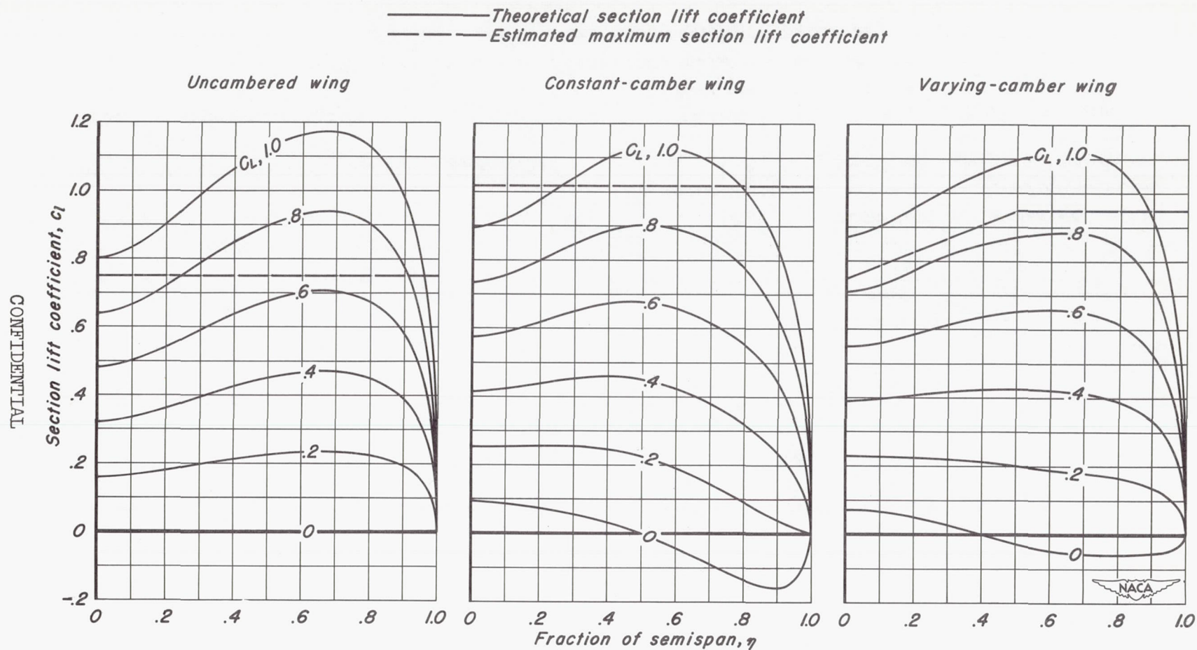
(b) Estimated spanwise variation of section lift coefficient and maximum section lift coefficient for the three wings. Figure 1.—Continued.
