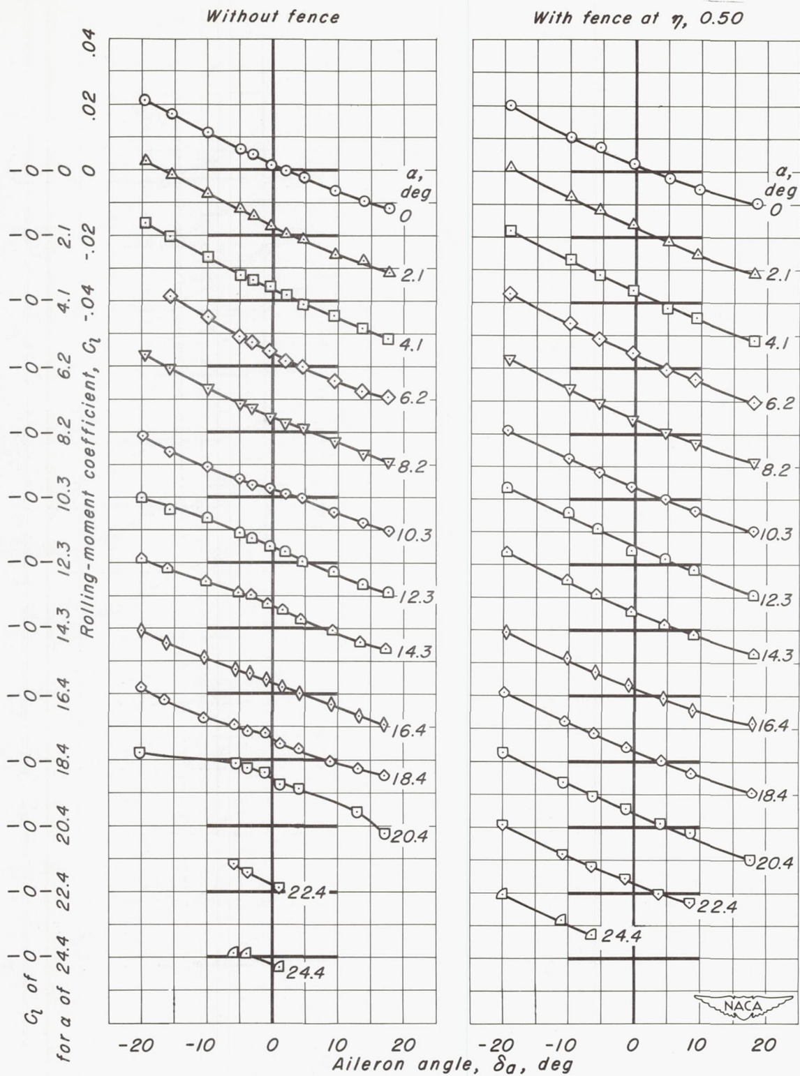
(b) M, 0.80 Figure 8.—Continued.
