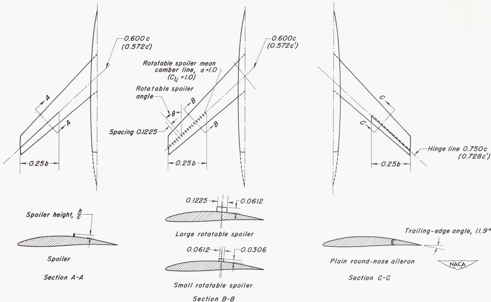
(d) Lateral-control devices on the varying-camber wing. Figure 1.- Concluded.
