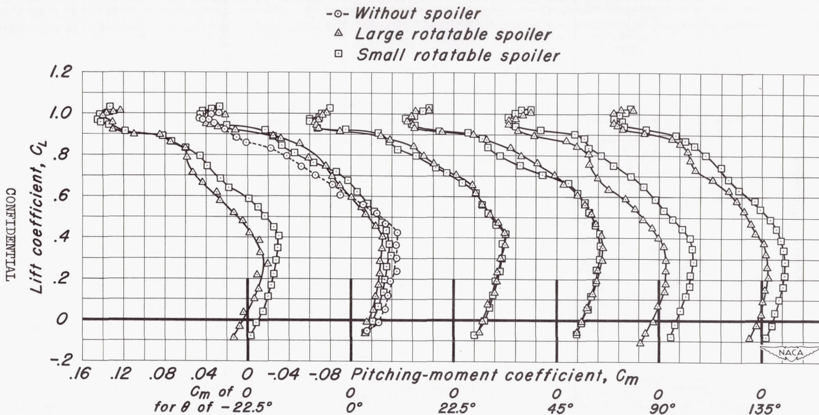
Figure 19.—The pitching-moment characteristics of the rotatable spoilers.
