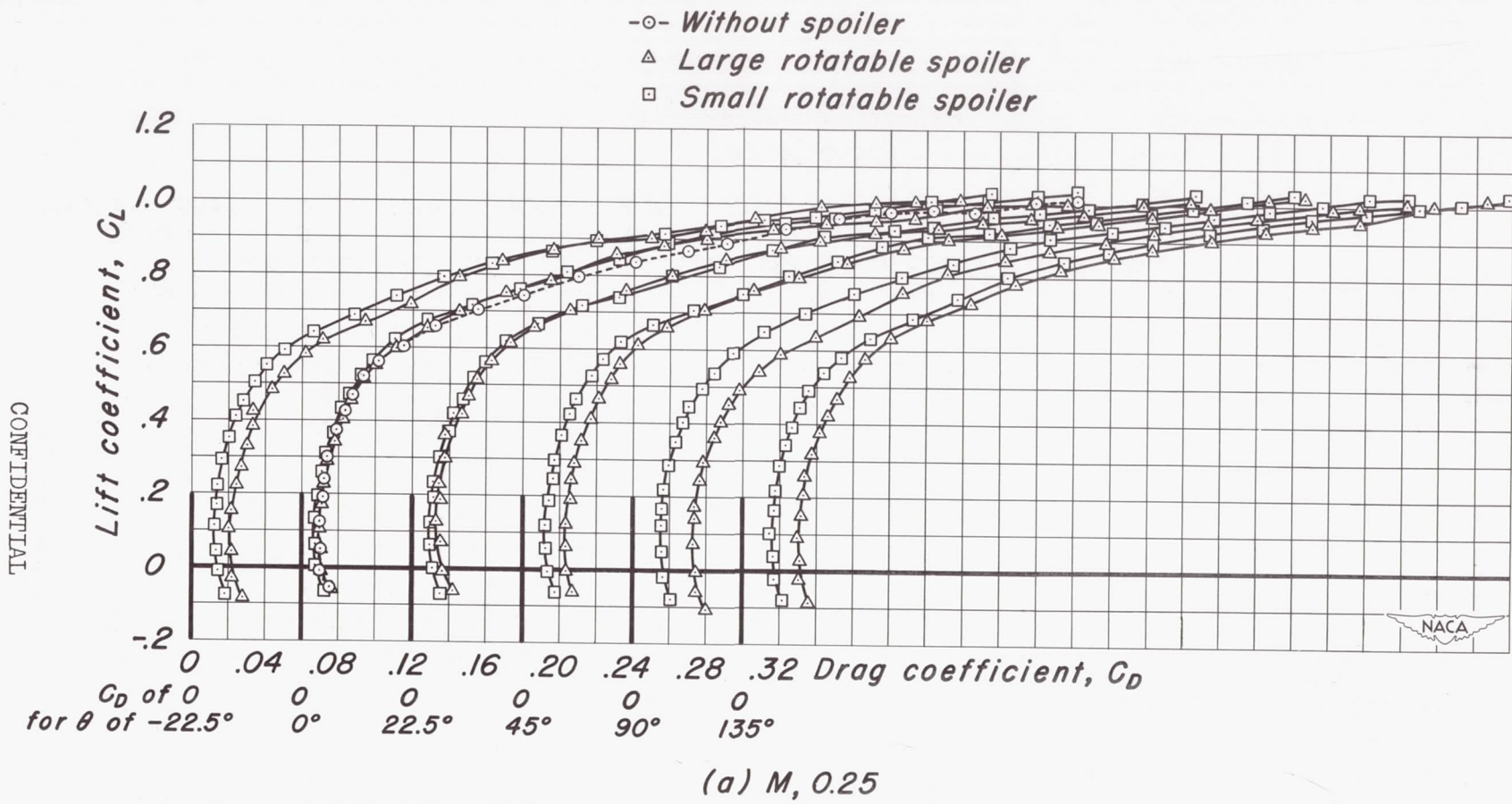
Figure 20.-The drag characteristics of the rotatable spoiler.
