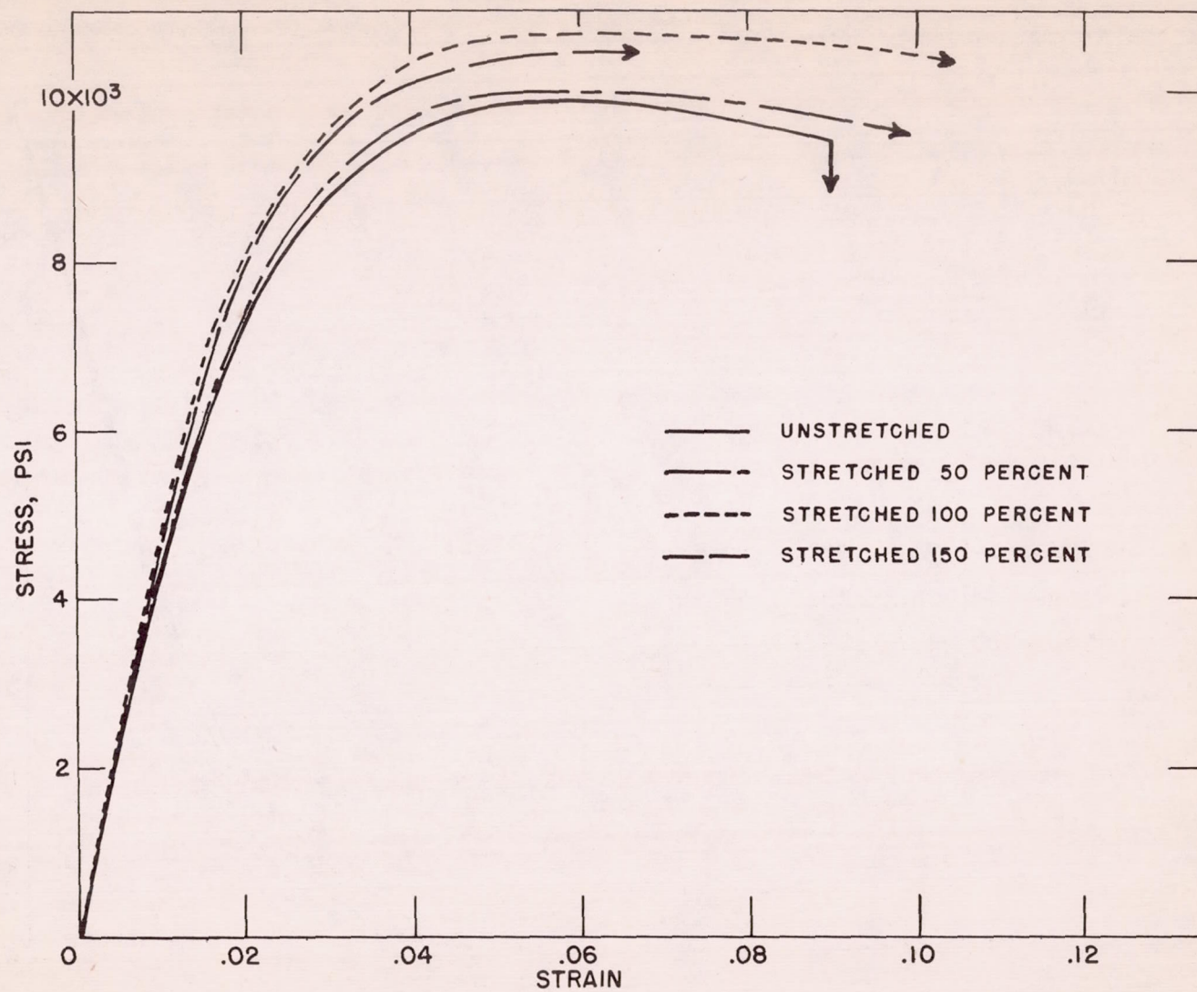
Figure 1.- Stress-strain diagrams of Lucite HC-222 (polymethyl methacrylate).
