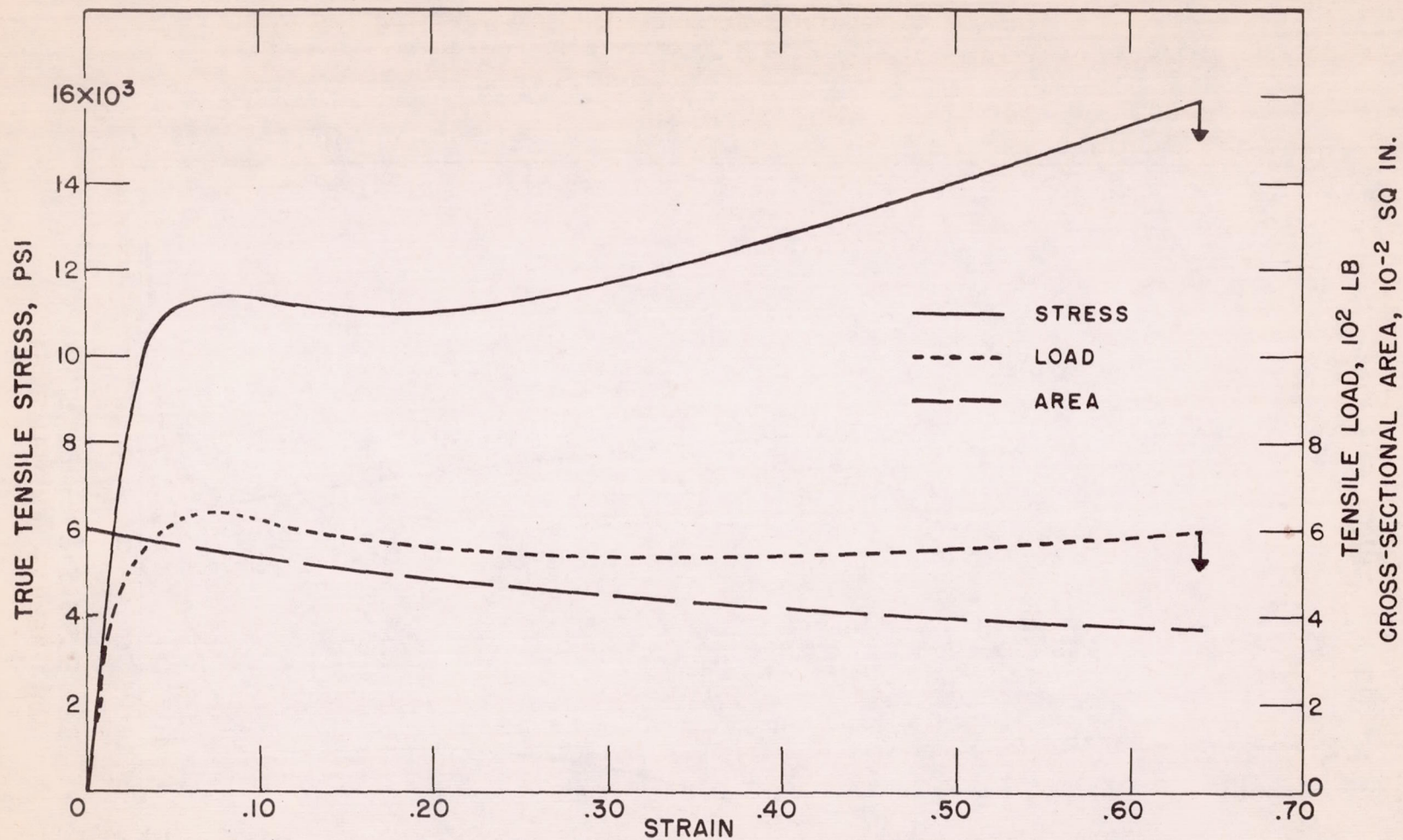
Figure 5.- Stress-strain diagram of Plexiglas 55 (modified polymethyl methacrylate), multiaxially stretched 45 percent.
