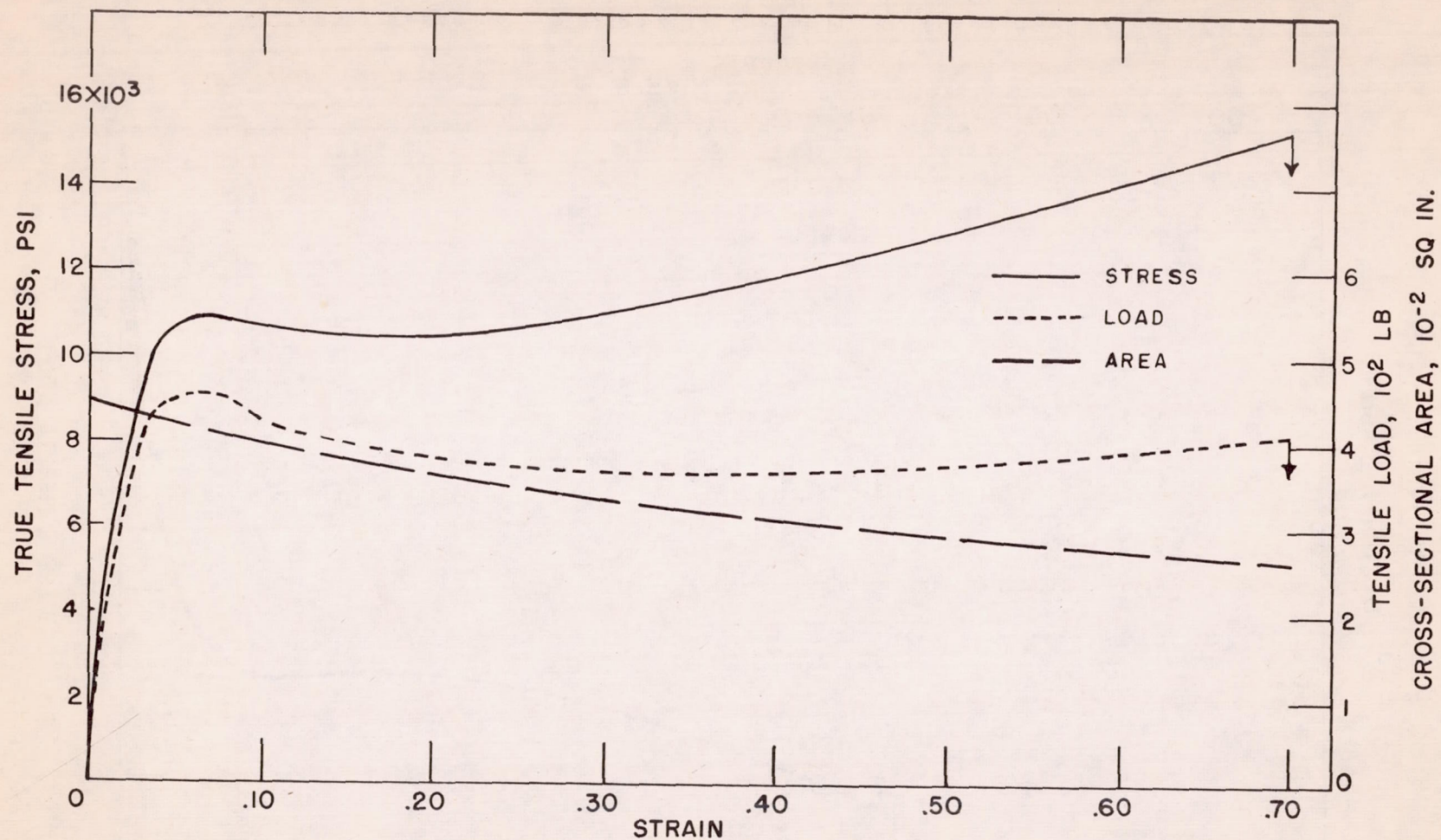
Figure 3.- Stress-strain diagram of Lucite HC-222 (polymethyl methacrylate), multiaxially stretched 50 percent.
