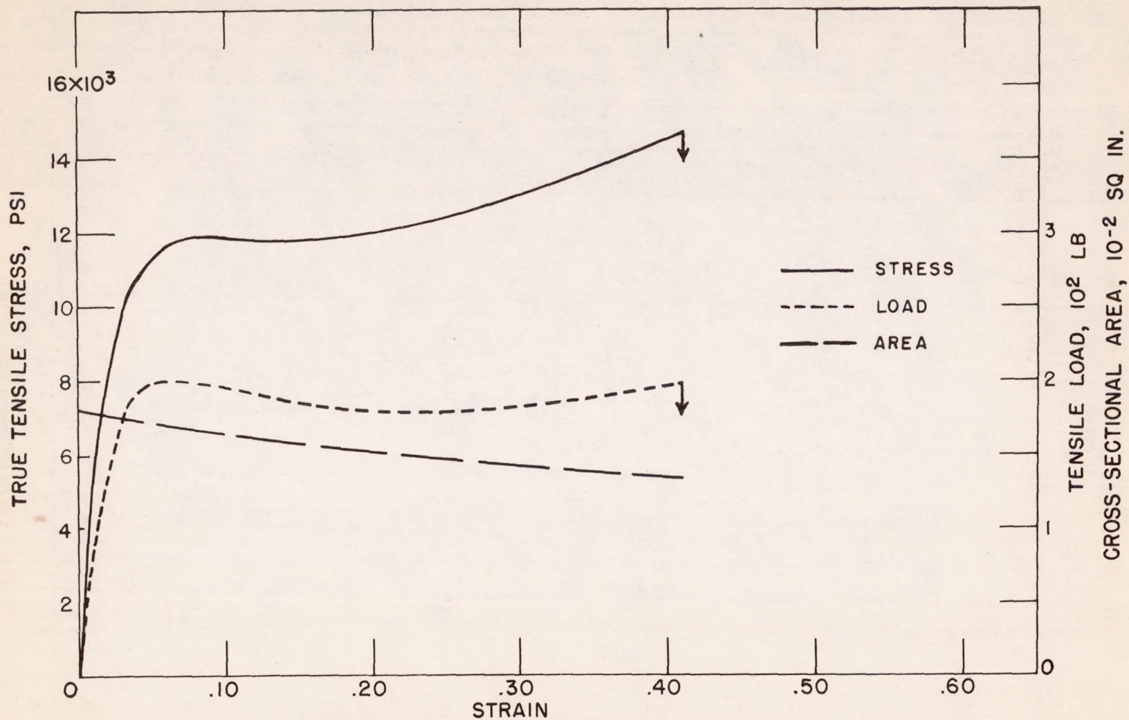
Figure 4.- Stress-strain diagram of Lucite HC-222 (polymethyl methacrylate), multiaxially stretched 150 percent.
