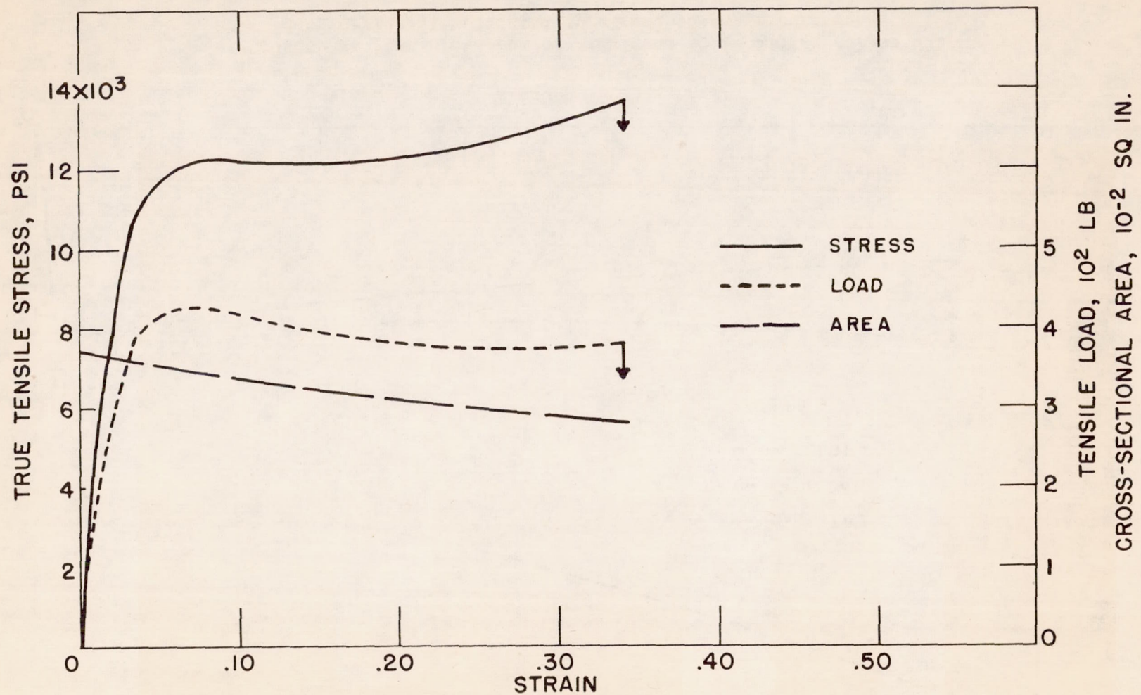
Figure 6.- Stress-strain diagram of Plexiglas 55 (modified polymethyl methacrylate), multiaxially stretched 85 percent.
