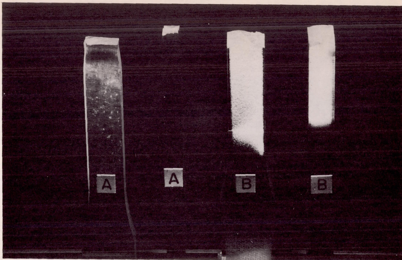
Figure 7.- Stress-crazed specimens of Lucite HC-222 (polymethyl methacrylate) and resin C (polymethyl alpha-chloroacrylate). Note internal crazing apparent in side view (second specimen) of polymethyl alpha-chloroacrylate but not in side view (second specimen) of polymethyl methacrylate.
