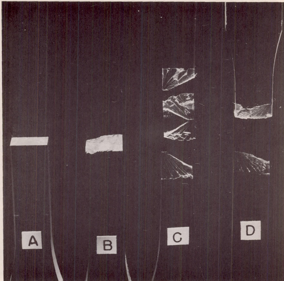
Figure 8.- Fracture surfaces of unstretched and stretched Lucite HC-222 (polymethyl methacrylate) and resin C (polymethyl alpha-chloroacrylate): (A) unstretched polymethyl methacrylate; (B) unstretched polymethyl alpha-chloroacrylate; (C) modified polymethyl methacrylate stretched 45 percent; (D) polymethyl alpha-chloroacrylate stretched 100 percent. Note third piece (turned over) broken out of specimen C. Specimen D broke into two pieces only (top piece is turned over).
