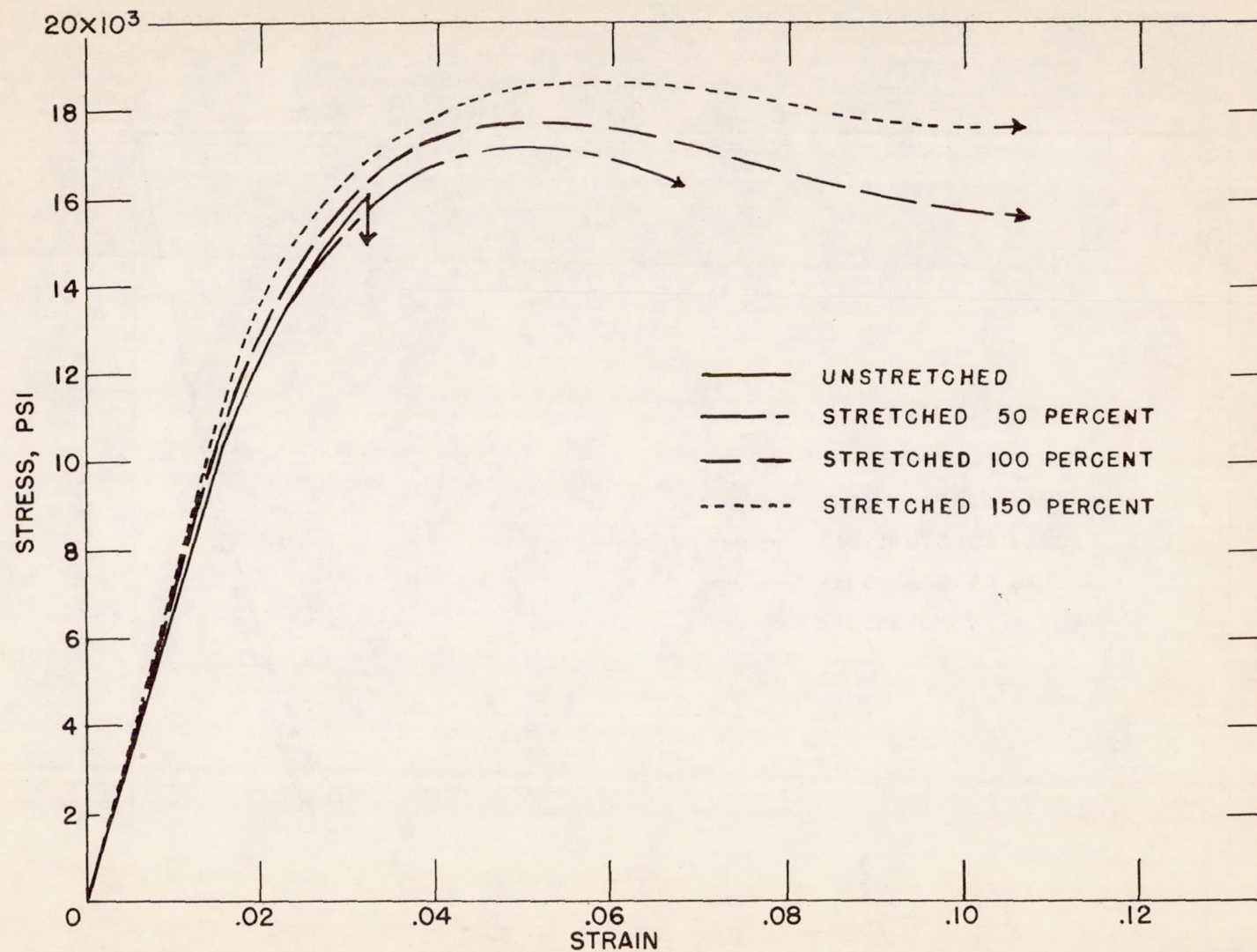
Figure 2.- Stress-strain diagrams of resin C (polymethyl alpha-chloroacrylate).
