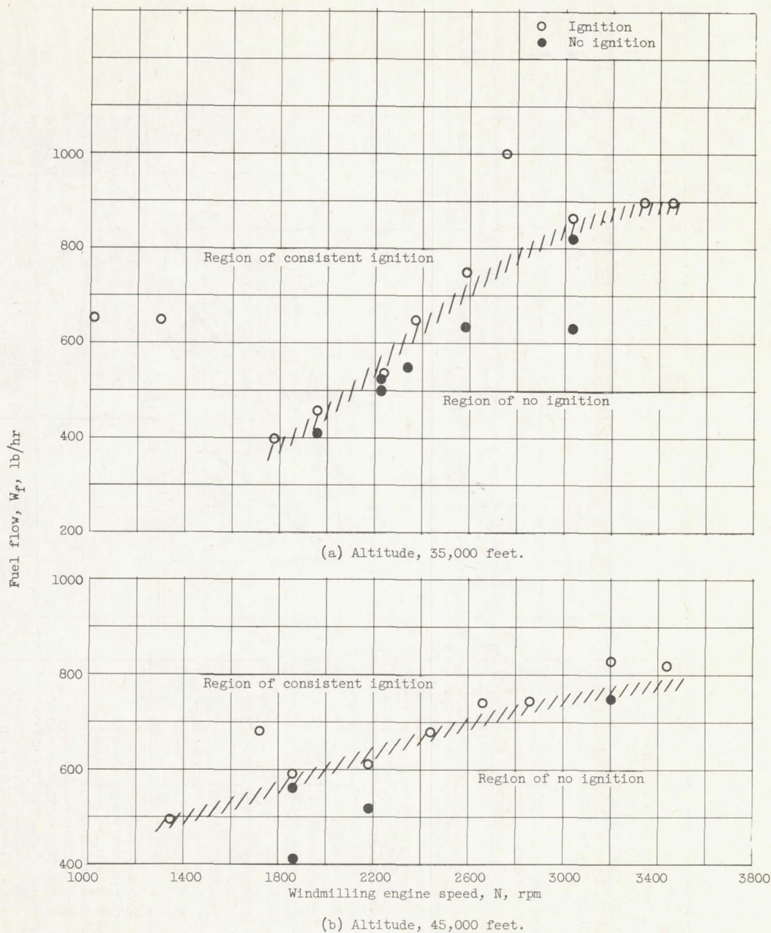
Figure 18. - Effect of fuel flow on altitude-ignition characteristics. Fuel temperature, approximately 60° F; engine-inlet air temperature, 5° to -50° F.
