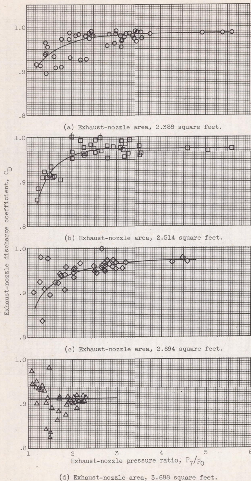
Figure 10. - Exhaust-nozzle discharge coefficient.
