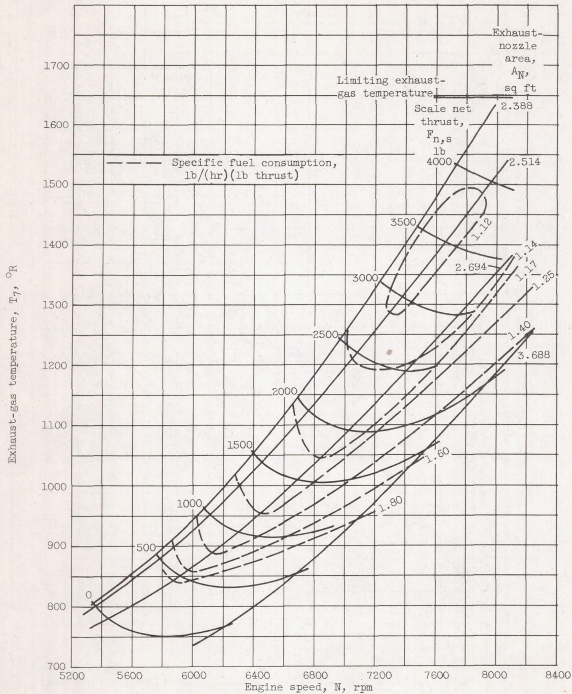
Figure 5. - Continued. Engine performance maps.
