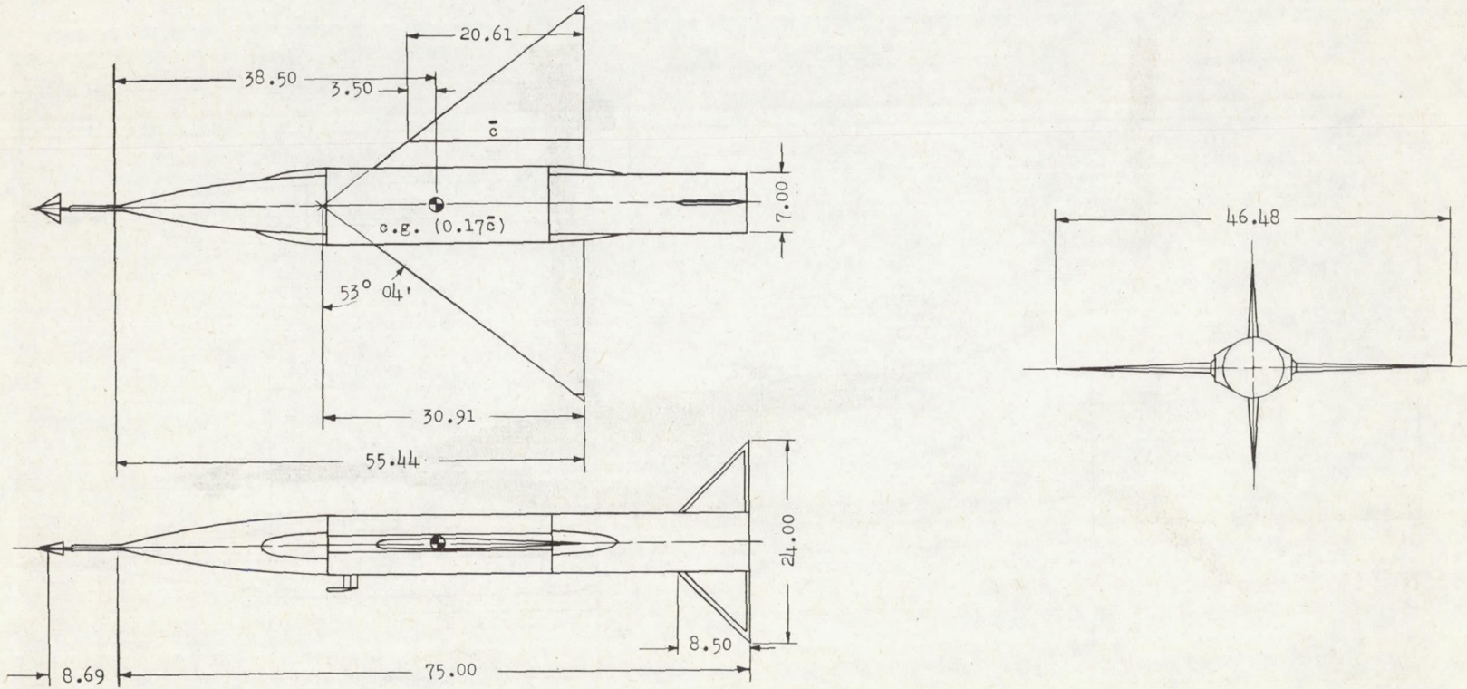
(c) Model 3. With afterbody; A = 3 .
