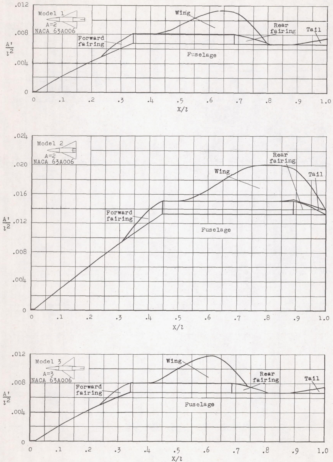
Figure 4.- Longitudinal distribution of cross-sectional area.
