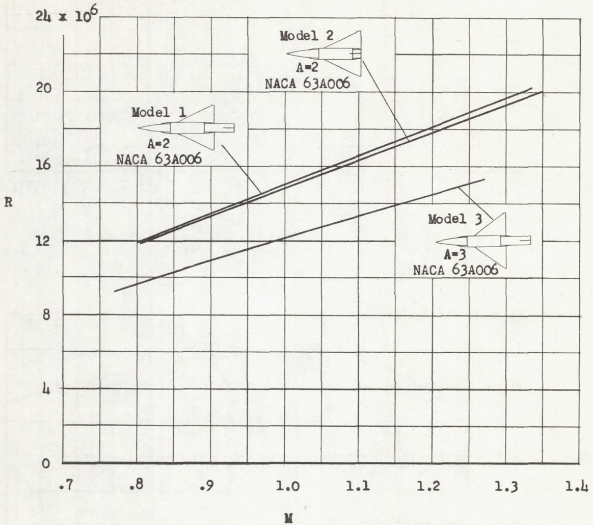
Figure 9.- Scale of tests based on respective mean aerodynamic chord.
