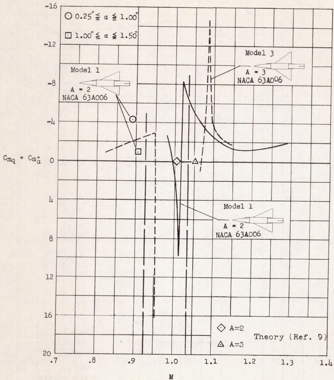
Figure 14.- Variation of the rotational damping-in-pitch derivatives with Mach number. (The vertical long-dash lines represent region of limited data.)
