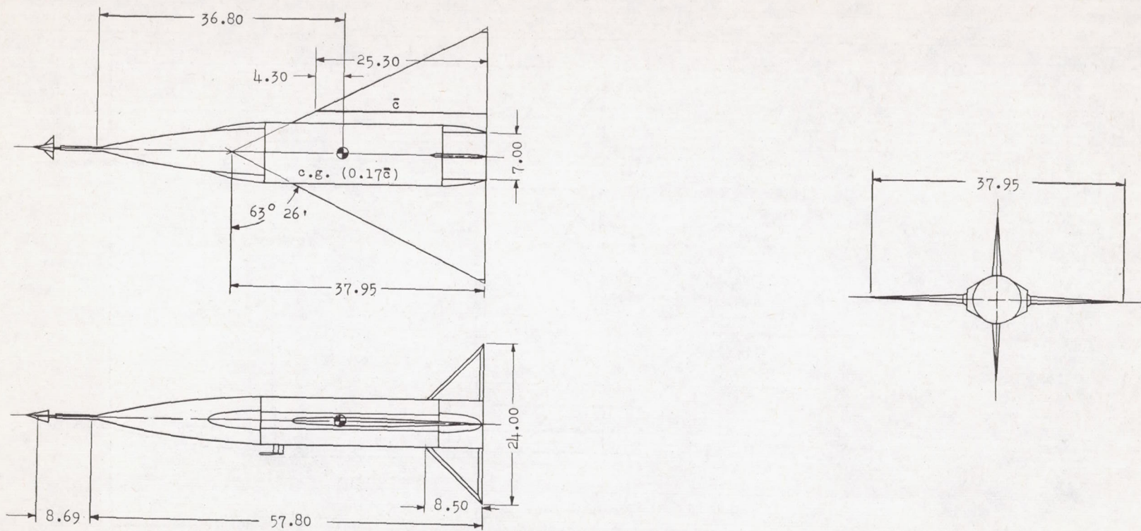
(b) Model 2. No afterbody; A = 2 .
