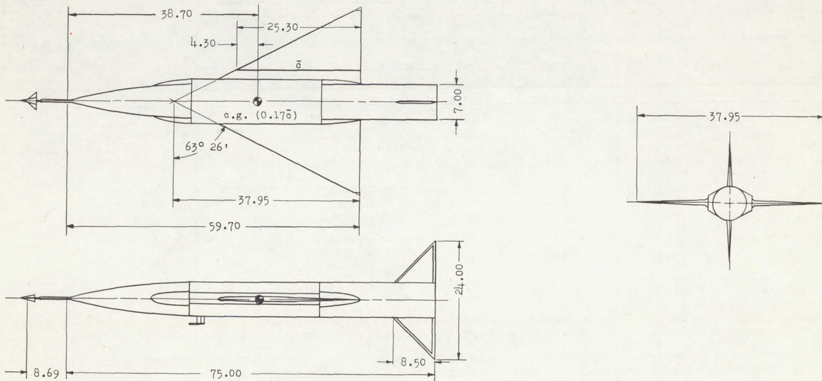
(a) Model 1. With afterbody; A = 2 .
