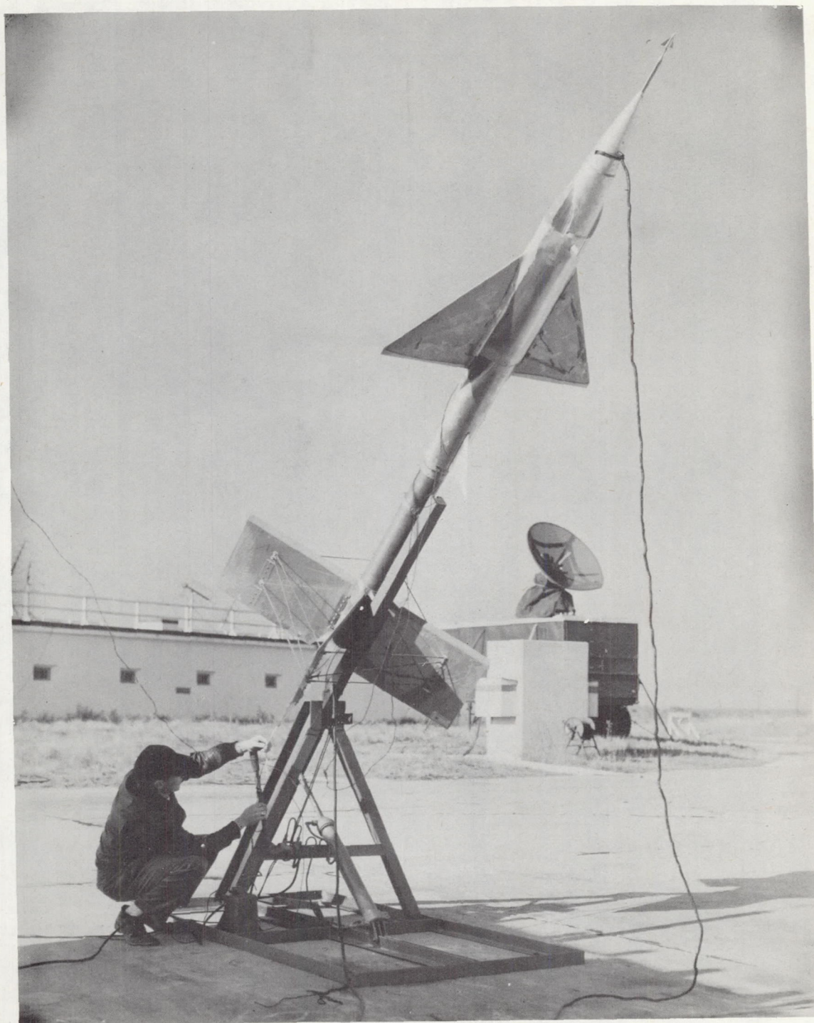
Figure 3.- Photograph of one of the models on the launcher.
