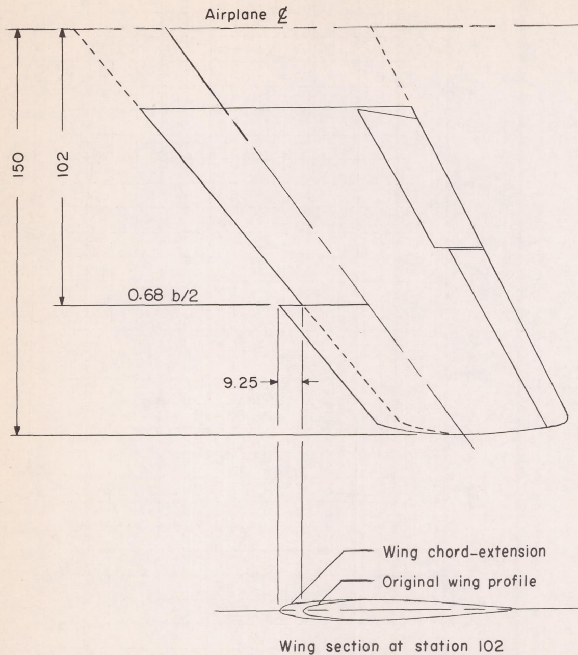
Figure 3.- Wing plan form and profile section showing leading-edge chord-extensions on the Douglas D-558-II research airplane. Dimensions given in inches unless otherwise noted.
