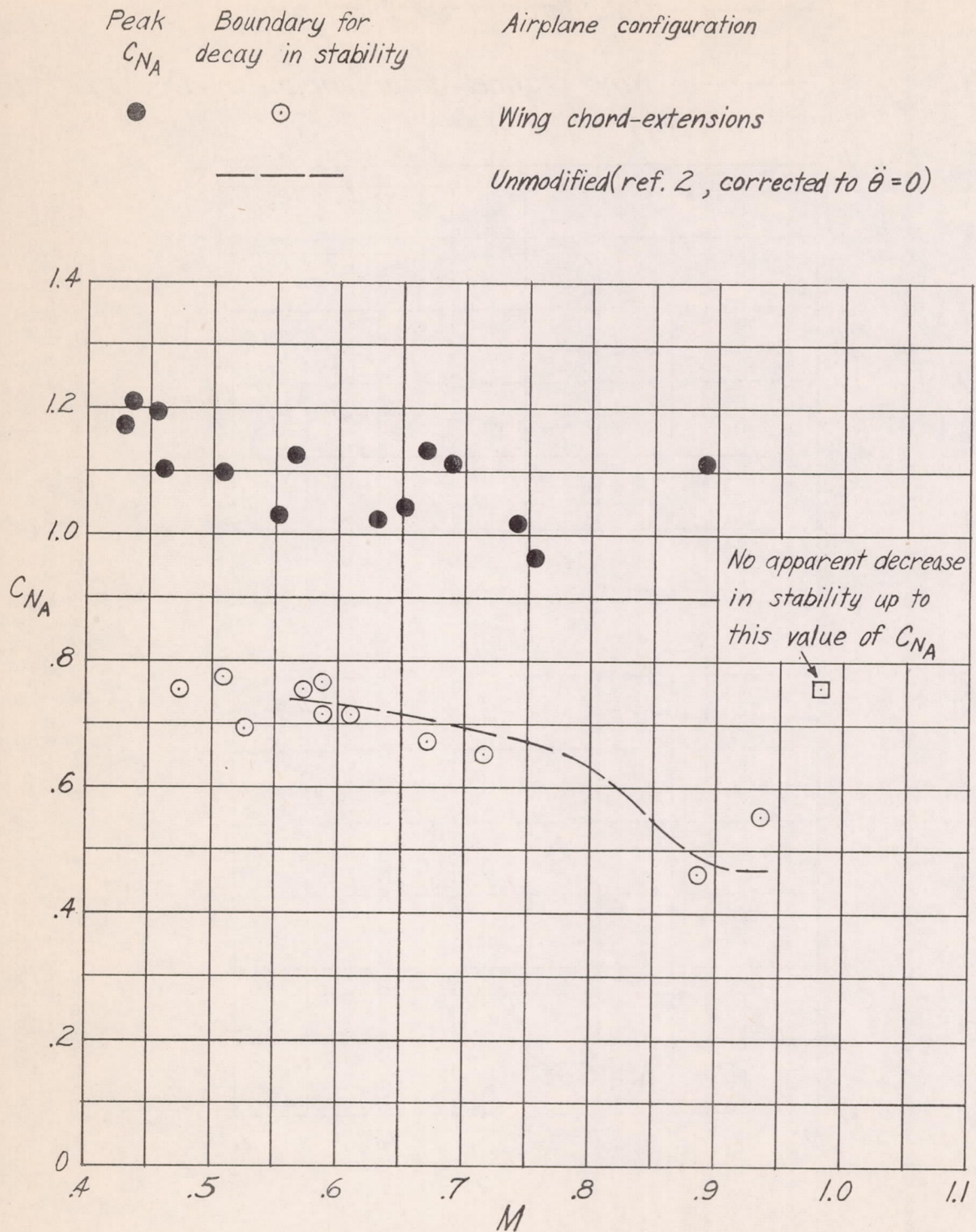
Figure 8.- Normal-force coefficient for decay in longitudinal stability as a function of Mach number for the Douglas D-558-II research airplane.
