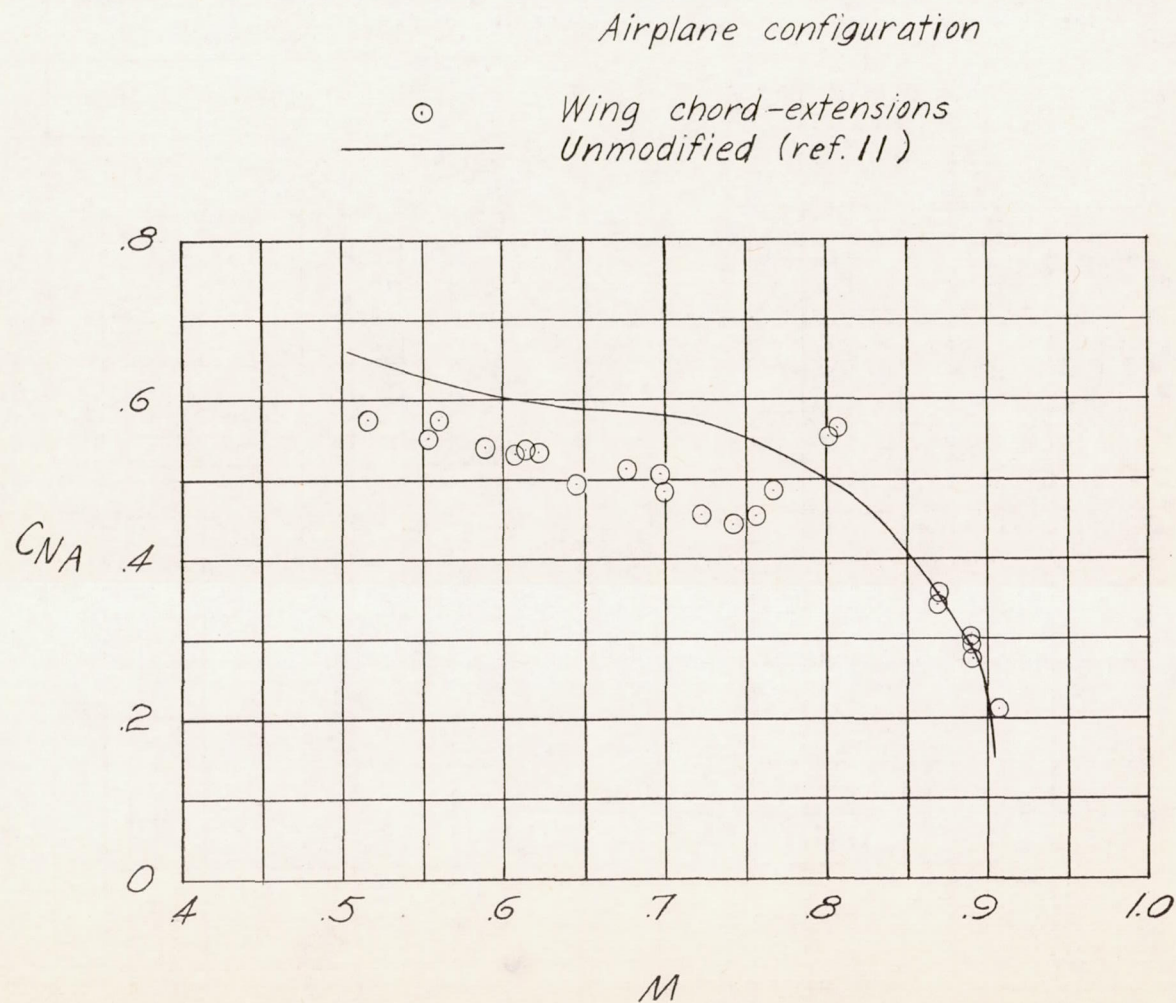
Figure 7.- Comparison of the buffet boundary of the D-558-II research airplane equipped with wing chord extensions with the unmodified configuration.
