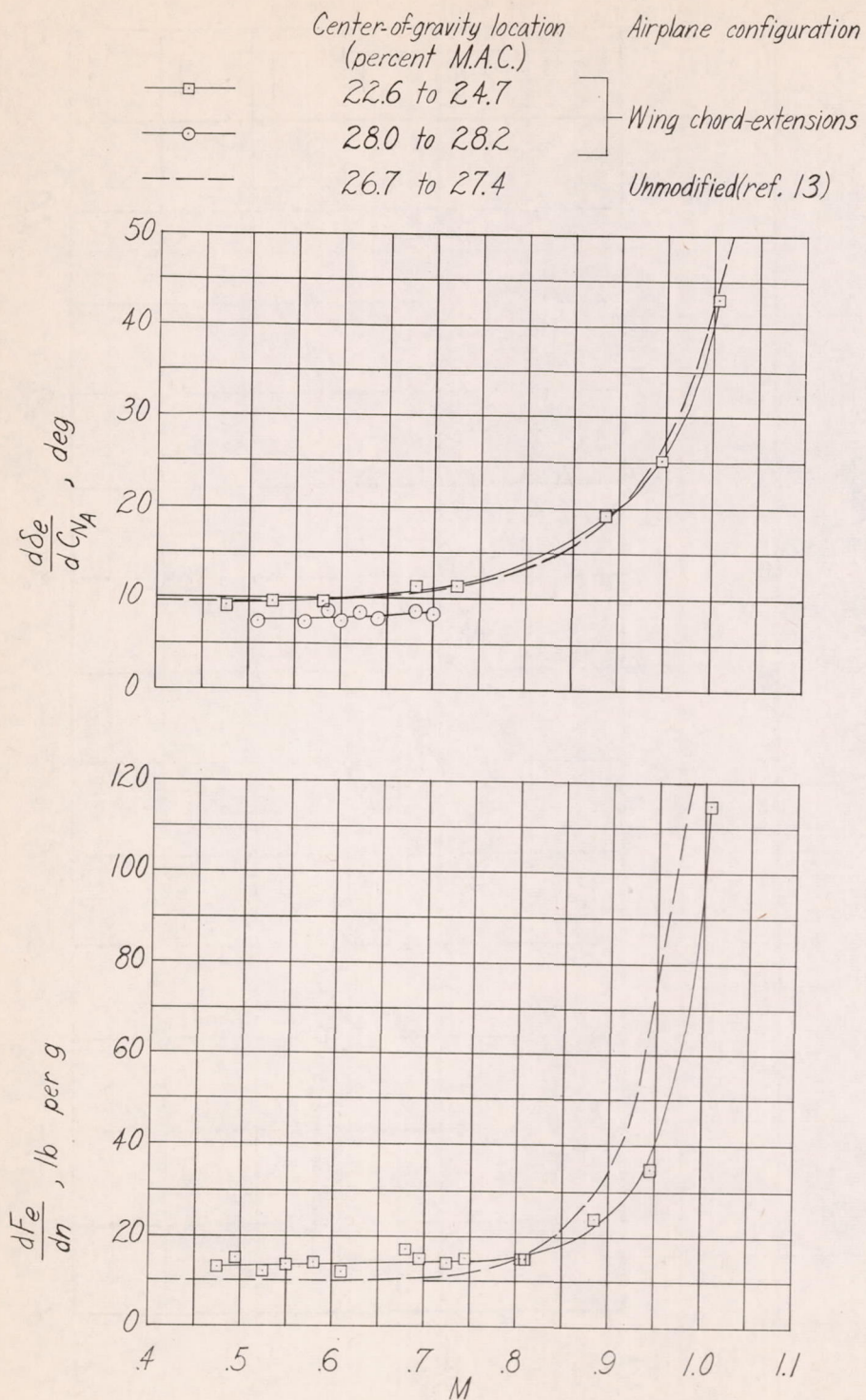
Figure 12.- Variation with Mach number of d\delta_e/dC_{N_A} and dF_e/dn for the Douglas D-558-II research airplane.
