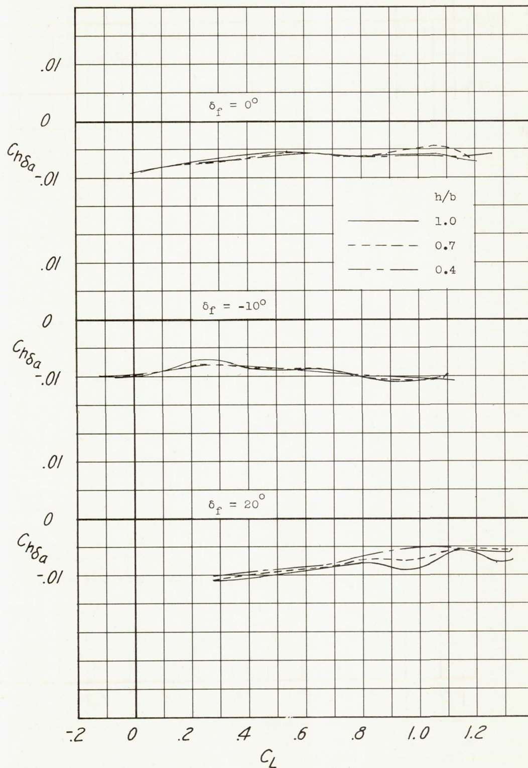
Figure 19.- Variation of aileron hinge-moment parameters with lift coefficient at three ground heights and three flap deflections.
