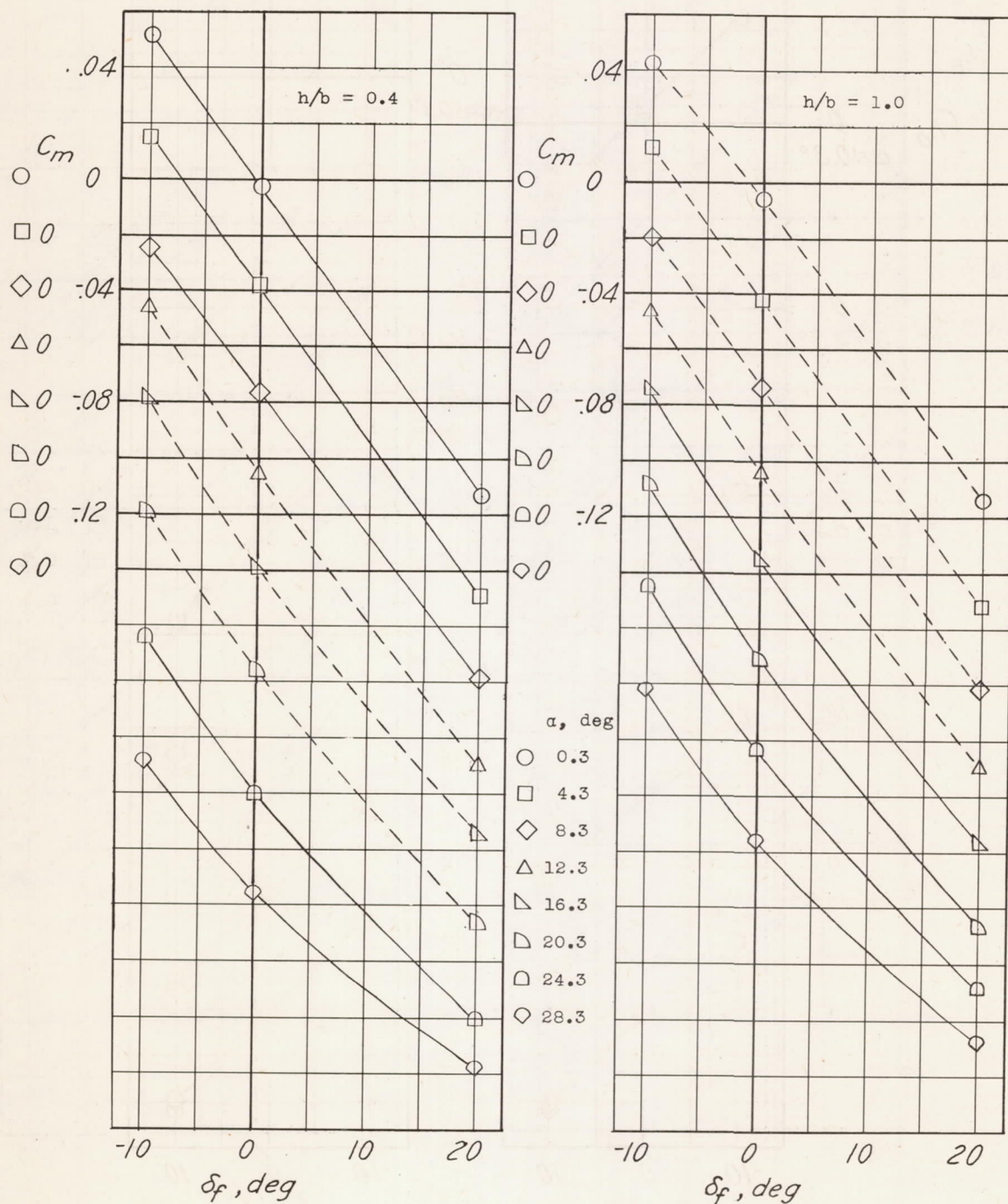
Figure 14.- Variation of pitching-moment coefficient with flap deflection at two ground heights. \delta_a = 0^\circ .
