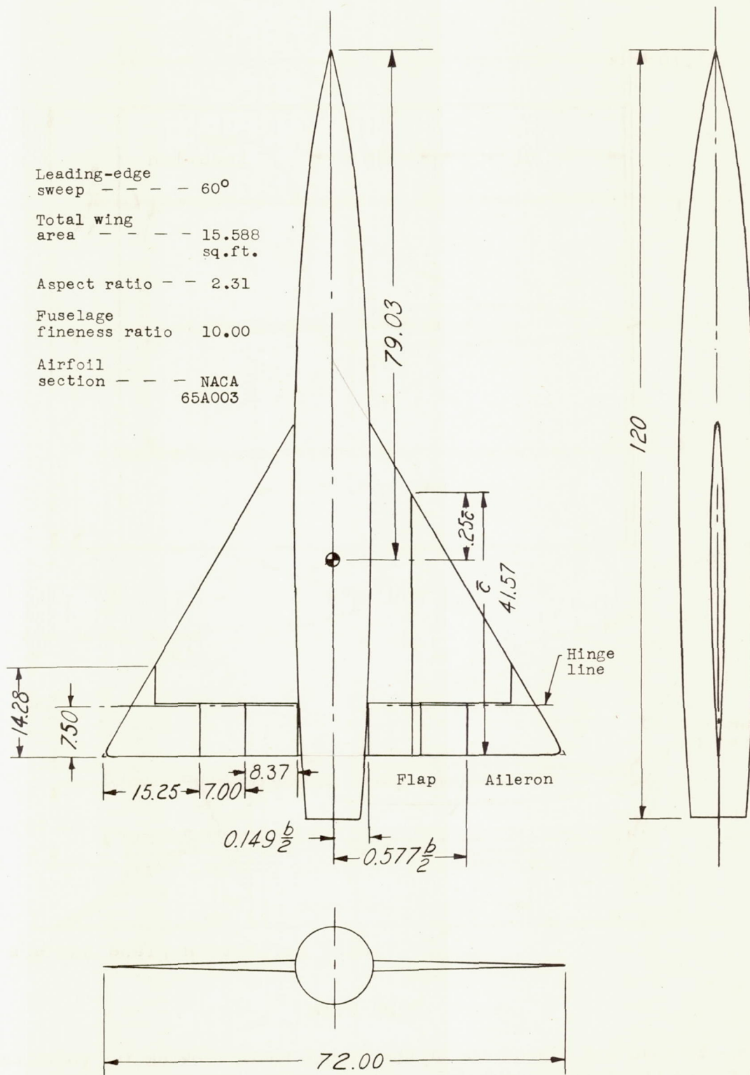
Figure 2.- General arrangement and principal dimensions of the 60^\circ delta-wing model. All dimensions are given in inches.
