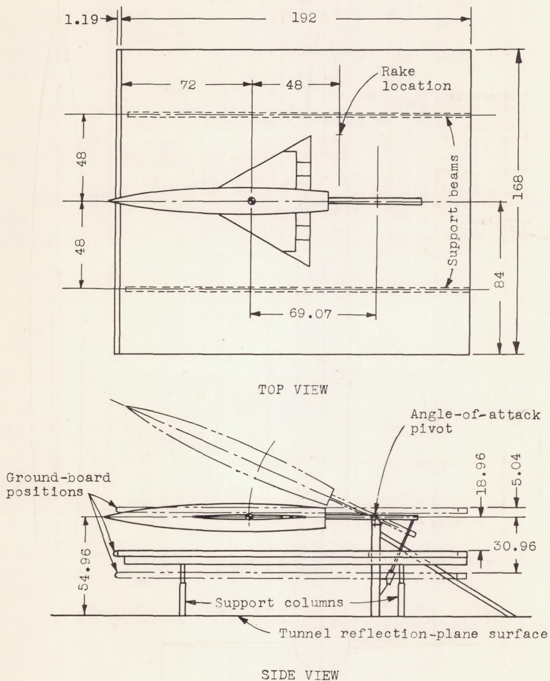
Figure 3.- Details and dimensions of the ground board showing its positions relative to the delta-wing model. All dimensions are given in inches.
