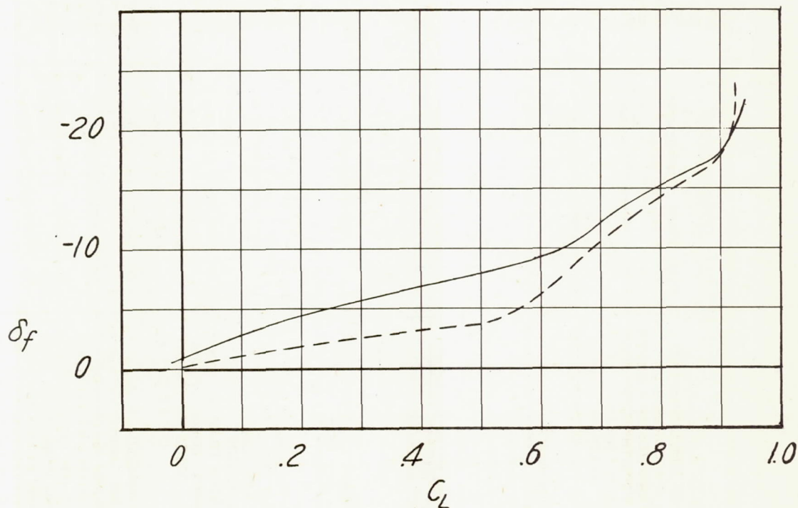
(b) h/b = 0.4 .
