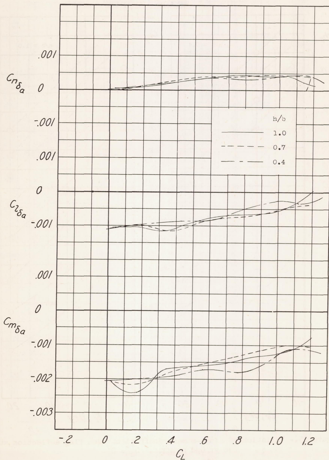
Figure 16.- Variation of aileron-control-effectiveness parameters with lift coefficient at three ground heights. \delta_f = 0^\circ .
