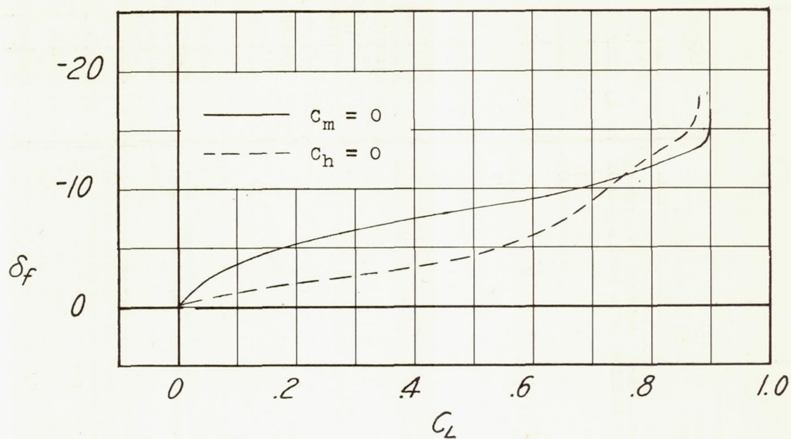
(a) h/b = 1.0 .
