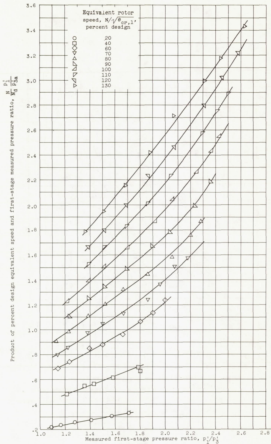
(b) Relation of measured pressure ratios at stations 3 and 3a.
