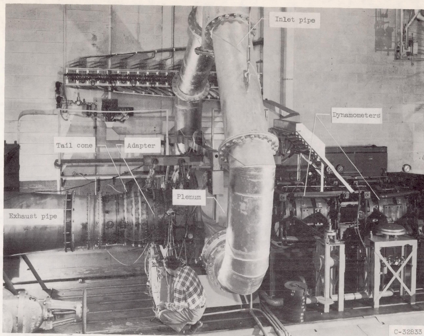
Figure 1. - Setup for investigation of performance of J73 turbine.
