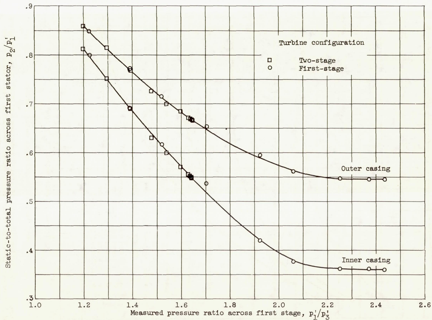
Figure 6. - Variation of static-to-total pressure ratio across first stator with measured total-pressure ratio across first stage for standard-bladed turbines at design speed.
