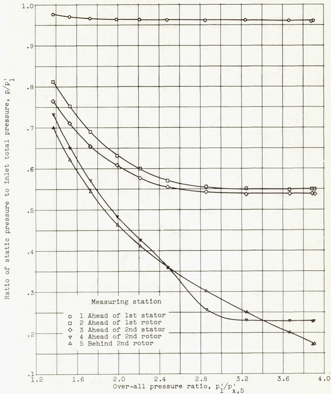
(b) Static pressures at inner casing.
