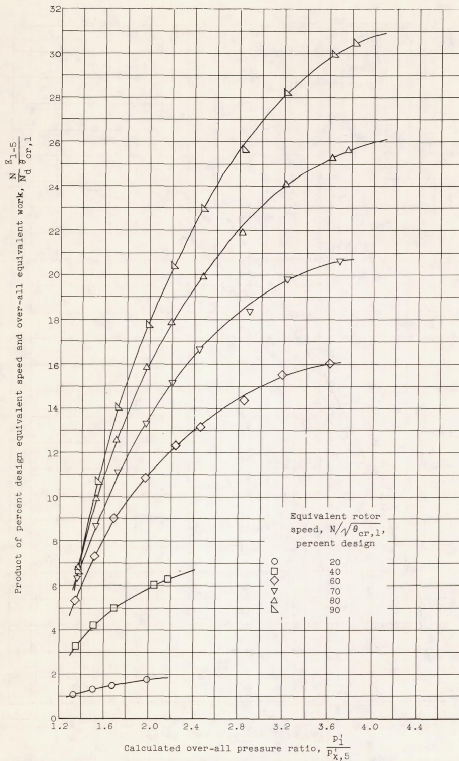
(b) Relation of equivalent work and calculated pressure ratio for equivalent speeds from 20 to 90 percent of design.
