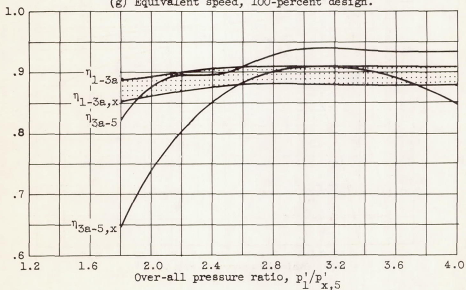
Figure 9. - Continued. Variation of stage efficiencies with turbine speed and over-all pressure ratio for J73 two-stage turbine.
