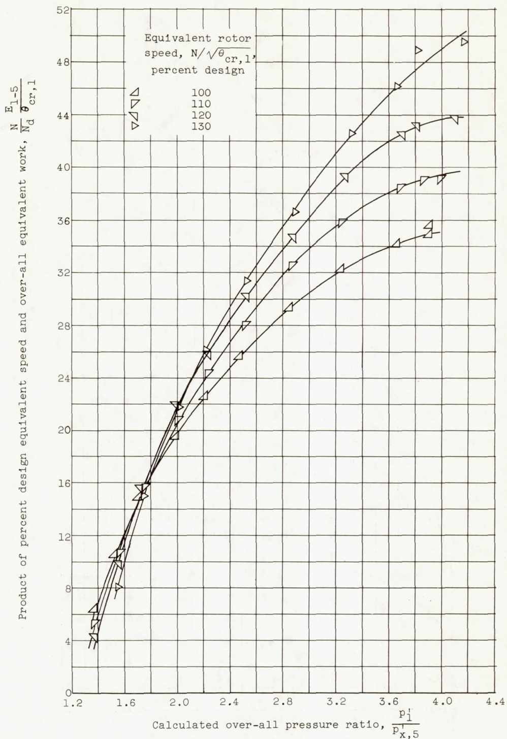
(c) Relation of equivalent work and calculated pressure ratio for equivalent speeds from 100 to 130 percent of design.
