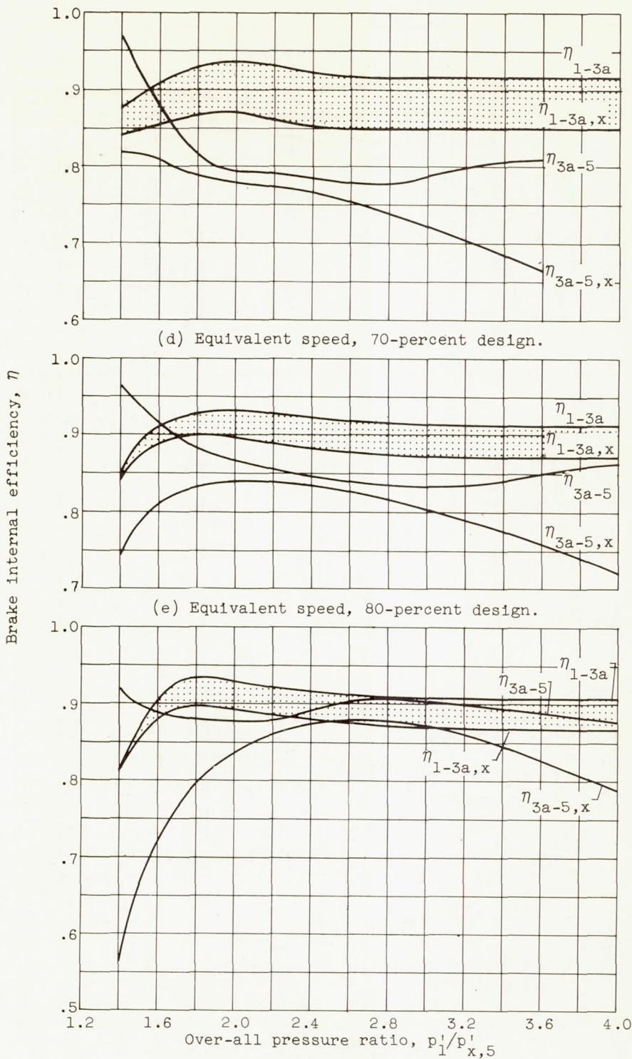
Figure 9. - Continued. Variation of stage efficiencies with turbine speed and over-all pressure ratio for J73 two-stage turbine.
