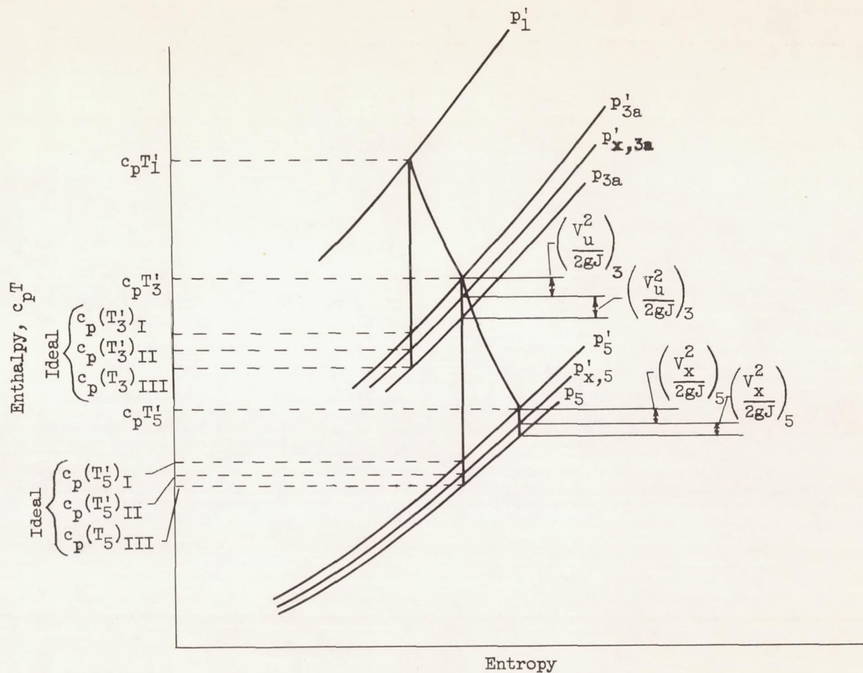
Figure 12. - Temperature-entropy diagram used to define stage efficiencies.
