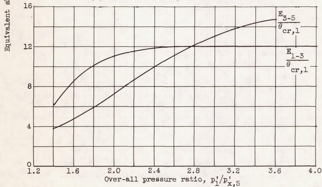
(c) Equivalent speed, 60-percent design.
