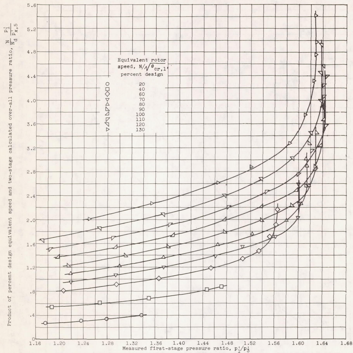
Figure 5. - Correlation curves indicating variation of calculated over-all pressure ratio with measured first-stage pressure ratio for J73 two-stage turbine.
