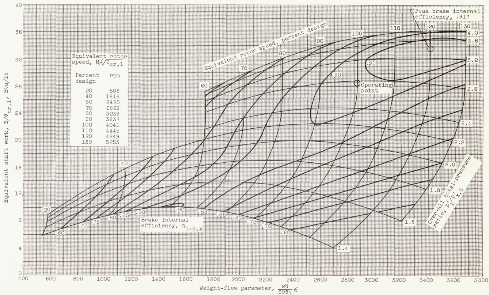
Figure 11. - Over-all performance of J73 two-stage turbine equipped with standard rotor blading. Turbine-inlet pressure, 35 inches of mercury absolute; turbine-inlet temperature, 700° R (ref. 2).
