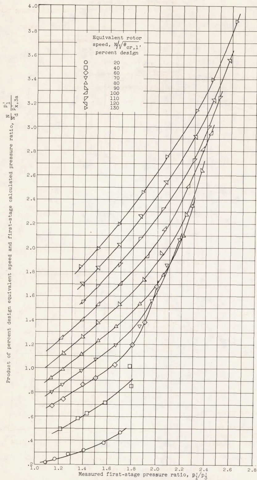
(a) Relation of calculated and measured pressure ratios.
