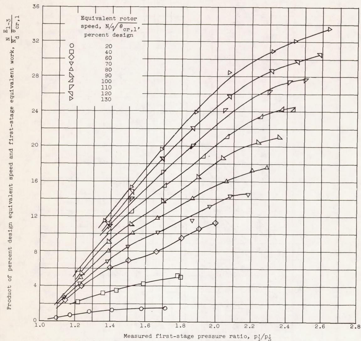
(c) Relation of equivalent work and measured pressure ratio.
