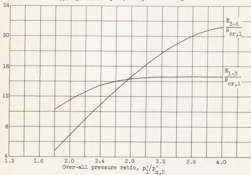
Figure 8. - Continued. Variation of stage equivalent shaft work with turbine speed and over-all pressure ratio for J73 two-stage turbine.
