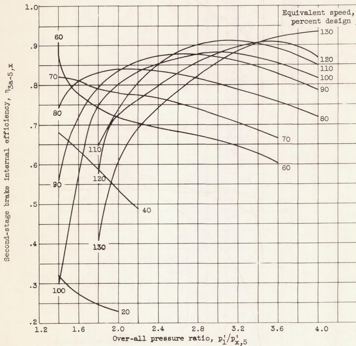
Figure 10. - Effect of turbine equivalent speed on second-stage efficiency.
