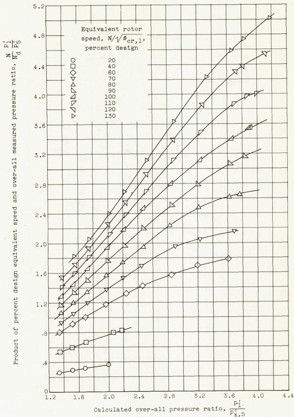
(a) Relation of calculated and measured pressure ratios.
