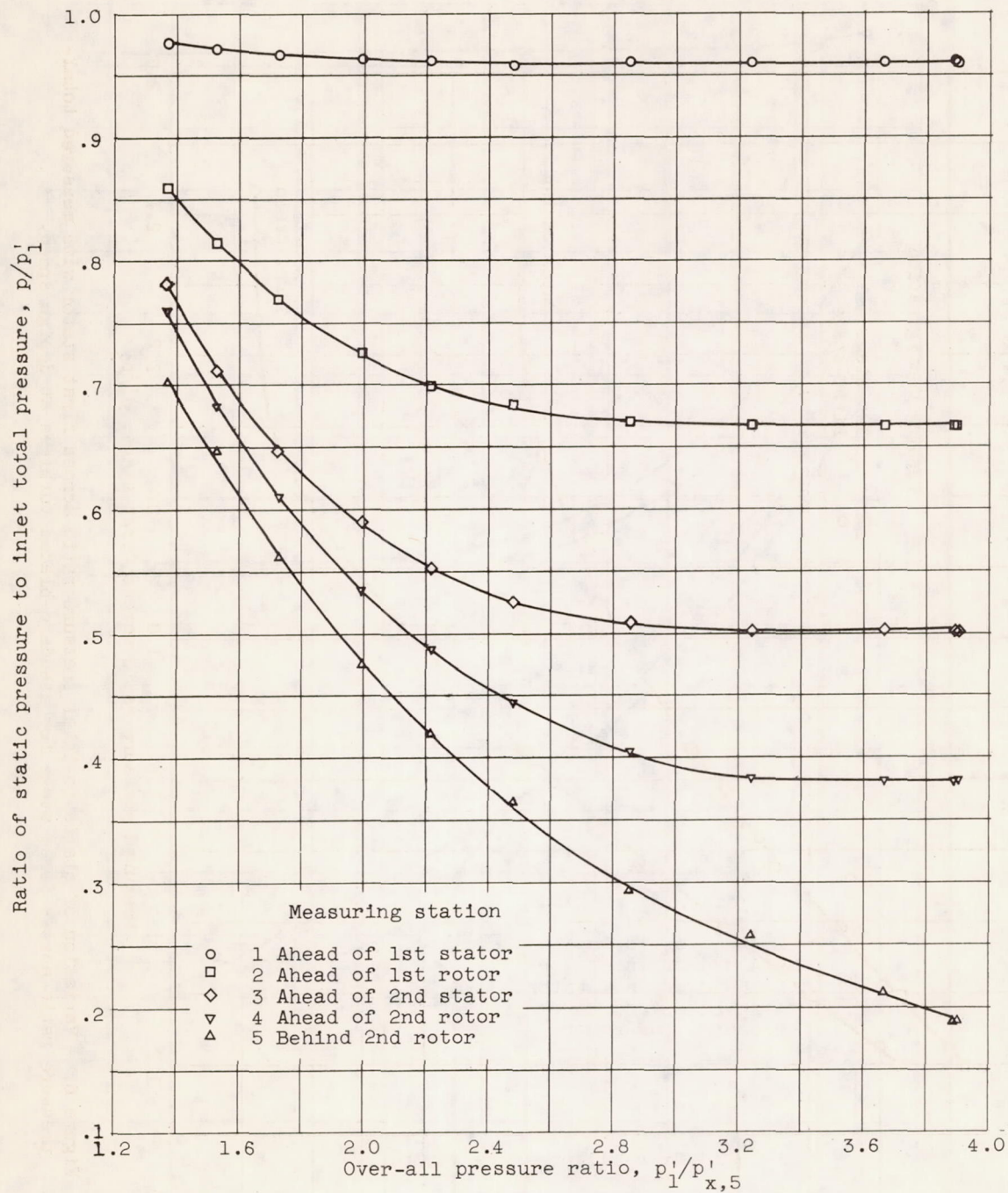
(a) Static pressures at outer casing.
