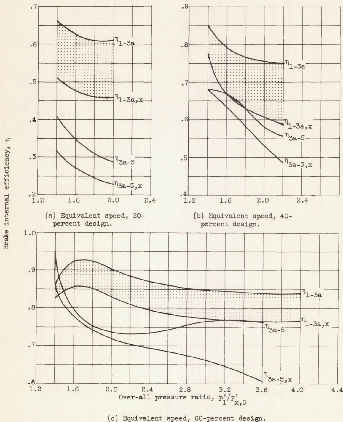
Figure 9. - Variation of stage efficiencies with turbine speed and over-all pressure ratio for J73 two-stage turbine.
