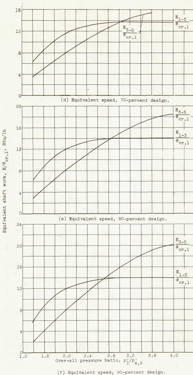
Figure 8. - Continued. Variation of stage equivalent shaft work with turbine speed and over-all pressure ratio for J73 two-stage turbine.
