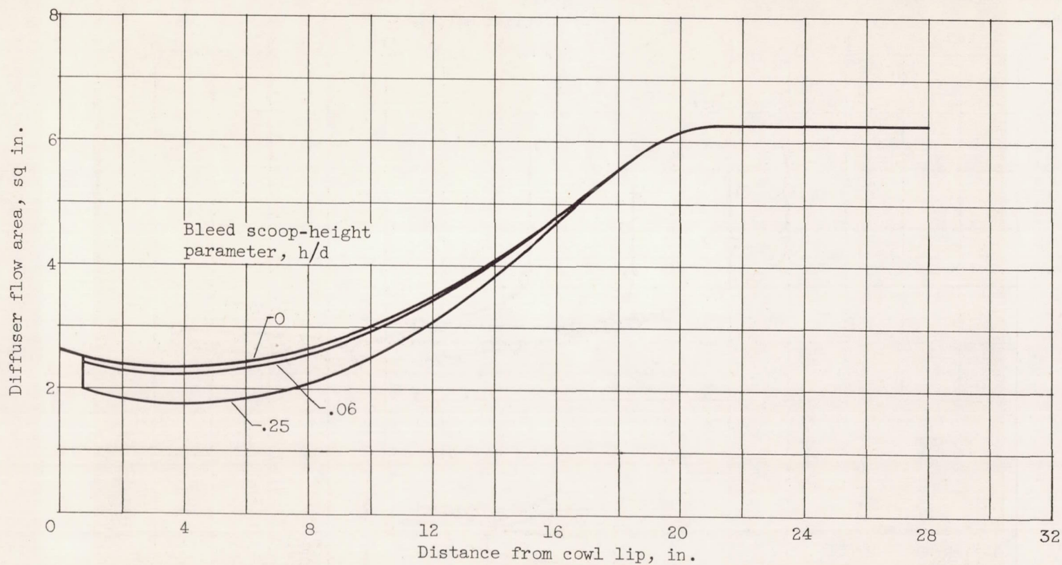
Figure 3. - Subsonic-diffuser area variations.
