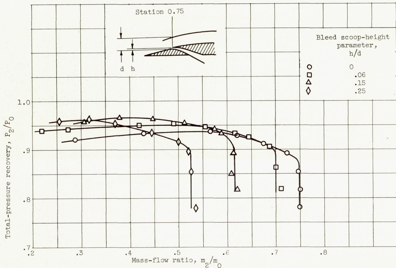
Figure 4. - Effect of internal-bleed scoop height on inlet performance.
