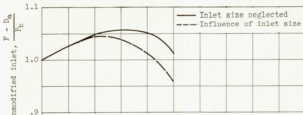
(a) Free-stream Mach number, 1.5.
