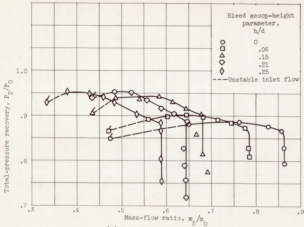
Figure 4. - Continued. Effect of internal-bleed scoop height on inlet performance.
