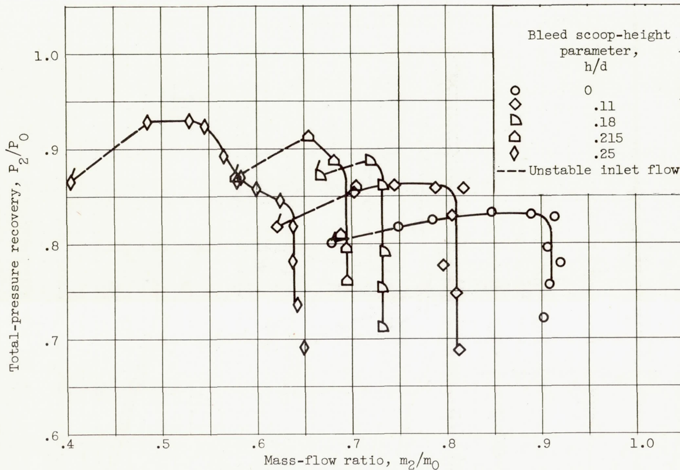
Figure 4. - Concluded. Effect of internal-bleed scoop height on inlet performance.
