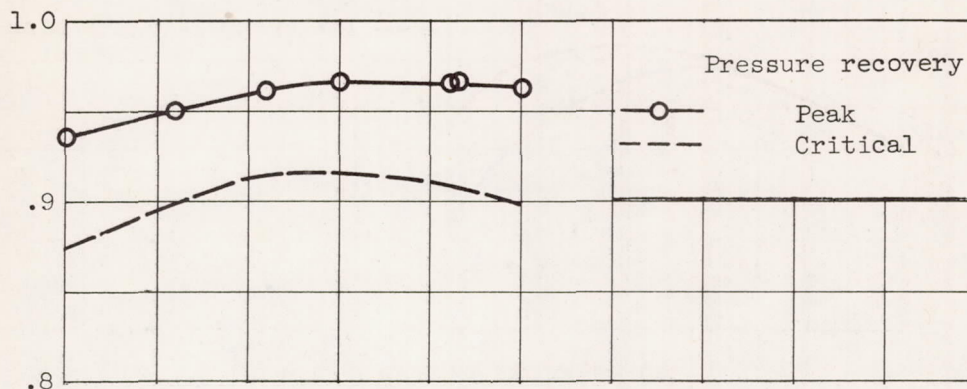
(a) Free-stream Mach number, 1.5.
