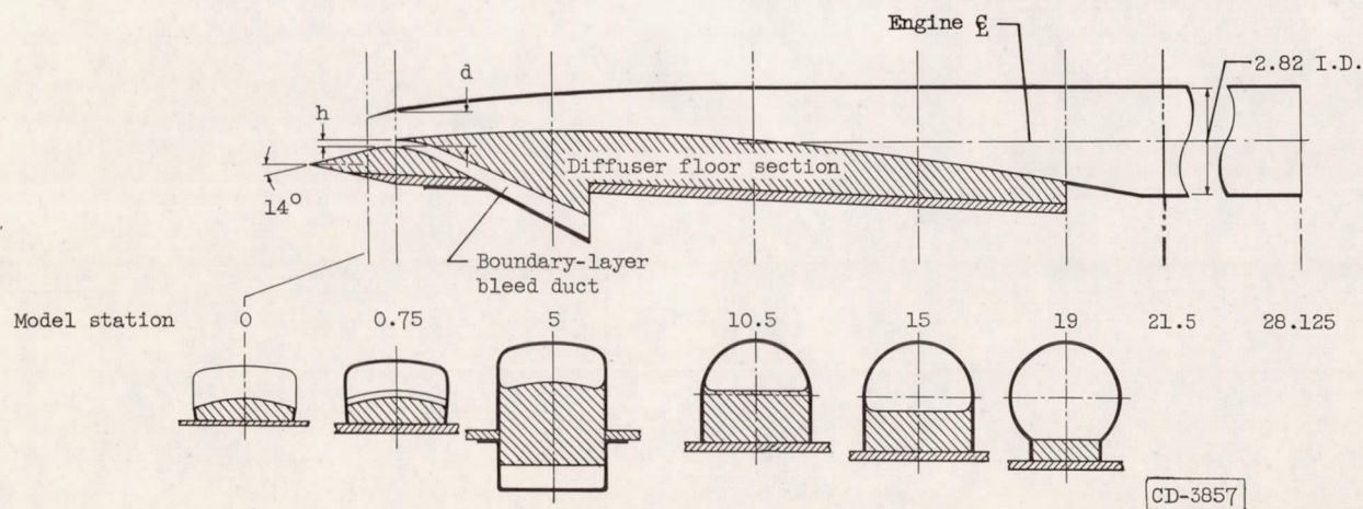
Figure 1. - Diagram of model with representative cross sections (all dimensions in inches).
